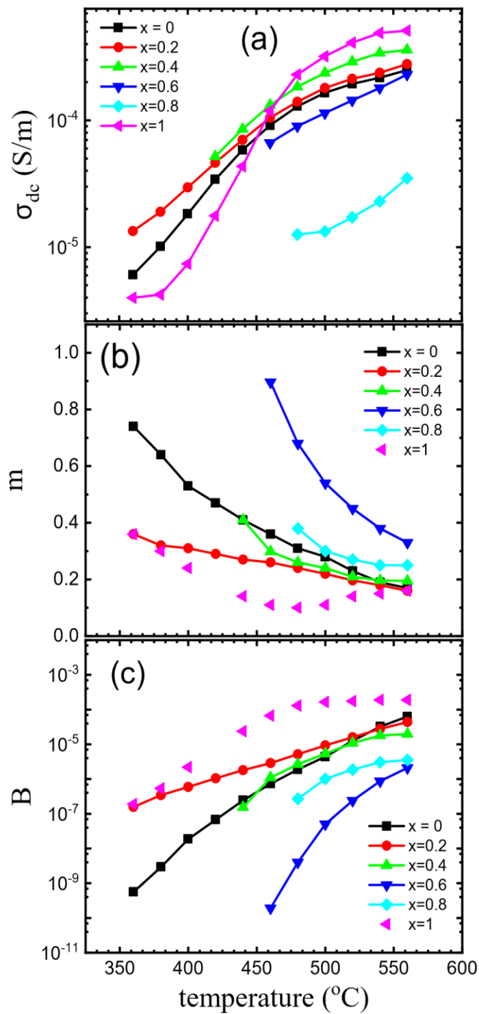
Fig. 4.8: The best fit parameters of the ac conductivity using Jonscher power law, (a) the dc conductivity (b) the exponent m , and (c) the constant B as a function of temperature for the \text{LaV}_{1-x}\text{Nb}_x\text{O}_4 ( x = 0-1 ) samples.
