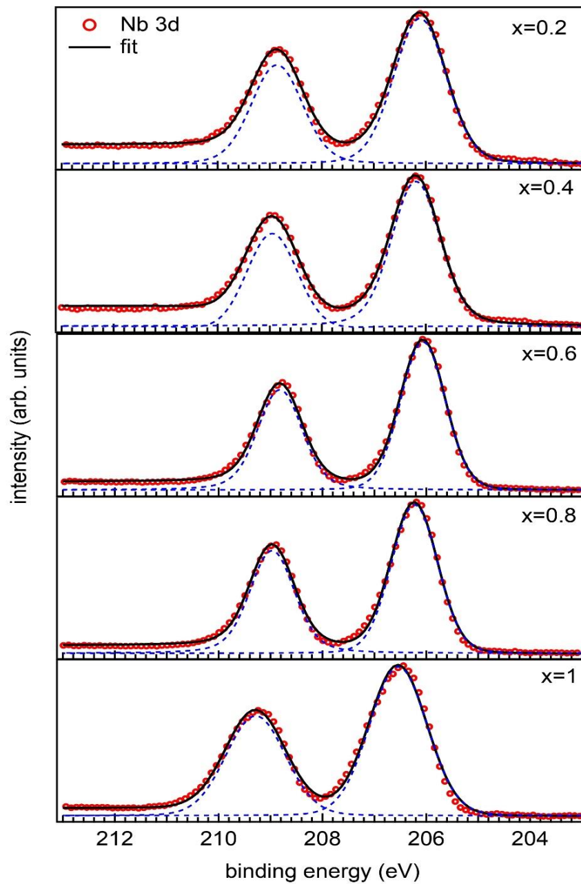
Fig. 3.7: The Nb 3d core level spectra of \text{LaV}_{1-x}\text{Nb}_x\text{O}_4 , x = 0-1 sample. The fitted spin-orbit split components are also shown for each sample.
