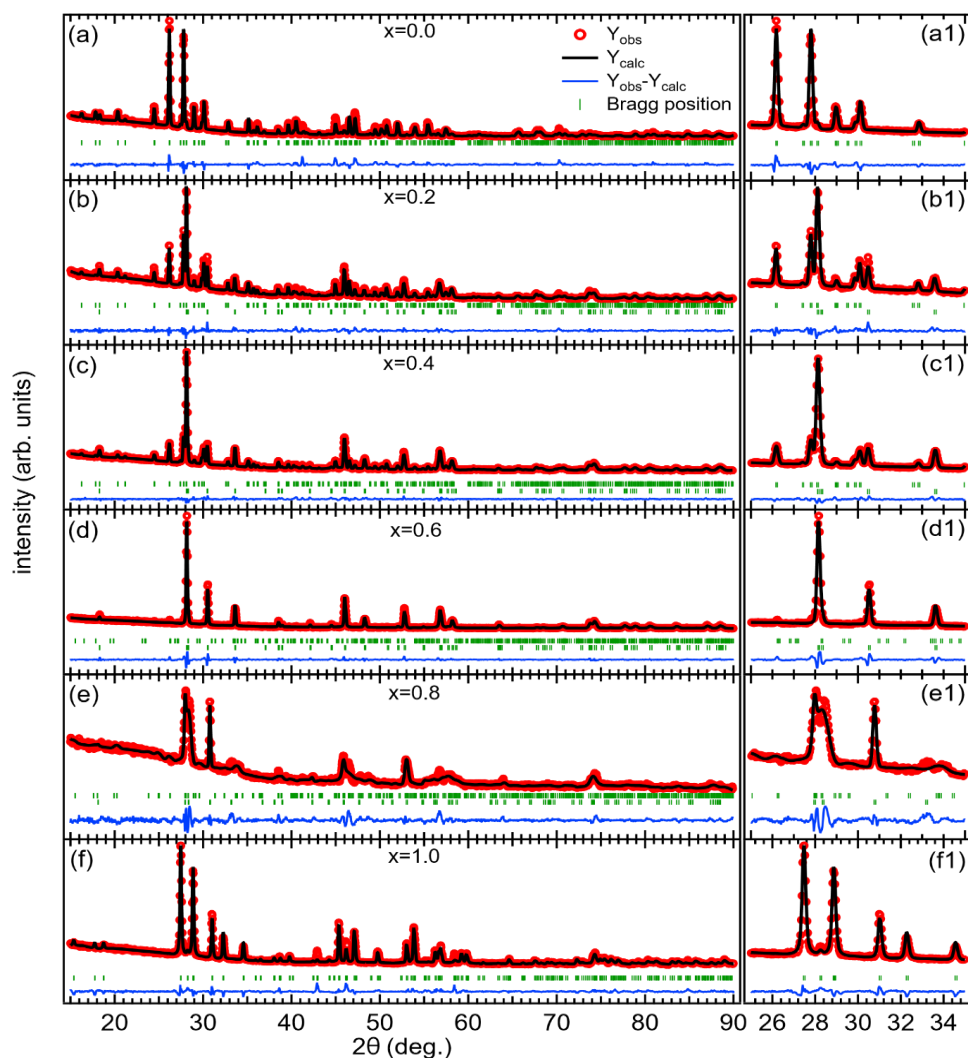
Fig. 3.1: (a–f) The Rietveld refined x-ray diffraction patterns of \text{LaV}_{1-x}\text{Nb}_x\text{O}_4 ( x = 0–1 ) samples. The experimental, simulated, and difference between the experimental and simulated spectra are shown by open red circles, black solid lines, and blue solid lines, respectively. The Bragg positions corresponding to their respective space groups are shown by green vertical markers. In the side of each panel (a1–f1), we show partial amplification for clarity between 2\theta = 25–35^\circ for all the samples.
