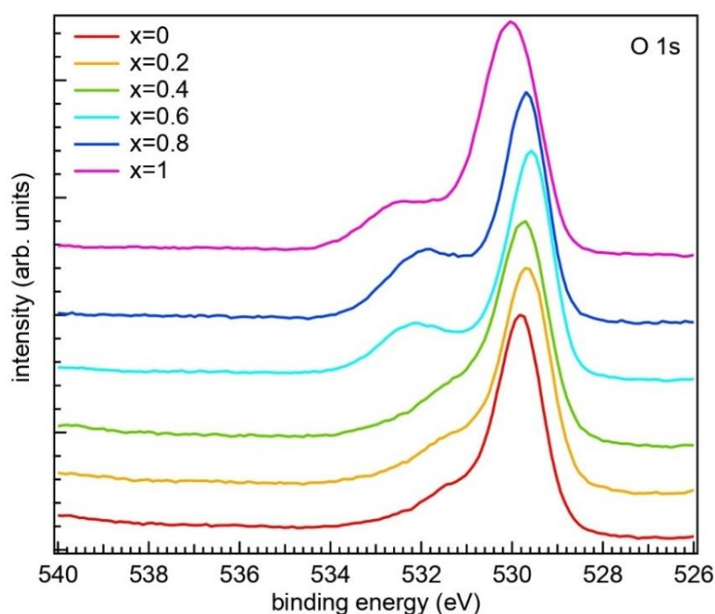
Fig. 3.8: The O 1s core level spectra of \text{LaV}_{1-x}\text{Nb}_x\text{O}_4 , x = 0-1 sample. Each spectrum is shifted vertically for the clarity.
