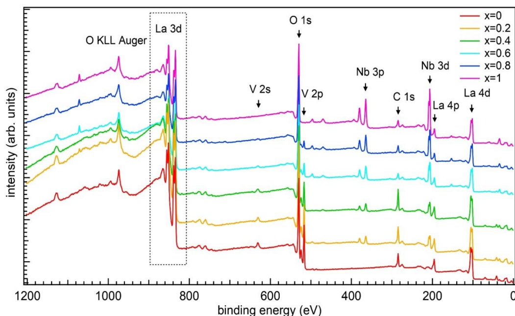
Fig. 3.5: The room temperature XPS survey spectra of \text{LaV}_{1-x}\text{Nb}_x\text{O}_4 ( x = 0 to 1 ) samples.
