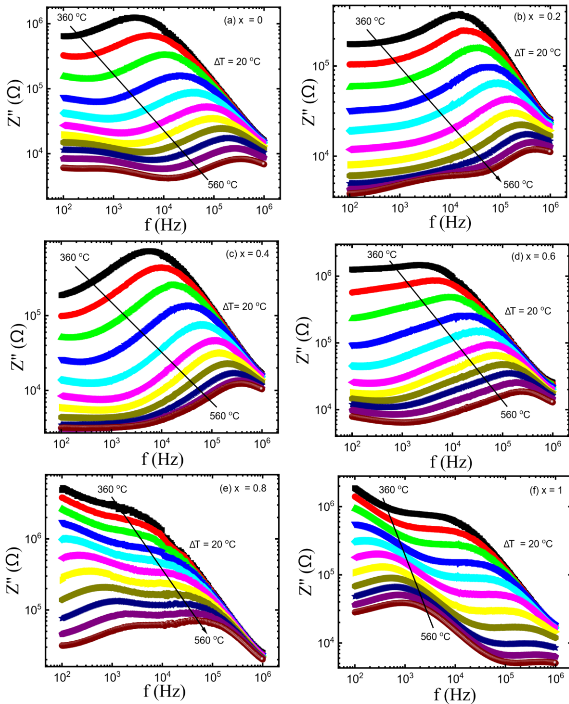
Fig. 4.4: (a-f) The imaginary part of impedance ( Z'' ) of \text{LaV}_{1-x}\text{Nb}_x\text{O}_4 ( x = 0-1 ) samples plotted as a function of frequency from 100 Hz to 1 MHz at the selected temperatures from 360°C–560°C.
