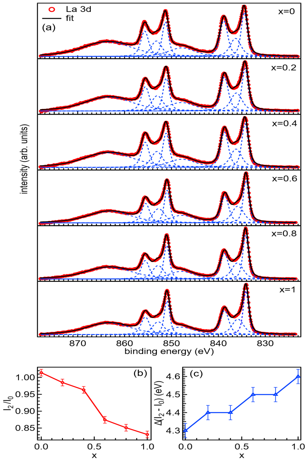
Fig. 3.6: (a) The La 3d core-level spectra of \text{LaV}_{1-x}\text{Nb}_x\text{O}_4 , x = 0-1 sample. (b) The intensity ratio I_2/I_0 , and (c) energy separation I_2 - I_0 as a function of doping level x . The fitted spin-orbit split components are also shown for each sample.
