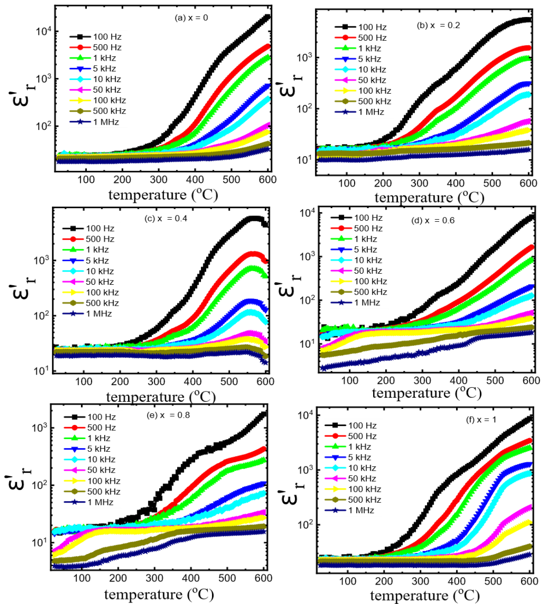
Fig. 4.1: (a–f) The temperature dependent real part of dielectric constant ( \epsilon'_r ) for \text{LaV}_{1-x}\text{Nb}_x\text{O}_4 ( x = 0-1 ) samples from 25^\circ\text{C} – 600^\circ\text{C} in the frequency range of 100 Hz–1 MHz.
