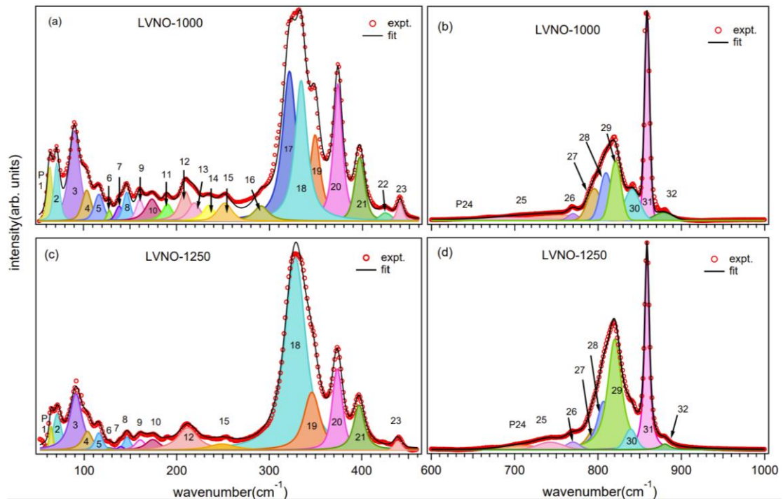
Fig. 5.4: The room temperature Raman spectra of LVNO sample, (a, b) sintered at 1000^{\circ}\text{C} and (c, d) for sample sintered at 1250^{\circ}\text{C} in the low and middle wavenumber regions, respectively; fitted using the Voigt peak function and solid thick black line presents the total fit of the measured spectra.
