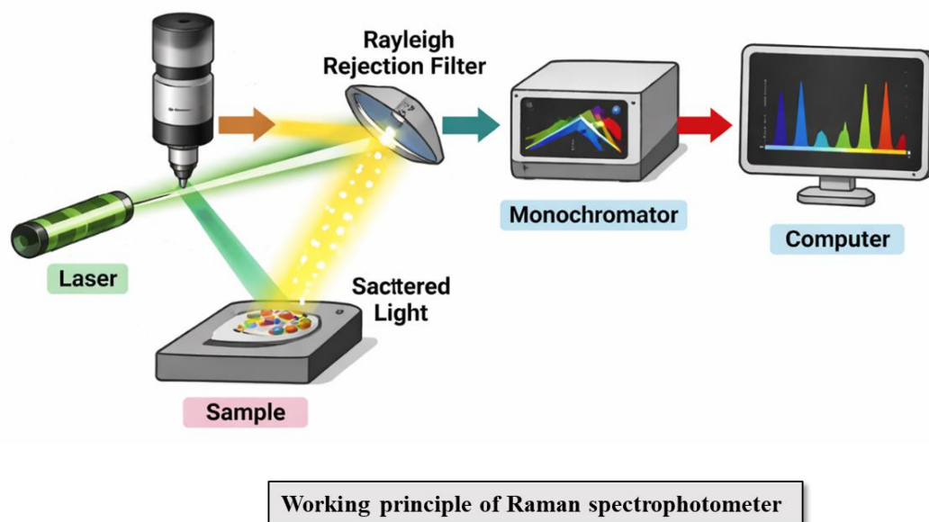
Fig. 2.5: Block diagram representation of working of Raman Spectroscope.
