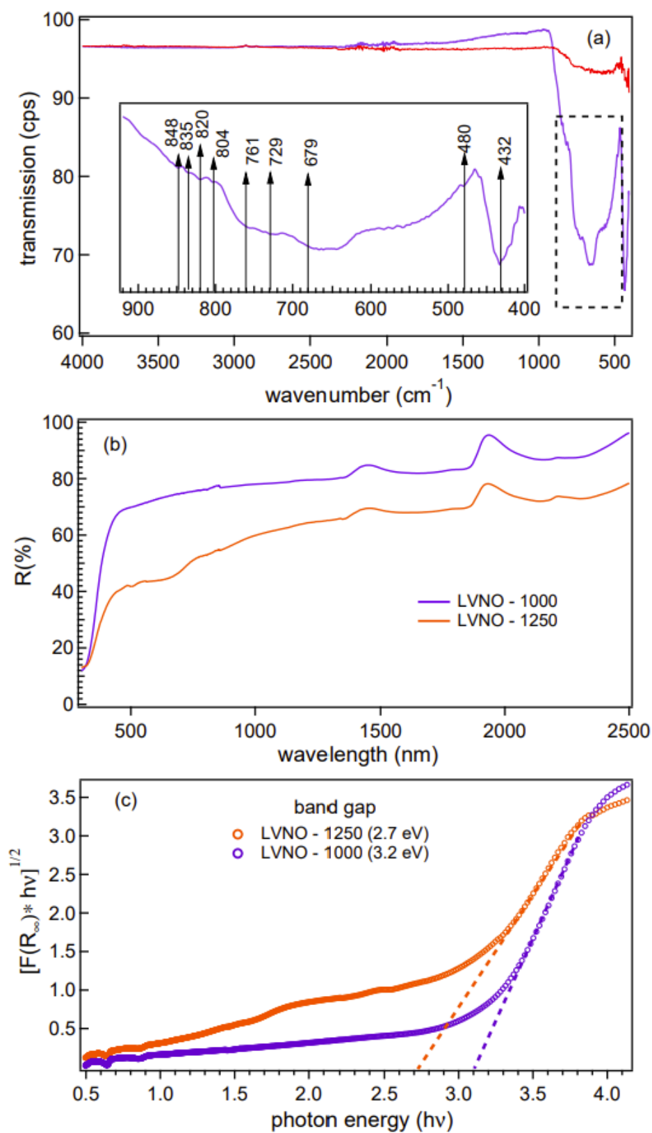
Fig. 5.3: (a) The FTIR spectra, (b) the UV-vis DRS plots and (c) the Kubelka-Munk plots obtained from the DRS data for the LVNO-1000 and LVNO-1250 samples, respectively.
