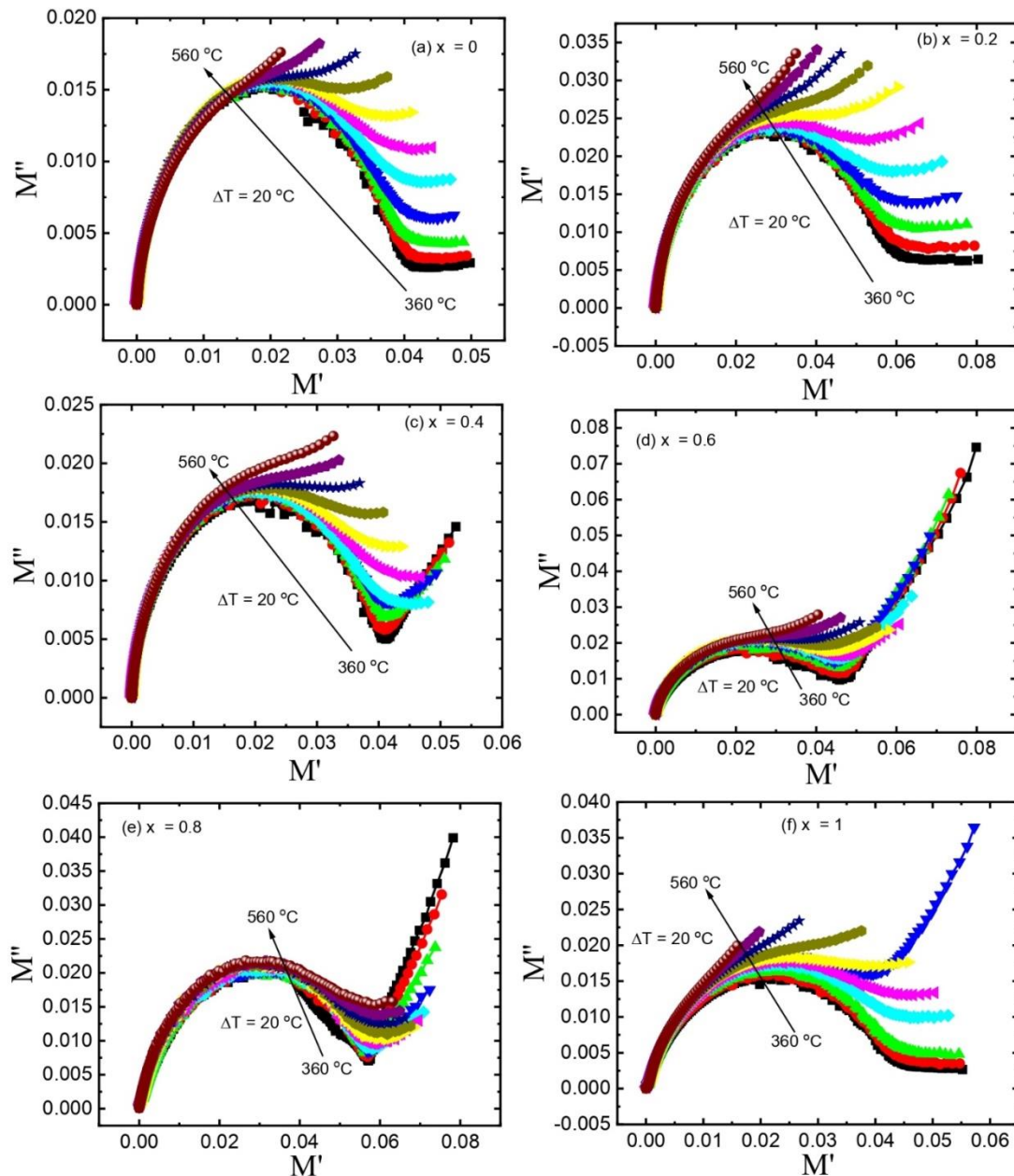
Fig. 4.5: (a-f) The imaginary ( M'' ) versus real ( M' ) parts of electric modulus as a function of frequency from 100 Hz to 1 MHz at various temperatures from 360°C to 560°C for the \text{LaV}_{1-x}\text{Nb}_x\text{O}_4 ( x = 0 - 1 ) samples.
