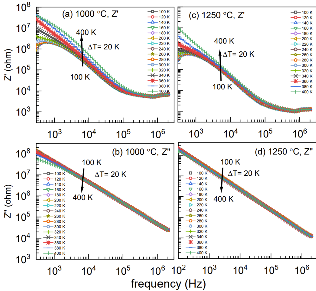
Fig. 5.7: The real ( Z' ) and imaginary ( Z'' ) parts of total impedance ( Z ), (a, b) for the LVNO-1000 and (c, d) for the LVNO-1250 samples. The arrow shows the direction of increasing temperatures.
