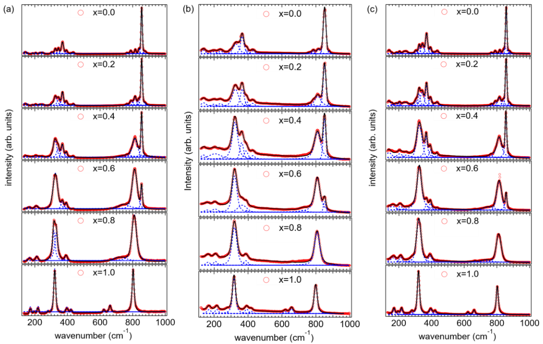
Fig. 3.4: The room temperature Raman spectra of \text{LaV}_{1-x}\text{Nb}_x\text{O}_4 ( x = 0 to 1) samples using (a) 532 nm, (b) 633 nm, and (c) 785 nm excitation wavelengths. The dotted blue lines represent the Lorentzian line shape to deconvolute the individual modes.
