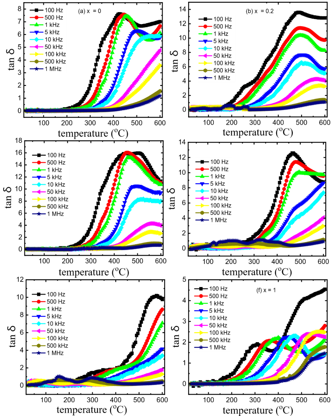
Fig. 4.2: (a–f) The dielectric loss ( \tan \delta ) for \text{LaV}_{1-x}\text{Nb}_x\text{O}_4 ( x = 0-1 ) samples plotted as a function of temperature at the selected frequencies.
