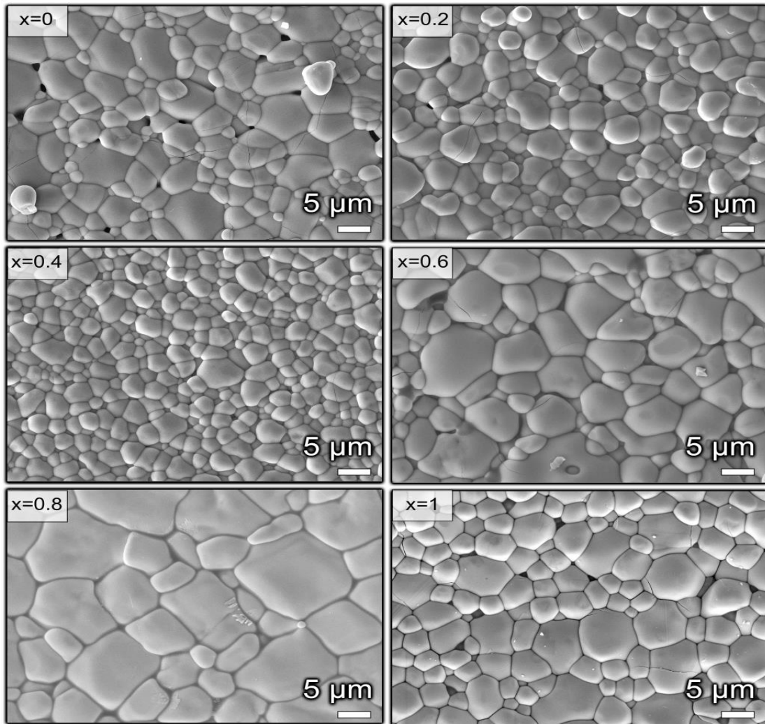
Fig. 3.2: The scanning electron microscope images of the \text{LaV}_{1-x}\text{Nb}_x\text{O}_4 ( x = 0-1 ) samples.
