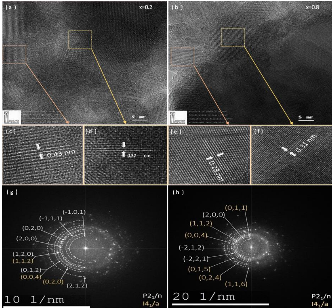
Fig. 3.3: The HR-TEM images of \text{LaV}_{1-x}\text{Nb}_x\text{O}_4 for the (a) x = 0.2 and (b) x = 0.8 samples. The magnified view of HRTEM images in (c, d) for the x = 0.2 sample, and (e, f) for the x = 0.8 sample. (g, h) The SAED patterns for the x = 0.2 and 0.8 samples, respectively.
