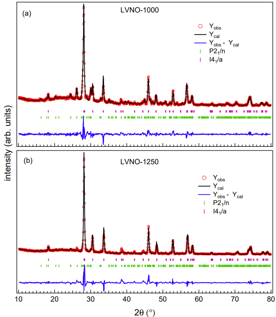
Fig. 5.1: The room temperature XRD patterns with Rietveld refinement of (a) LVNO-1000 and (b) LVNO-1250 samples. The open red circles, black solid line, and blue solid line exhibits the experimental, calculated, and the difference between experimental and calculated pattern, respectively. The vertical green and purple markers show the Bragg positions corresponding to the P2_1/n and I4_1/a space groups.
