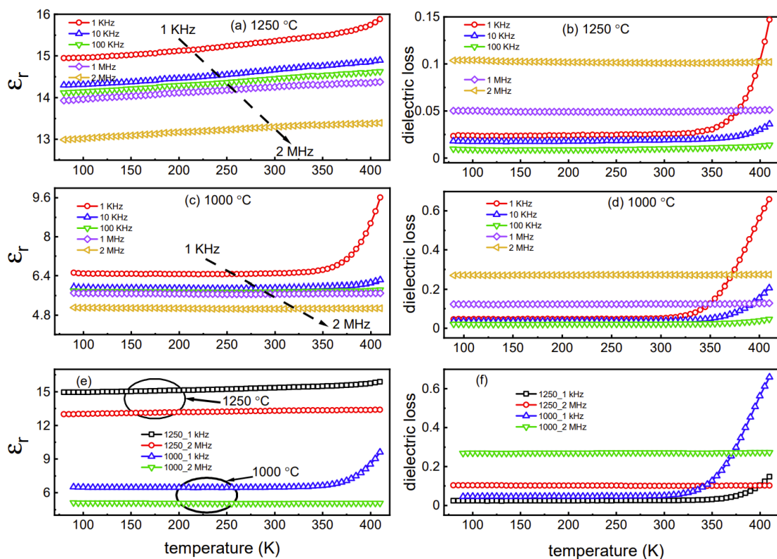
Fig. 5.6: The variations of electric permittivity ( \epsilon_r ) and dielectric loss at various temperatures for selected frequencies for both the samples, sintered 1000°C and 1250°C temperatures; (a-d) the variations of electric permittivity and dielectric loss at various temperatures, (e-f) a comparison of electric permittivity and dielectric loss at two different frequencies of 1 kHz and 2 MHz, respectively. The arrow in this figure shows the direction of increasing frequency.
