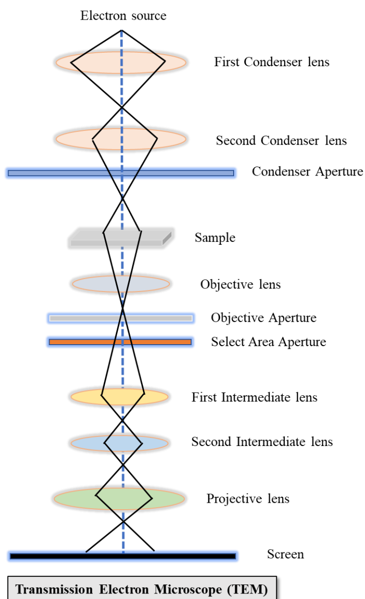
Fig. 2.4: Image formation using a Transmission Electron Microscope.
