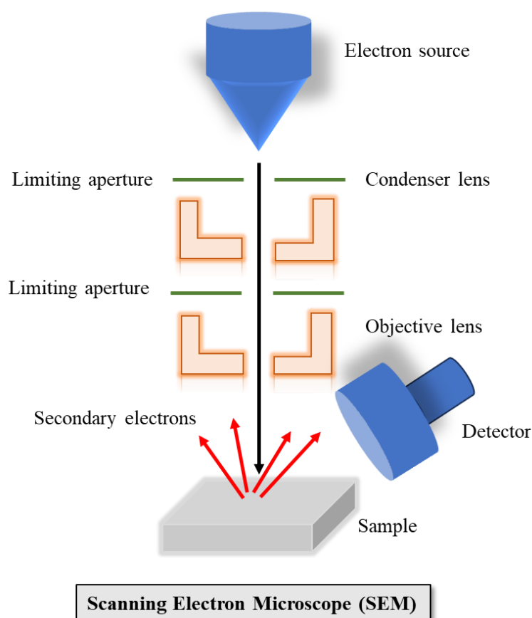
Fig. 2.3: Diagram showing path of electron beam inside SEM.
