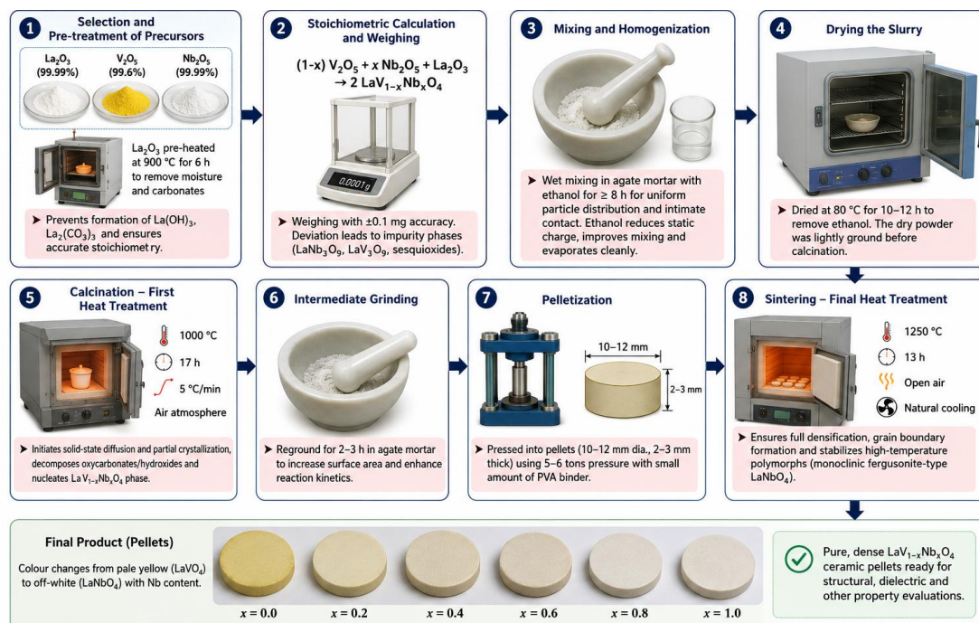
Fig. 2.1: Schematic diagram showing step by step synthesis using solid state route.
