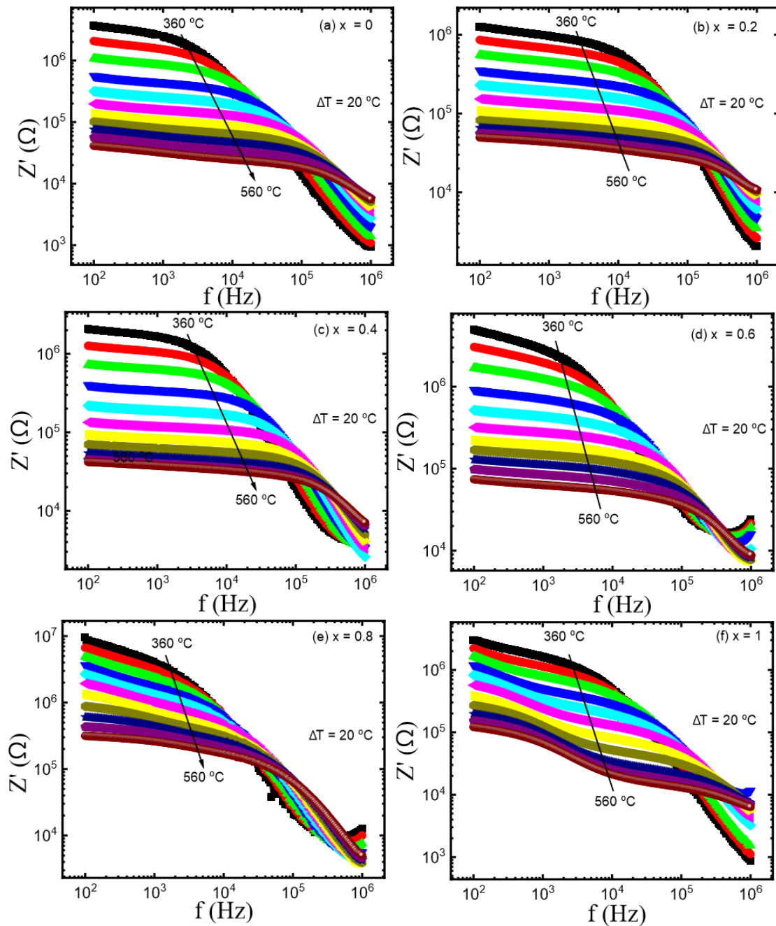
Fig. 4.3: (a–f) The real part of impedance ( Z' ) of \text{LaV}_{1-x}\text{Nb}_x\text{O}_4 ( x = 0-1 ) samples plotted as a function of frequency from 100 Hz to 1 MHz at the selected temperature from 360°C–560°C.
