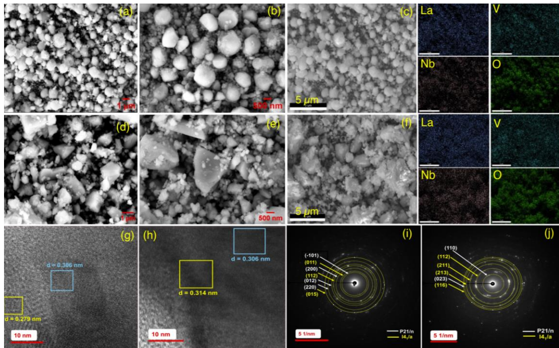
Fig. 5.2: The FE-SEM images of the LVNO-1000 sample at (a) 1 \mu\text{m} , (b) 500 nm and (c) probed region of scan (at 5 \mu\text{m} ) with the corresponding elemental mappings of all elements; the FE-SEM images of the LVNO-1250 sample at (d) 1 \mu\text{m} , (e) 500 nm and (f) probed region of scan (at 5 \mu\text{m} ) with the corresponding elemental mappings of all elements; the HR-TEM images of (g) sintered at 1000°C and (h) sintered at 1250°C with the marked d-spacings across the selected region; the SAED patterns for the LVNO-1000 (i) and LVNO-1250 (j), respectively.
