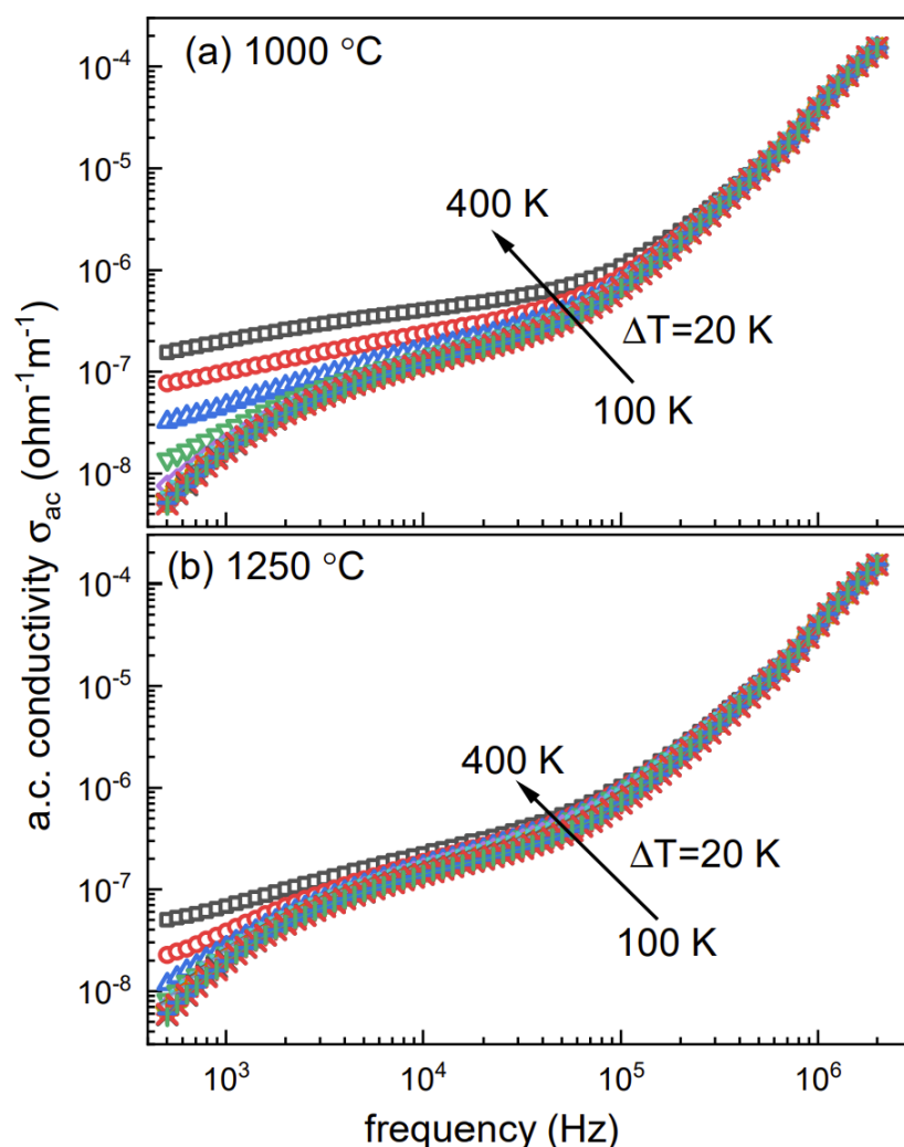
Fig. 5.8: The variation of ac conductivity with frequency for (a) 1000°C and (b) 1250°C sintered samples. The arrow shows the direction of increasing temperature.
