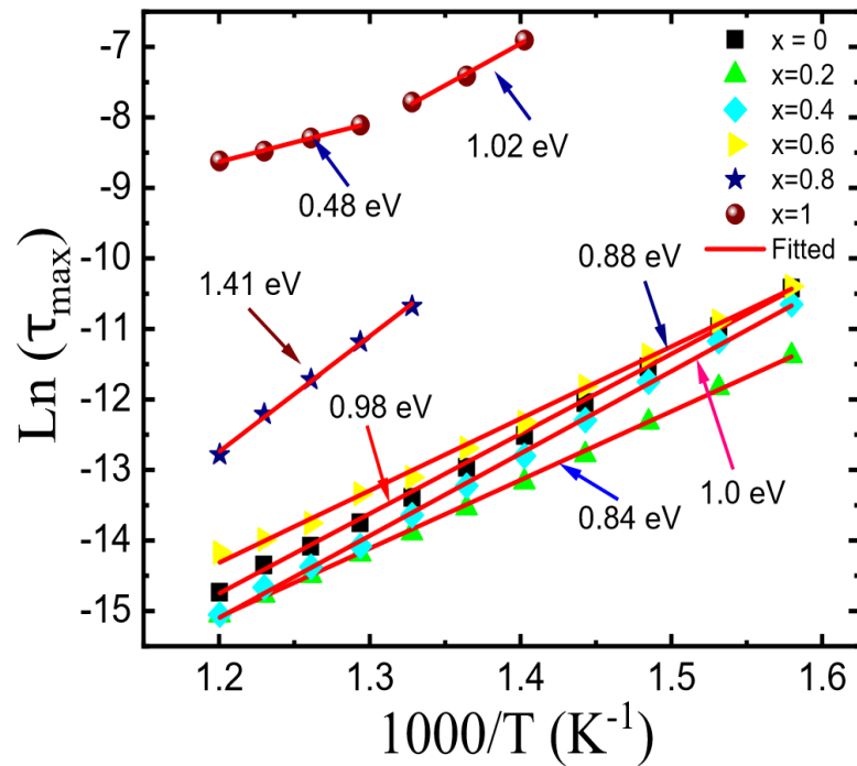
Fig. 4.6: The variation in the relaxation time with inverse of the temperature for \text{LaV}_{1-x}\text{Nb}_x\text{O}_4 ( x = 0-1 ) samples. The solid red lines represent the best fit using the Arrhenius equation.
