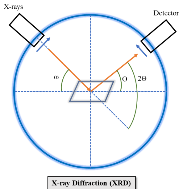
Fig. 2.2: X-ray diffraction working principle.
