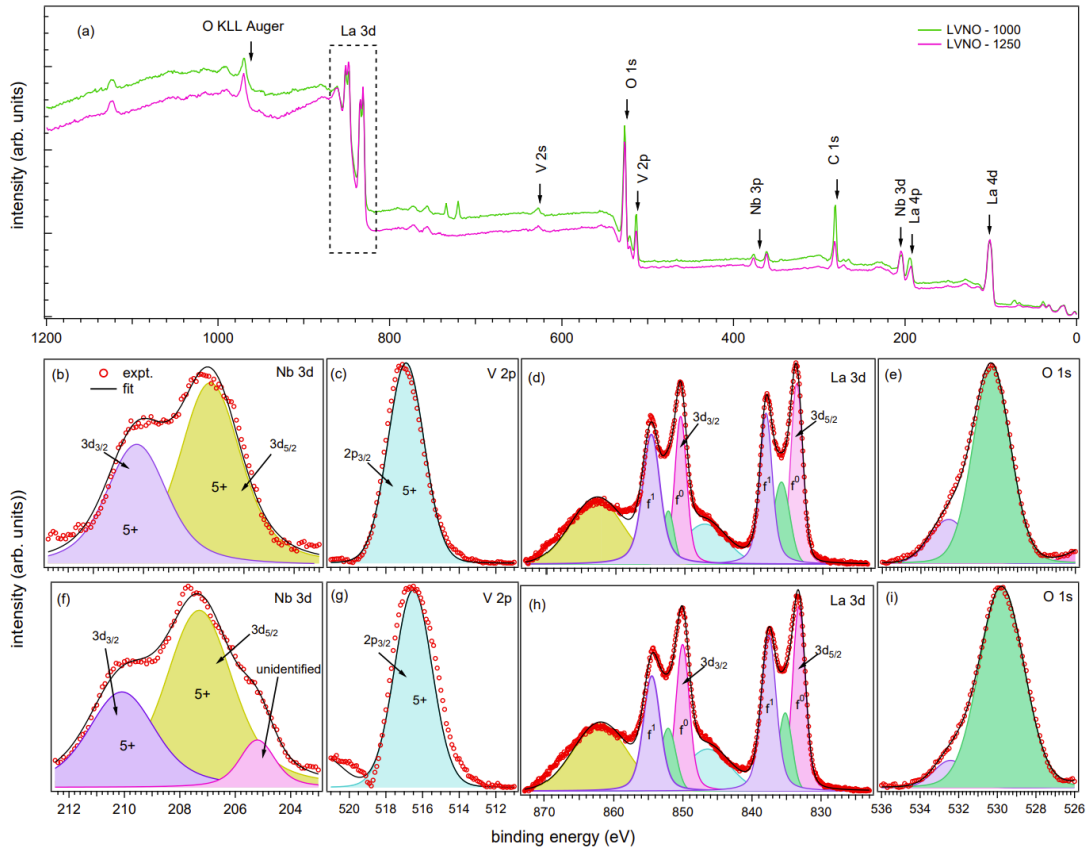
Fig. 5.5: (a) The room temperature XPS survey spectrum; the core level spectra of (b, f) Nb 3d; (c, g) V 2p; (d, h) La 3d and (e, i) O 1s elements of the LVNO sample sintered at 1000°C (b, c, d, e) and 1250°C (f, g, h, i), respectively.
