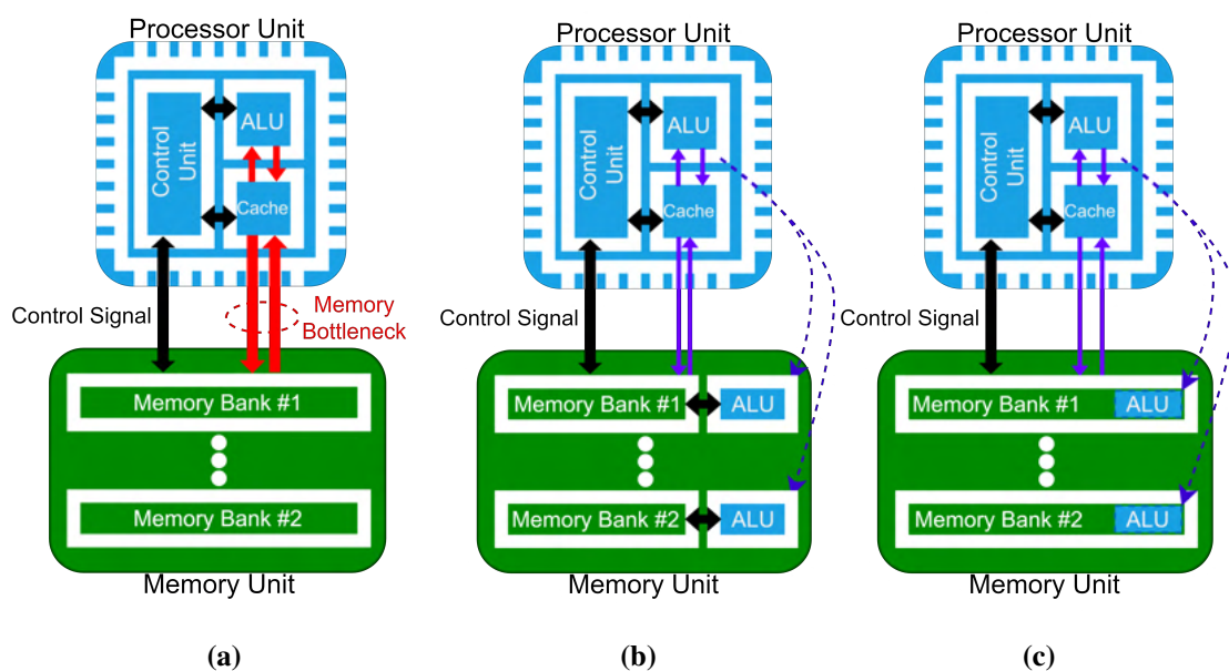
Figure 1.4: Memory bottleneck dilemma and architectural alternatives: (a) conventional von Neumann organization, (b) near-memory computing, (c) in-memory computing.
