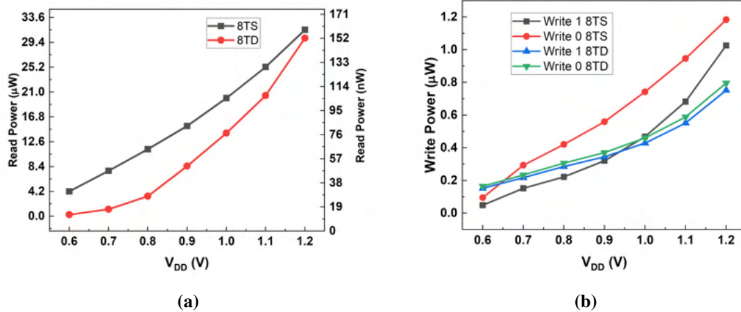
Figure 3.15: Comparison of (a) Read power ( \mu W ) (b) Write power ( \mu W ) of 8TS and 8TD SRAM Cells as a function of supply voltage
