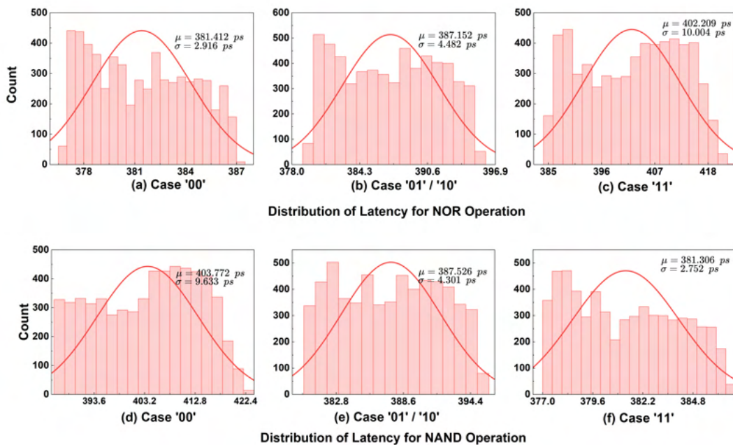
Figure 4.7: Distribution of latency for NOR and NAND logic operation for all possible combinations of input operands (AB), '00,01,10,11' for 6k Monte Carlo simulation runs at T = 300.15 K and V_{DD} = 0.8 V with \Delta V_{TH} = 50 mV.
