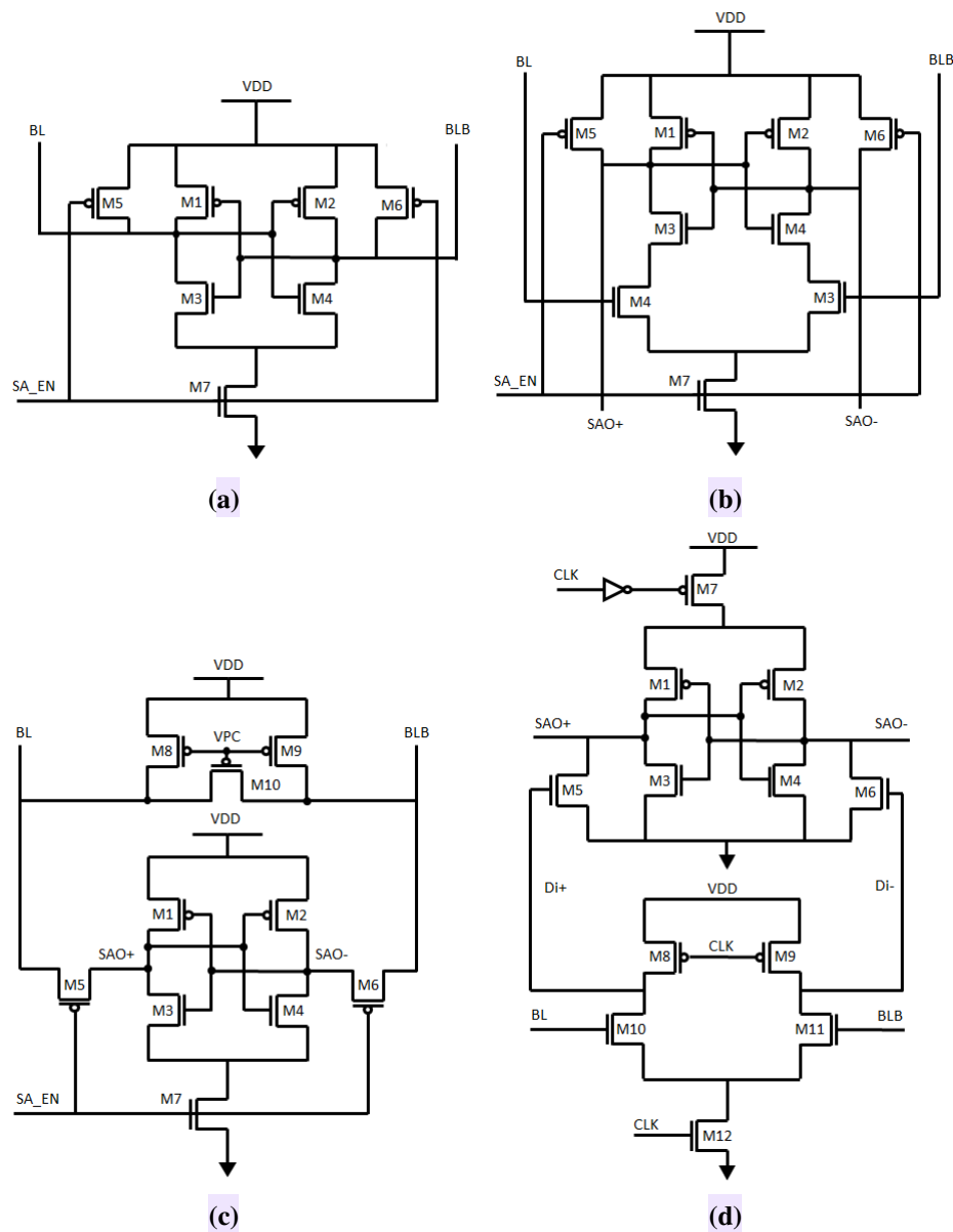
Figure 2.6: Circuit schematics for Voltage SAs (a) Conventional latch-type SA, (b) Current-controlled latch-type SA, (c) Decoupled latch-type SA, and (d) Double tail SA.
