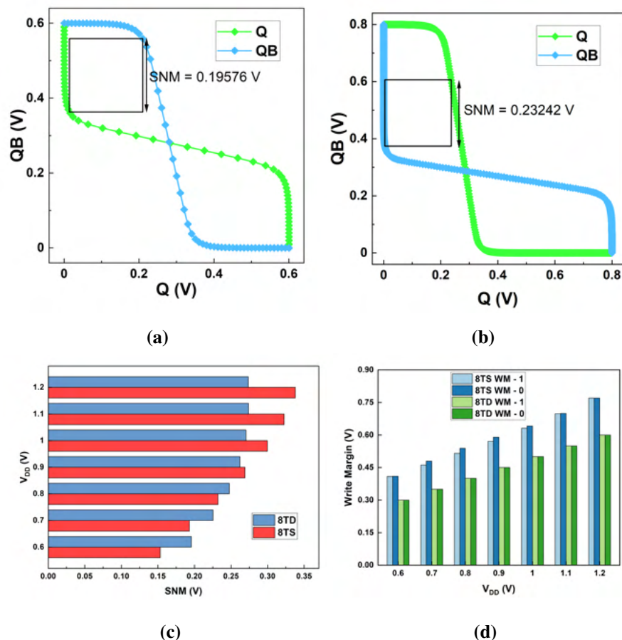
Figure 3.13: Butterfly Curve for calculation of static noise margin (SNM) (a) differential 8TD SRAM cell and (b) single-ended 8TS SRAM cell. (c) Impact of voltage scaling on (c) SNM and (d) Write margin (WM) of 8TD and 8TS cells.
