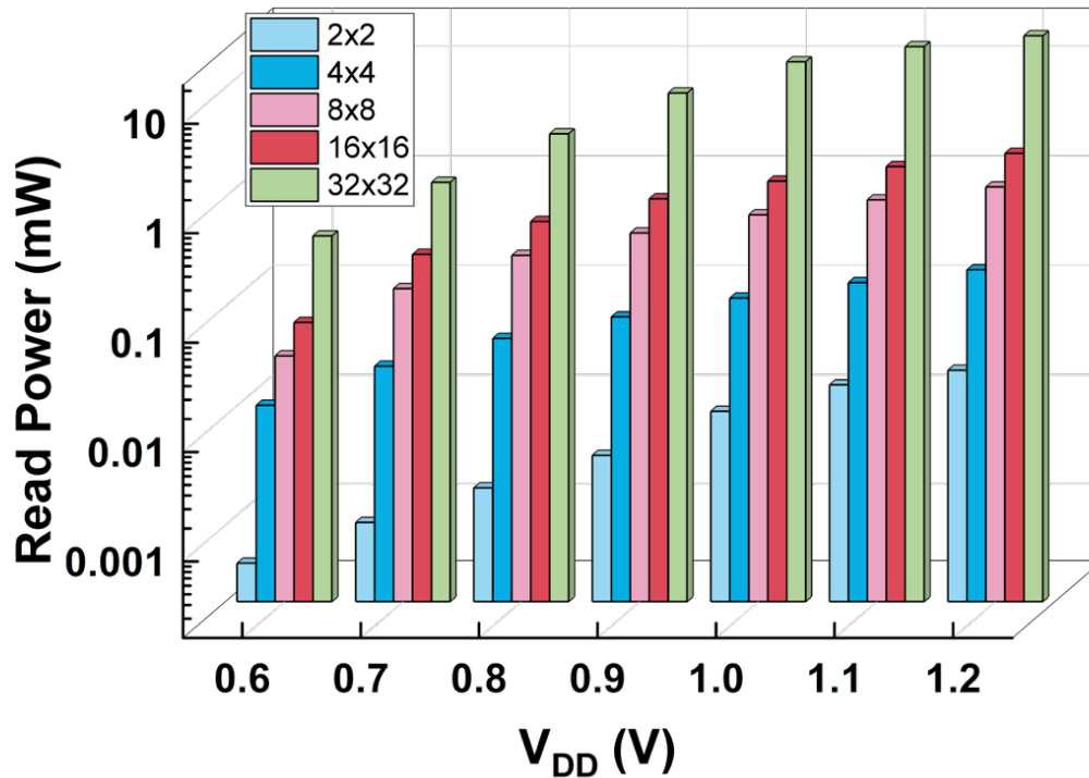
Figure 5.5: Read-power variation with array size from 2 \times 2 to 32 \times 32 across the supply-voltage sweep. The logarithmic y-axis highlights the wide power spread under array scaling.
