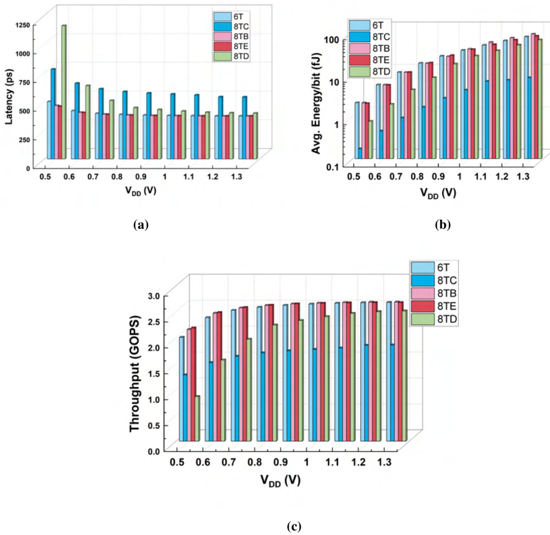
Figure 4.11: Performance comparison of SRAM-IMC cell architectures as a function of V_{DD} at the TT process corner and T = 300.15 K: (a) latency, (b) average energy per bit, and (c) throughput for 6T, 8TC, 8TB, 8TE, and 8TD SRAM-IMC cells.
