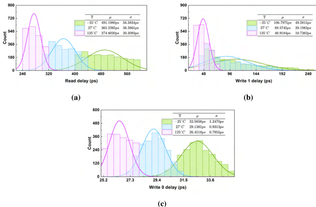
Figure 3.6: Temperature-dependent delay analysis of the proposed 8TS SRAM bit-cell for read and write operations at V_{DD} = 0.8 V. (A) Read delay, (B) Write-1 delay, and (C) Write-0 delay histograms, highlighting the impact of temperature variations on SRAM cell performance.
