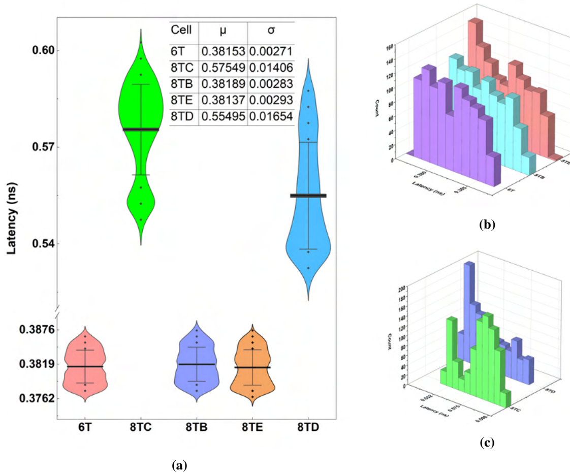
Figure 4.10: SRAM-IMC latency distributions under device mismatch at V_{DD} = 0.8 V and \Delta V_{TH} = 50 mV: (a) violin-plot summary with extracted \mu and \sigma , (b) Monte Carlo latency distribution for the fast cluster consisting of 6T, 8TB, and 8TE cells, and (c) Monte Carlo latency distribution for the higher-latency 8TC and 8TD cells.
