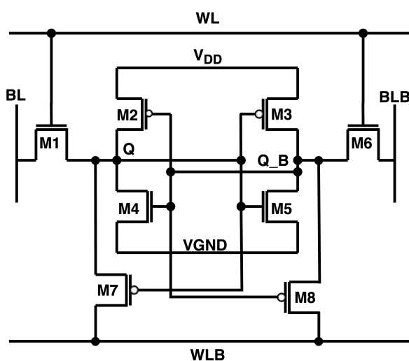
Figure 3.12: Circuit diagram of the proposed differential 8TD SRAM cell
