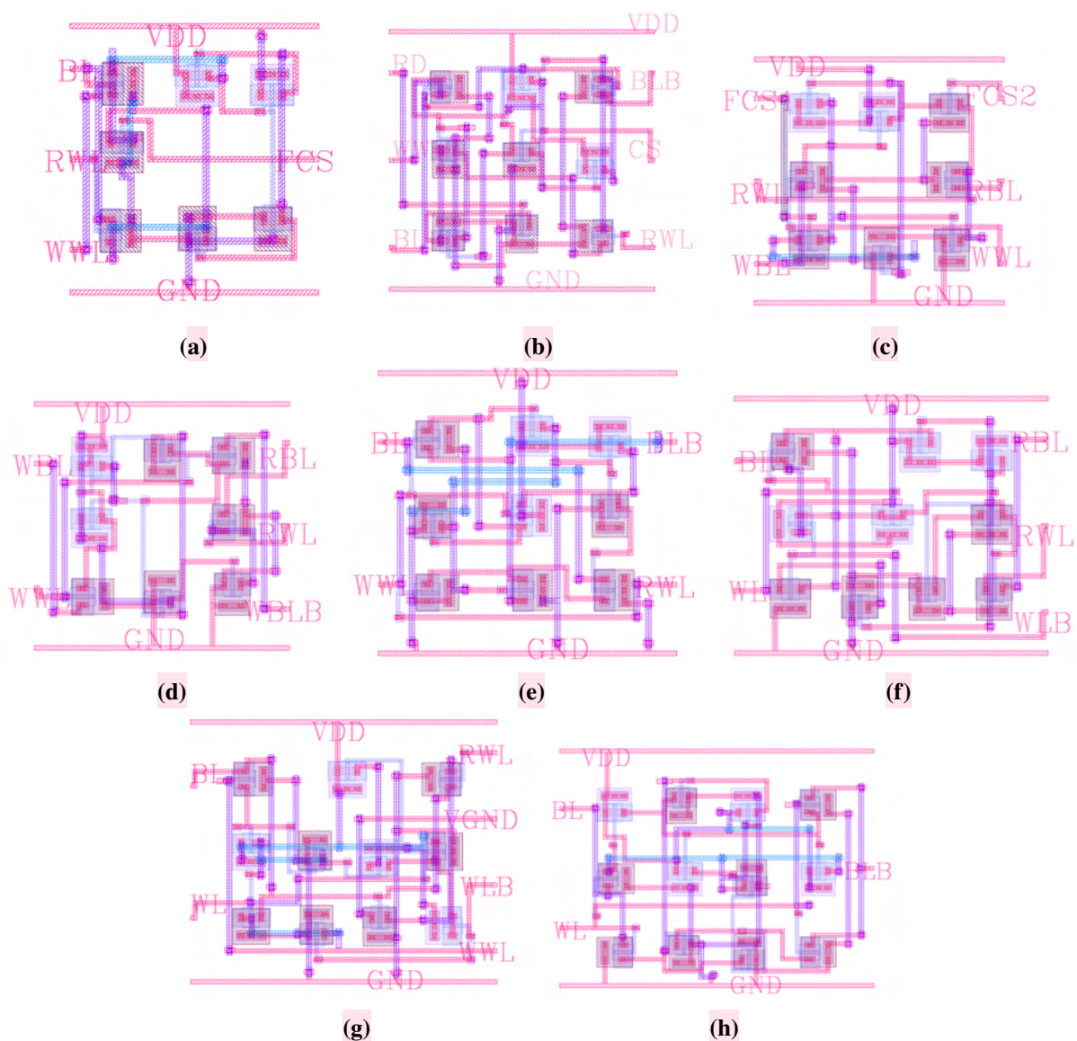
Figure 3.11: Layout representations of different SRAM bit-cells (7T–12T) used for comparative analysis, illustrating transistor arrangement and routing complexity: (A) 7T, (B) 8Ta, (C) 8Tb, (D) 8Tc, (E) 9T, (F) 10T, (G) 11T, and (H) 12T. Note: Layouts are not optimized for array-level implementation.
