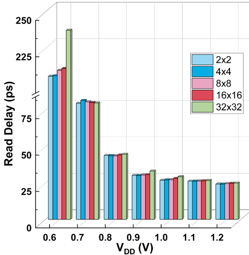
Figure 5.4: Read-delay variation with array size from 2 \times 2 to 32 \times 32 across the supply-voltage sweep.
