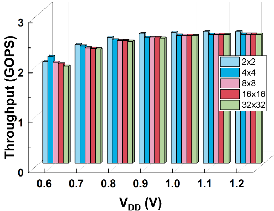
Figure 5.8: Compute-mode throughput of the proposed SRAM-IMC array for 2×2 to 32×32 organizations across V_{DD} = 0.6\text{--}1.2 V.
