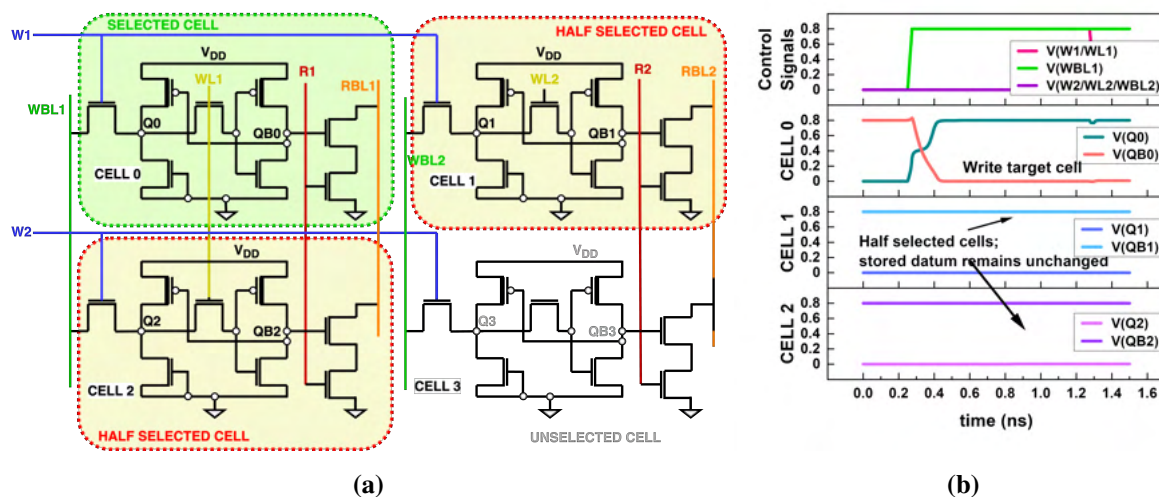
Figure 3.7: Illustration of half-select resilience in the proposed 8TS SRAM bit-cell. (A) A 2x2 array of 8TS SRAM cells, highlighting the selected, half-selected, and unselected cells. (B) Transient response of control signals and storage node voltages for selected, half-selected, and unselected cells, demonstrating the robustness of the proposed design.
