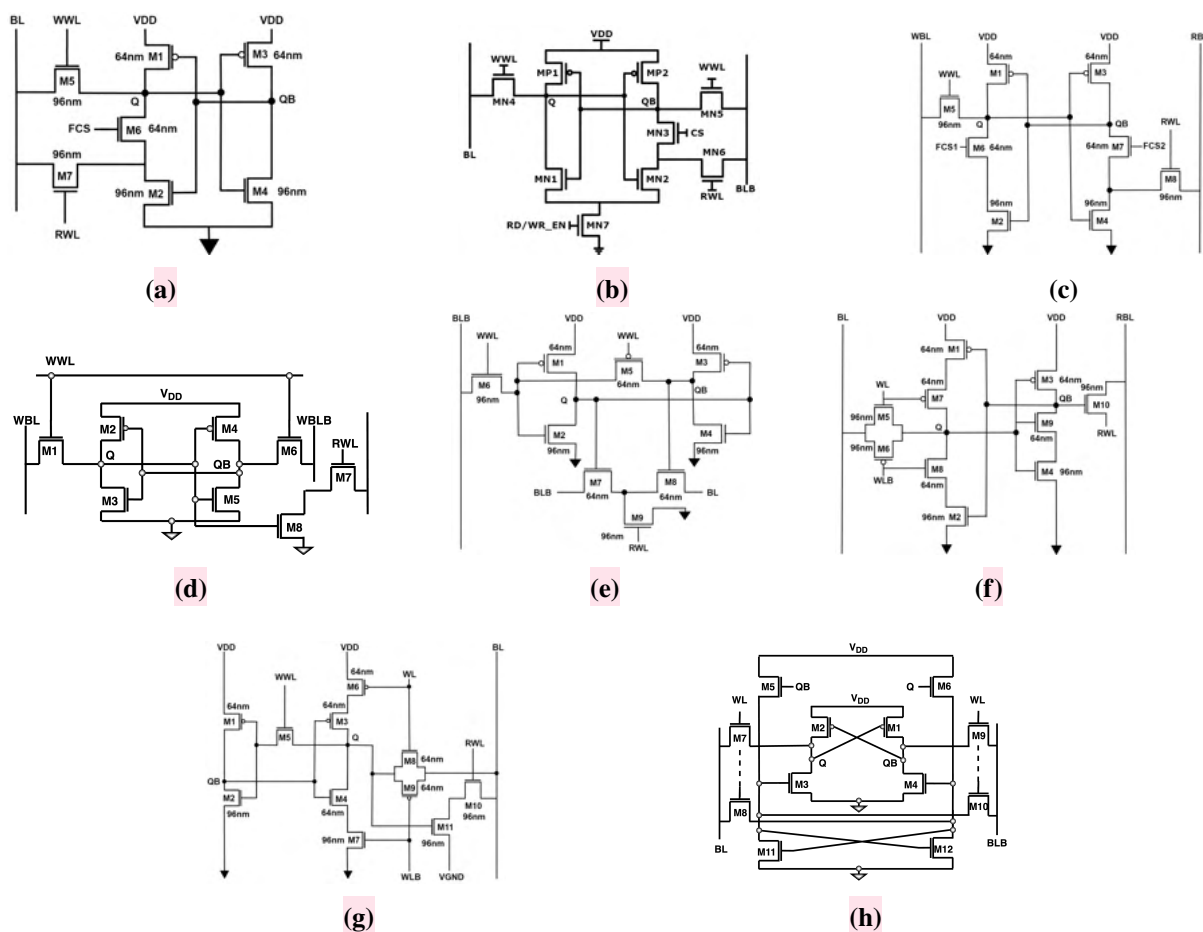
Figure 3.8: Circuit schematics of existing SRAM bit-cells with varied transistor count (A) 7T, (B) 8Ta, (C) 8Tb, (D) 8Tc, (E) 9T, (F) 10T, (G) 11T, and (H) 12T.
