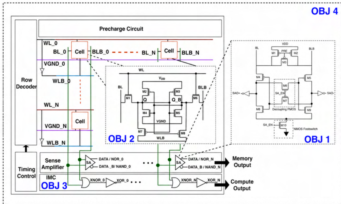
Figure 5.1: Proposed reconfigurable SRAM-IMC architecture showing the shared memory-mode and compute-mode data paths.
