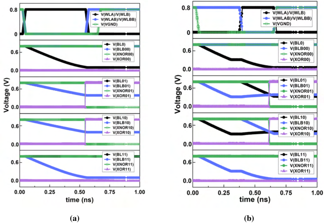
Figure 4.5: Transient response for compute mode of proposed 8TD SRAM cell for all possible input operand combinations (AB), '00,01,10,11' using (a) concurrent word-line and (b) sequential word-line activations at V_{DD} = 0.8 V.
