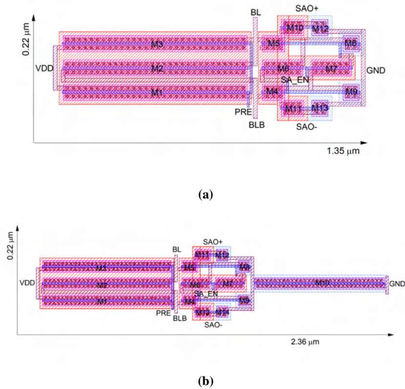
Figure 2.12: Layout design for area estimation of (a) MDSA and (b) MDSANF
