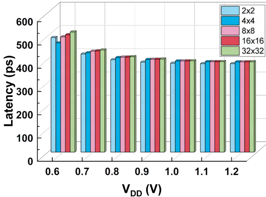
Figure 5.6: Compute-mode NAND-evaluation latency of the proposed SRAM-IMC array for 2 \times 2 to 32 \times 32 organizations across V_{DD} = 0.6\text{--}1.2 V.
