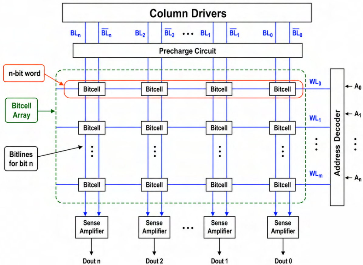
Figure 1.1: Basic organization of an SRAM array showing the bitcell matrix, wordline selection through the address decoder, differential bitline pairs, column drivers, precharge circuit, and sense-amplifier readout path.
