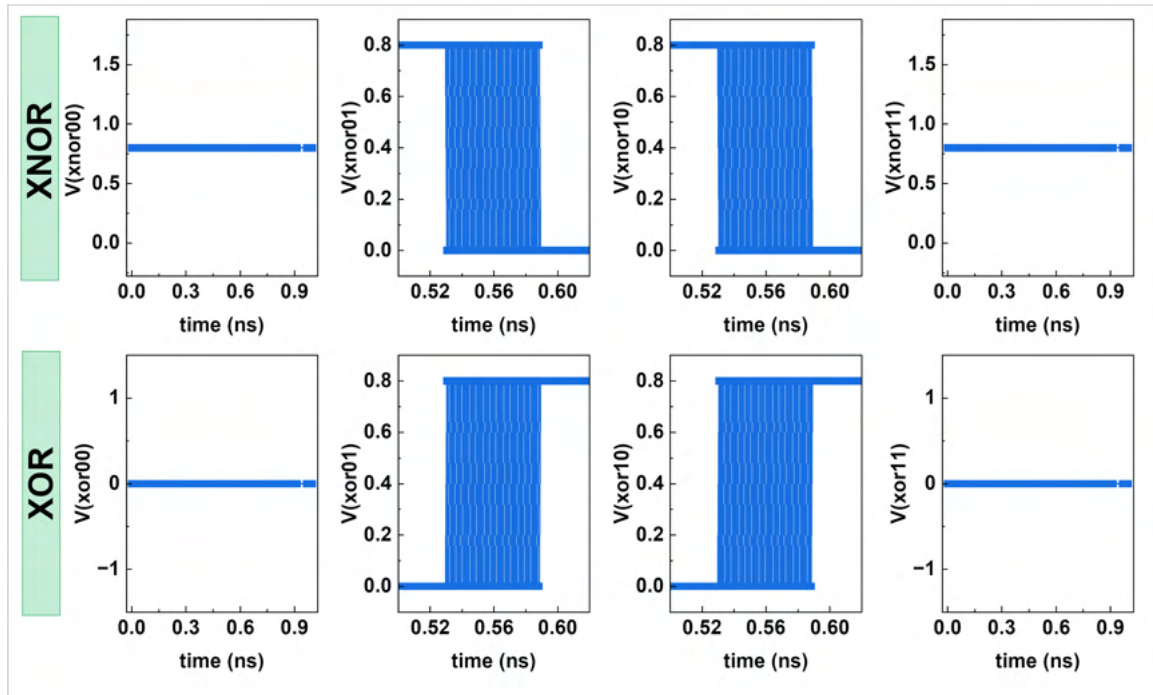
Figure 4.8: Transient simulations for (a) XNOR and (b) XOR logic operations for all possible input operand combinations, AB = 00, 01, 10 , and 11 . The results are obtained from 2000 Monte Carlo simulation runs at T = 300.15 K, V_{DD} = 0.8 V, and \Delta V_{TH} = 50 mV.
