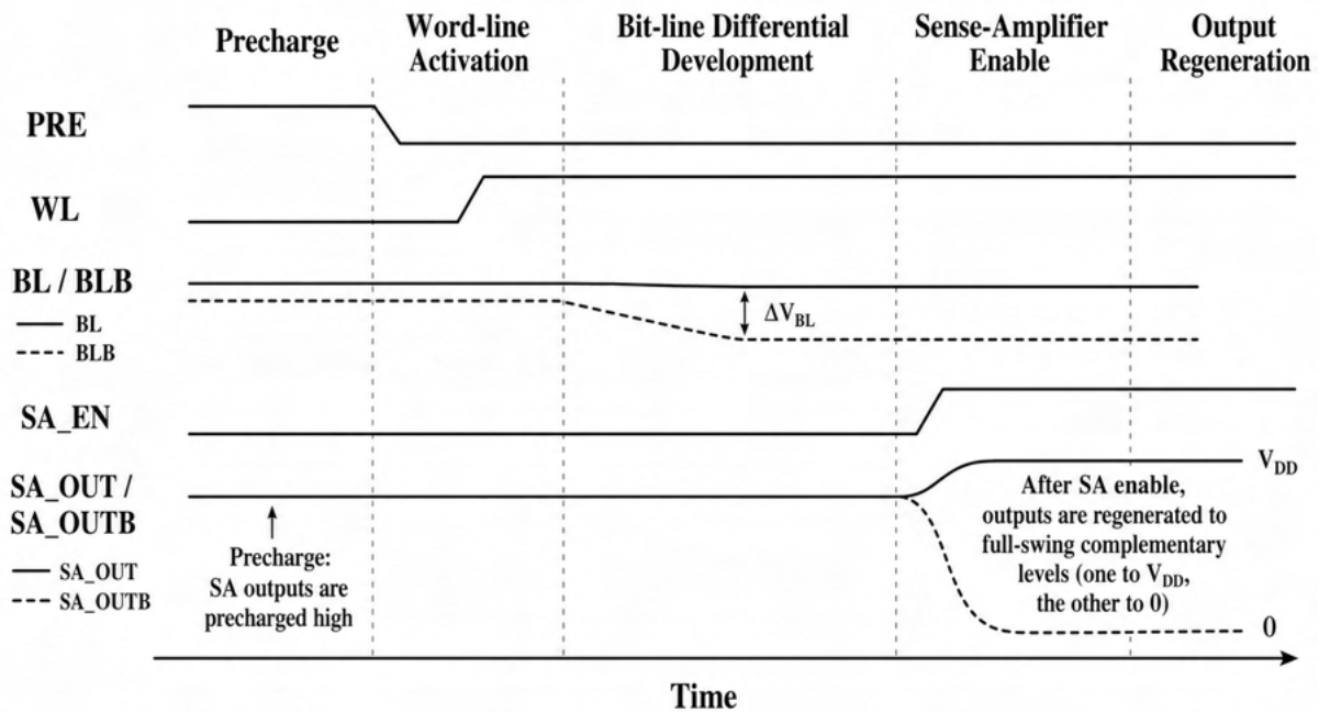
Figure 1.3: Typical SRAM read sequence showing precharge, word-line activation, bit-line differential development, sense-amplifier enable, and full-swing output regeneration.
