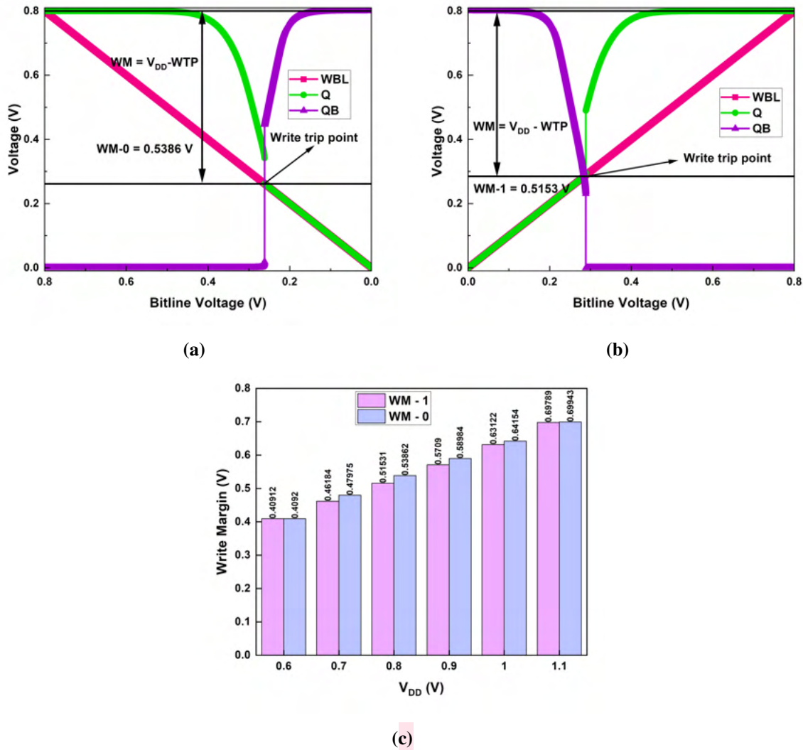
Figure 3.3: Write Margin's calculation for the proposed 8TS SRAM bit-cell (A) WM-0, (B) WM-1, and (C) the impact of supply voltage scaling.
