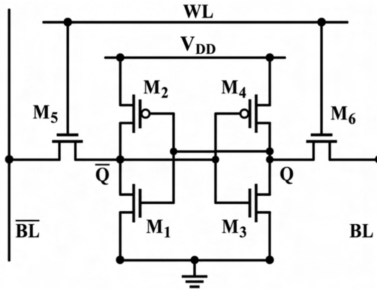
Figure 1.2: Conventional 6T SRAM bit-cell showing the storage nodes and differential bit-line access.
