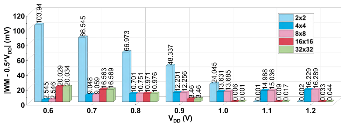
Figure 5.3: Array-size dependence of write-margin deviation, |WM - V_{DD}/2| , across the supply-voltage range.
