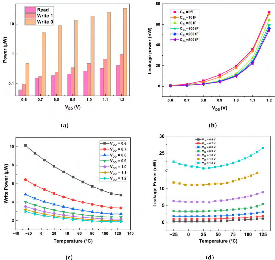
Figure 3.5: Power consumption of the 8TS SRAM cell as a function of supply voltage: (A) read and write power variation, (B) leakage power as a function of bitline capacitance, and (C) temperature dependence of write power and (D) leakage power at multiple V_{DD} .
