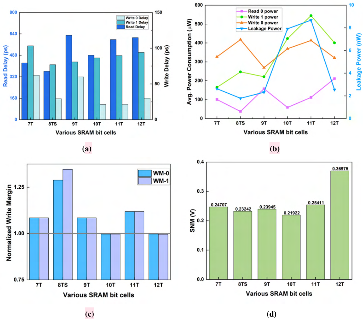
Figure 3.10: Comparative analysis of the proposed 8TS SRAM bit-cell compared to existing SRAM bit-cells with varying transistor counts: (A) Read/Write delay, (B) Power consumption, (C) Normalized Write Margin (WM) and (D) Static Noise Margin (SNM).
