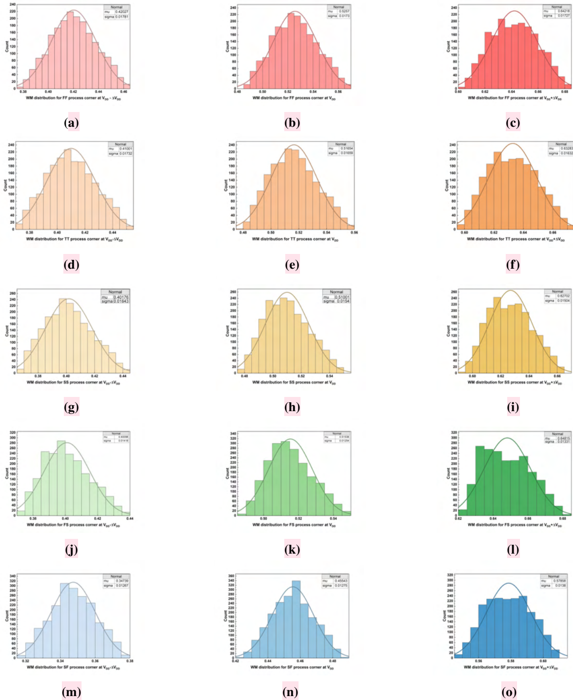
Figure 3.4: Monte Carlo simulations of the proposed 8TS cell across process corners, evaluating write margin (WM) under threshold voltage V_{TH} variations of \pm 30 mV and supply voltage fluctuations \Delta V_{DD} of 25% around the nominal 0.8 V.
