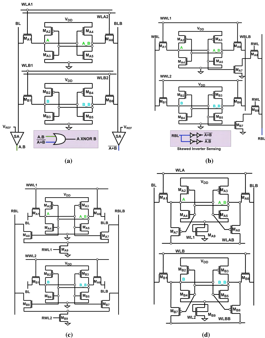
Figure 4.1: Circuit schematics for implementation of single bit boolean logic for two operands A,B along with the sensing strategy employed. (a) 6T SRAM-IMC (b) 8TC SRAM-IMC (c) 8TB SRAM-IMC and (d) 8TE SRAM-IMC
