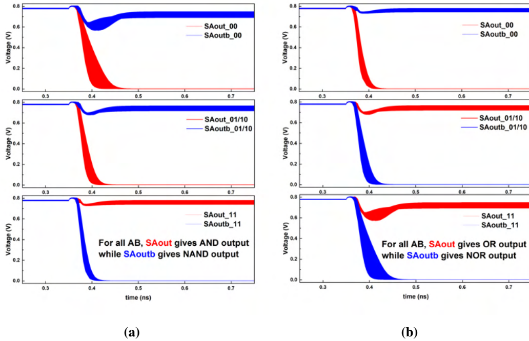
Figure 4.6: Transient response of the asymmetric sense amplifier for 6k Monte carlo simulations at TT corner for T = 300.15 K and V_{DD} = 0.8 V to implement (a) NAND and (b) NOR outputs for all possible input cases of input operands (AB), '00,01,10,11', at for \Delta V_{TH} = 50 mV.
