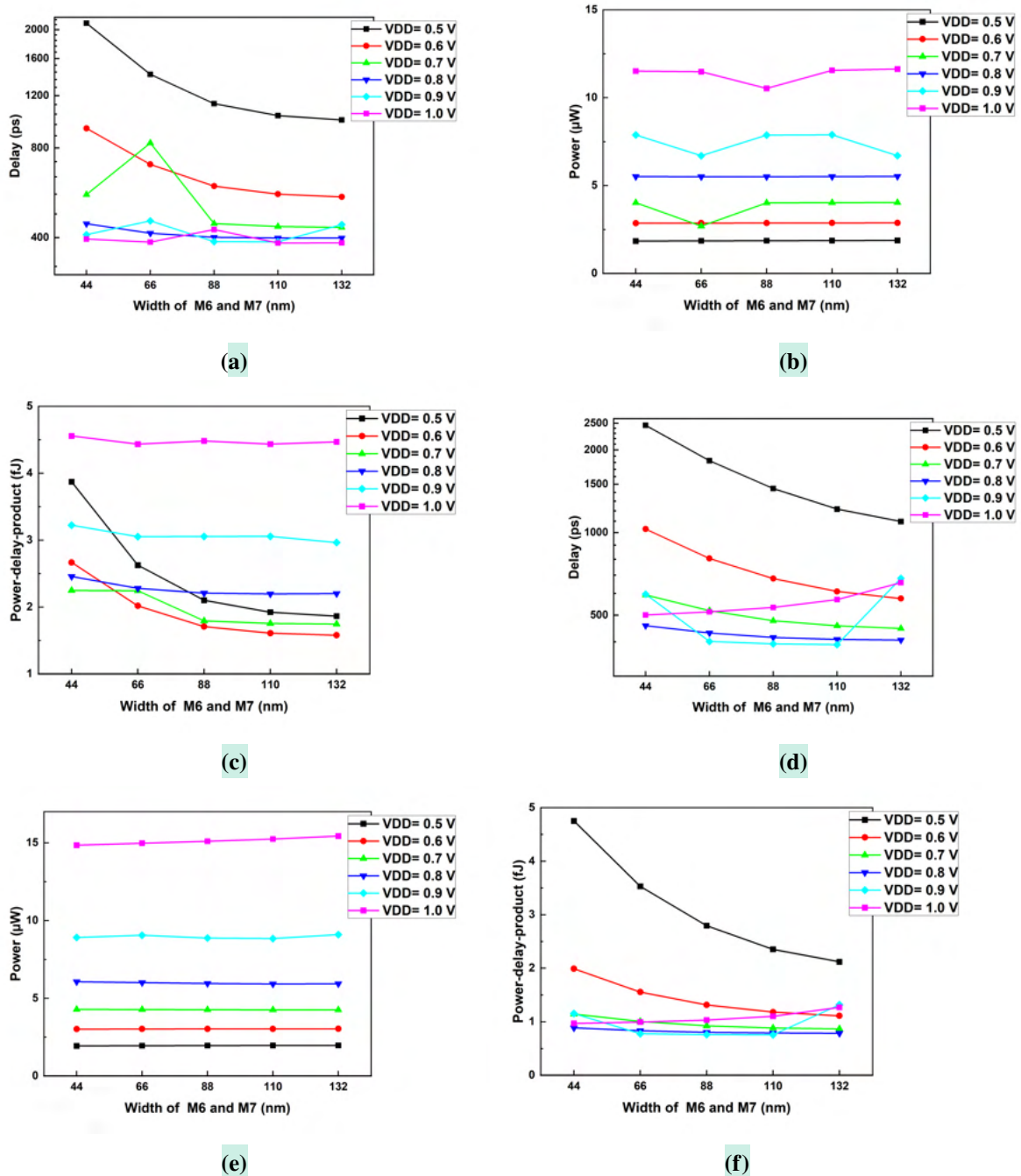
Figure 2.2: Investigating the impact of PMOS devices M6 and M7 width on MDSA and MDSANF performance: (a) Delay, (b) Power consumption, and (c) Power-delay-product for MDSA and (d) Delay, (e) Power consumption, and (f) Power-delay-product of MDSANF examined for different supply voltages
