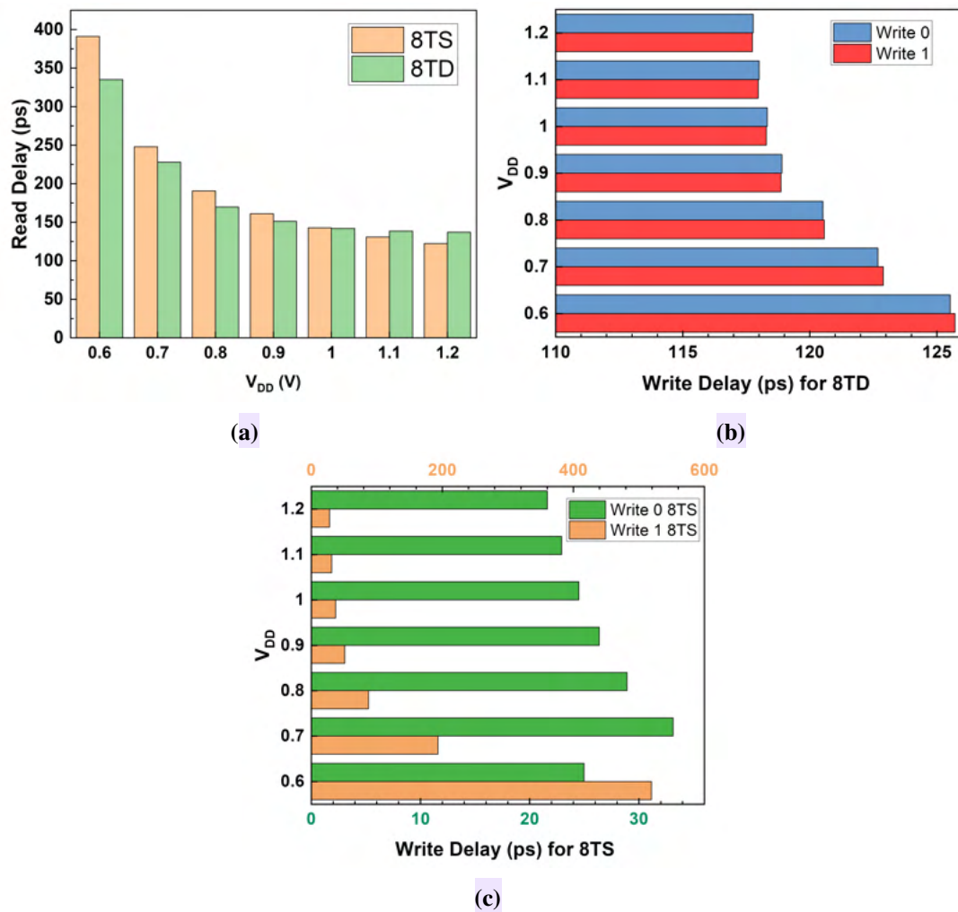
Figure 3.14: Timing analysis of the differential 8TD and single ended 8TS SRAM cells. (a) Read Delay comparison and Write Delay for (b) 8TD and (c) 8TS for V_{DD} = 0.6V to 1.2V
