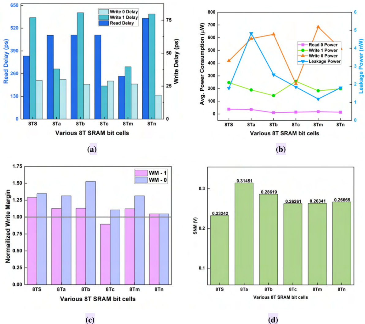
Figure 3.9: Performance comparison of the proposed 8TS SRAM bit-cell with existing 8T SRAM variants: (A) Read/Write delay, (B) Power consumption, (C) Normalized Write Margin (WM) and (D) Static Noise Margin (SNM).
