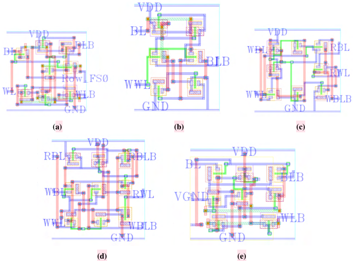
Figure 4.13: Layout views of the SRAM cells considered for IMC implementation: (a) 8TE, (b) 6T, (c) 8TC, (d) 8TB and (e) 8TD. The layouts are used to support the normalized area comparison reported in Table 4.2.
