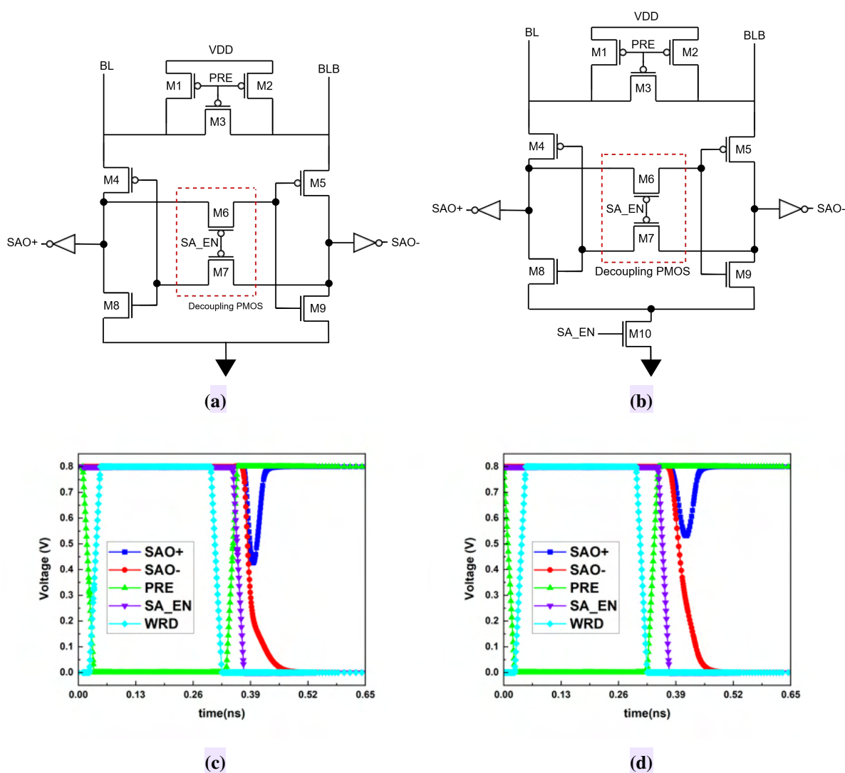
Figure 2.1: Circuit schematics for (a) MDSA and (b) MDSANF, along with the transient response showing timing control signals at V_{DD} = 0.8 V and C_{BL} = 50 fF for (c) MDSA and (d) MDSANF
