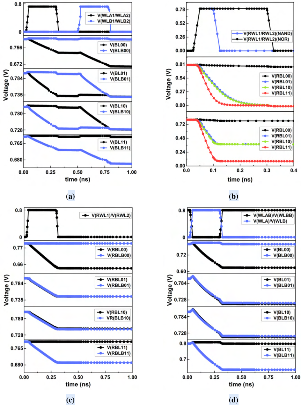
Figure 4.3: Transient response of SRAM bitcells in compute-mode for all possible bit combinations of two single bit operands (A,B) '00', '01', '10' and '11' at V_{DD} = 0.8 V for (a) 6T SRAM cell (b) 8TC SRAM cell (c) 8TB SRAM cell (d) 8TE SRAM cell
