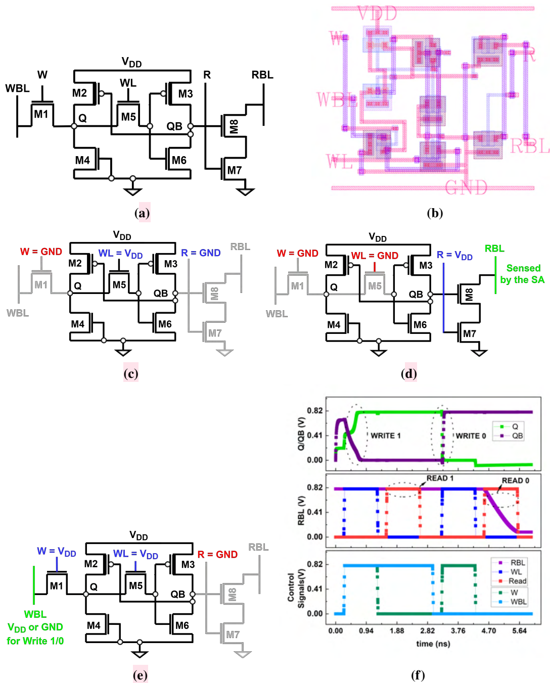
Figure 3.1: Proposed single-ended, single port 8T SRAM bitcell (A) 8TS circuit schematic, (B) layout of the 8TS bit-cell; Equivalent circuit for (C) hold mode, (D) read mode, and (E) write mode; (F) transient simulation with control signals for all the operations of 8TS Cell.
