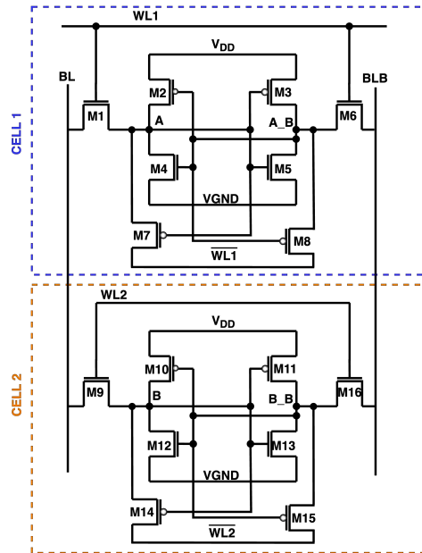
Figure 4.4: Circuit schematic for implementation of single bit boolean logic (NAND/NOR and XOR/XNOR) for two operands A,B using proposed 8TD SRAM cell
