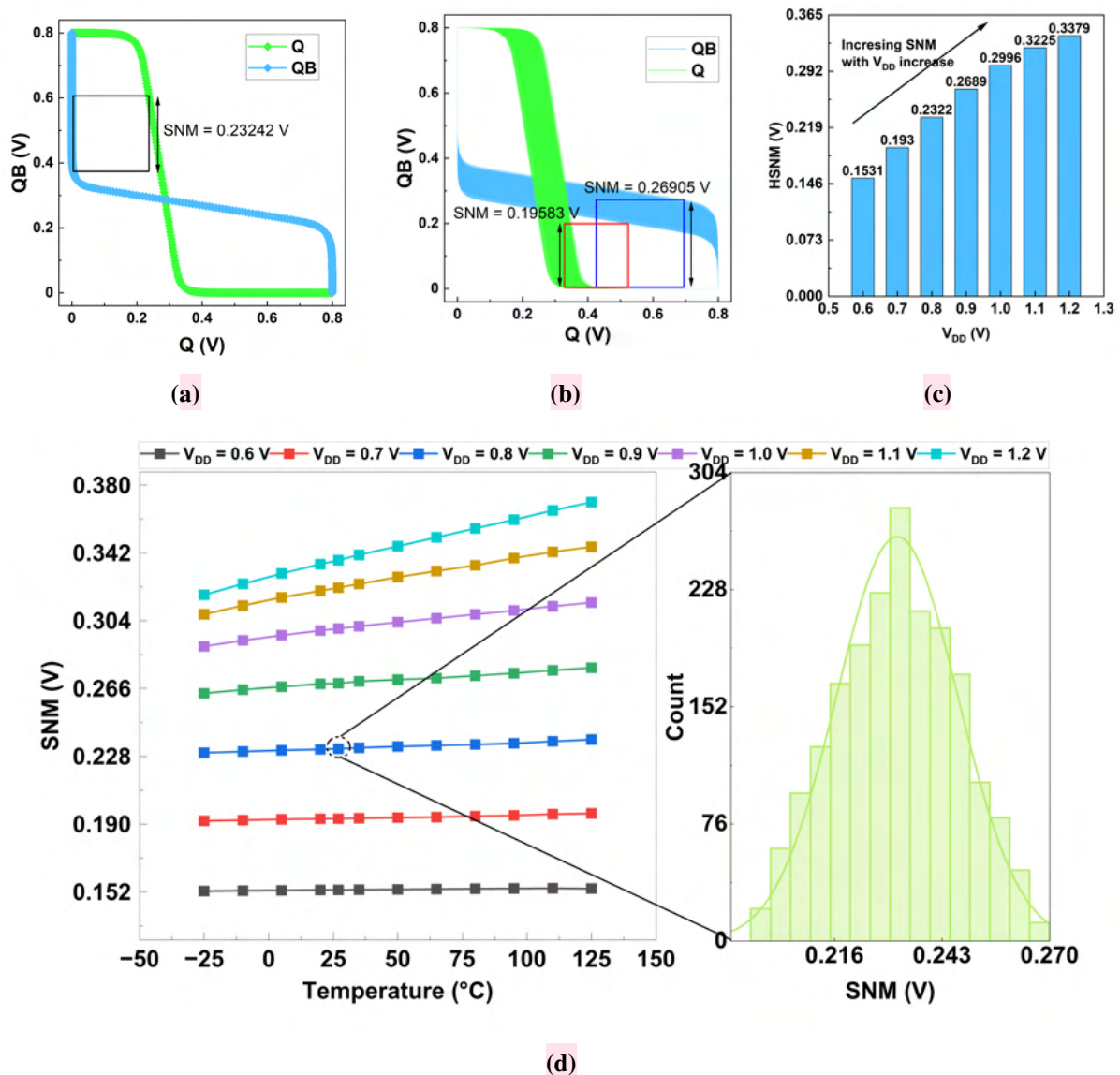
Figure 3.2: Static noise margin butterfly curve of the 8TS SRAM cell for (A) SNM calculation, (B) butterfly curve for Monte Carlo (2000-point) analysis at V_{DD} = 0.8 V, (C) SNM as a function of supply voltage, and (D) SNM as a function of temperature (Inset: distribution of SNM at T = 27^{\circ}\text{C} for V_{DD} = 0.8 V)
