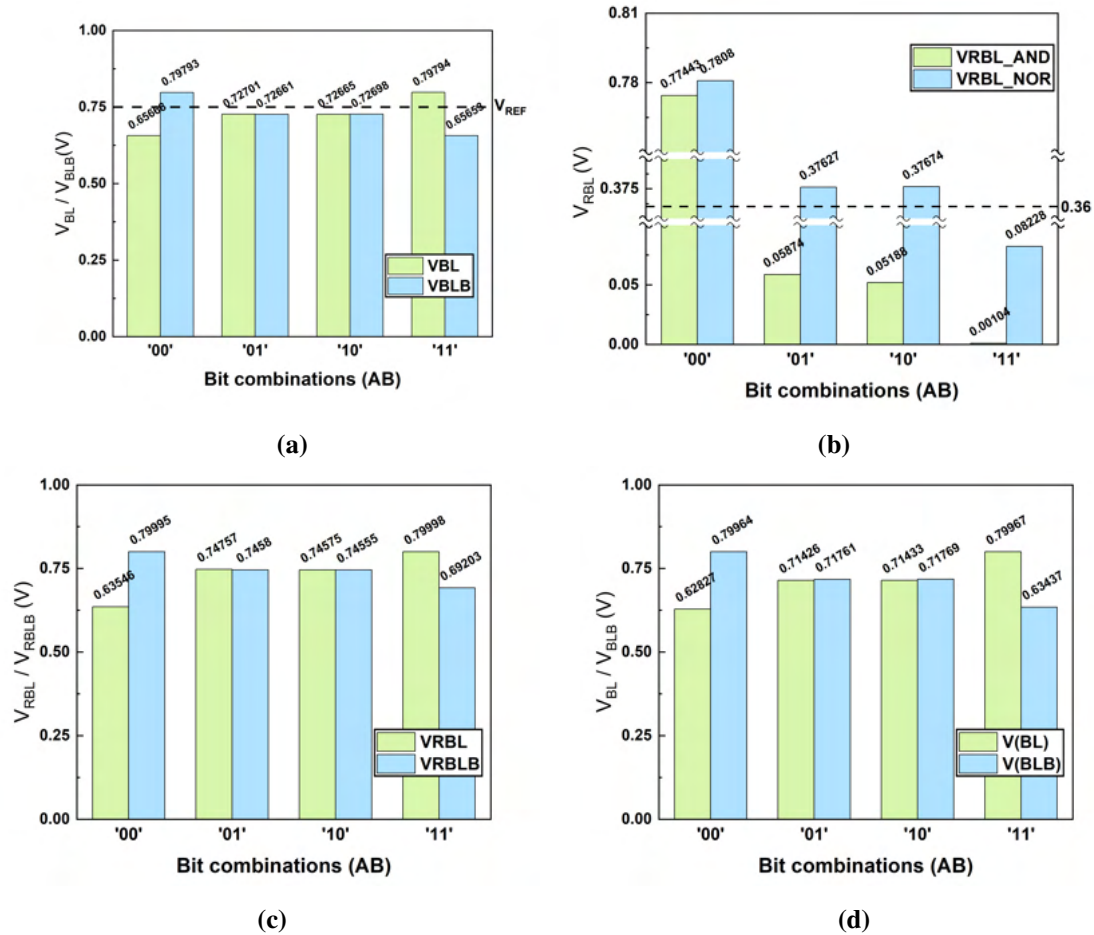
Figure 4.2: SRAM bit lines (BL/BLB) voltage levels to be sensed by SAs for IMC bitwise logical operations for (a) 6T SRAM cell (b) 8TC SRAM cell (c) 8TB SRAM cell and (d) 8TE SRAM cell
