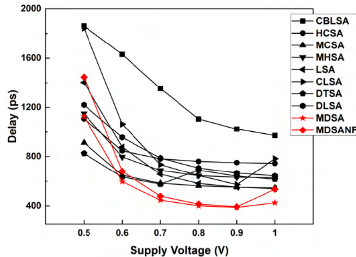
Figure 2.9: Delay comparison of all sense amplifiers as a function of the supply voltage at C_{BL} = 50 fF.
