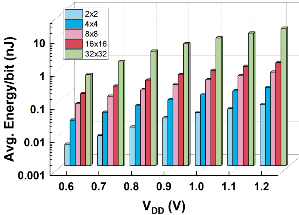
Figure 5.7: Average compute energy per bit of the proposed SRAM-IMC array for 2 \times 2 to 32 \times 32 organizations across V_{DD} = 0.6 – 1.2 V.
