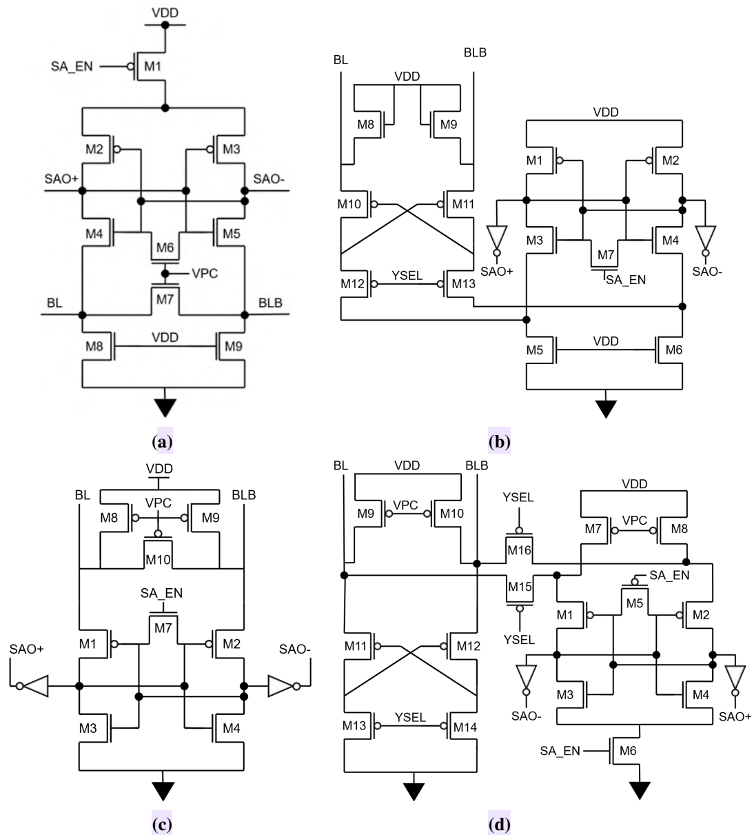
Figure 2.7: Representative current-mode and hybrid SRAM sense amplifier architectures: (a) clamped bit-line sense amplifier, (b) hybrid current sense amplifier, (c) modified clamped sense amplifier, and (d) modified hybrid sense amplifier.
