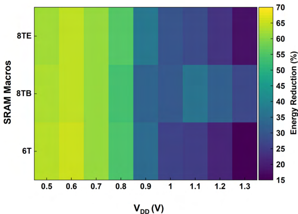
Figure 4.12: Energy reduction of the proposed 8TD SRAM-IMC cell with respect to 6T, 8TB, and 8TE SRAM-IMC macros across V_{DD} .
