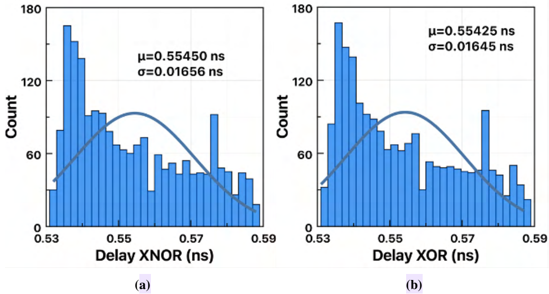
Figure 4.9: Latency distributions for (a) XNOR and (b) XOR logic operations for all possible input operand combinations, AB = 00, 01, 10, \text{ and } 11 . The results are obtained from 2000 Monte Carlo simulation runs at T = 300.15 \text{ K} , V_{DD} = 0.8 \text{ V} , and \Delta V_{TH} = 50 \text{ mV} .
