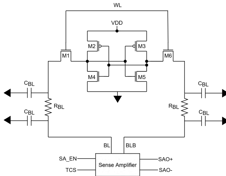
Figure 2.8: Simulation test-bench used for comparison of sense amplifiers.
