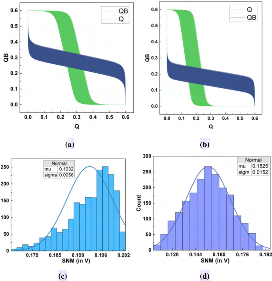
Figure 3.16: Monte Carlo (2000 point) analysis of differential 8TD and single-ended 8TS SRAM cells at V_{DD} = 0.6V . Butterfly curves for (a) 8TD (b) 8TS. The histograms for the SNM extracted from the butterfly curves for (c) 8TD and (d) 8TS.
