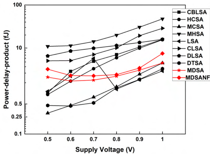
Figure 2.11: Power-delay-product comparison of all SAs as a function of the supply voltage ( C_{BL} = 50 fF)
