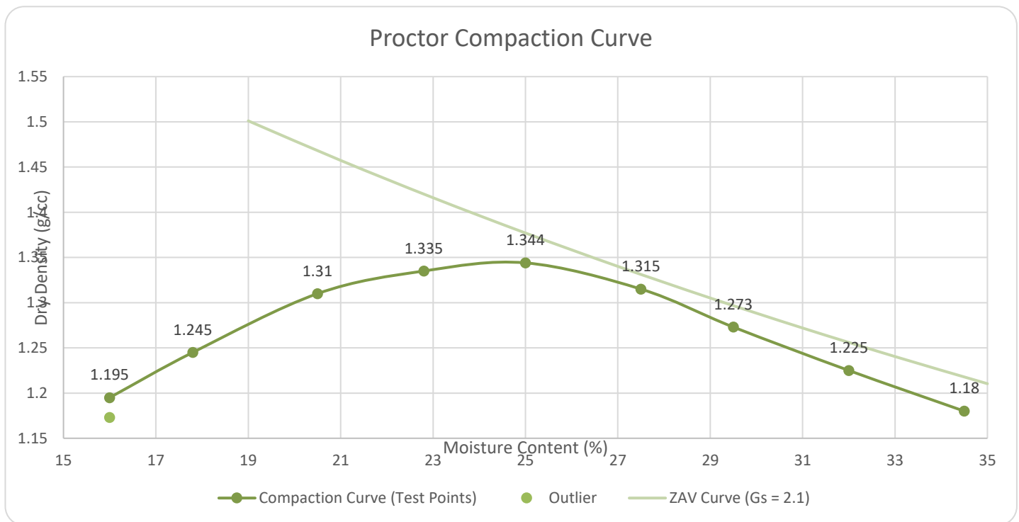
Figure 5.3: Proctor Compaction Curve Graph
