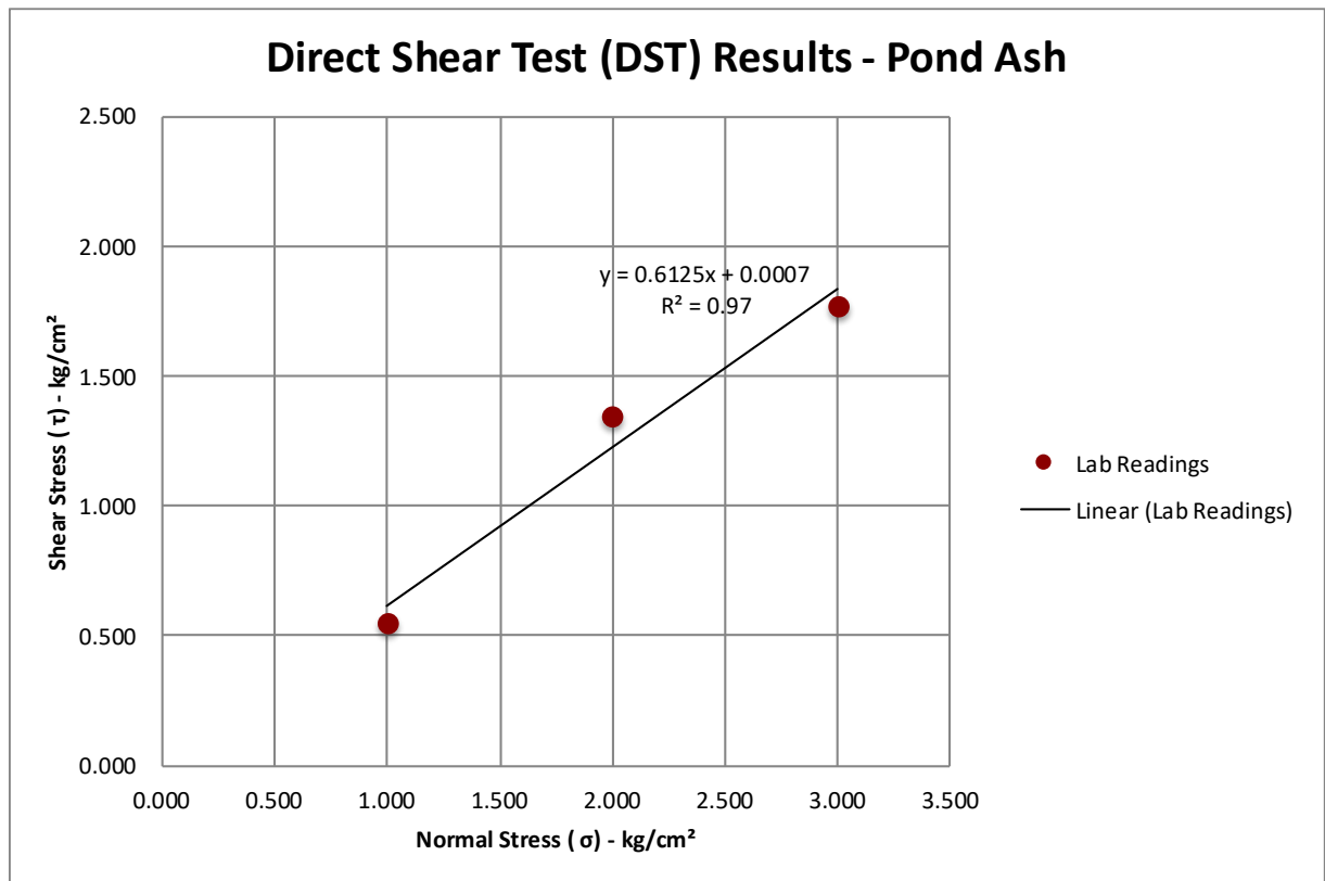
Figure 5.4: Direct shear failure envelope for pond ash
