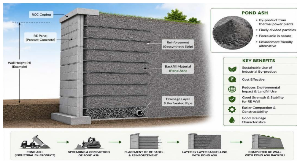
Figure 1.1: Conceptual representation of pond ash as sustainable backfill for a Reinforced Earth wall (Source: https://share.google/yQBs9btHaseUJhM75 )
