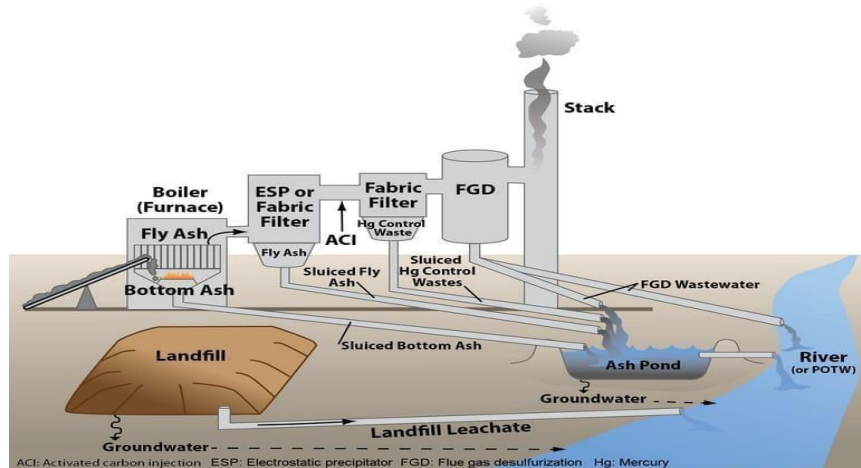
Figure 3.2: Schematic representation of ash generation and disposal in a thermal power plant (Source : https://share.google/dDgs2Ng07vYLTg4uu )
