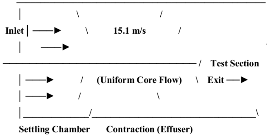
Figure 1. Diagram of acceleration across the contraction section.
