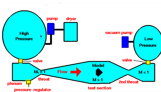
Figure 2: A pressure vacuum wind tunnel
