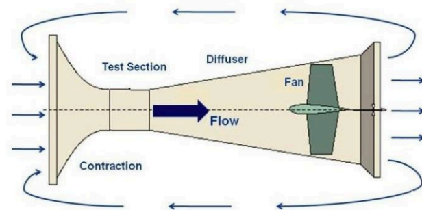
Figure 3: Open loop wind tunnel
