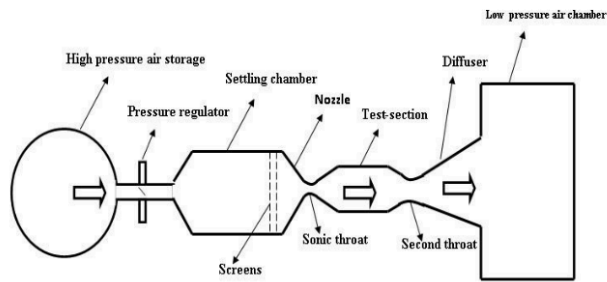
Figure 1: Type of Pressure Storage wind tunnel.
