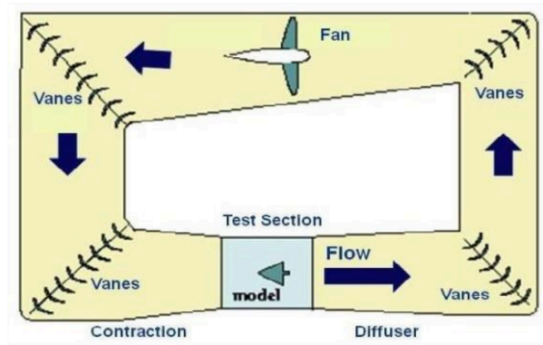
Figure 4: Closed loop wind tunnel
