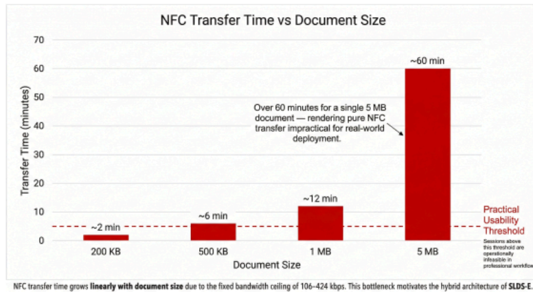
Figure 1.3: NFC transfer time vs. document size
