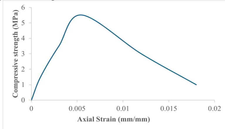
Figure 3.10 Compressive Strain-Strain Curve of Lime mortar
