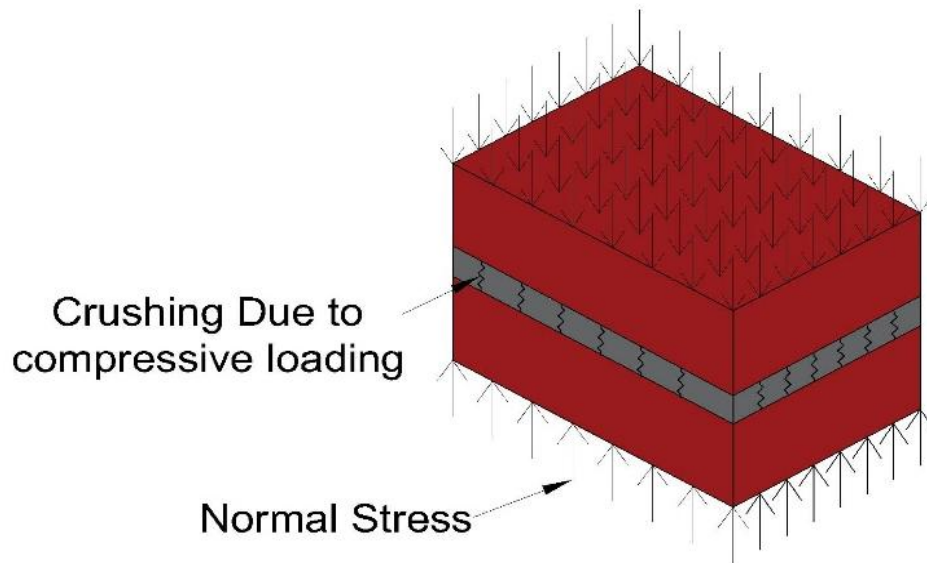
Figure 3.5 crack in masonry due to compressive loading.
