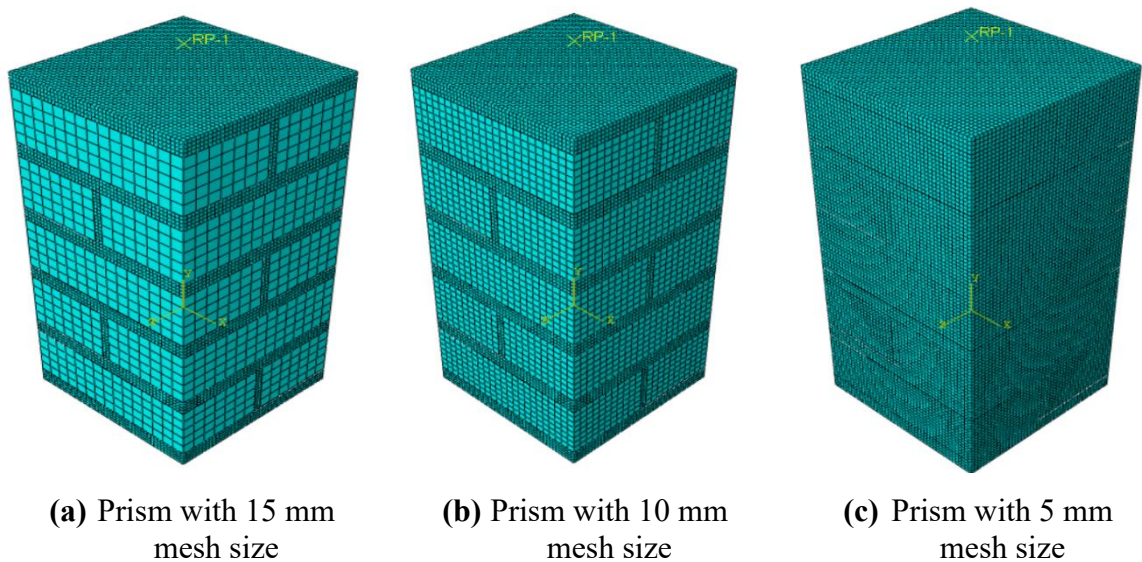
Figure 3.12 Prism with different mesh size
