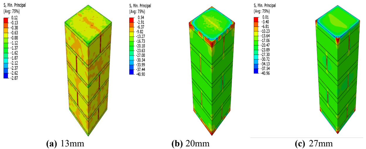
Figure 4.11 Compressive Stress distribution in Prisms
