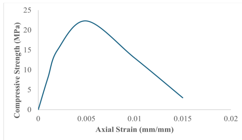
Figure 3.8 Compressive Strain-Strain Curve of Brick
