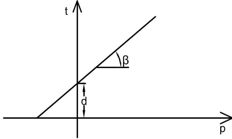
Figure 3.6 Linear yield surface of Drucker-Prager Model[19]
