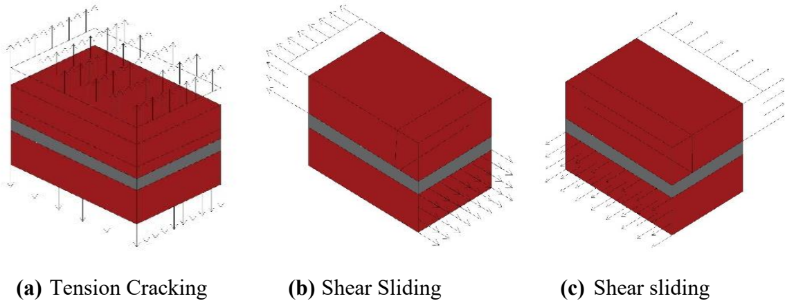
Figure 3.4 Failure Modes of Joints
