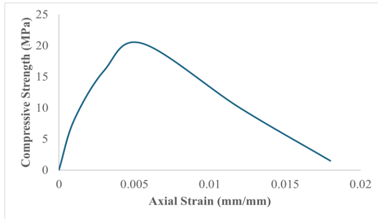
Figure 3.9 Compressive Strain-Strain Curve of Cement mortar
