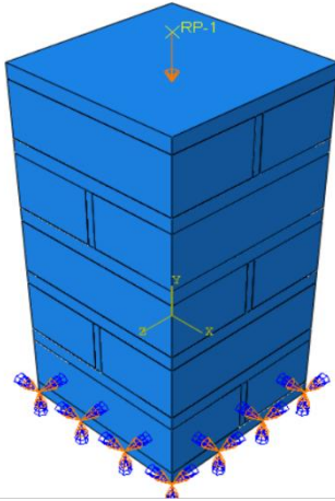
Figure 3.11 Boundary condition and loading condition
