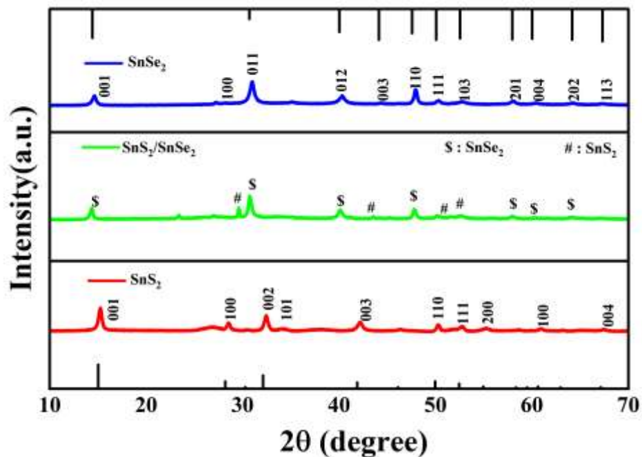
Fig. 4: XRD results of synthesised powders.
