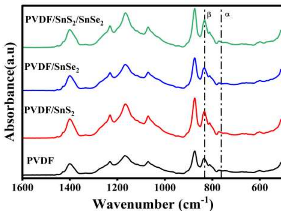
Fig. 9: FTIR spectra of synthesized thin films.
