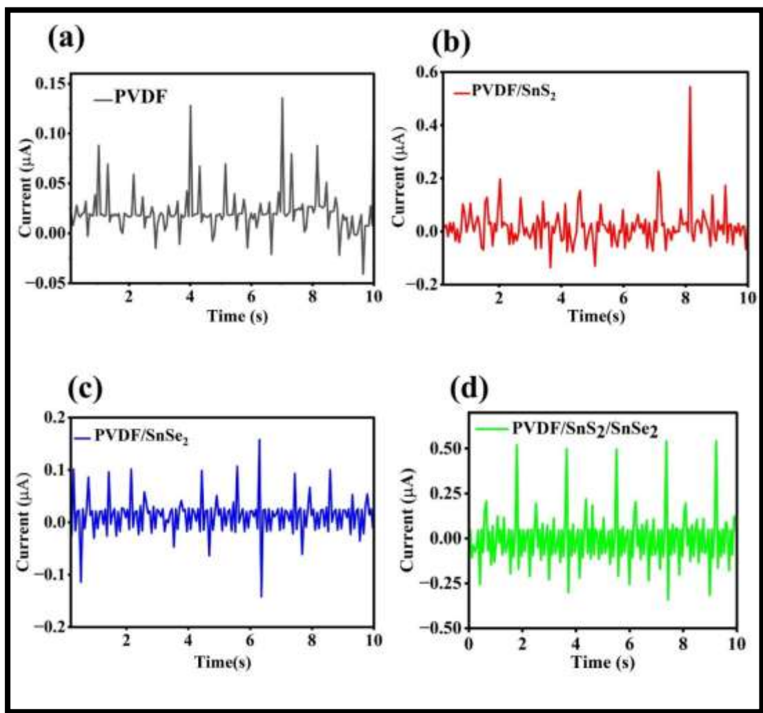
Fig. 12: Short circuit current for (a) PVDF, (b) PVDF/SnS 2 , (c) PVDF/SnSe 2 and (d) PVDF/SnS 2 /SnSe 2 thin film nanogenerators by continuous tapping at 7 Hz frequency.
