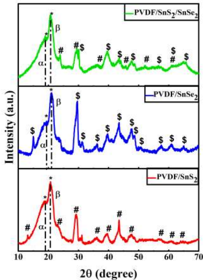
Fig. 5: XRD results of synthesized films.
