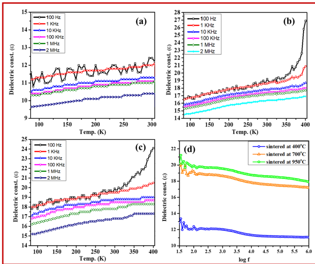
Figure 3.6: Dielectric constant ( \epsilon ) curves of \text{Ta}_2\text{O}_5 as a function of operating temperatures at different frequencies for sample sintered at (a) 400 °C, (b) 700 °C, (c) 950 °C and (d) comparative graph of dielectric constant at 300 K
