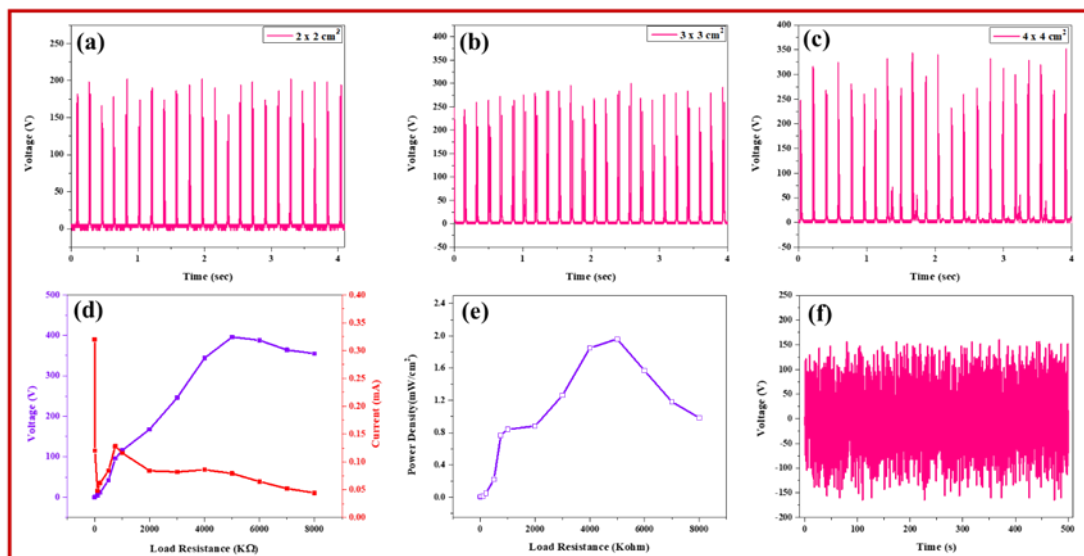
Figure 6.10 (a) Voltage generated by fabricated PTM1.2 based TENG with dimensions (a) 2 \times 2 \text{ cm}^2 , (b) 3 \times 3 \text{ cm}^2 , (c) 4 \times 4 \text{ cm}^2 , (d) voltage output and (e) power density across different load resistance and (f) stability curve for 4 \times 4 \text{ cm}^2 PTM1.2 based TENG
