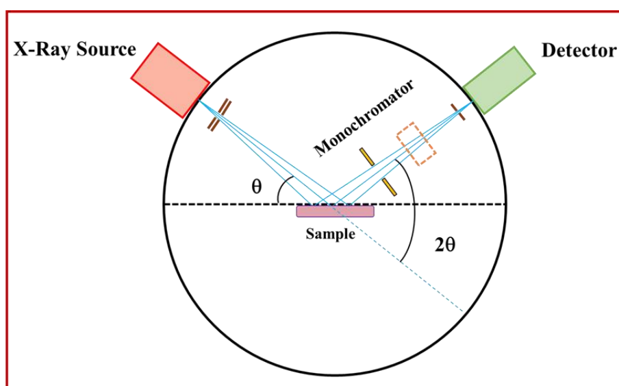
Figure 2.3 A schematic diagram representing components of XRD instrument
