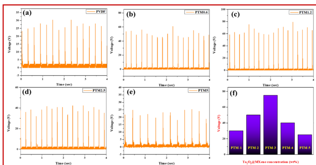
Figure 6.5 Generated voltage output vs time waveforms for (a) PVDF, (b) PTM0.6, (c) PTM1.2, (d) PTM2.5, (e) PTM5 and (f) comparative voltage for different films
