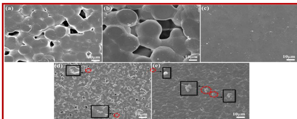
Figure 4.6: FESEM images of the PVDF films with wt% (a) 0%, (b) 0.625%, (c) 1.25%, (d) 2.5% and (e) 5% of Ta 2 O 5 NPs
