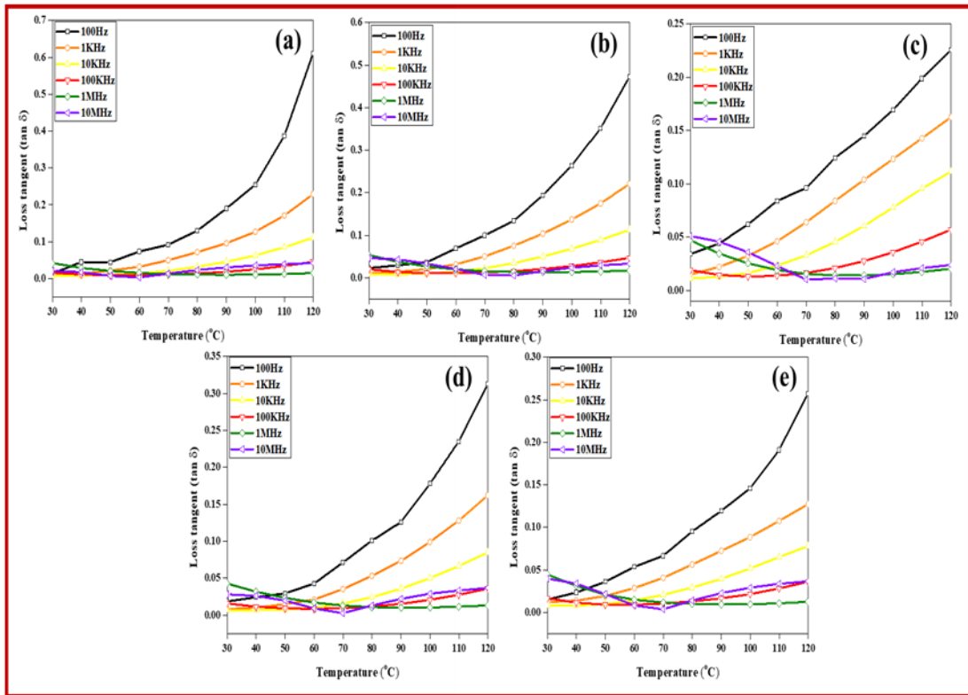
Figure 5.9 Loss tangent curves w.r.t. temp. at different applied freq. for the films (a) PVDF, (b) PTM0.6, (c) PTM1.2, (d) PTM2.5, and (e) PTM5
