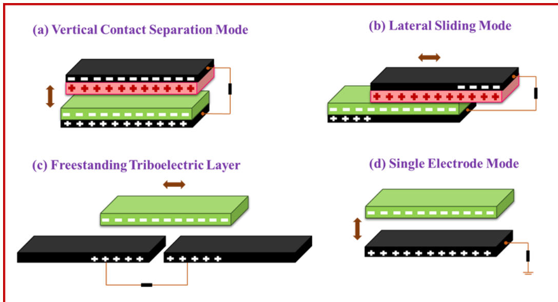
Figure 1.4: The fundamental operational modes of TENG includes: (a) vertical contact separation mode, (b) lateral sliding mode, (c) freestanding triboelectric layer and (D) single electrode mode
