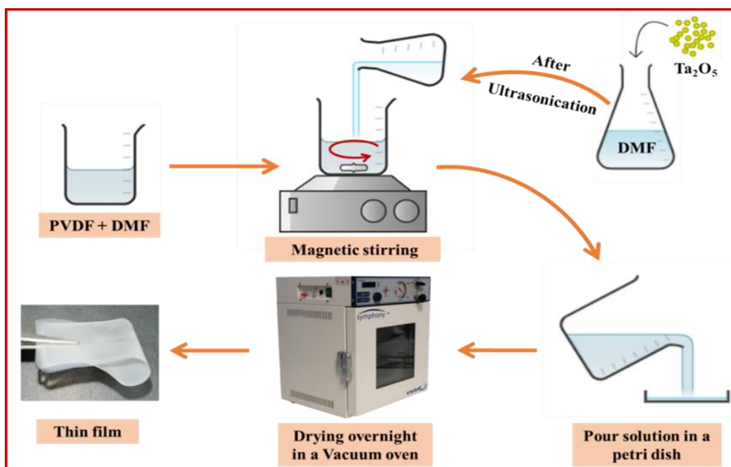
Figure 4.2: Schematic representation for the preparation of the PVDF based nanocomposite thin films
