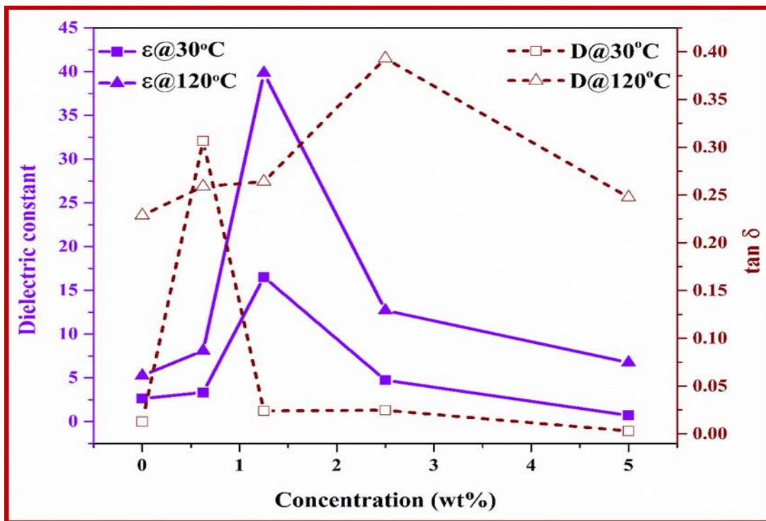
Figure 4.11: Comparative graph of dielectric constant and loss tangent for different filler concentrations at operating temperature 30 & 120°C and 1 KHz frequency of applied electric field
