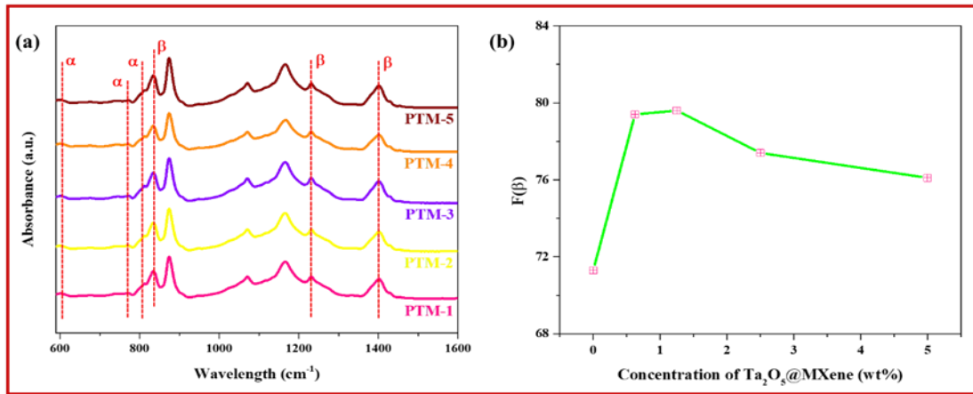
Figure 5.7 (a) FTIR spectra of pristine PVDF and MXene@Ta 2 O 5 /PVDF nanocomposite films and (b) graph of \beta -phase content w.r.t. nanofiller concentration in the nanocomposite films
