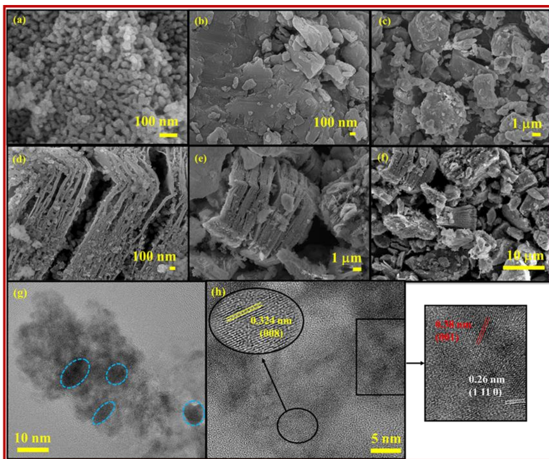
Figure 5.3 FESEM images of (a) \text{Ta}_2\text{O}_5 nanoparticles, (b & c) Max phase ( \text{Ti}_3\text{AlC}_2 ), (d-f) MXene ( \text{Ti}_3\text{C}_2\text{T}_x ) nanosheets and (g) HRTEM image and (h) fringe pattern of MXene@ \text{Ta}_2\text{O}_5 heterostructure
