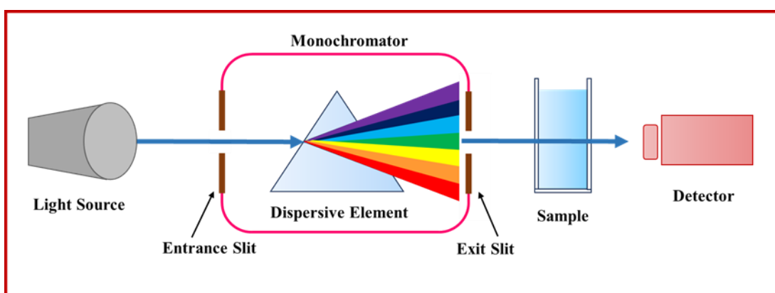
Figure 2.8 Schematic diagram illustrating UV-visible spectrometer
