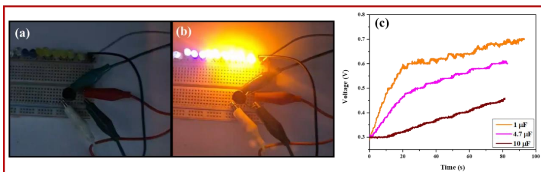
Figure 6.8 (a) Digital image of breadboard circuit for LEDs without mechanical force, (b) LEDs glowing on applying mechanical force, (c) Voltage output curve across capacitor 1 , 4.7 and 10\ \mu\text{F}
