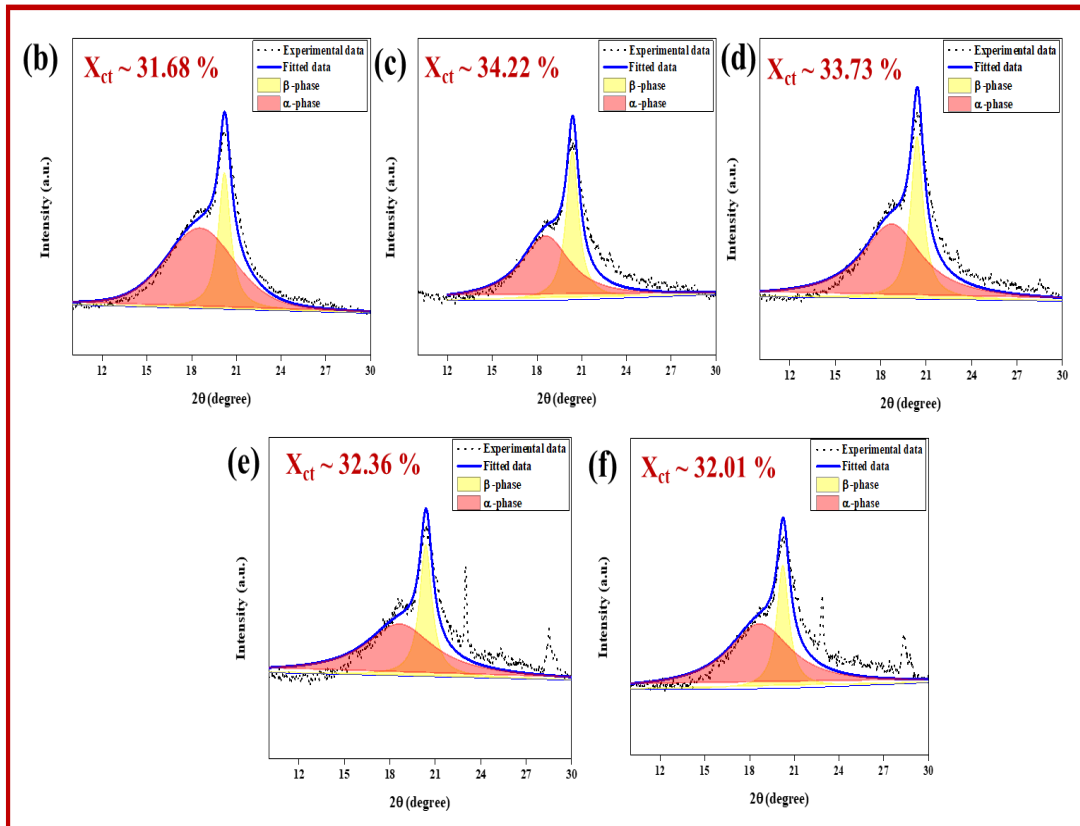
Figure 5.5 (b) deconvoluted curves of XRD pattern for (b) pure PVDF, (c) PTM0.6, (d) PTM1.2, (e) PTM2.5, (f) PTM5 films
