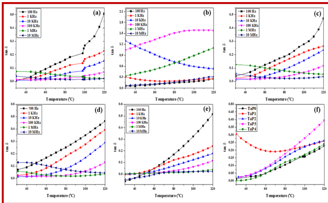
Figure 4.10: Loss tangent ( \tan \delta ) as a function of temperature at different applied frequencies for the films with wt% (a) 0%, (b) 0.625%, (c) 1.25%, (d) 2.5%, (e) 5% of \text{Ta}_2\text{O}_5 and (f) comparative graph of \tan \delta vs temperature at 1 KHz for different concentration of thin films
