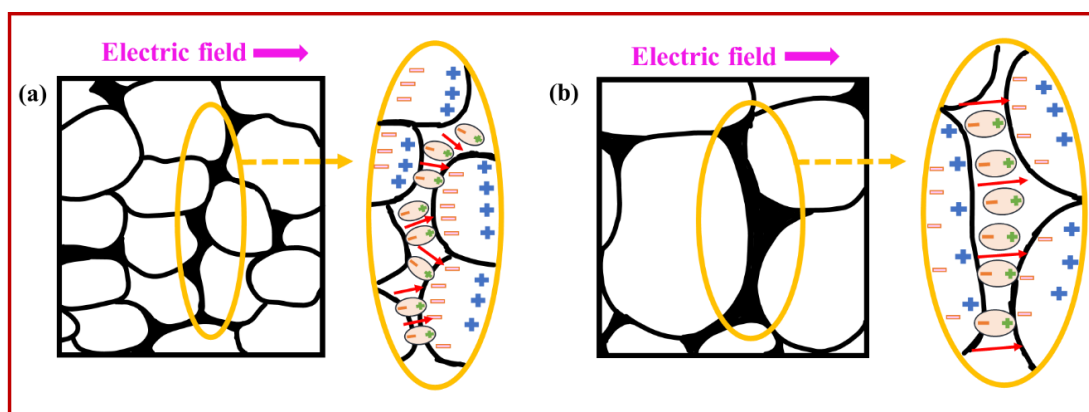
Figure 3.7: Schematic diagram representing the orientation of charge carriers along with the applied field for (a) smaller (sample sintered at 400 °C) and (b) larger (sample sintered at 950 °C) grains
