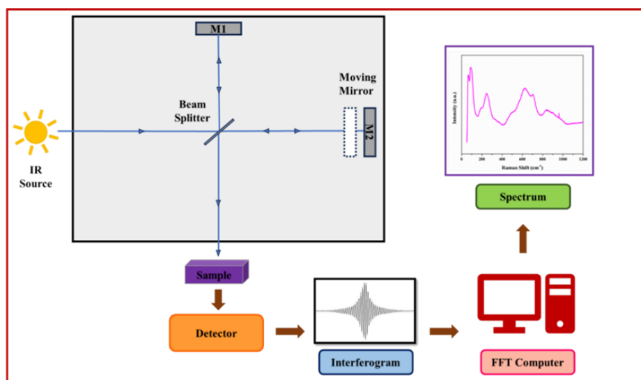
Figure 2.6: Schematic diagram representing FTIR spectroscopy
