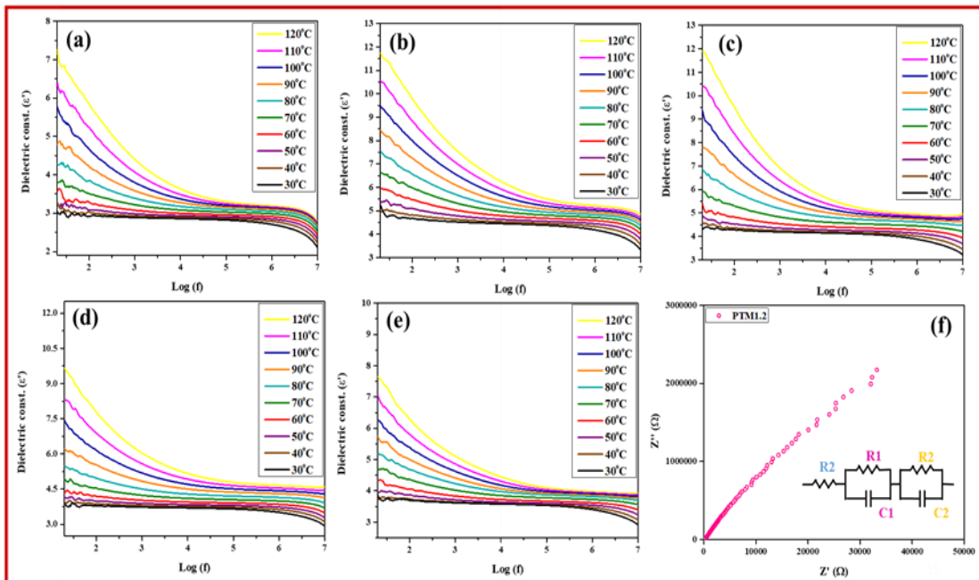
Figure 5.10 Dielectric constant vs. applied frequency at different operating temp. for the films (a) PVDF, (b) PTM0.6, (c) PTM1.2, (d) PTM2.5, (e) PTM5 and (f) Nyquist plot for PTM1.2 film at RT
