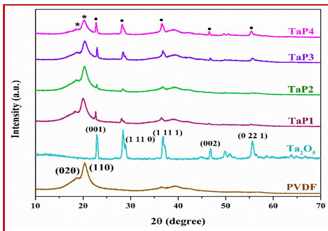
Figure 4.3: X-Ray Diffraction pattern for pristine PVDF, Ta 2 O 5 NPs and nanocomposite thin films with different wt% of Ta 2 O 5 NPs where * and • represent peaks for PVDF and Ta 2 O 5 , respectively
