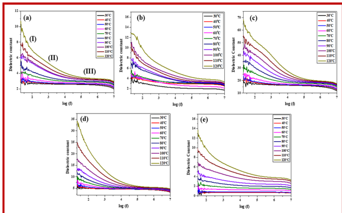
Figure 4.12: Dielectric constant as a function of log of applied frequency at different temperatures for the films with wt% (a) 0%, (b) 0.625%, (c) 1.25%, (d) 2.5% and (e) 5% of \text{Ta}_2\text{O}_5 NPs
