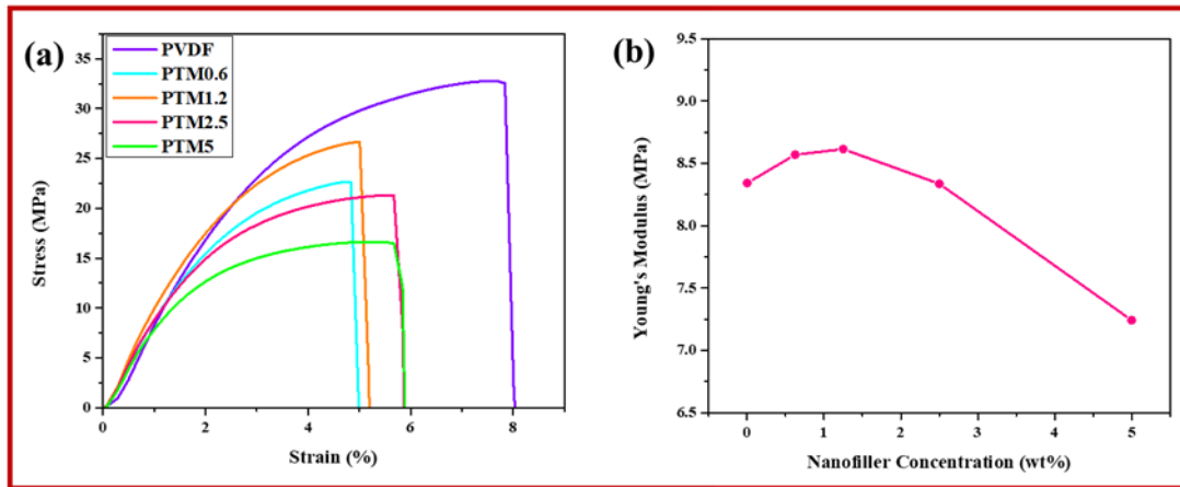
Figure 5.11 (a) Stress-Strain curves and (b) variation in Young's Modulus with MXene@Ta 2 O 5 concentration for pure PVDF and nanocomposite films
