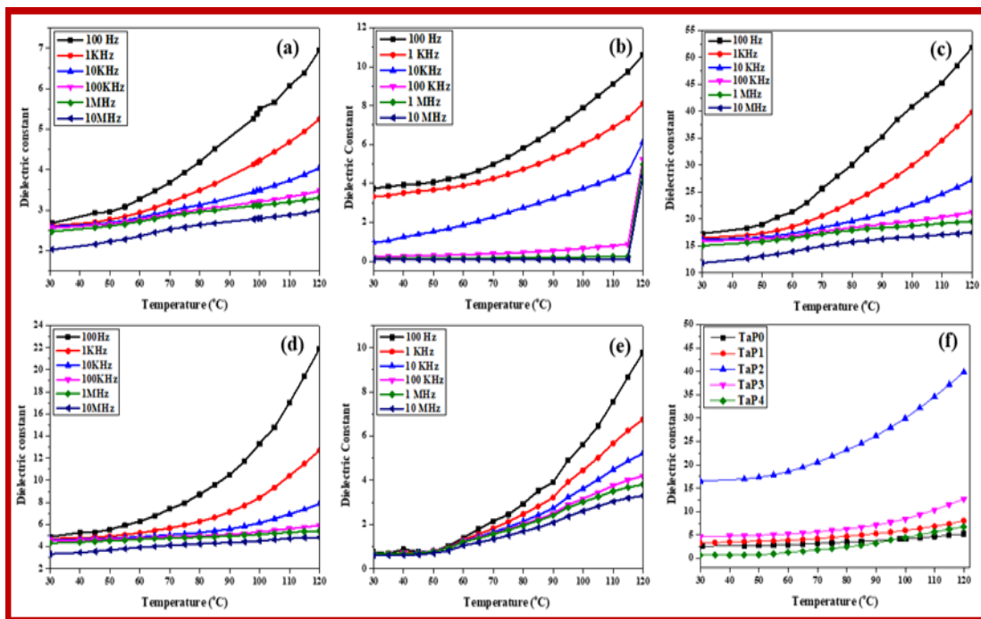
Figure 4.9 Dielectric constant curves w.r.t. temperature at different applied frequencies for the films with wt% (a) 0%, (b) 0.625%, (c) 1.25%, (d) 2.5%, (e) 5% of Ta 2 O 5 NPs and (f) comparative graph of dielectric const. vs temperature at 1 KHz for different concentration of thin films
