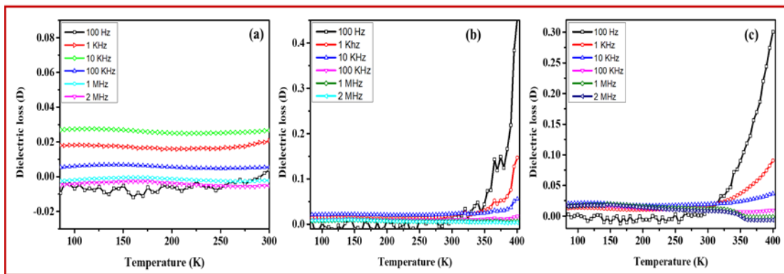
Figure 3.8: Dielectric loss curves of \text{Ta}_2\text{O}_5 as a function of the operating temperature at several frequencies for sample sintered at (a) 400 °C, (b) 700 °C, and (c) 950 °C
