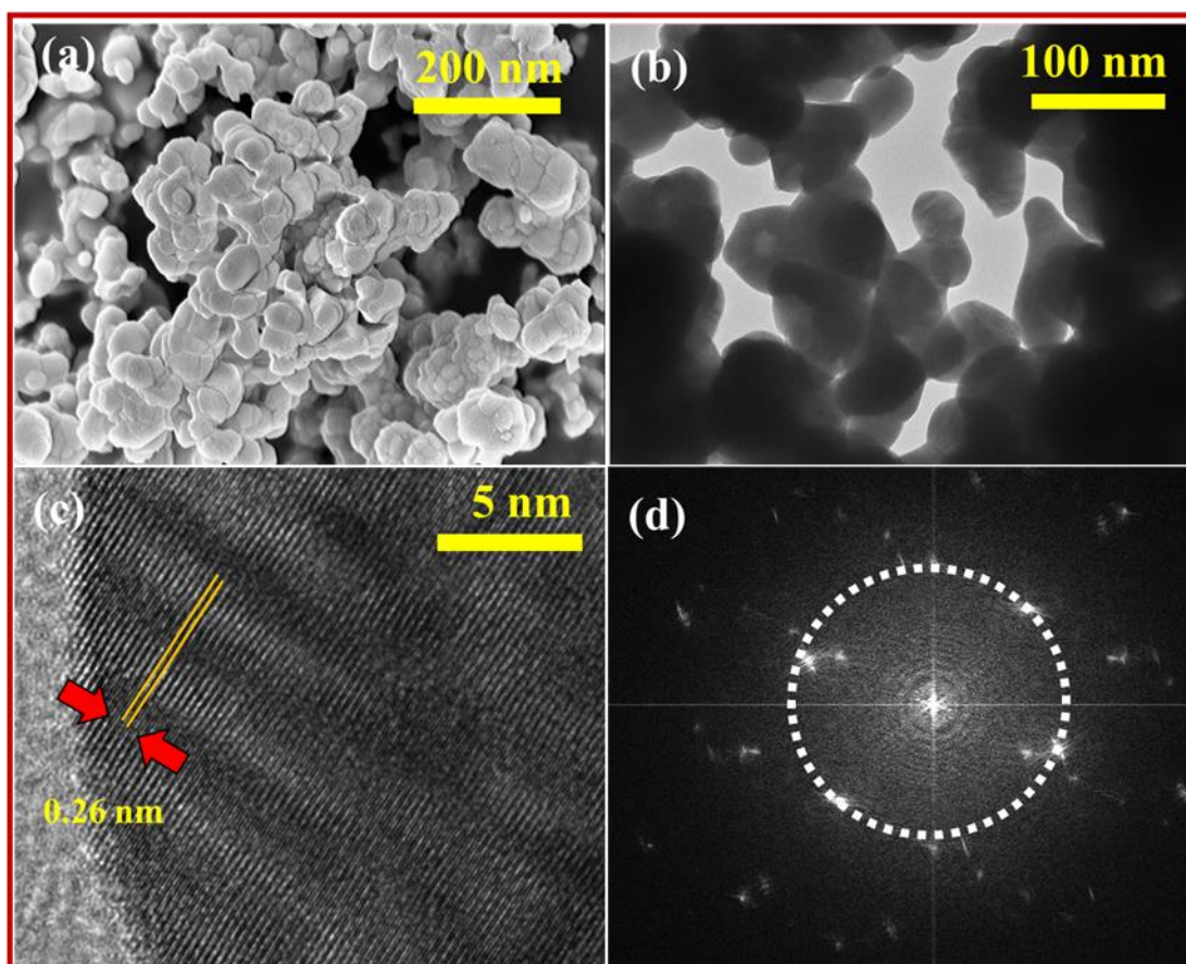
Figure 3.3 (a): FE-SEM image, (b & c) TEM images and (d) SAED pattern of synthesized \text{Ta}_2\text{O}_5 nanostructures calcinated at 800 °C
