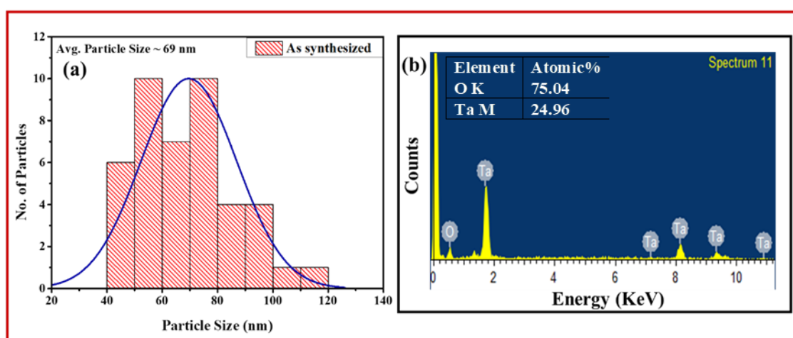
Figure 3.4 (a): Particle distribution histogram calculated from SEM micrograph and (b) EDS pattern of the synthesized \text{Ta}_2\text{O}_5
