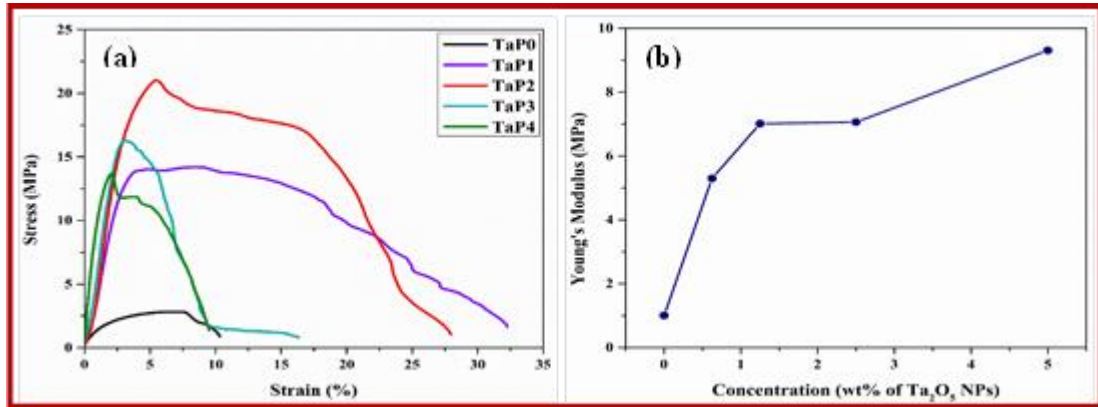
Figure 4.8 (a): Stress-Strain curves and (b) variation in Young's Modulus with Ta 2 O 5 NPs concentration for pure PVDF and Ta 2 O 5 @PVDF nanocomposite thin films
