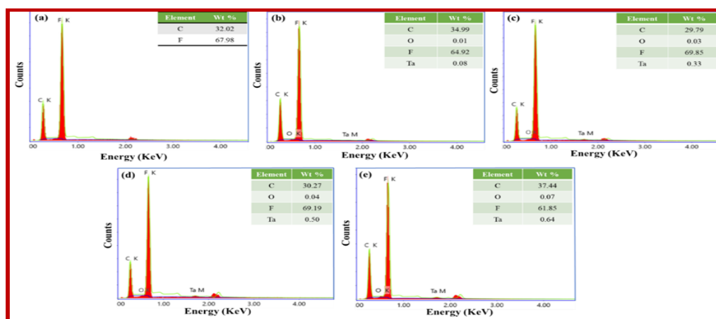
Figure 4.7: EDS graph of the PVDF films with wt% (a) 0%, (b) 0.625%, (c) 1.25%, (d) 2.5% and (e) 5% of Ta 2 O 5 NPs
