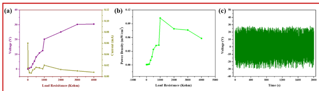
Figure 6.3 (a) Voltage output across different load resistance, (b) power density w.r.t. different load resistance and (c) stability curve of TaP2 based PENG
