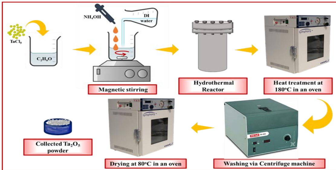
Figure 5.1 (a): The schematic diagram to synthesize Ta 2 O 5 nanoparticles via hydrothermal method
