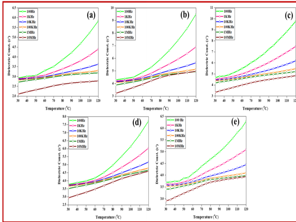
Figure 5.8 Dielectric constant curves w.r.t. temp. at different applied freq. for the films (a) PVDF, (b) PTM0.6, (c) PTM1.2, (d) PTM2.5, and (e) PTM5
