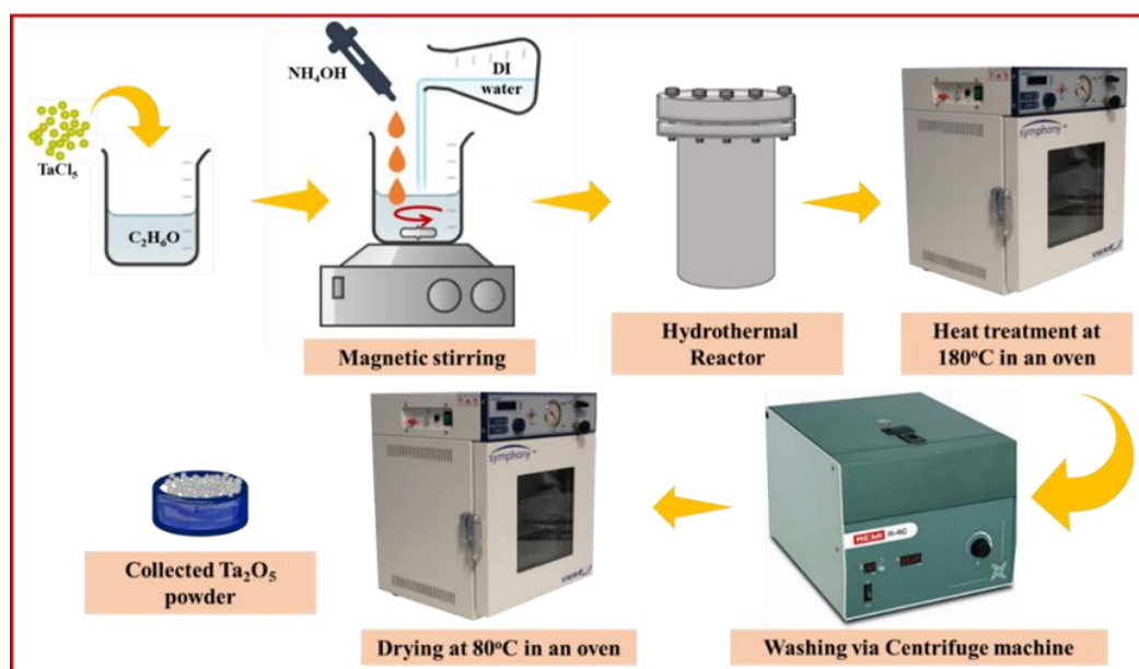
Figure 4.1: The schematic diagram to synthesize \text{Ta}_2\text{O}_5 nanoparticles via hydrothermal method
