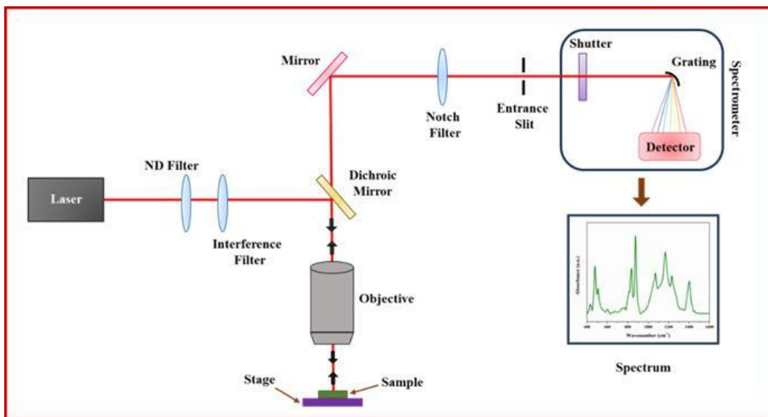
Figure 2.7 Schematic representation of Raman spectrometer
