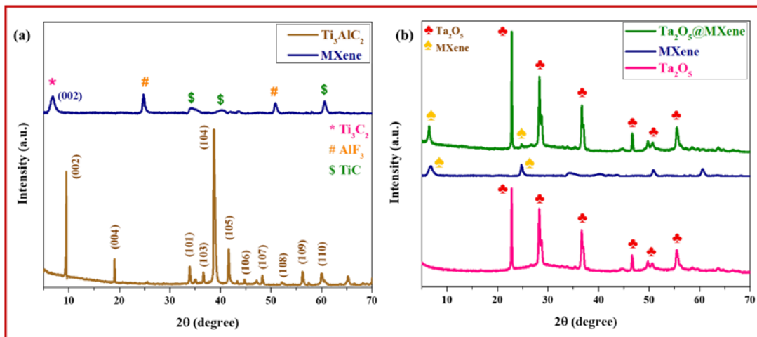
Figure 5.2: XRD pattern of (a) MAX phase and synthesized MXene, (b) \text{Ta}_2\text{O}_5 NPs, MXene nanosheets and \text{MXene@Ta}_2\text{O}_5 heterostructure
