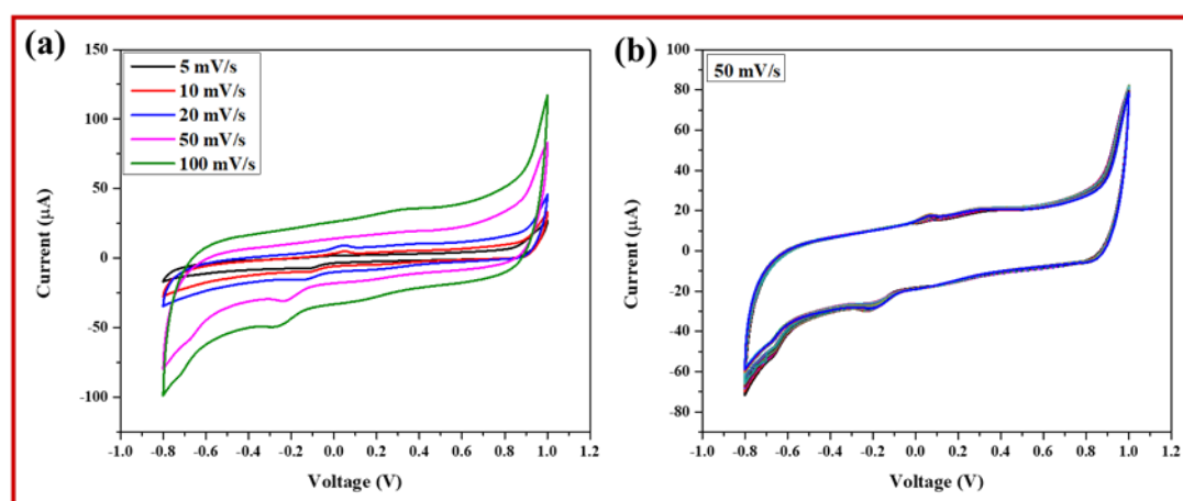
Figure 6.11 (a) CV curves at different scan rates and (b) CV cycle stability test for SCPC electrode
