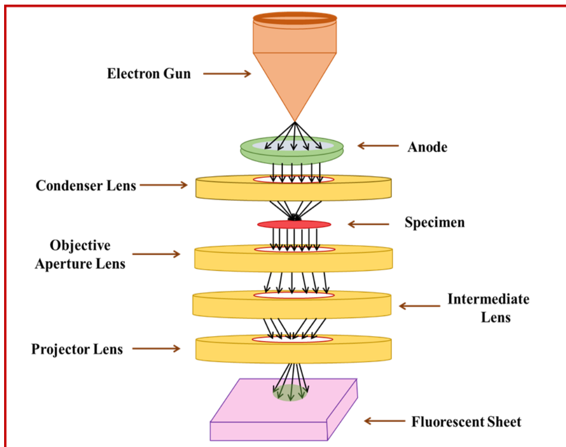
Figure 2.10: Schematic diagram representing the setup of transmission electron microscope
