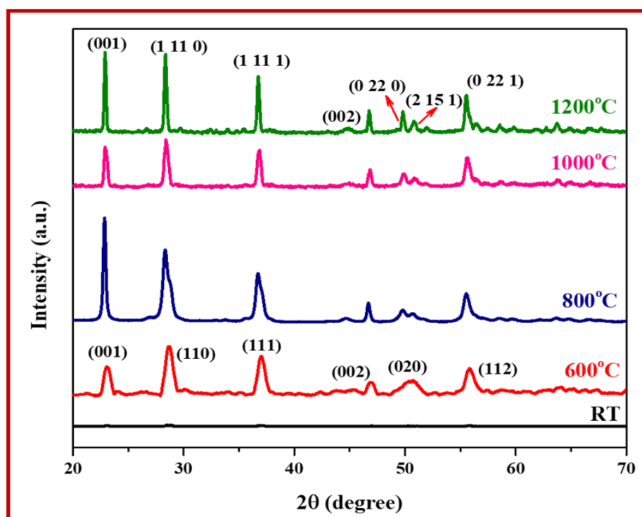
Figure 3.2: XRD pattern of synthesised \text{Ta}_2\text{O}_5 calcinated at different temperatures
