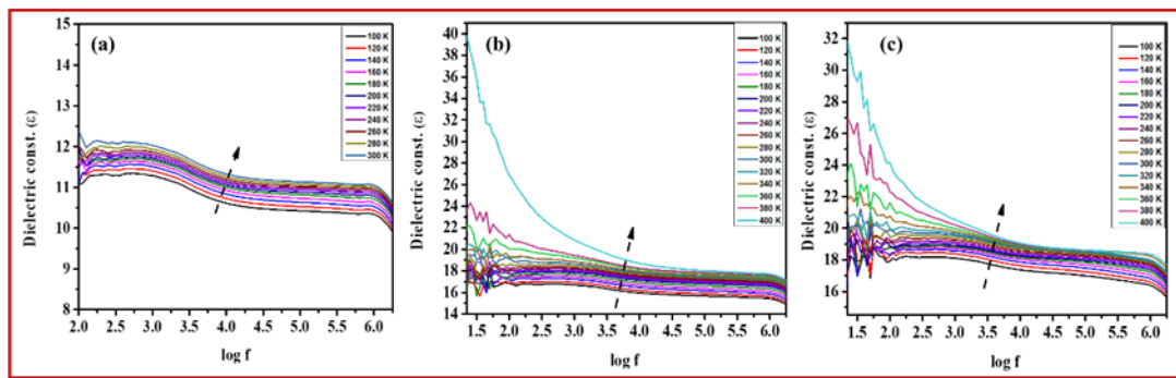
Figure 3.9: Dielectric constant ( \epsilon ) curves of \text{Ta}_2\text{O}_5 as a function of frequency at several operating temperatures for (a) as-synthesized sample, (b) sample sintered at 700 °C, and (c) 950 °C
