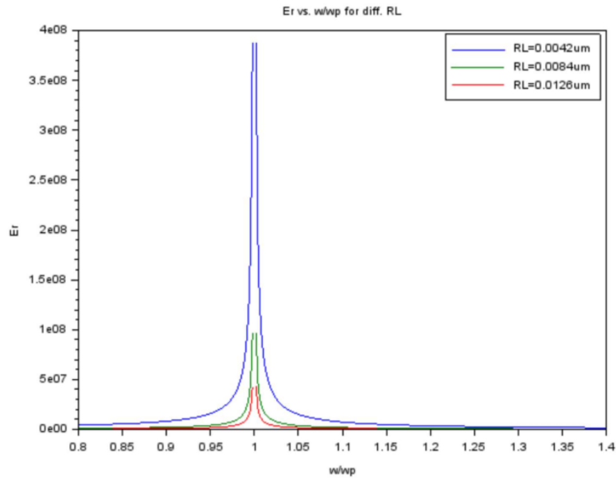
2 Fig. 1 Radial Electric field as a function of normalized field frequency for different focal spot size.
