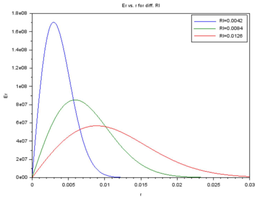
Fig. 5 Radial Electric field as a function of parameter r for different focal spot size.
