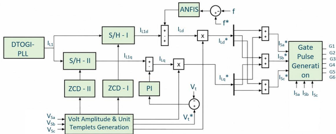
Fig.3.3 Pulse Generation
