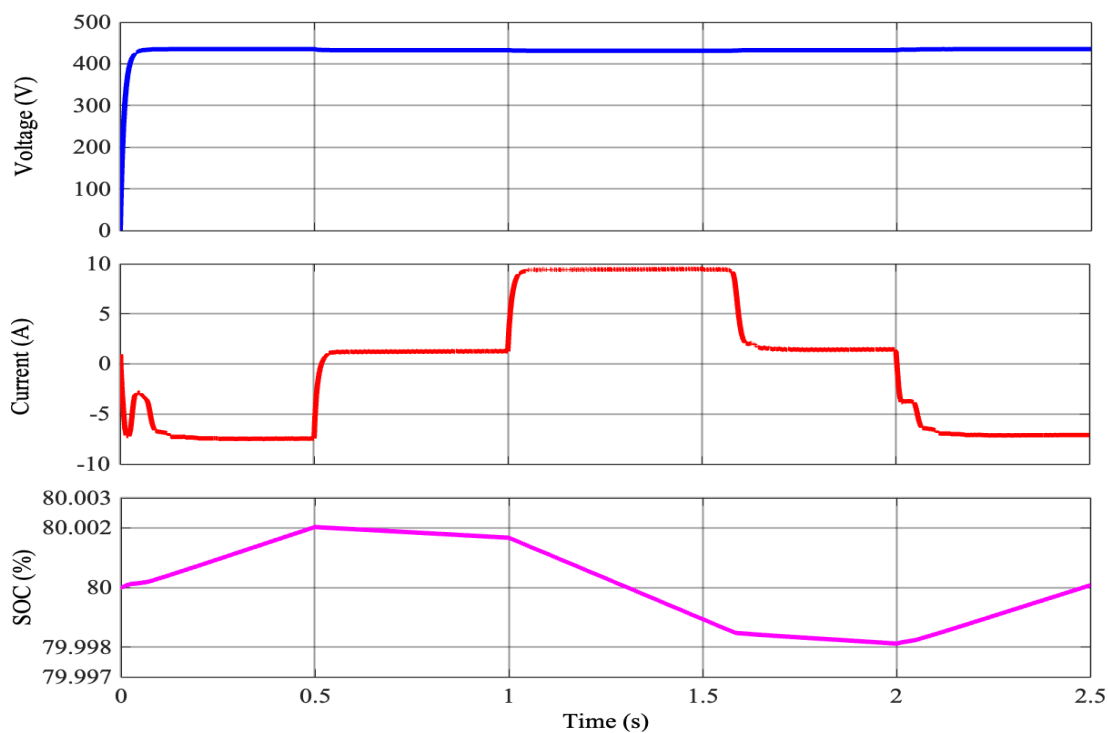
Fig. 4.4. Battery Voltage, Battery Current and SOC %
