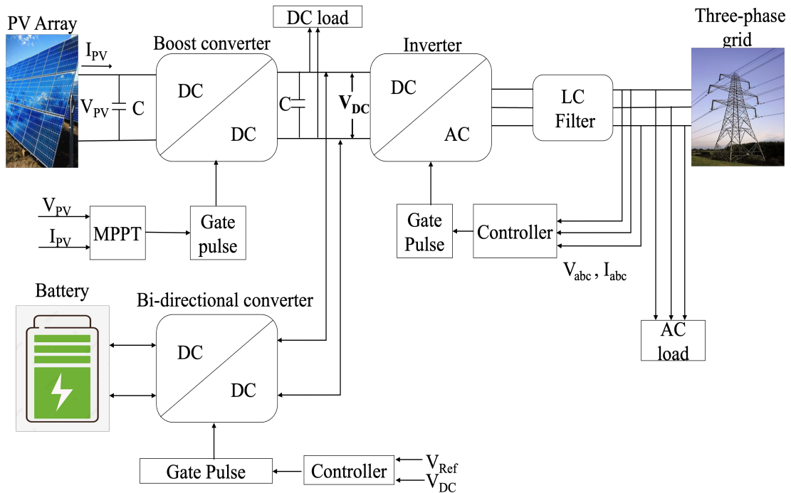
Fig. 2.1. Schematic representation of a dual-stage converter with BESS.
