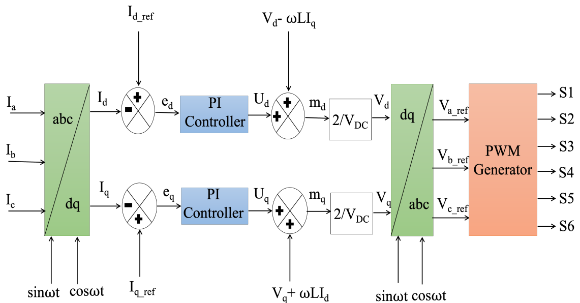
Fig. 3.3 Block diagram for inverter control
