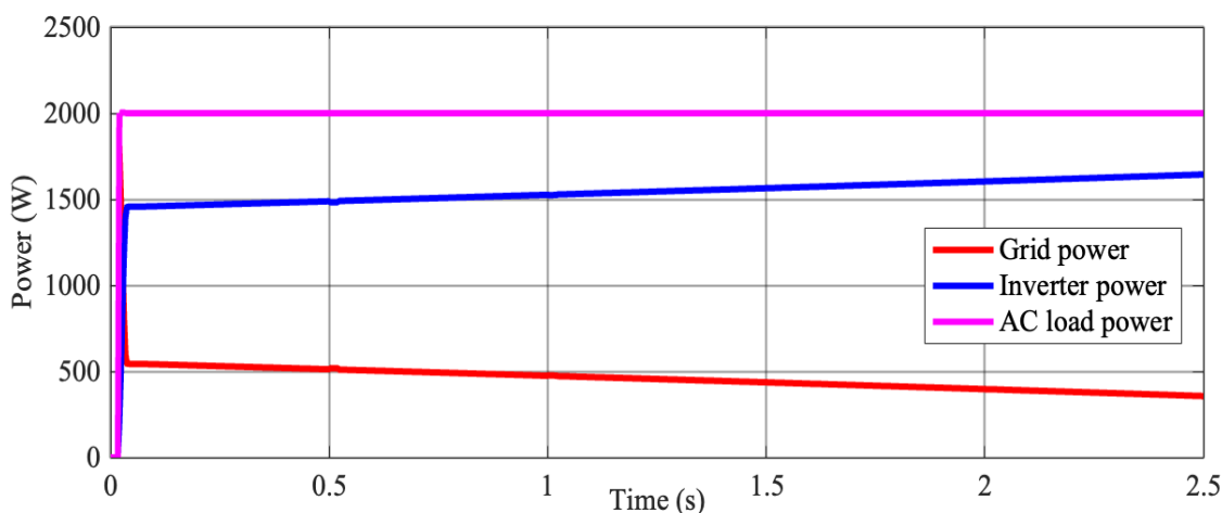
Fig. 4.10 Grid power, Inverter power and AC load power
