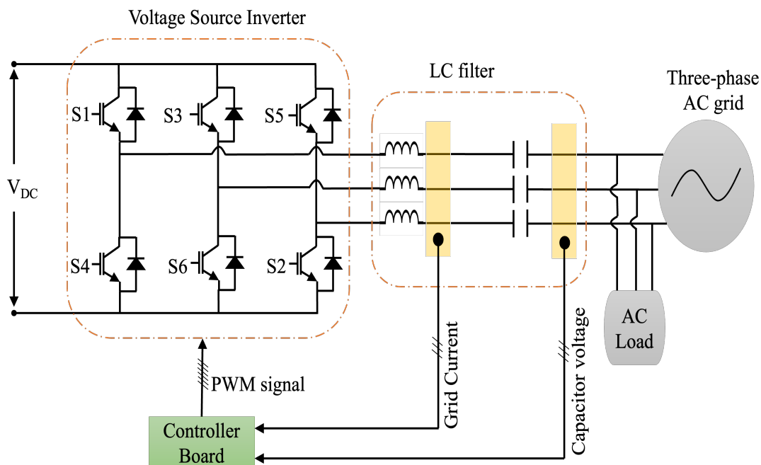
Fig. 2.4 Grid-connected VSI
