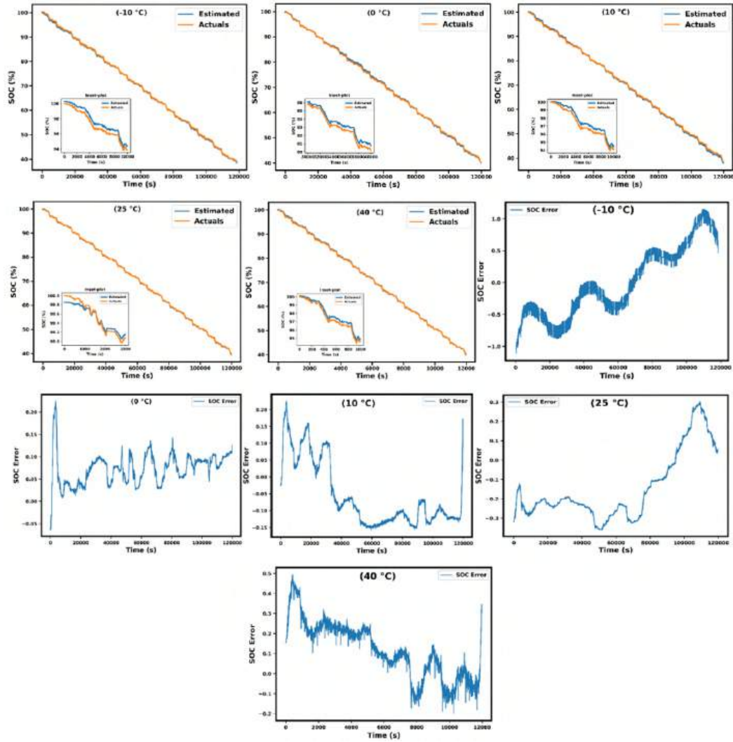
Figure 6.14 Actual and estimated performances and errors with GRU under different temperatures.
