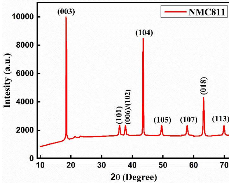
Figure 3.4 X-ray diffraction of pattern of NMC811 sample
