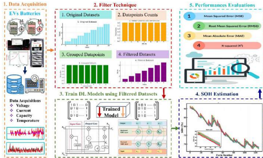
Figure 5.1 The proposed SOH estimation framework with filter technique
