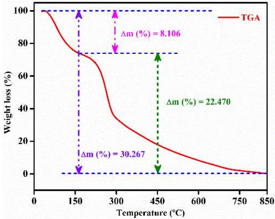
Figure 3.2 Thermogravimetric analysis of synthesized NMC811 sample
