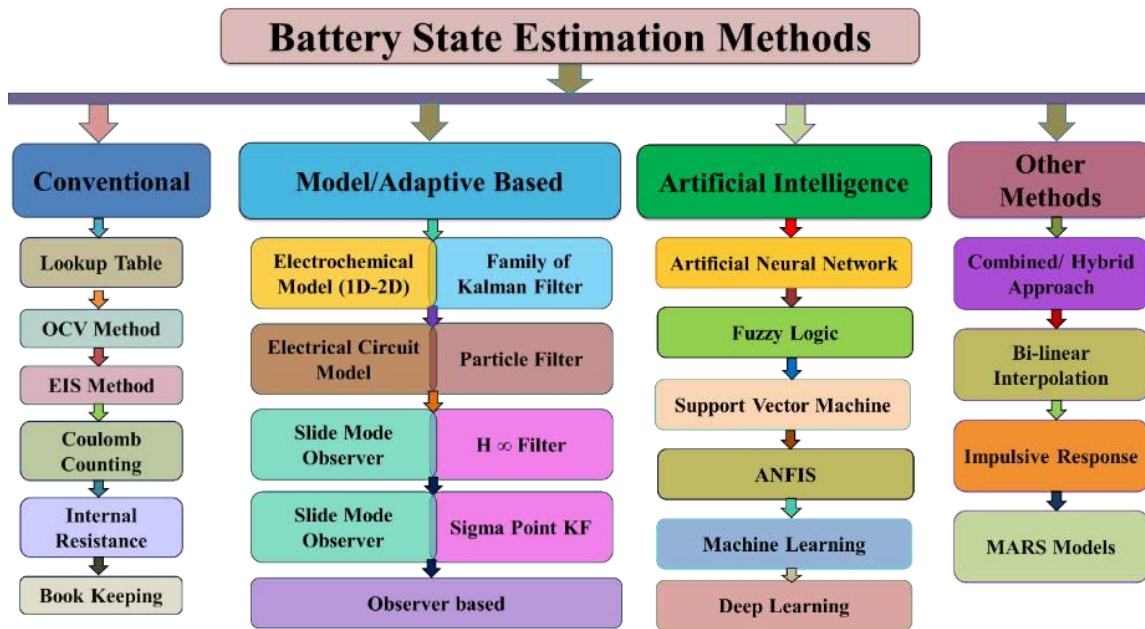
Figure 2.4 Different types of battery states estimation techniques
