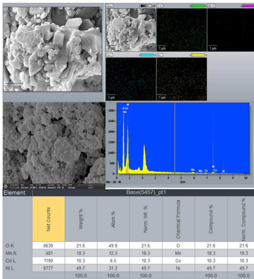
Figure 3.5 SEM images and EDX spectra of NMC811 sample
