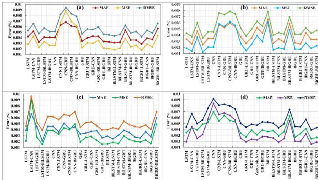
Figure 6.4 SOH estimation errors against the measurements of D1-D4 batteries, (a-d).
