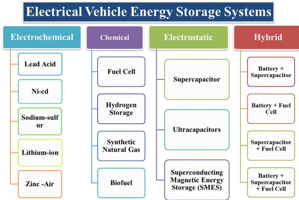
Figure 2.2 Different types of electric vehicle energy storage systems
