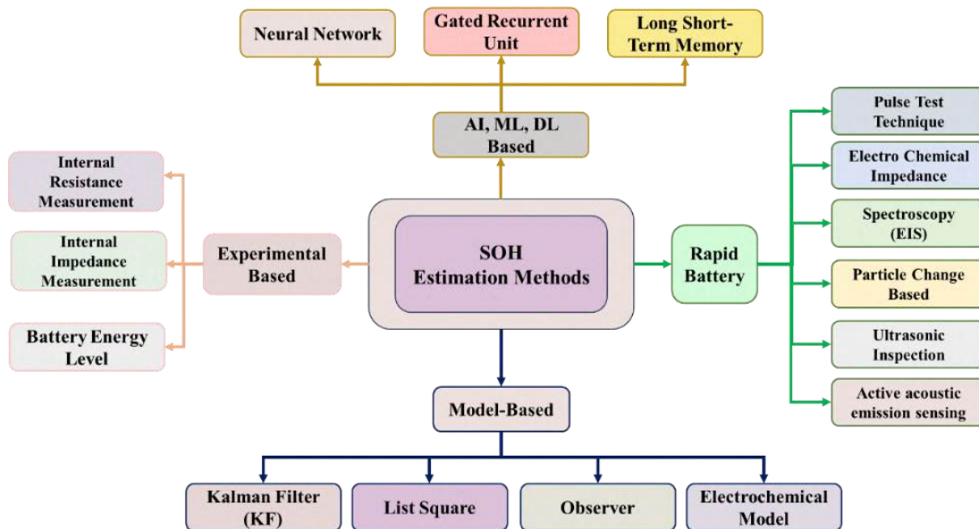
Figure 2.6 Classification of approaches for SOH estimation
