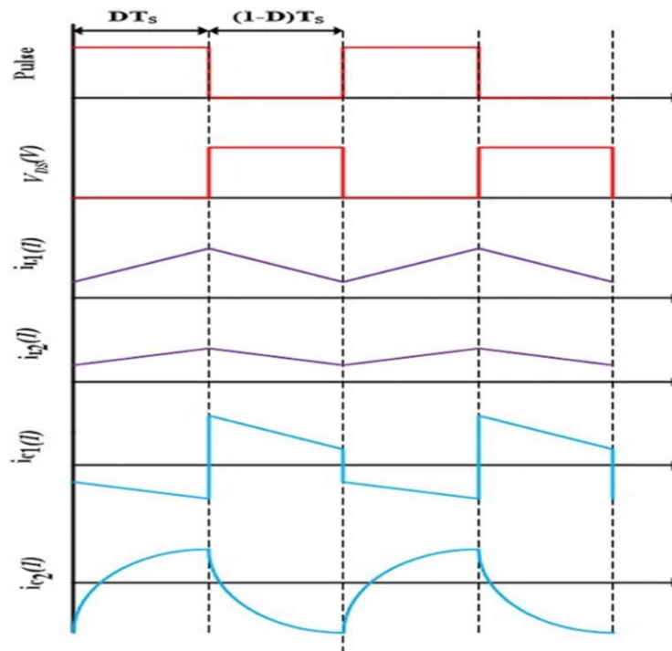
Fig 2.5: Switching waveform for Quadratic Boost converter.
