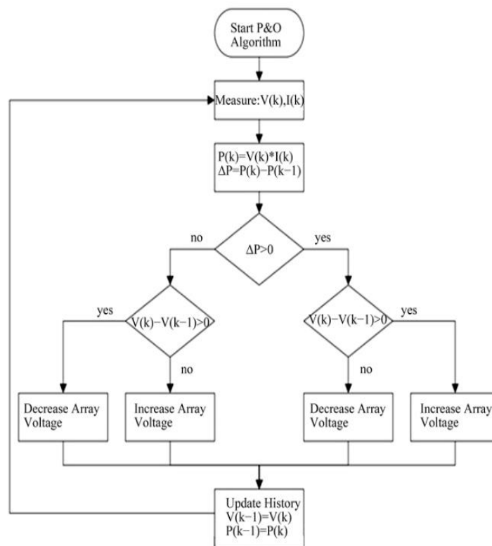
Fig.5.1: Flow Chart of P & O Technique
