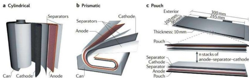
Figure 3.2: The three most common battery cells used in electric vehicle battery packs: a Cylindrical, b Prismatic and c “Pouch”. Taken from the article: “ Promise and reality of postlithium-ion batteries with high energy densities ” [6]
