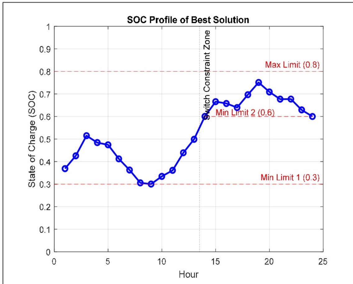
Fig 5.4: SOC Profile of Best Solution Curve
