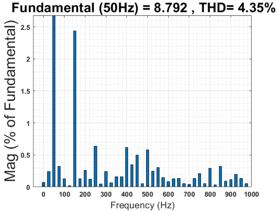
Figure 6.3: FFT analysis of source current with GI controller. THD = 4.35%, fundamental = 8.792 A.
