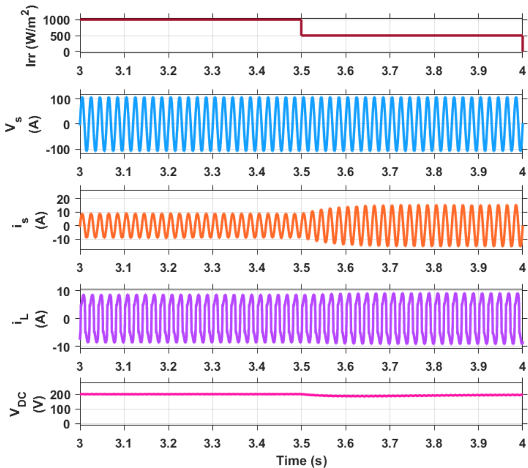
4 Figure 6.1: Time-domain waveforms with HNN controller: Irradiance, source voltage V_s , source current i_s , Load current i_L , and DC link voltage V_{dc} .
