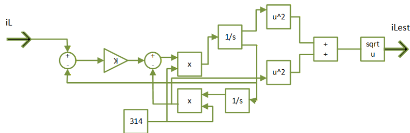
Figure 5.1: Block diagram of the Generalized Integrator based reference current estimation algorithm.
