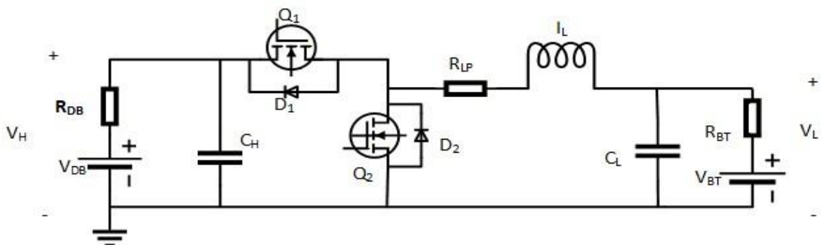
Fig.2.1. Circuit diagram of buck boost converter
