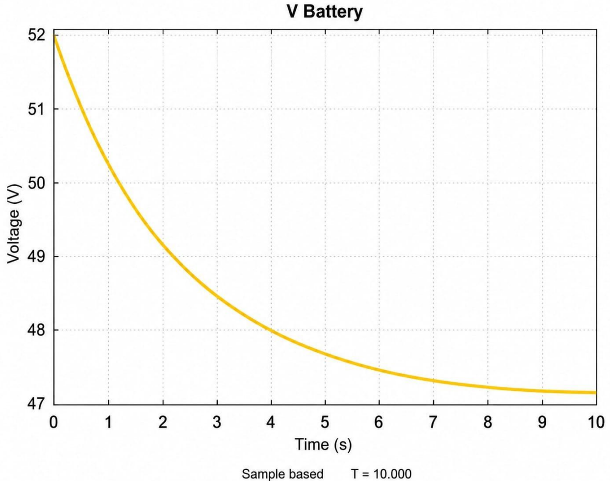
Fig.4.2. Battery voltage response during discharge
