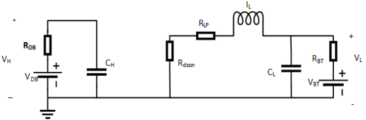
Fig.4.4.Boost mode circuit topology
