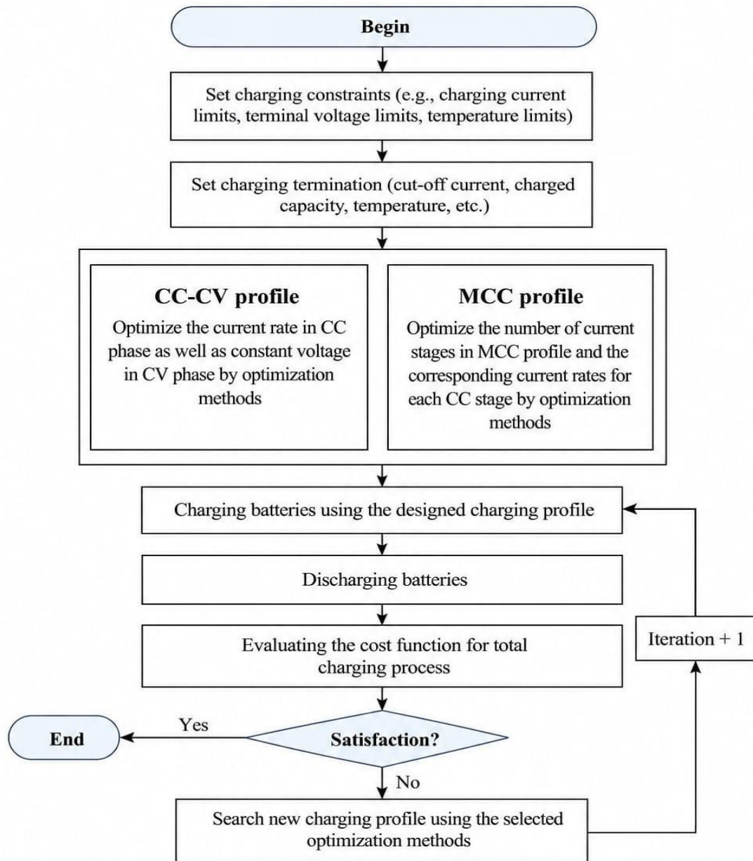
Figure.7.2 Overview of enhancements to the CC-CV/MCC charging strategy [39]
