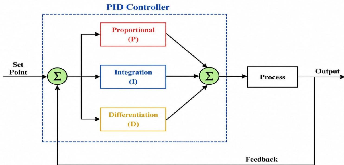
Fig.3.6. Block diagram of PID controller
