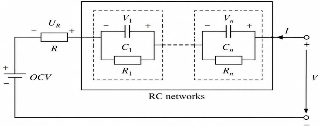
Fig.5.3 Battery circuit diagram
