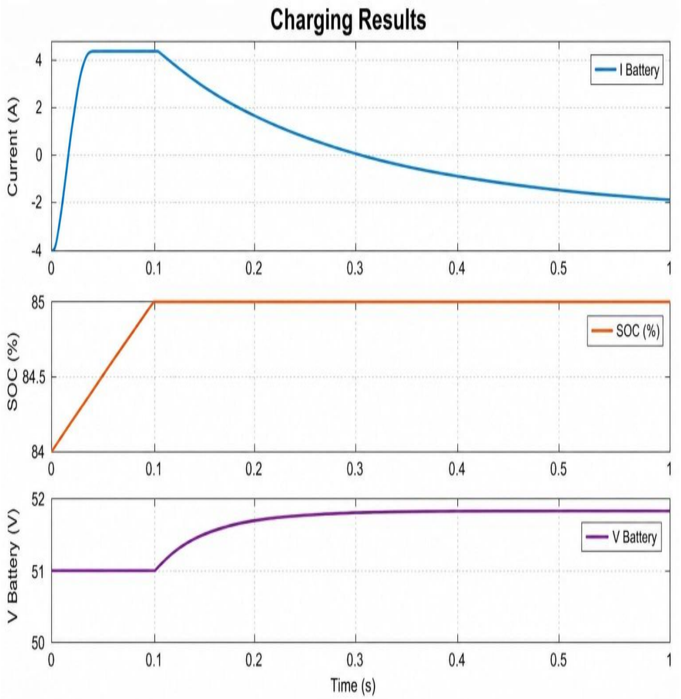
Fig.9.3. graph showing V Battery, I Battery
