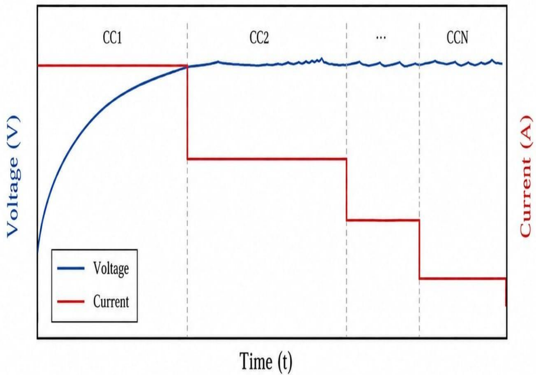
Fig.6.3. The MCC charging method's battery voltage and current
