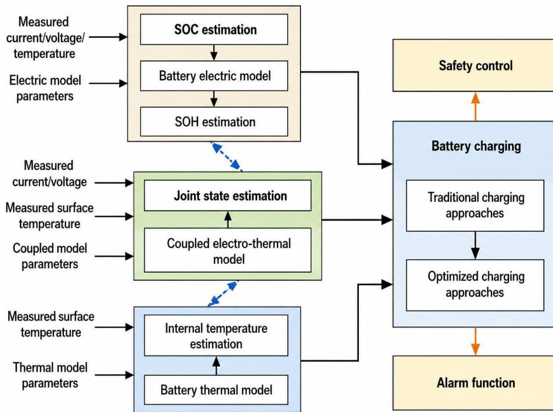
Fig.5.1. The relationship between the BMS's major technologies [39]
