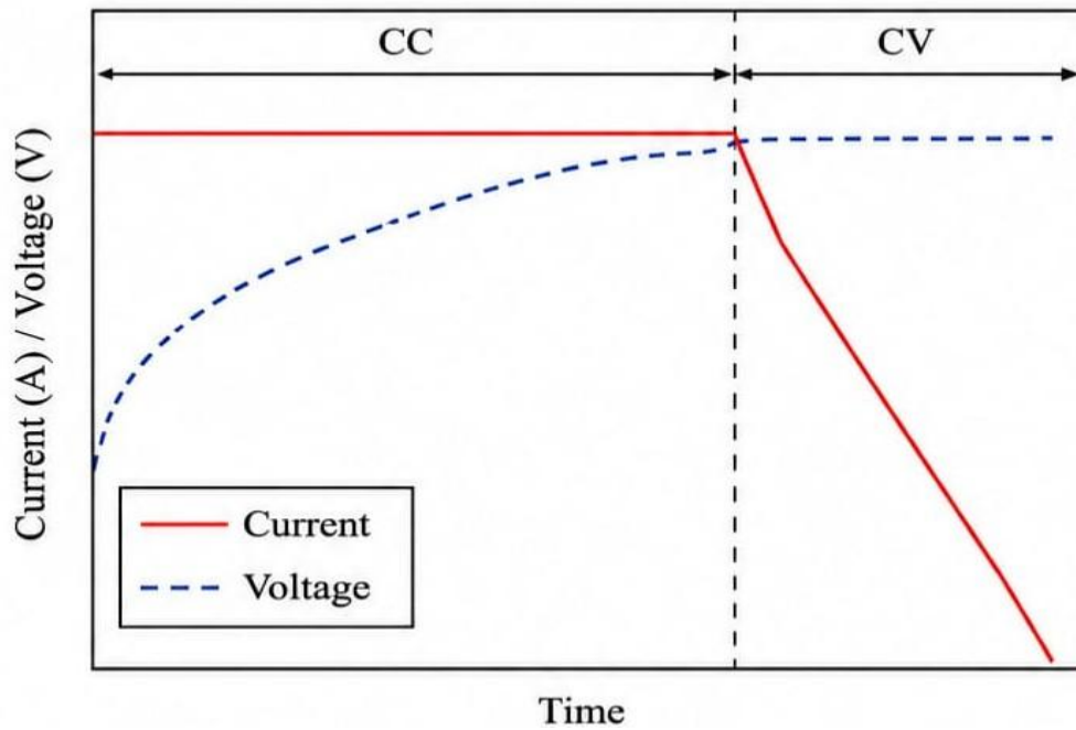
Fig.6.2. The CC-CV charging method's battery voltage and current
