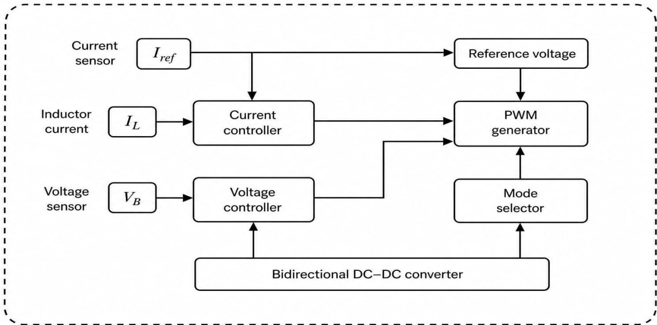
Fig.8.2 Block diagram of the proposed Converter Control System
