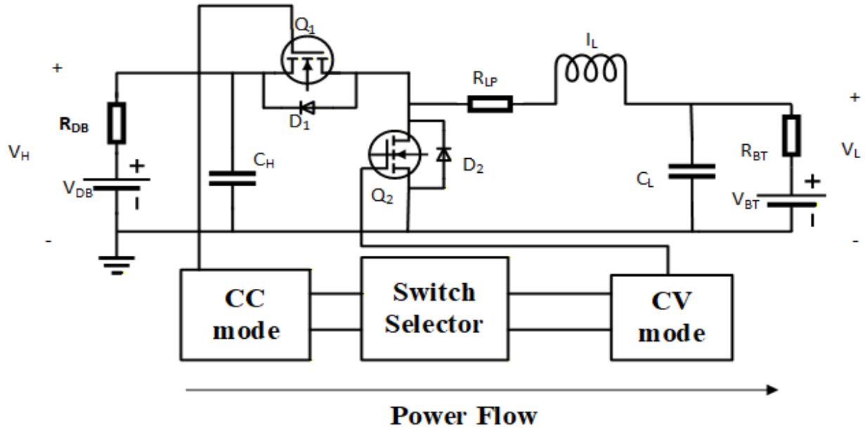
Fig. 8.1 Simulation Schematic of the proposed control algorithm of Converter
