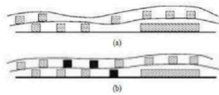
Fig. 1.4 ILD planarization due to non-uniform layout density
