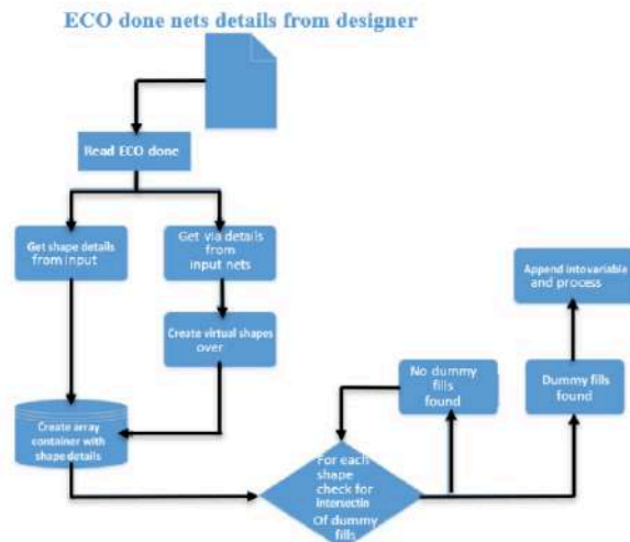
Fig. 5.1 Fill_Short_Finder tool flow
