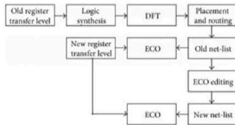
Fig. 2.2 Typical ECO Design Flow
