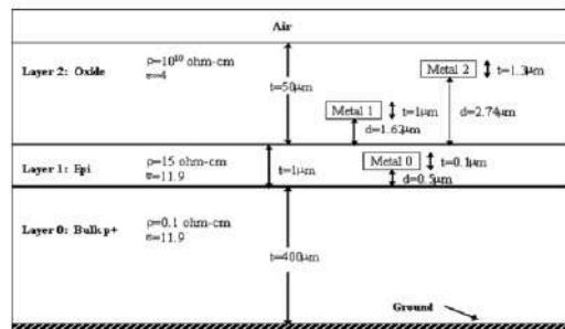
Fig. 5.3: CMOS cross-section view
