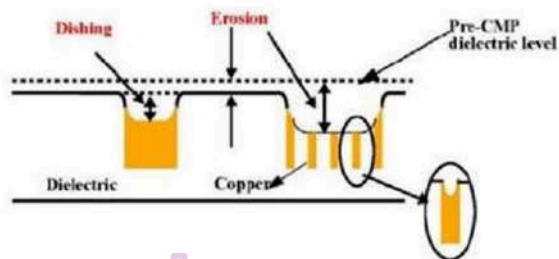
Fig. 1.3 Metal dishing and dielectric erosion
