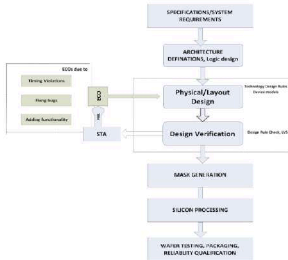
Fig. 1.1 ASIC Design Flow
