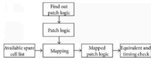
Fig. 2.3: Two-phase ECO design flow
