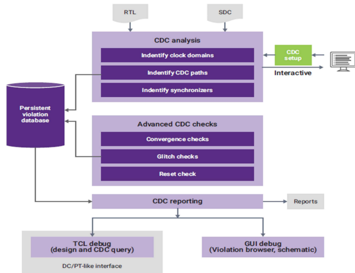
Figure 3.3: Spyglass CDC flow
