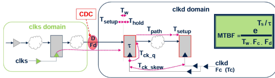
Figure 3.4: MTBF for a data flow between flops
