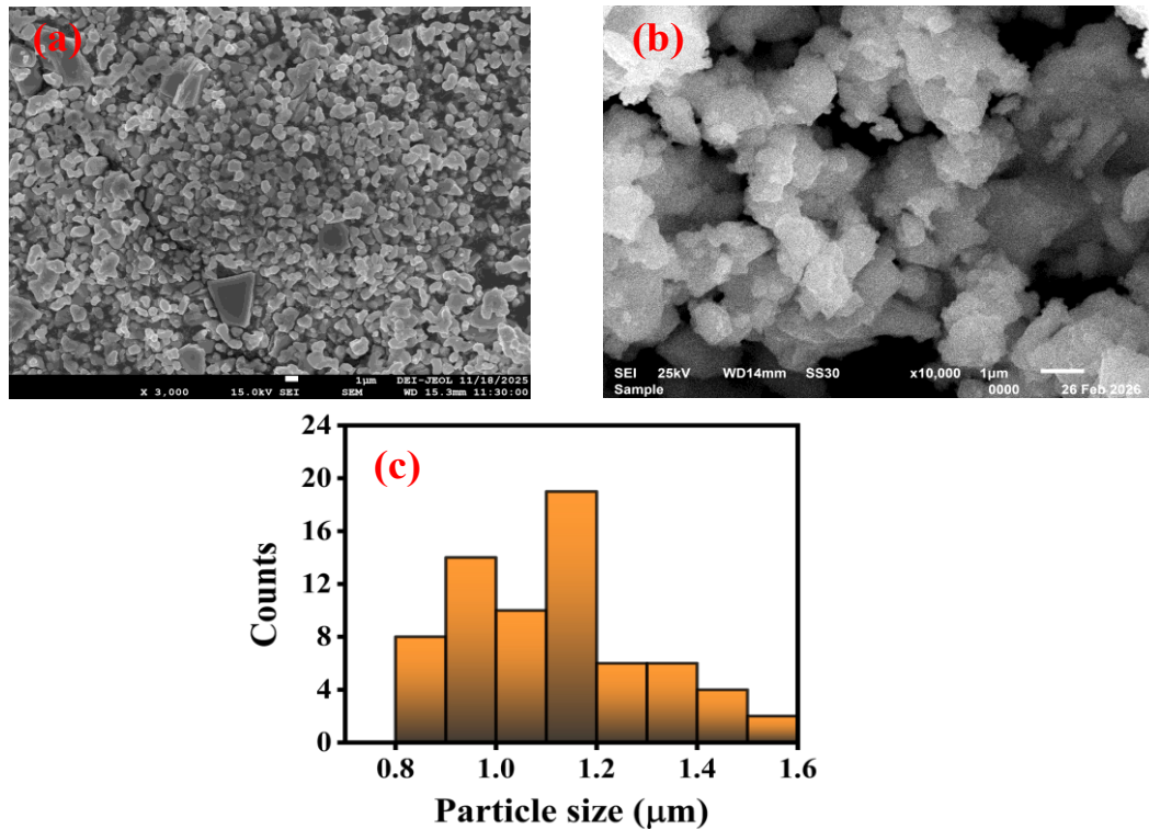
Figure 4.2: (a) SEM image for undoped BaSN, (b) For doped BaSN phosphor with 7.0 mol% concentration of \text{Eu}^{3+} , (c) Particle size distribution histogram obtained from SEM analysis.
