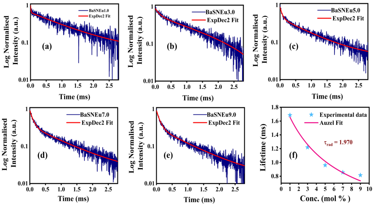
Figure 4.10: PL decay plots for \text{Eu}^{3+} doped \text{BaSN} phosphor with \text{Eu}^{3+} concentrations ( x=1.0, 3.0, 5.0, 7.0, 9.0 mol%) at \lambda_{\text{ex}}= 395 nm
