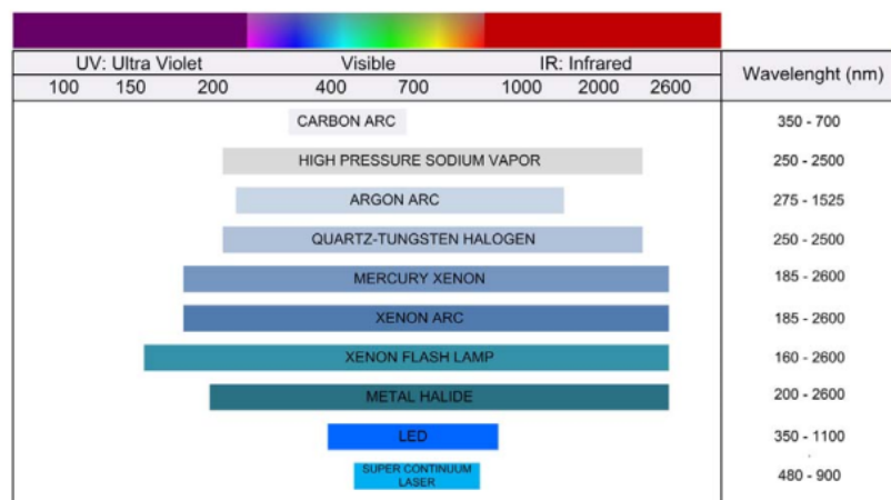
Figure 2.4: Wavelength range of light sources [3].
