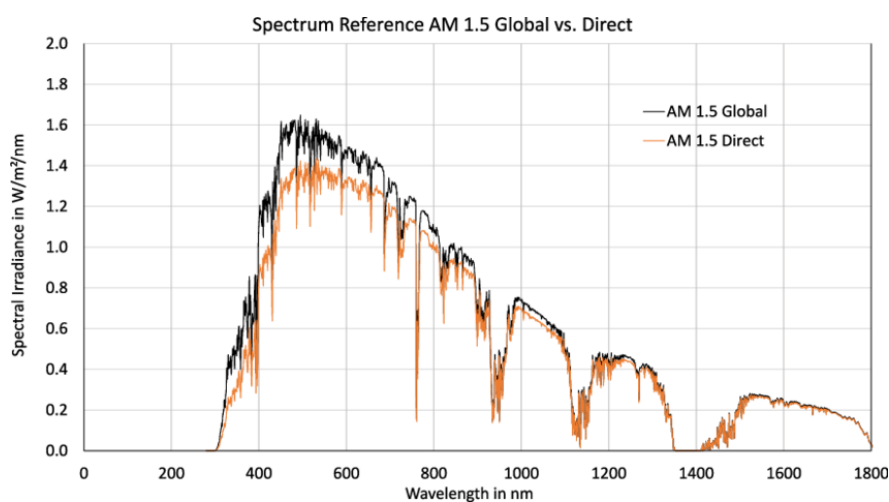
Figure 2.3: Spectrum reference AM 1.5 Global vs Direct [5]
