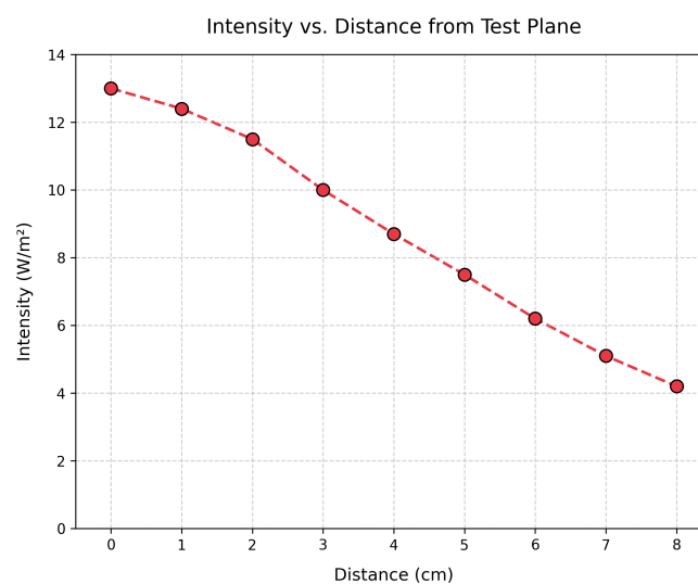
Figure 4.4: Intensity vs distance plot
