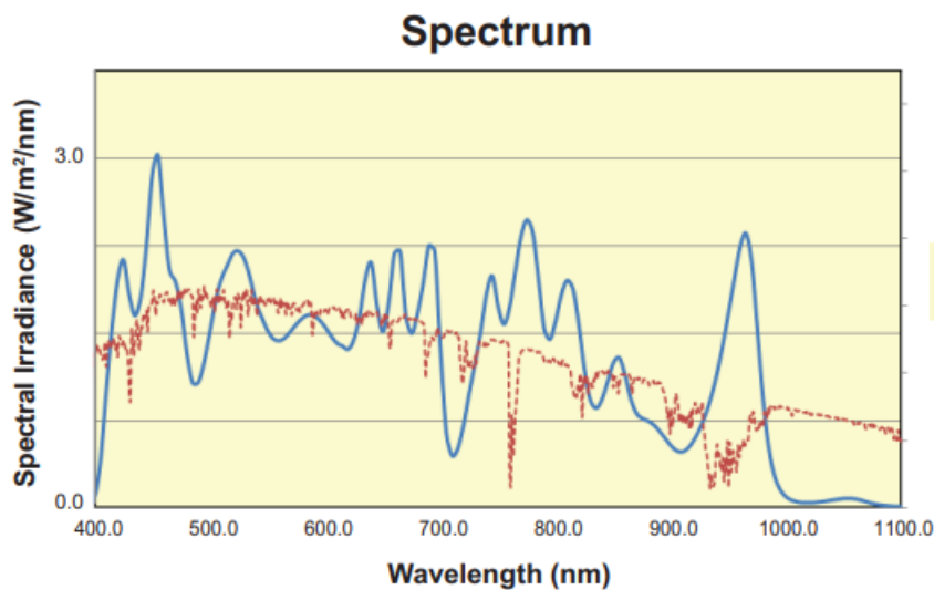
Figure 2.8: Solar simulator spectrum of Newport's VeraSol-2 [13].
