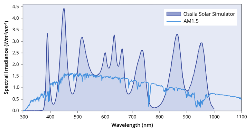
Figure 2.7: Solar simulator spectrum of Ossila Solar Simulator [12].
