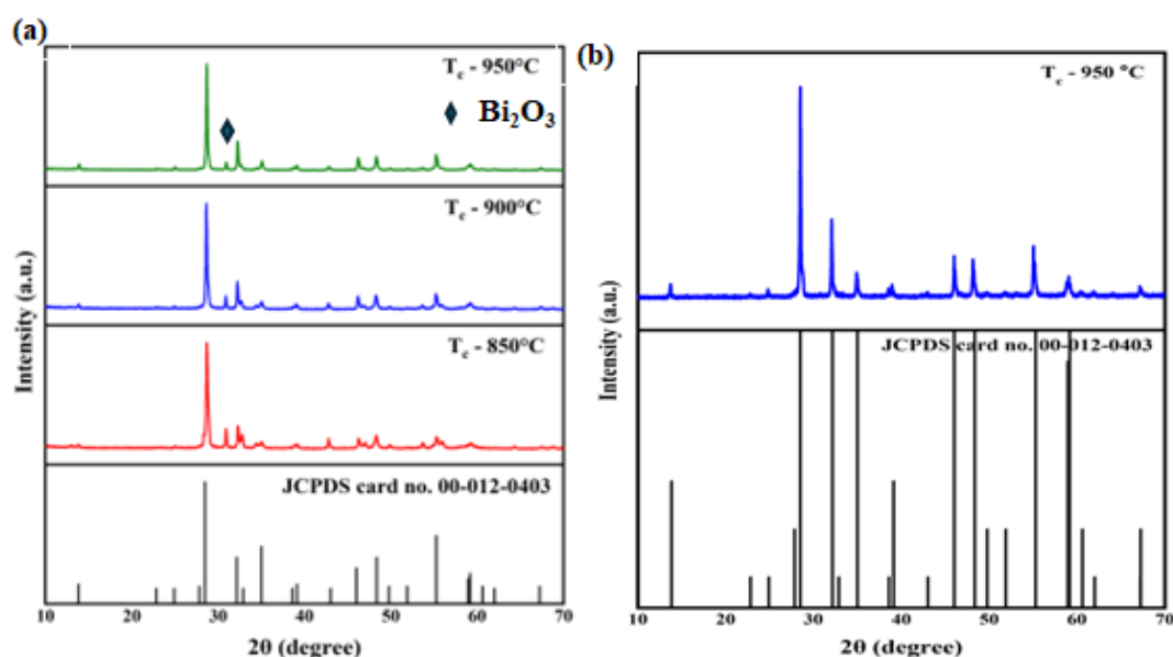
Fig. 3.1 XRD patterns of \text{BaBi}_2\text{Nb}_2\text{O}_9 ceramics showing (a) temperature optimization for calcination and (b) elimination of impurity phase upon addition of 2 wt% excess \text{Bi}_2\text{O}_3 at 950°C.
