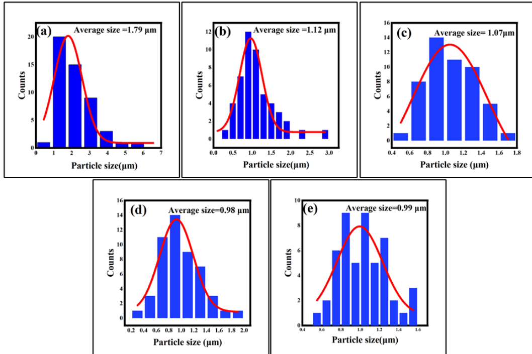
Fig. 3.5. Histograms of particle sizes obtained from SEM images of (a) BBNB0, (b) BBNB1, (c) BBNB2, (d) BBNB3, and (e) BBNB4 ceramics are shown. The solid curves represent Gaussians, which were fitted to get the average particle size.
