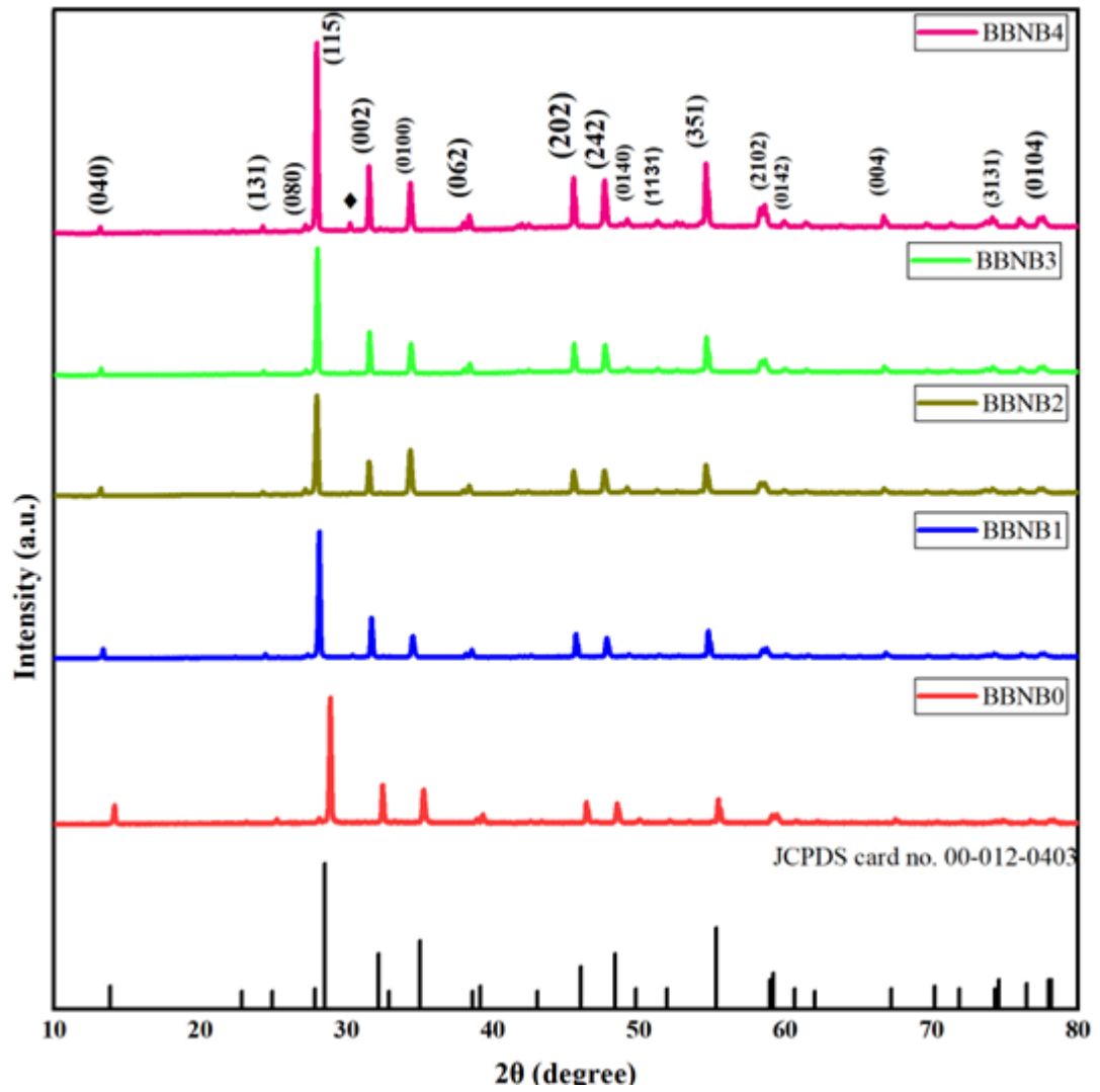
Fig. 3.3. XRD plot of all compositions of BBN
