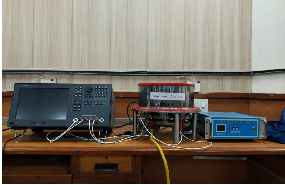
Fig 3.17. DIELECTRIC INSTRUMENT
