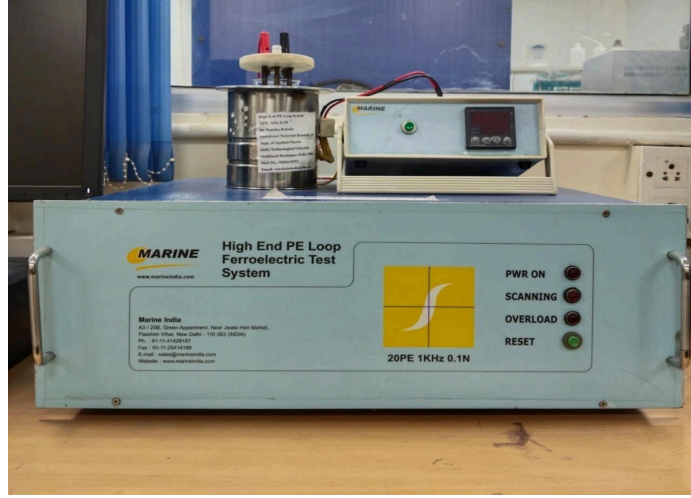
Fig. 3.13. P-E loop measurement instrument
