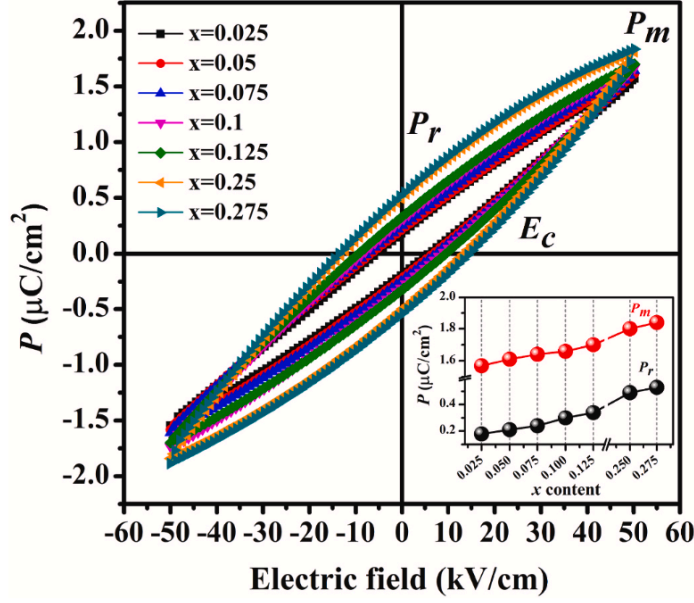
Fig. 1.2: Ferroelectric hysteresis loop ( P - E ) of \text{SrBi}_{2-x}\text{Nd}_x\text{Nb}_2\text{O}_9 measured at room temperature. The inset shows the polarisation ( P_r and P_m ) dependence on x content.
