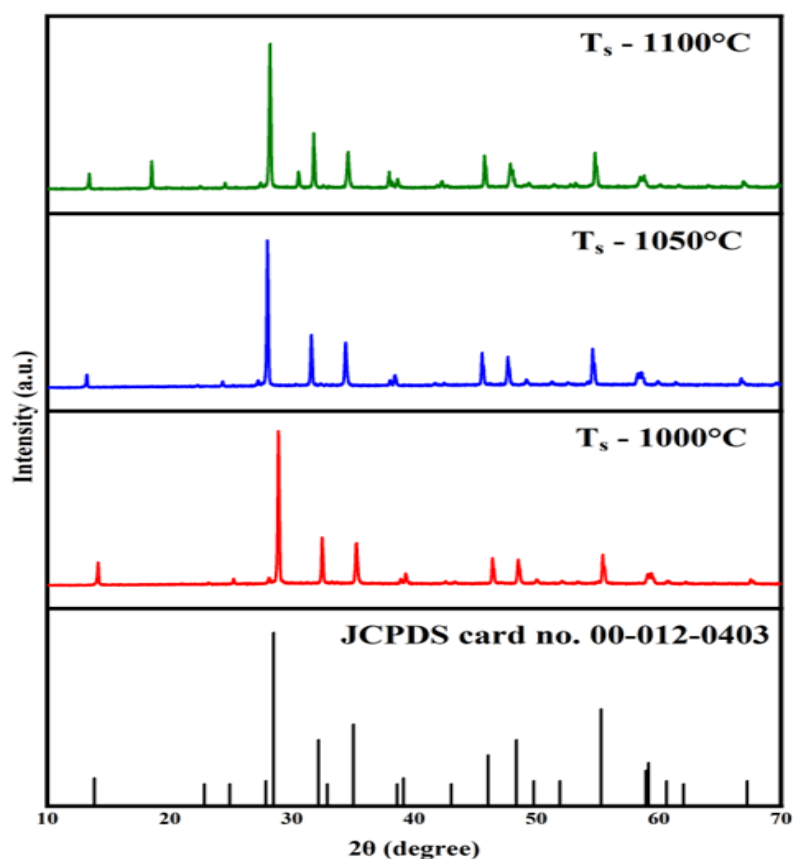
Fig. 3.2 XRD patterns of \text{BaBi}_2\text{Nb}_2\text{O}_9 ceramics sintered at 1000°C, 1050°C, and 1100°C, compared with the standard JCPDS card no. 00-012-0403, showing the effect of sintering temperature on phase purity.
