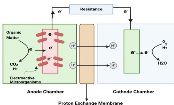
Fig 2.1: Schematic diagram of dual-chamber Microbial Fuel Cell
