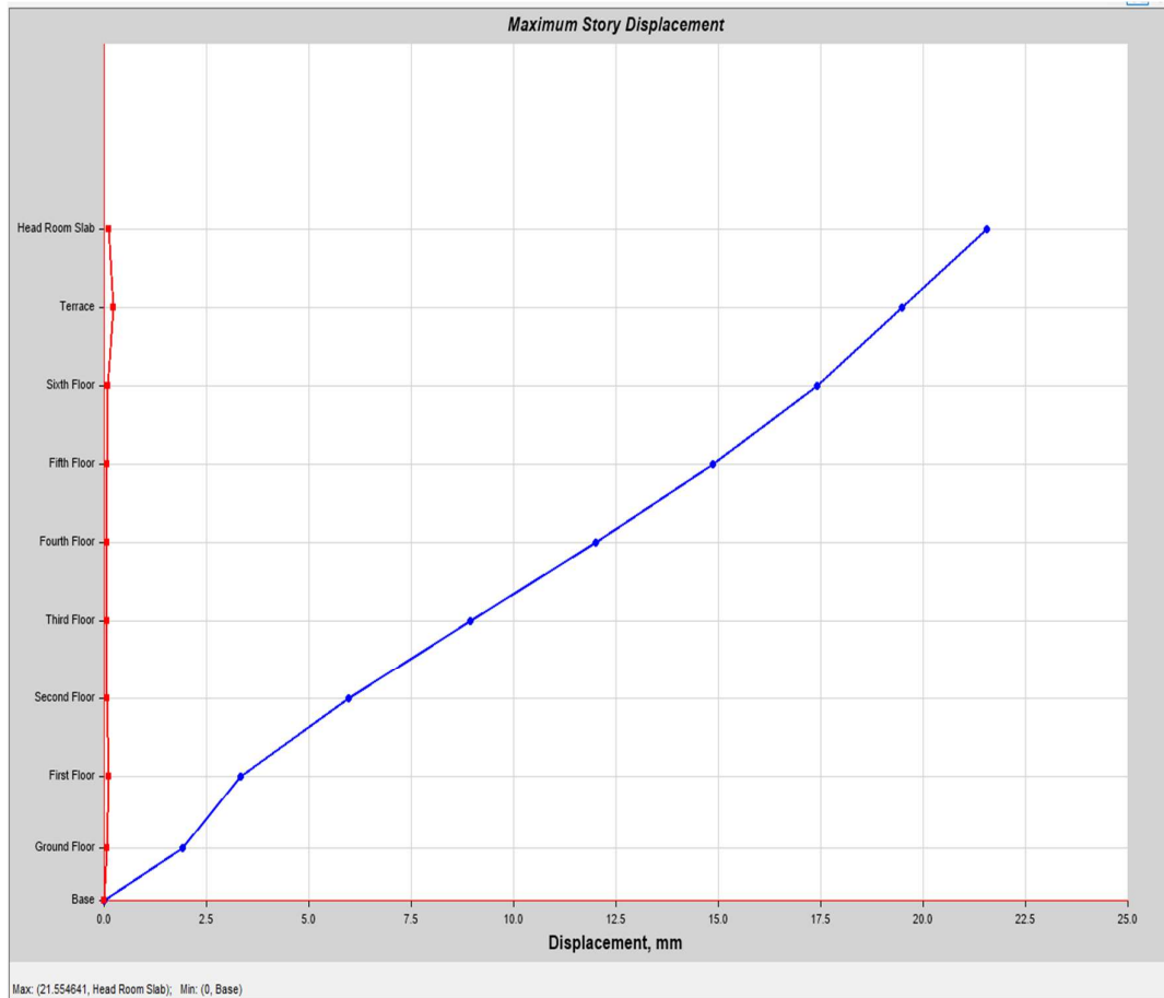
Fig 4.3.1: Maximum storey displacement of CASE C.
