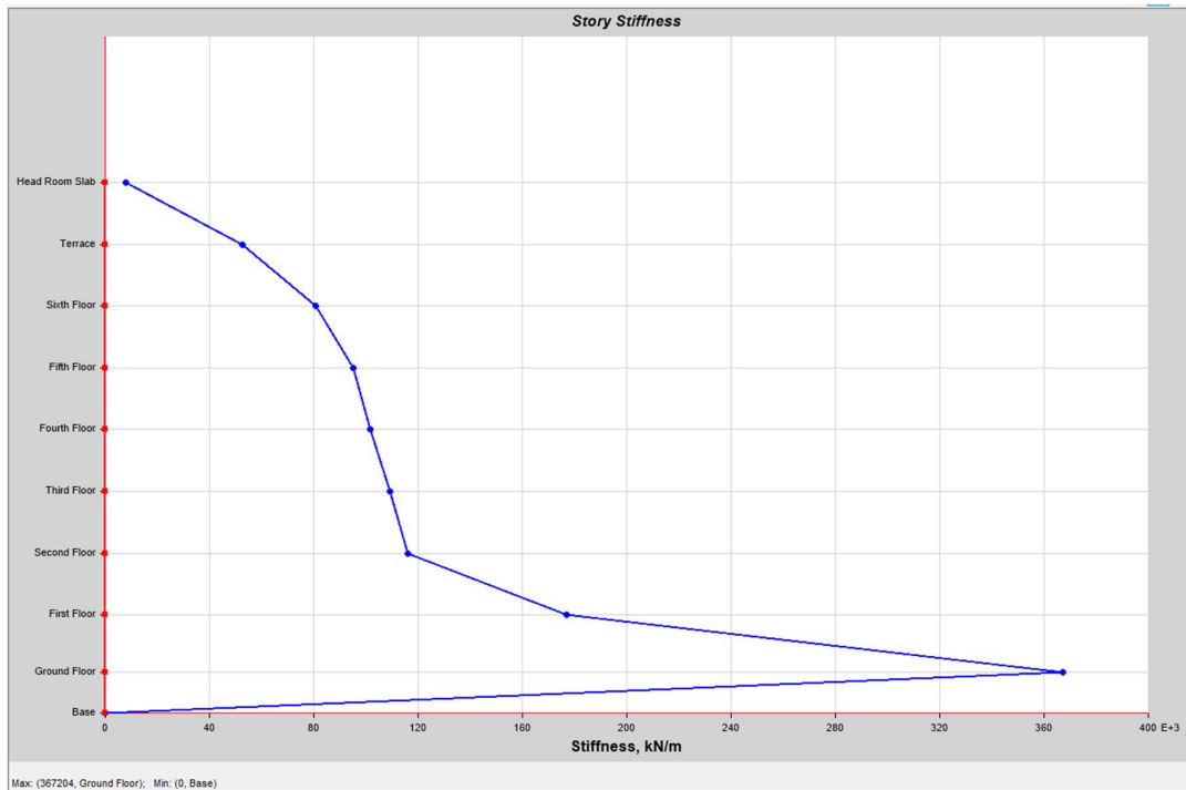
.Fig 4.1.3: storey Stiffness of CASE A.
