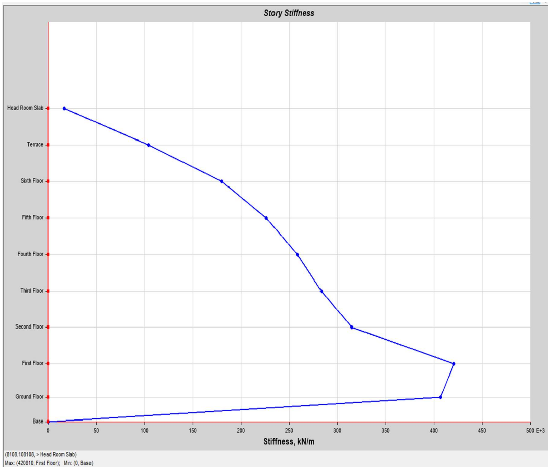
Fig 4.5.3: storey stiffness of CASE E.
