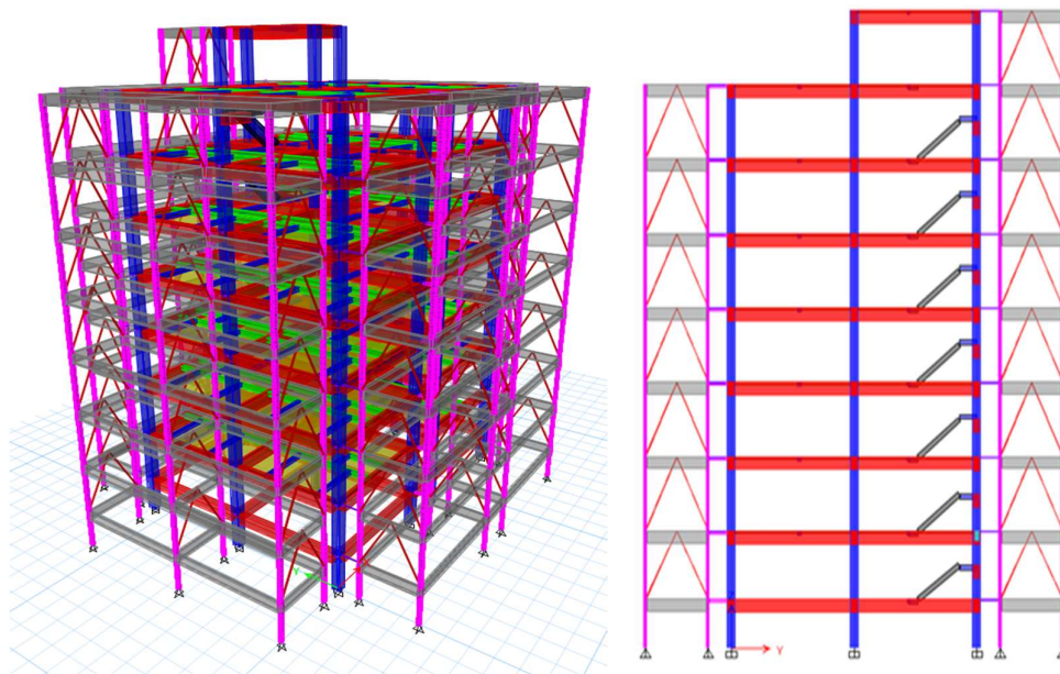
Fig 3.4: 3D view and elevation of V-braced exoskeleton.
