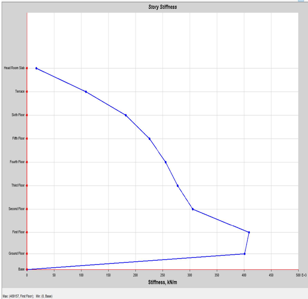
Fig 4.3.3: storey stiffness of CASE C.
