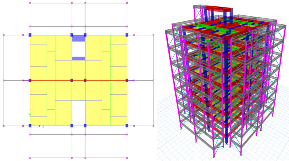
Fig 3.3: Plan & 3D view of X-braced exoskeleton.
