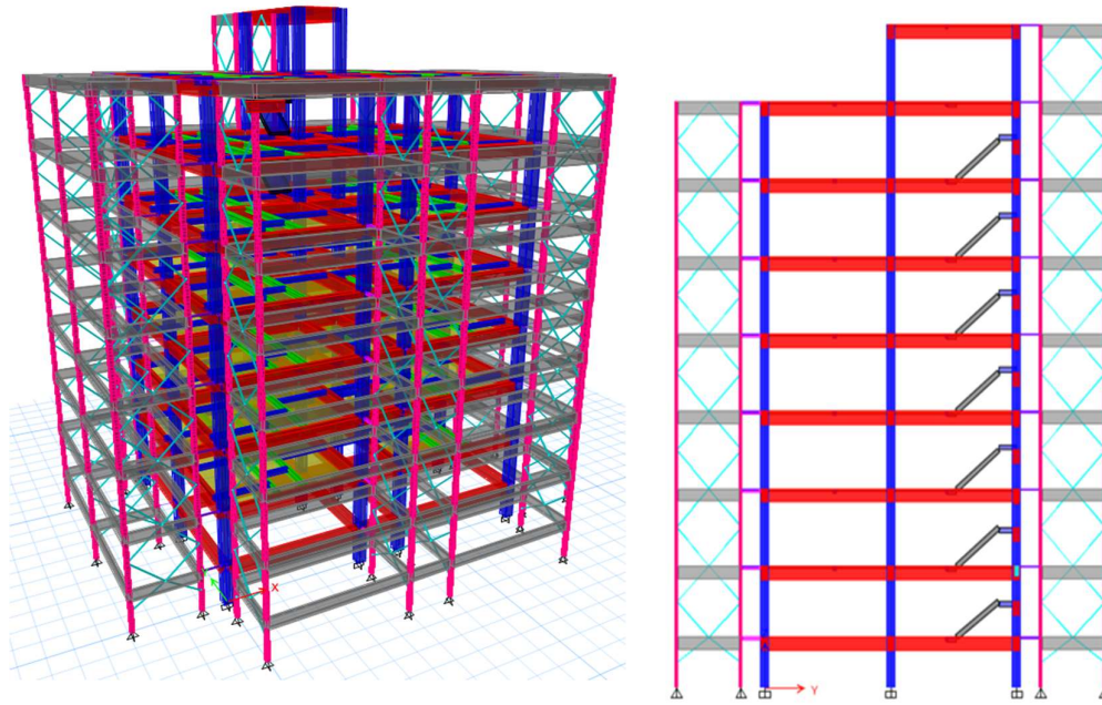
Fig 3.6: 3D view and elevation of Diamond-braced exoskeleton.
