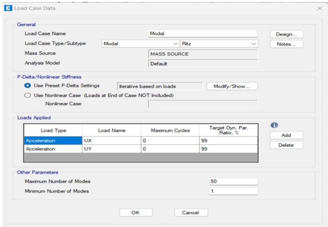
Fig 3.2.4: Model analysis definition.
