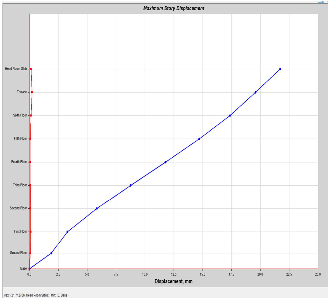
Fig 4.5.1: Maximum storey displacement of CASE E.
