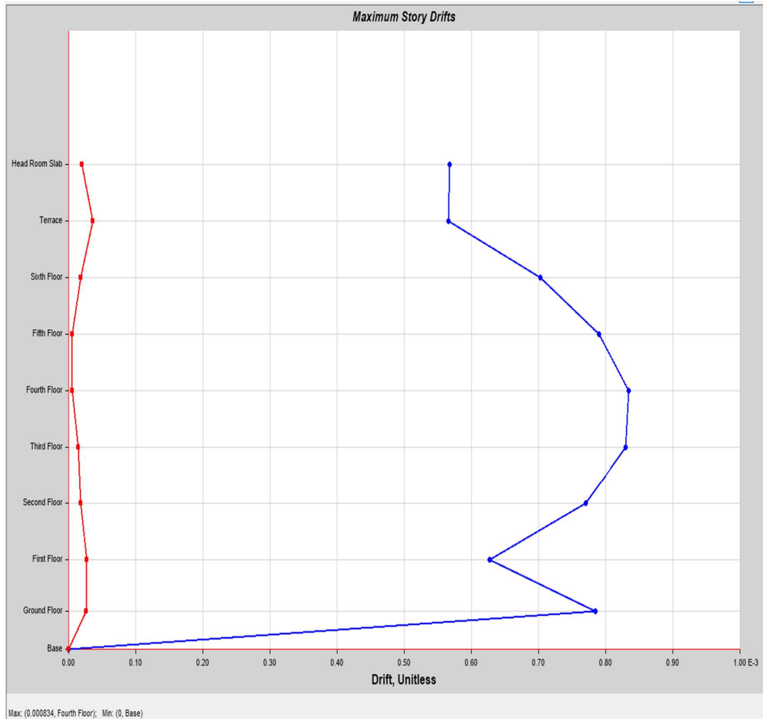
Fig 4.3.2: Maximum storey drift of CASE C.
