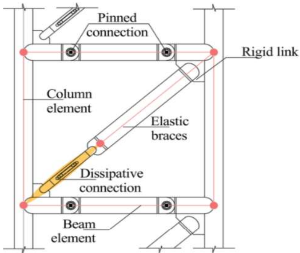
Fig 1.7.3: Hybrid Exoskeleton System.
