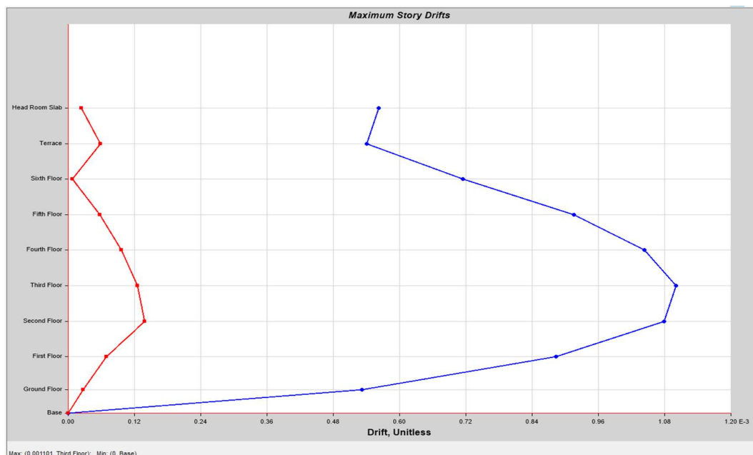
Fig 4.1.2: Maximum storey drifts of CASE A.
