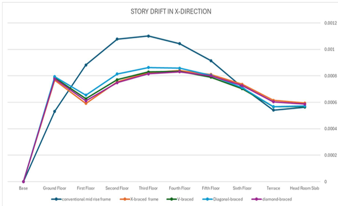
Fig 5.2: Comparative results of story drift under R S A .
