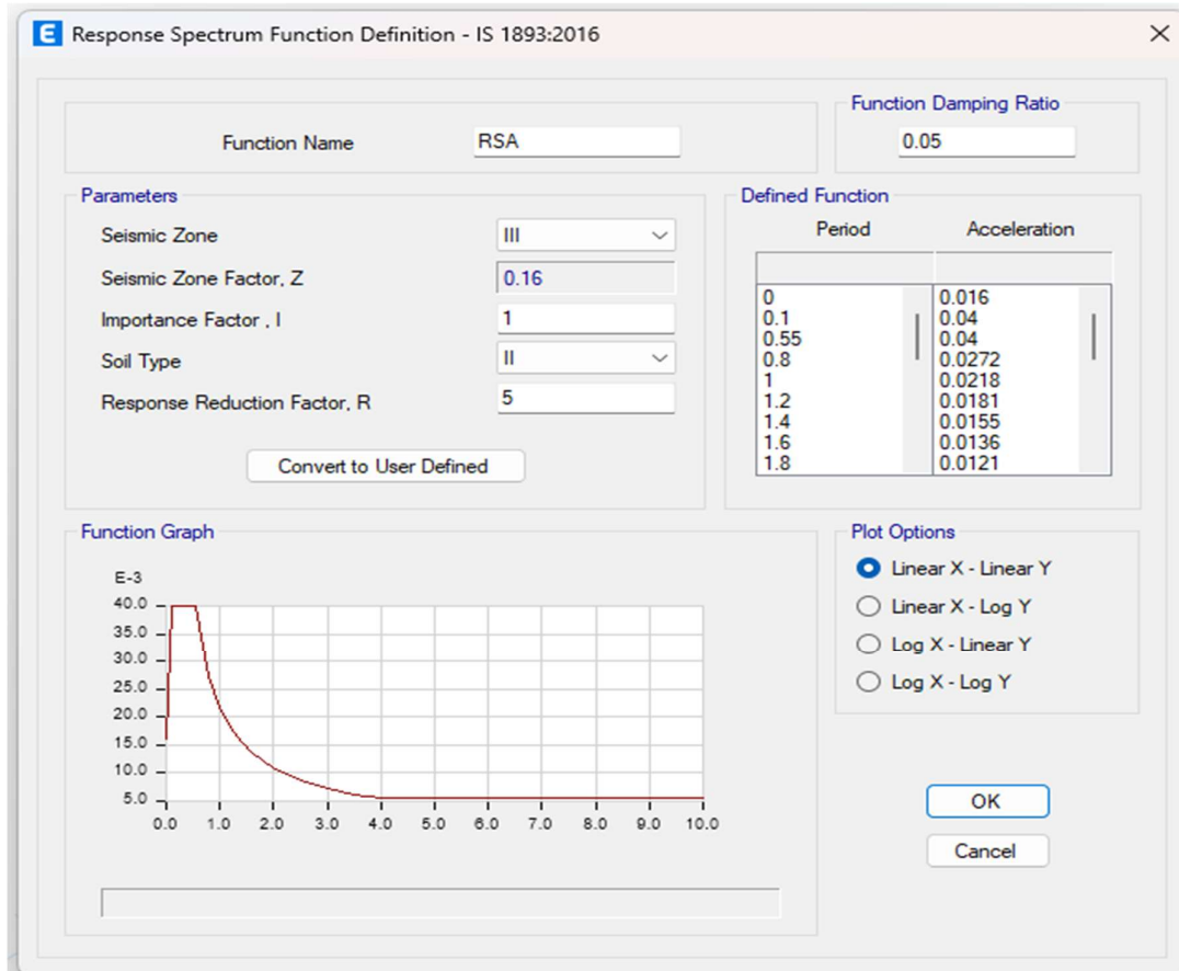
Fig 3.2.3: Response spectrum definition
