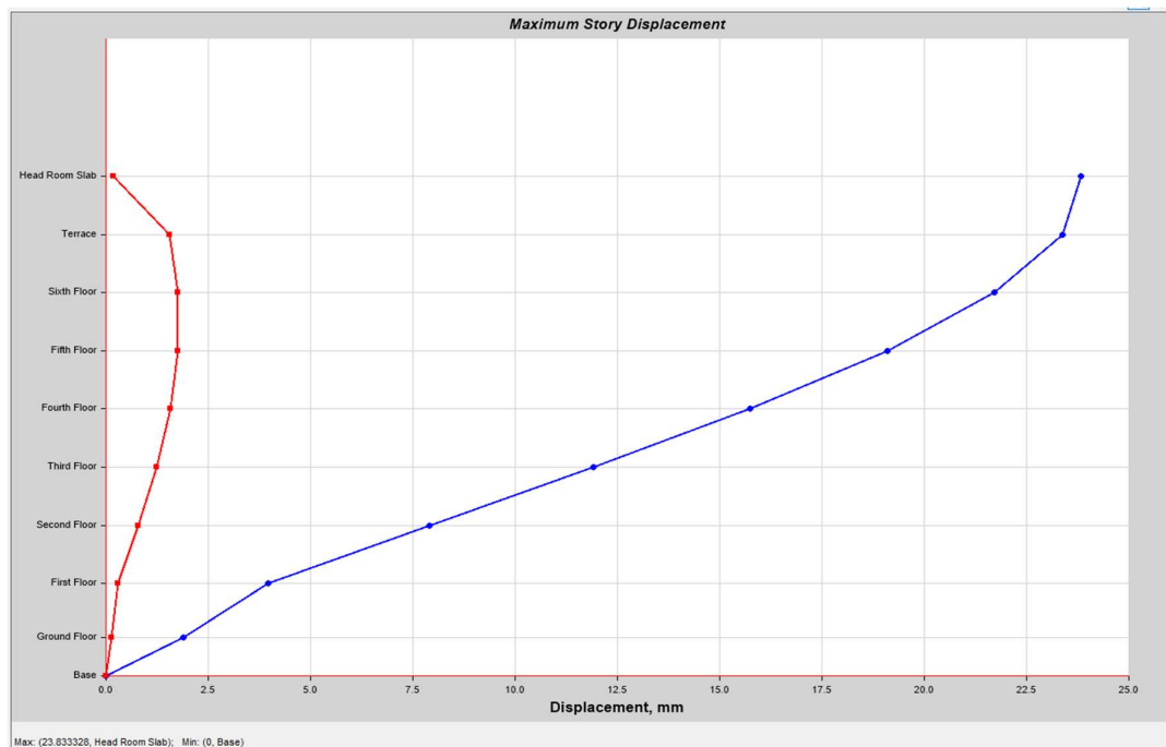
Fig 4.1.1: Maximum storey displacement of CASE A.
