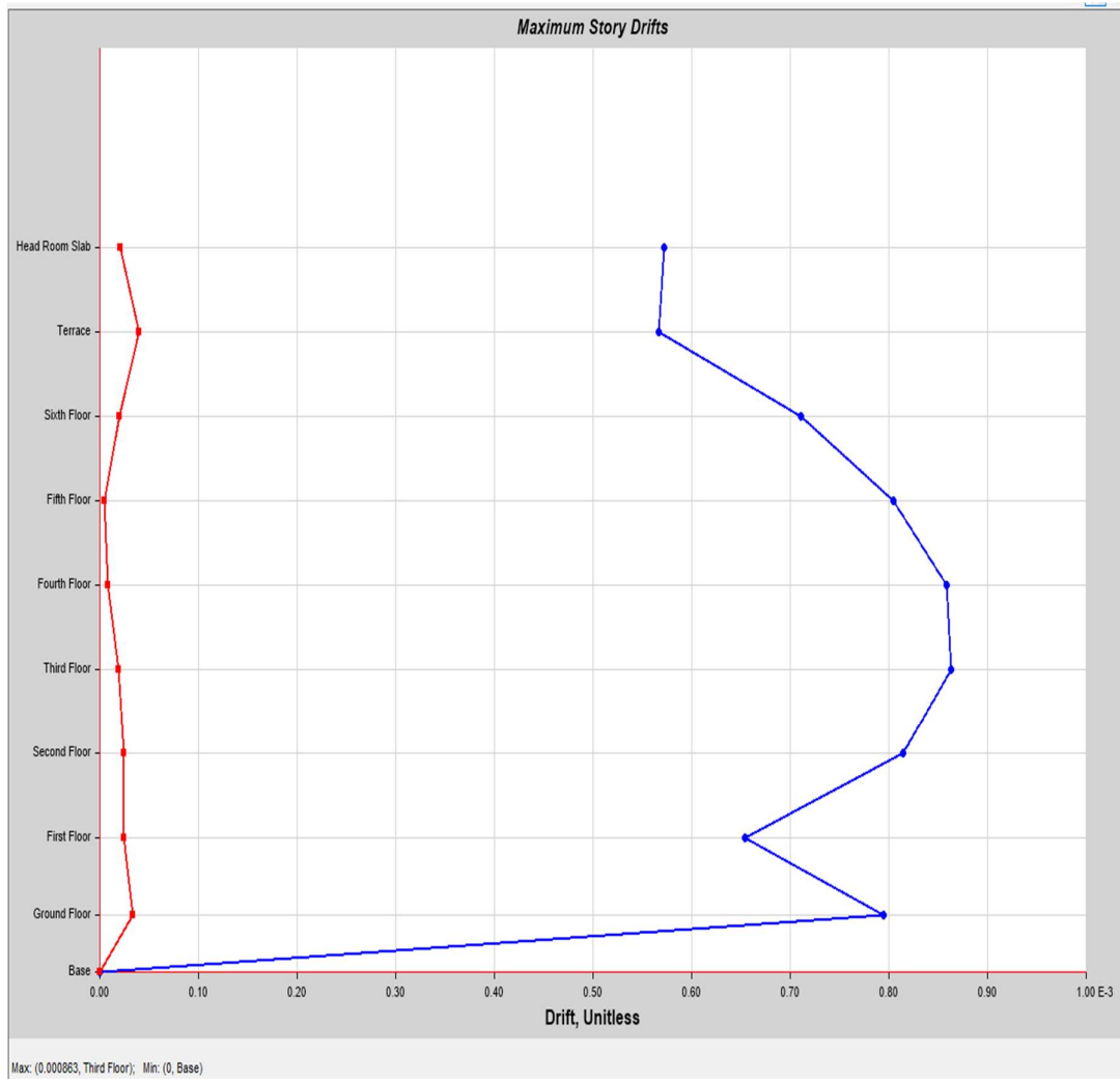
Fig 4.4.2: Maximum storey drift of CASE D.
