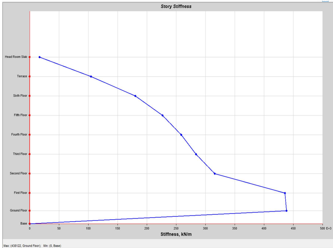
Fig 4.2.3: storey stiffness of CASE B.
