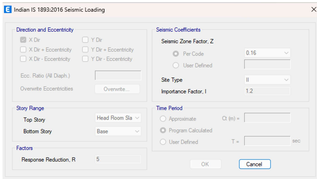
Fig 3.2.2: earthquake loading definition.
