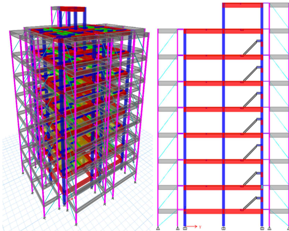
Fig 3.5: 3D view and elevation of Diagonal-braced exoskeleton.
