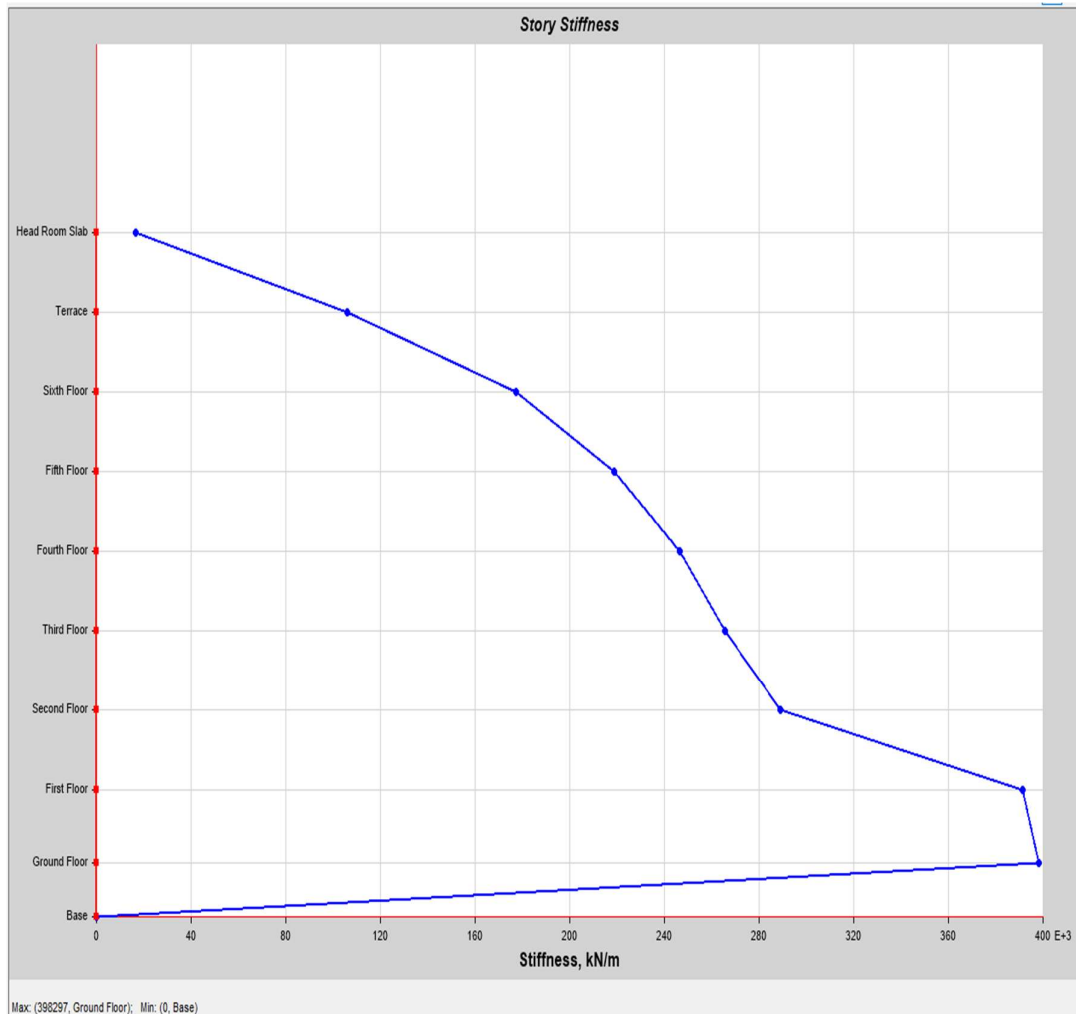
Fig 4.4.3: storey stiffness of CASE D.
