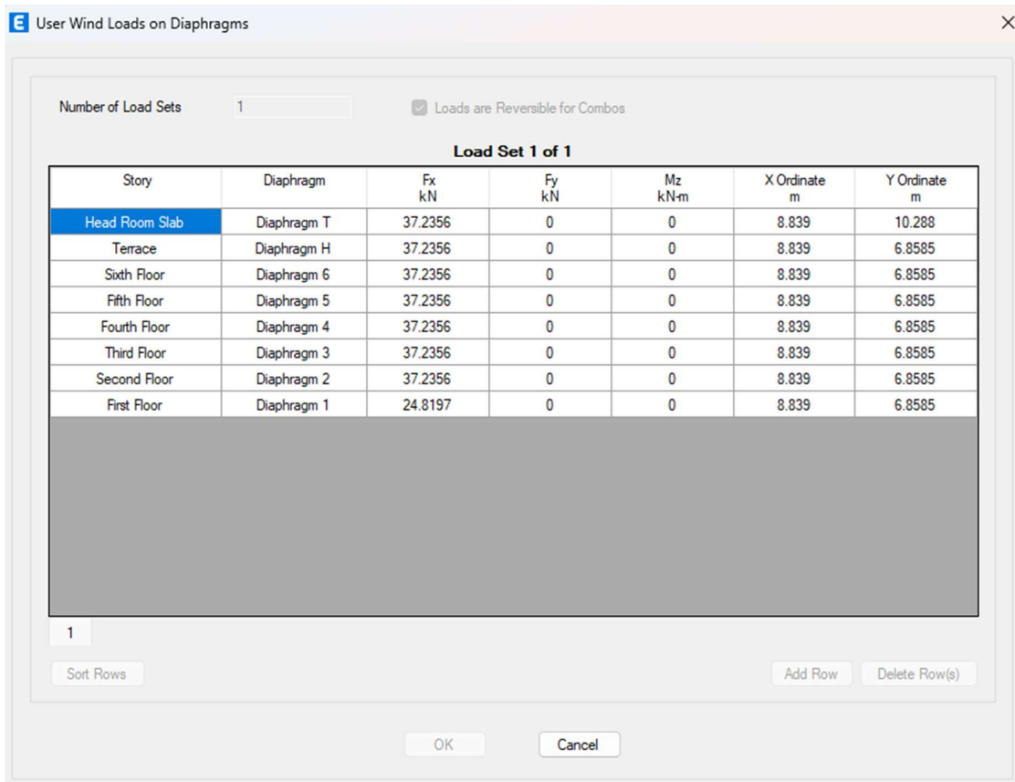
Fig 3.2.2.1: Wind load definition.
