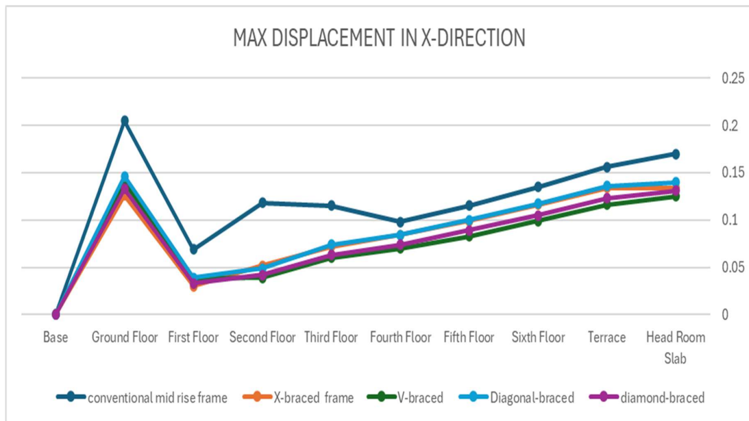
Fig 5.1: Comparative results of story displacement under R S A.
