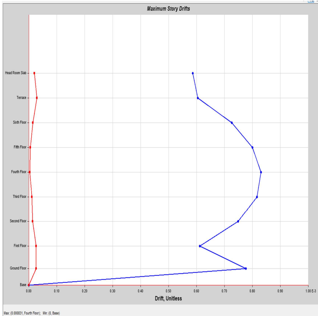
Fig 4.5.2: Maximum storey drift of CASE E.
