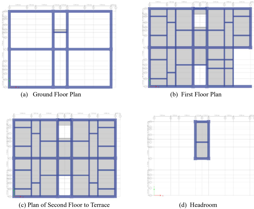
Fig 3.2.1A: Plan view of framing.
