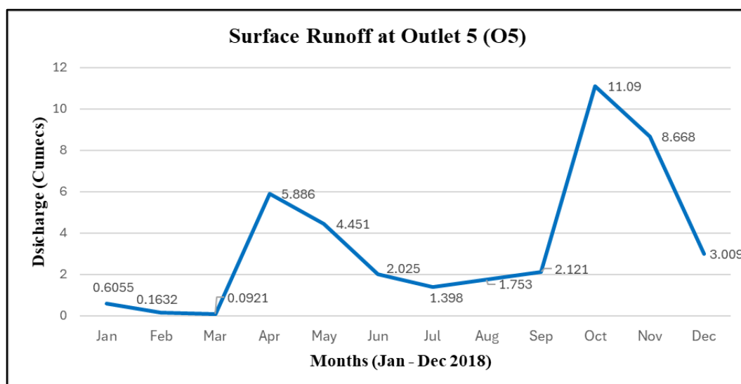
Figure 5.50 : Surface Runoff at Outlet 5 (O5)
