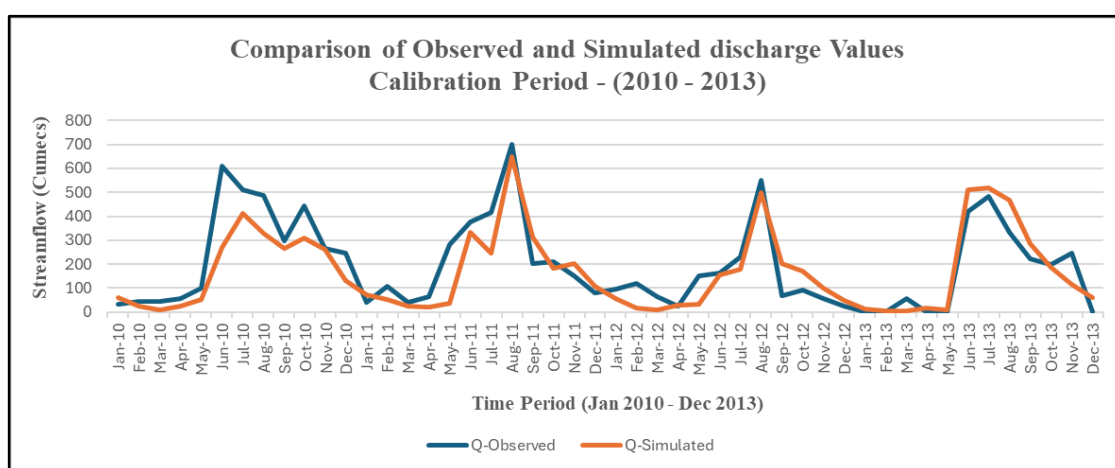
Figure 5.40 : Comparison of Observed and Simulated Discharge values for Calibration
