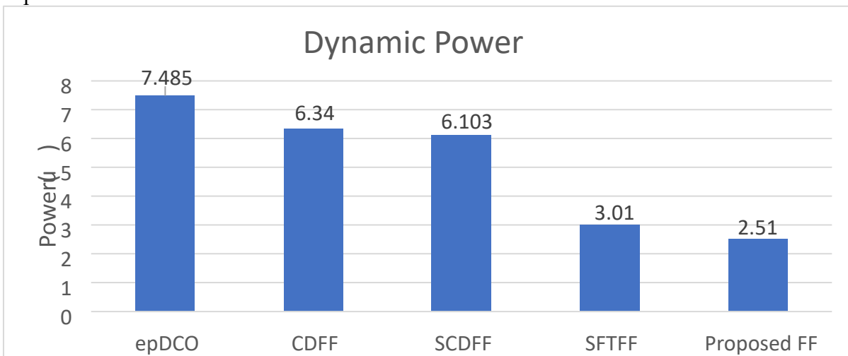
Fig 5.14 Dynamic Power
