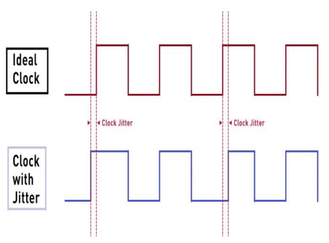
Figure 1.9 Clock Jitter
