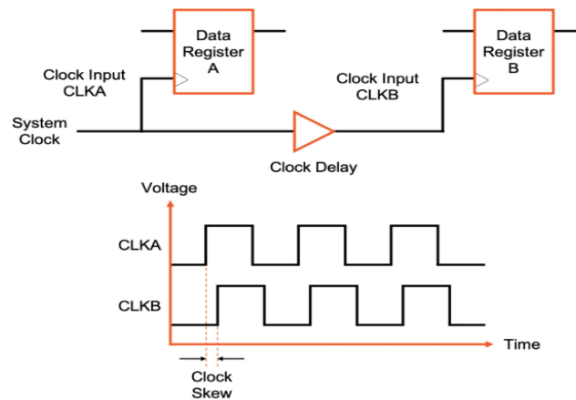
Figure 1.8 Clock Skew
