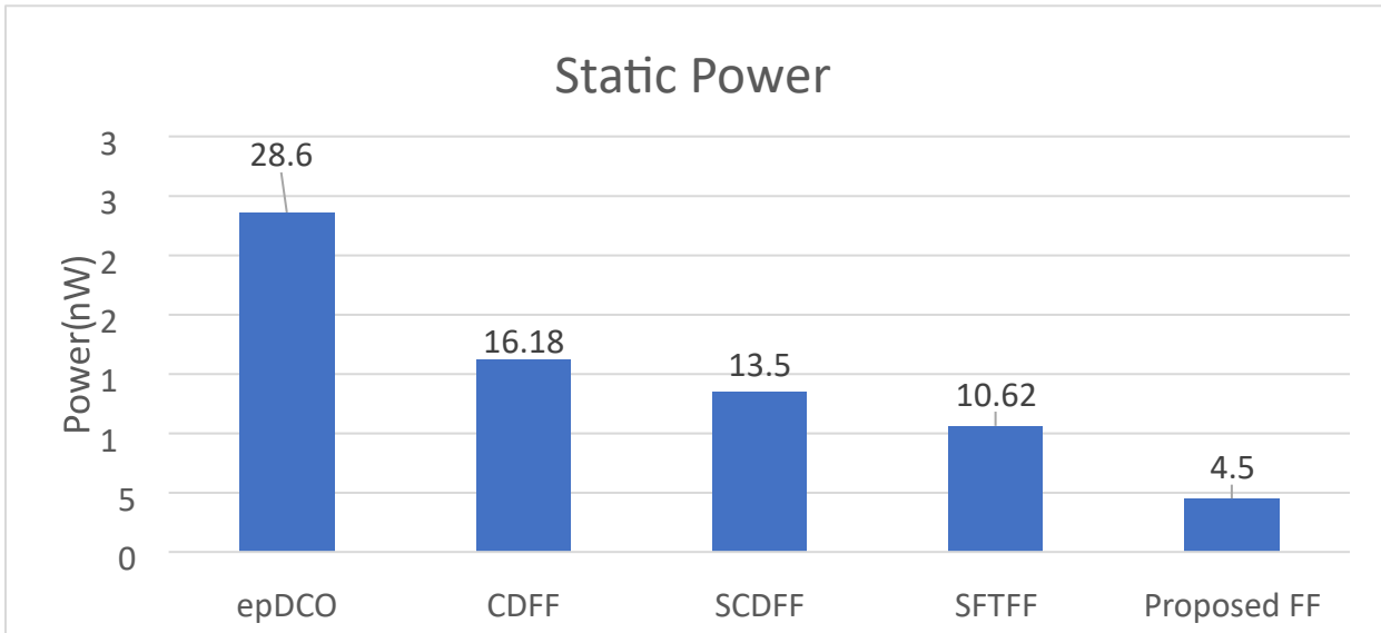
Fig 5.13 Static Power
