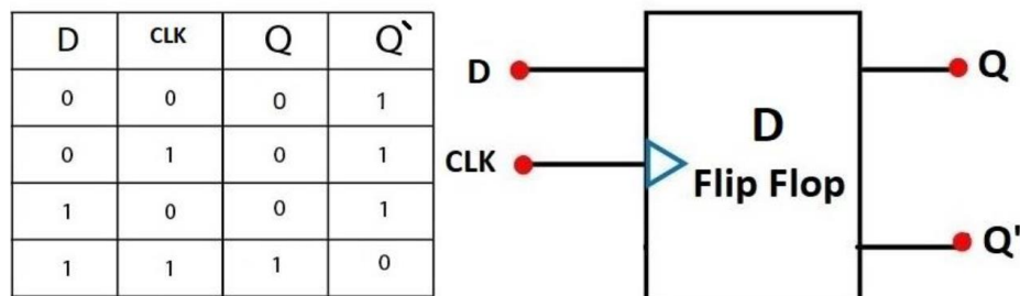
Figure 1.2 D Flipflop
