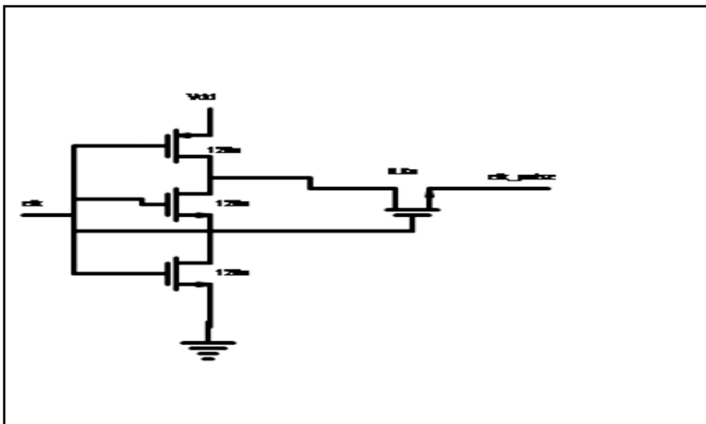
Fig4(a). Pulsed clock generation circuit
