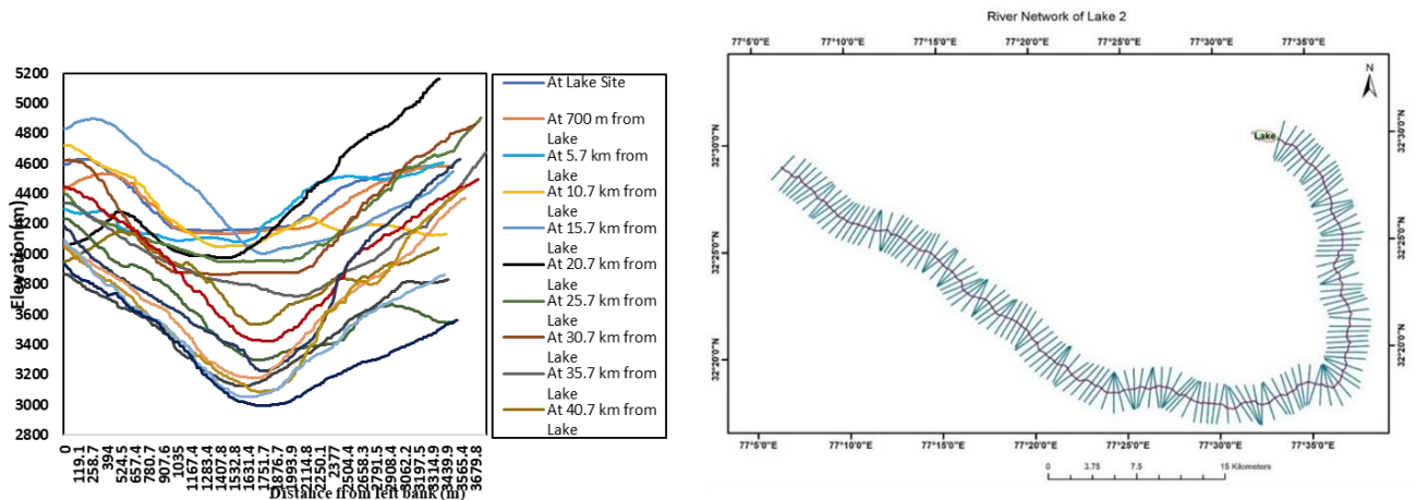
Figure 4.2 Cross Section Layout for Lake 2
