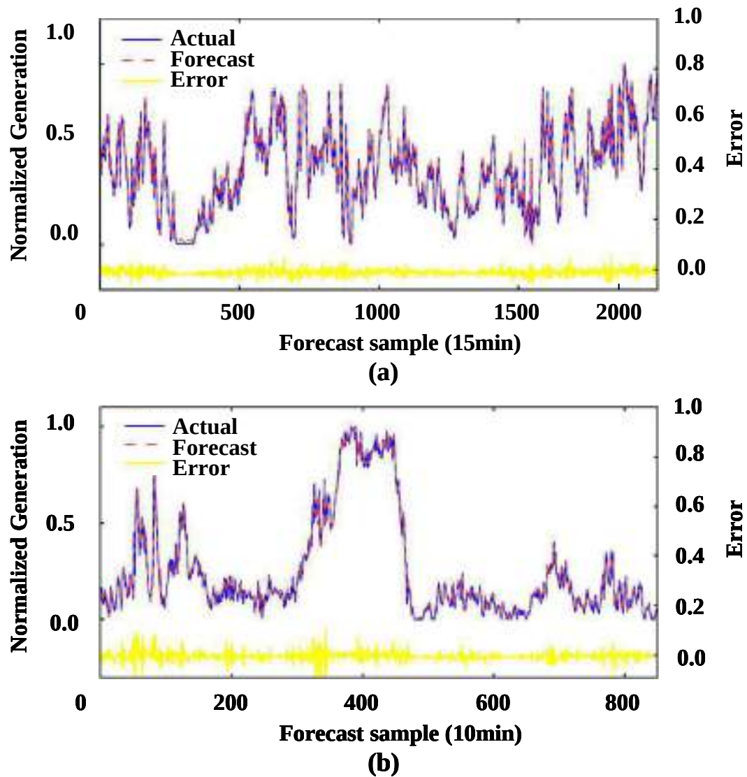
FIGURE 4.6: Wind power generation forecast for (a) Dataset-1 (b) Dataset-2.
