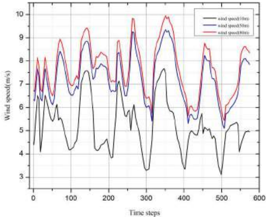
FIGURE 3.1: NWP values of wind speed for Tuticorin wind farm at 10, 50 and 80m .
