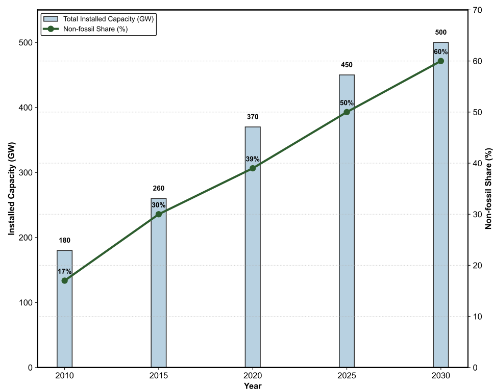
FIGURE 1.3: India's power capacity transition and non-fossil target for 2030.
