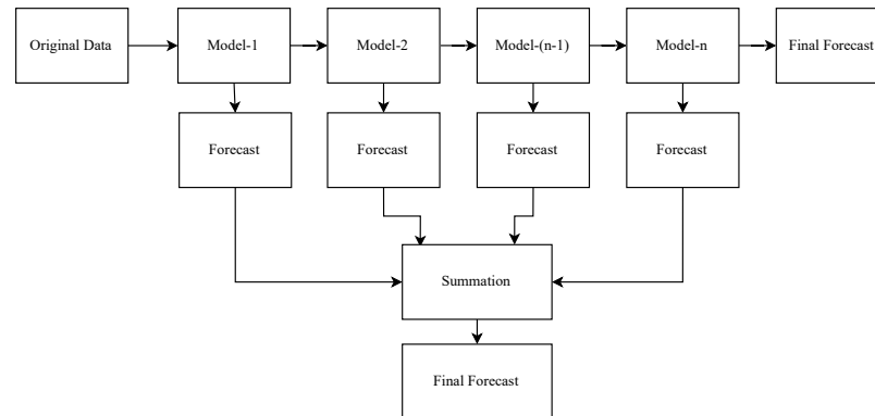
FIGURE 2.12: General architecture of series hybrid model
