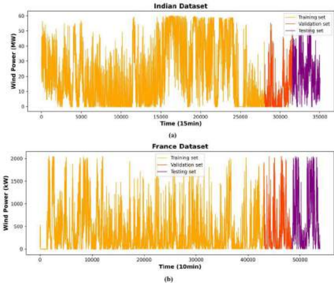
FIGURE 5.6: The wind power data of two datasets: (a) Dataset-1, (b) Dataset-2.
