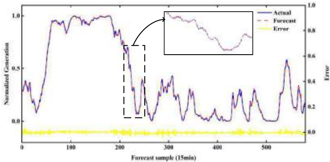
FIGURE 6.6: Wind power deterministic forecast with residuals for Dataset-1.
