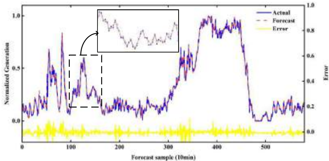
FIGURE 6.7: Wind power deterministic forecast with residuals for Dataset-2.
