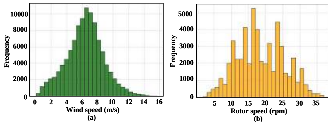
FIGURE 4.8: Distribution of wind speeds for Dataset-1 and rotor speeds for Dataset-2, highlighting differences in variability and frequency distribution between the two locations.
