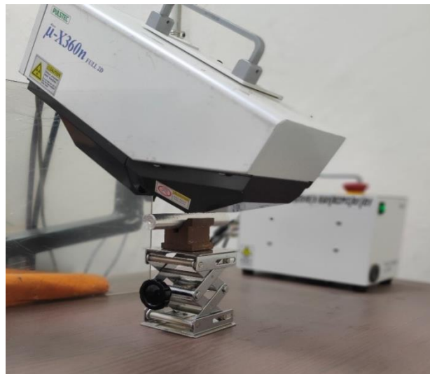
Figure 4.7: X-ray residual stress measuring machine
