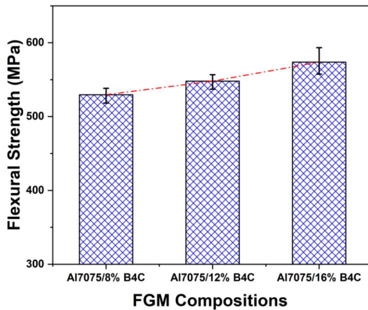
Figure 5.13: Flexural strength of all three compositions of FGM leaf
