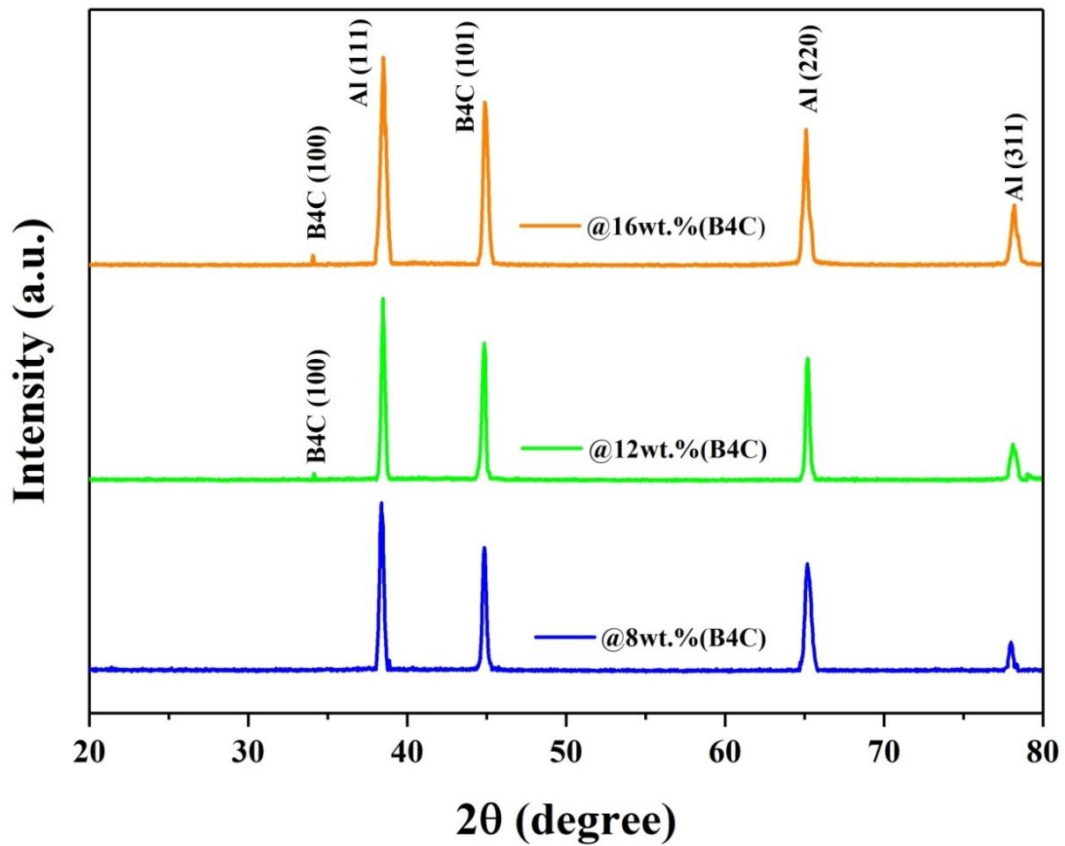
Figure 4.6: Cascade model of XRD pattern of compositions used in functionally graded materials plate
