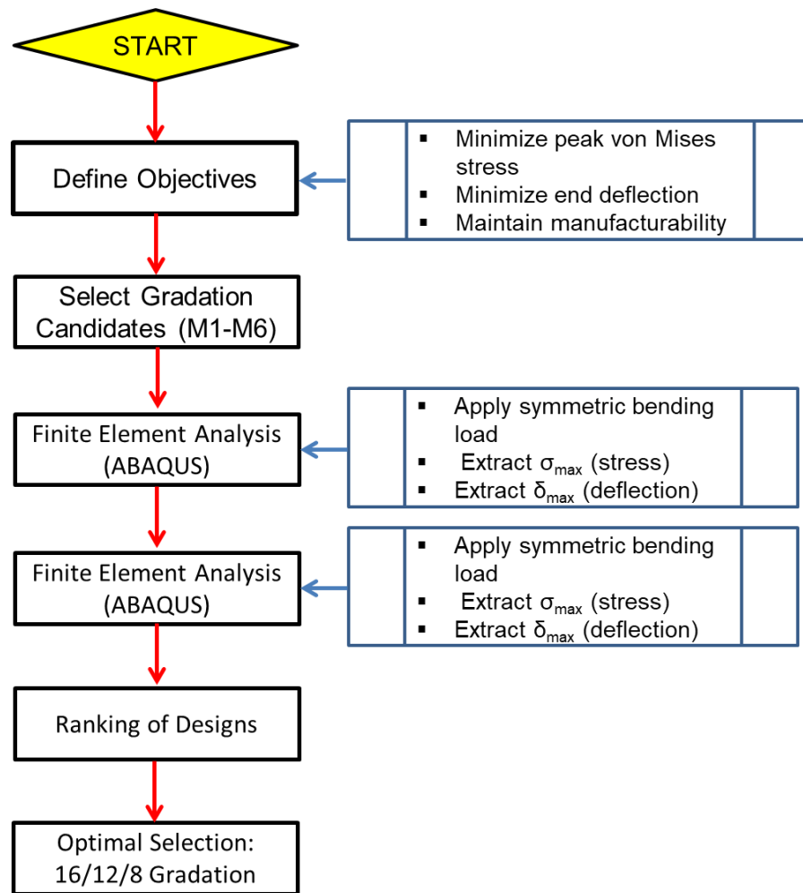
Figure 6.8: Flowchart of the optimization methodology for reinforcement gradient selection in the FGM Al7075–B4C leaf spring.
