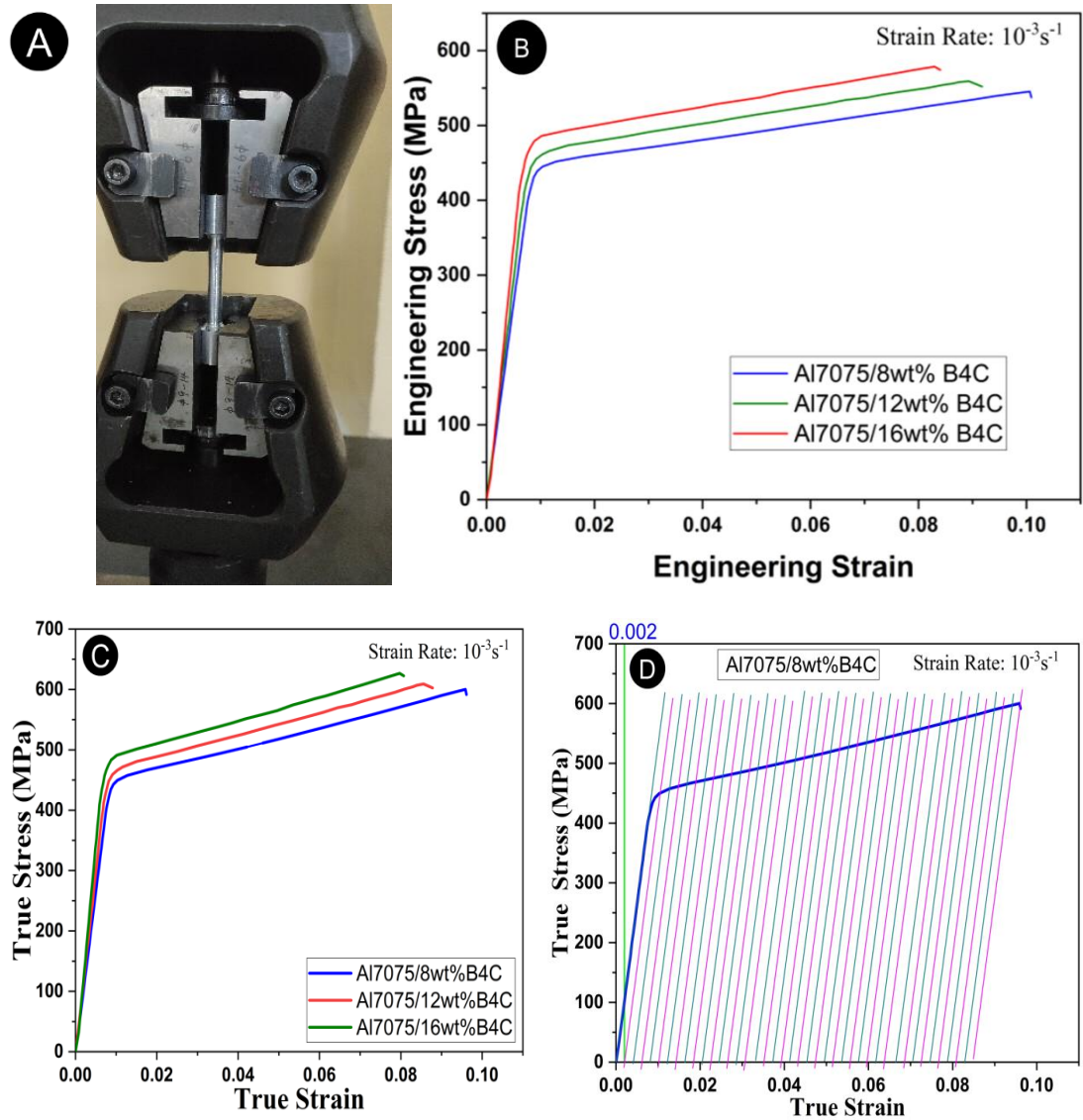
Figure 5.2. (A) Tensile Test setup (B) Engineering Stress vs. Engineering Strain (C) True stress vs. True strain. (D) Data reduction from true stress vs. True strain to True Strain
