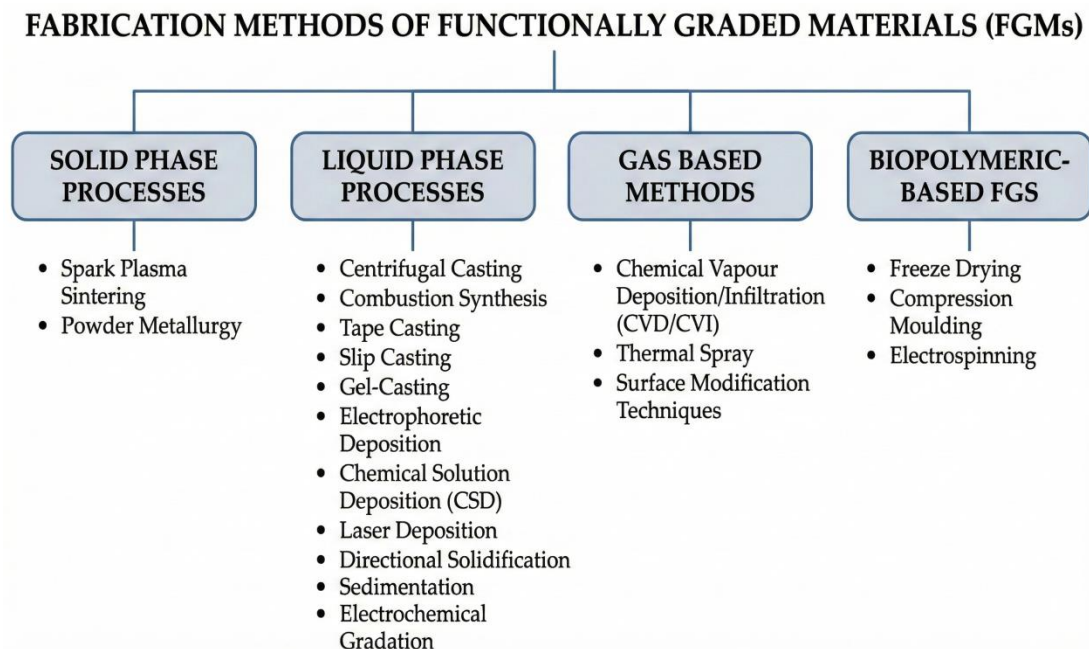
Figure 2.1: Classification for fabrication methods of FGMs
