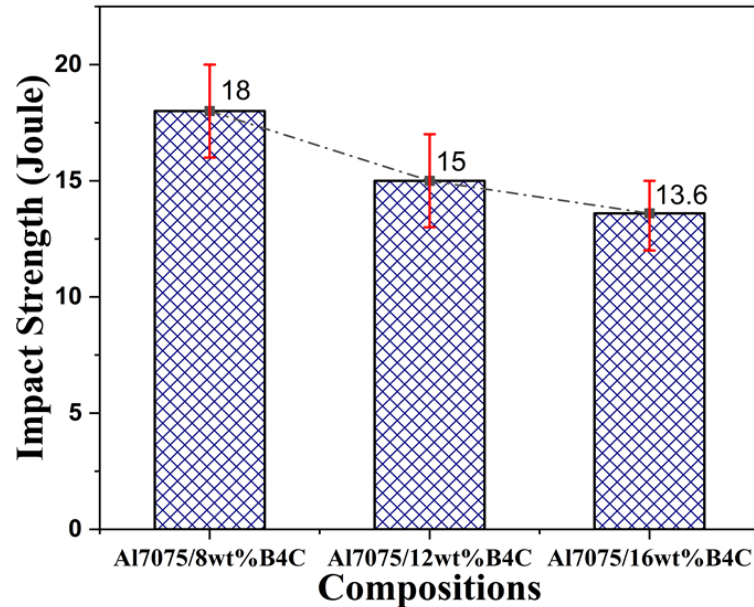
Figure 5.14: Impact strength of Al7075–B 4 C composites with different reinforcement levels.
