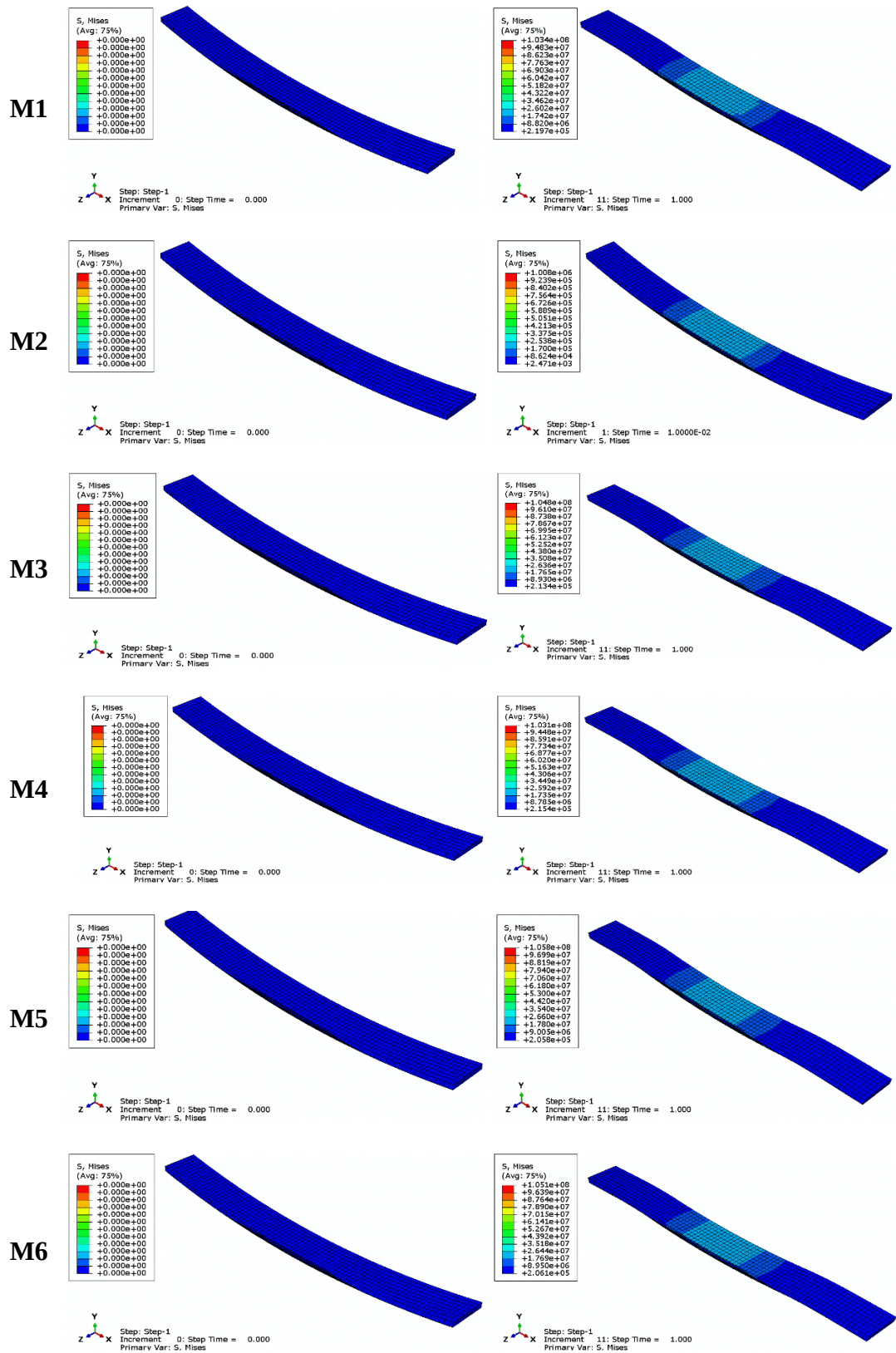
Figure 6.4: Von Mises stress contours for models M1–M6.
