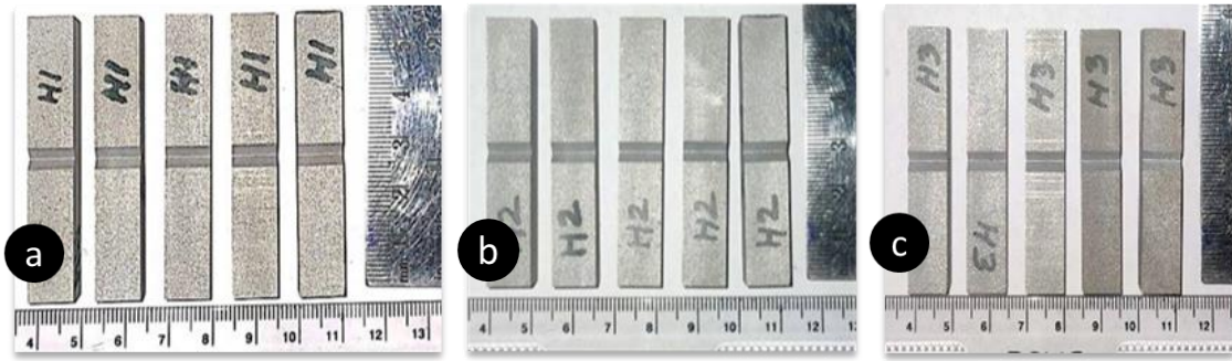
Figure 5.6 (a–c): Standard Charpy V-notch specimens for 8 wt %, 12 wt %, and 16 wt % B 4 C composites before testing.
