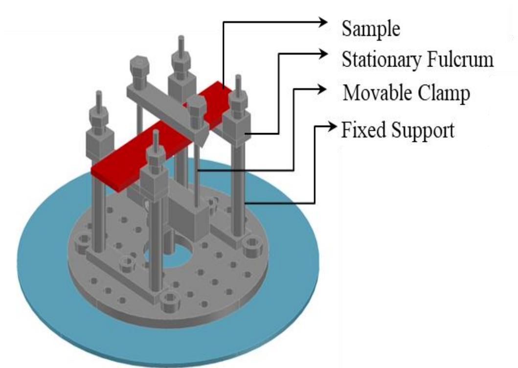
Figure 5.8: DMA three-point bend test fixture
