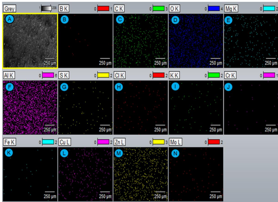
Figure 4.5: FESEM image with EDS elemental mapping of Al7075/16 wt.% B 4 C composite showing spatial distribution of Al, B, C and minor elements.
