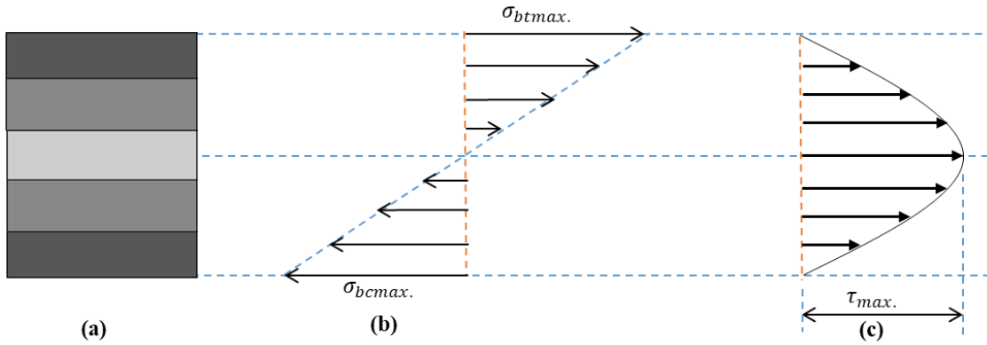
Figure 3.3: (a) cross-sectional view of fabricated leaf (b) Theoretical Distribution of bending Stresses (c) Shear stress distribution
