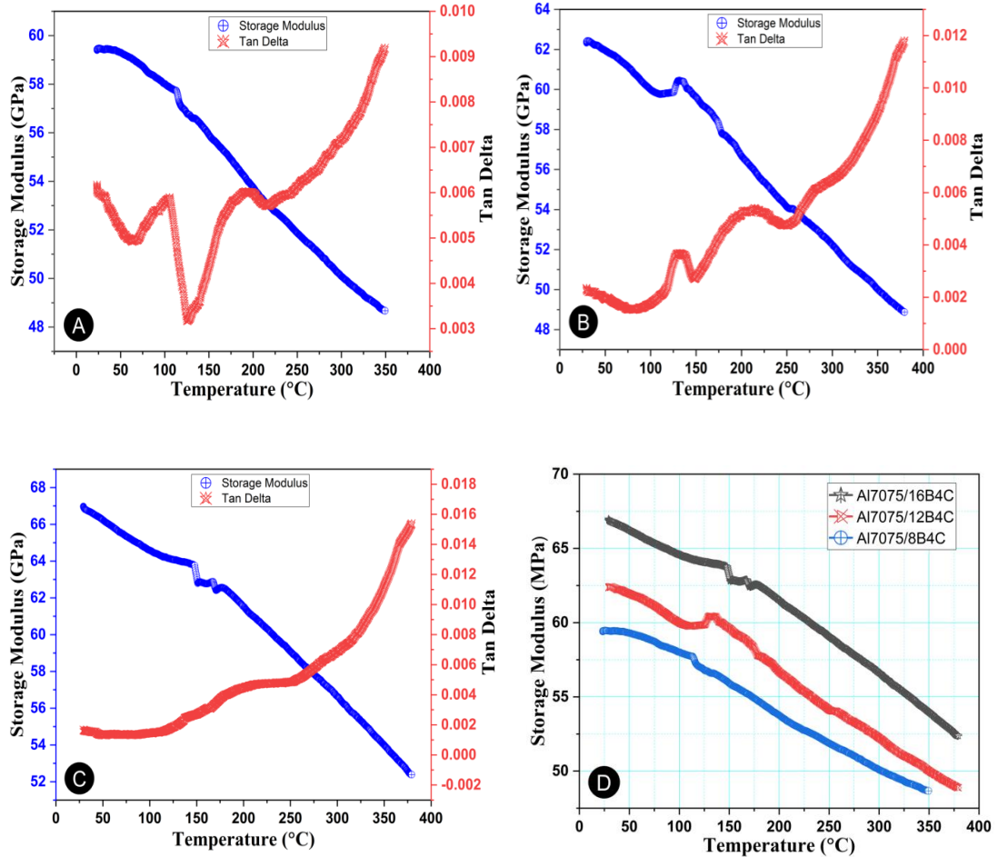
Figure 5.15: Storage modulus ( E' ) and tan delta ( \tan \delta ) as functions of temperature (A) Al7075/8B 4 C composite (B) Al7075/12B 4 C composite (C) Al7075/16B 4 C composite (D) Storage modulus as function of temperature of all three composites
