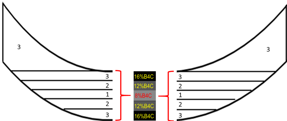
Figure 3.4: Layer-wise distribution of reinforcement in the Al 7075/B 4 C FGM leaf-spring plate.
