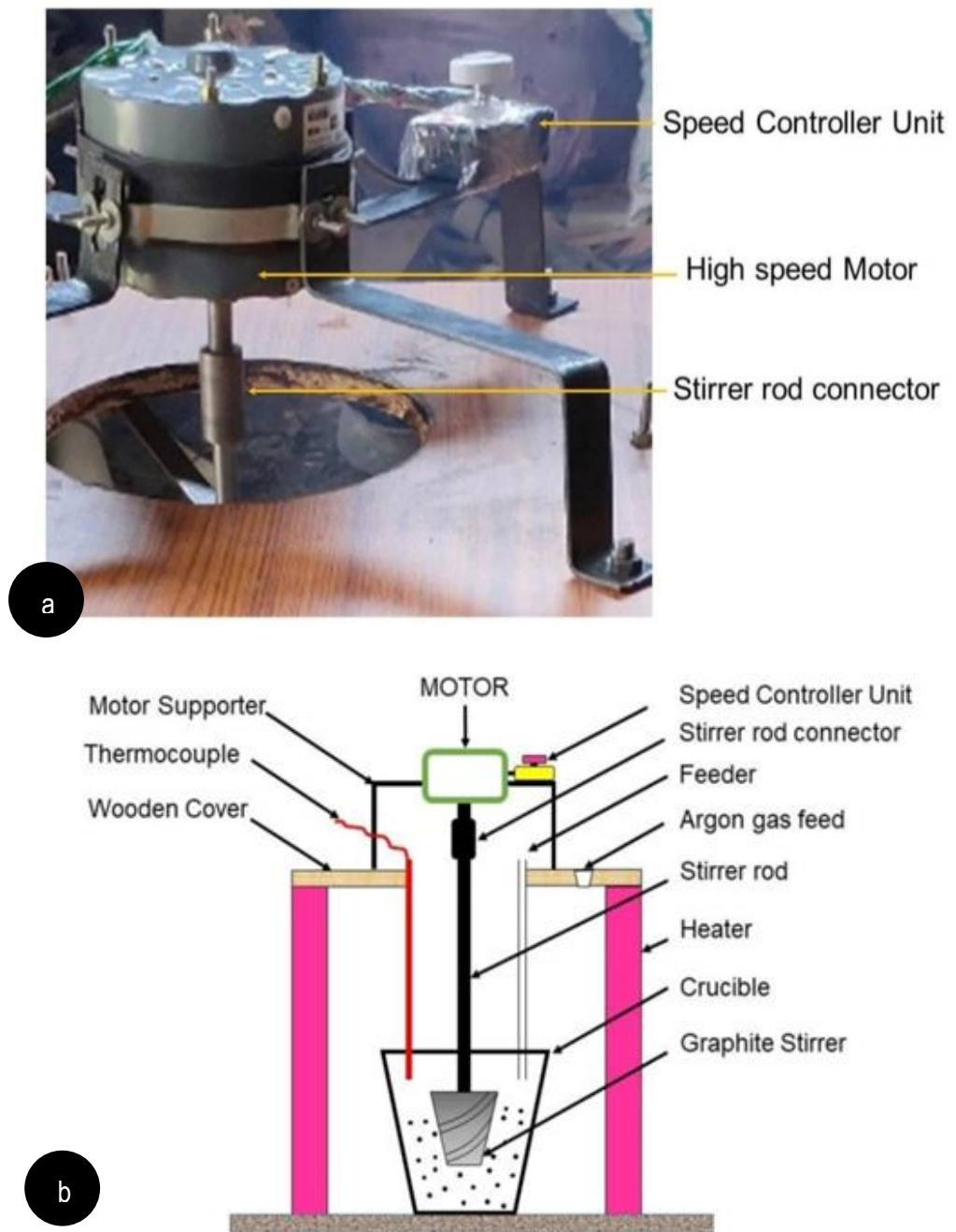
Figure 3.7: (a)Stirrer with a speed controller (b) Schemetic of Stir-Casting Setup
