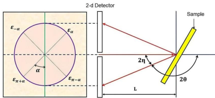
Figure 4.8: Strain measurement in debye-scherrer ring in cos \alpha method
