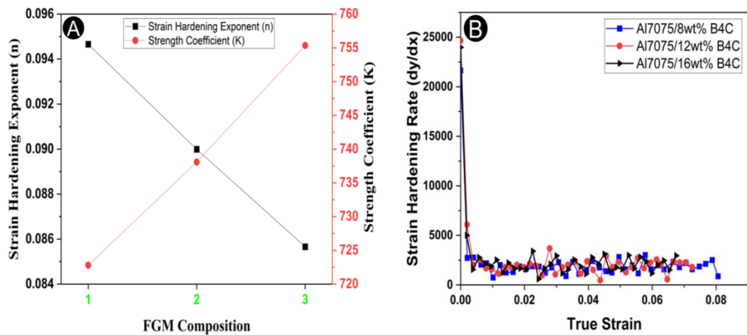
Figure 5.11: (A) Strain hardening exponent vs. Strain coefficient vs. composite compositions (B) Strain hardening rate vs. True plastic strain.
