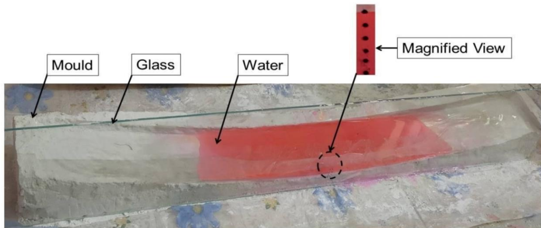
Figure 3.5: Experimental Setup for evaluation of the material required in each layer
