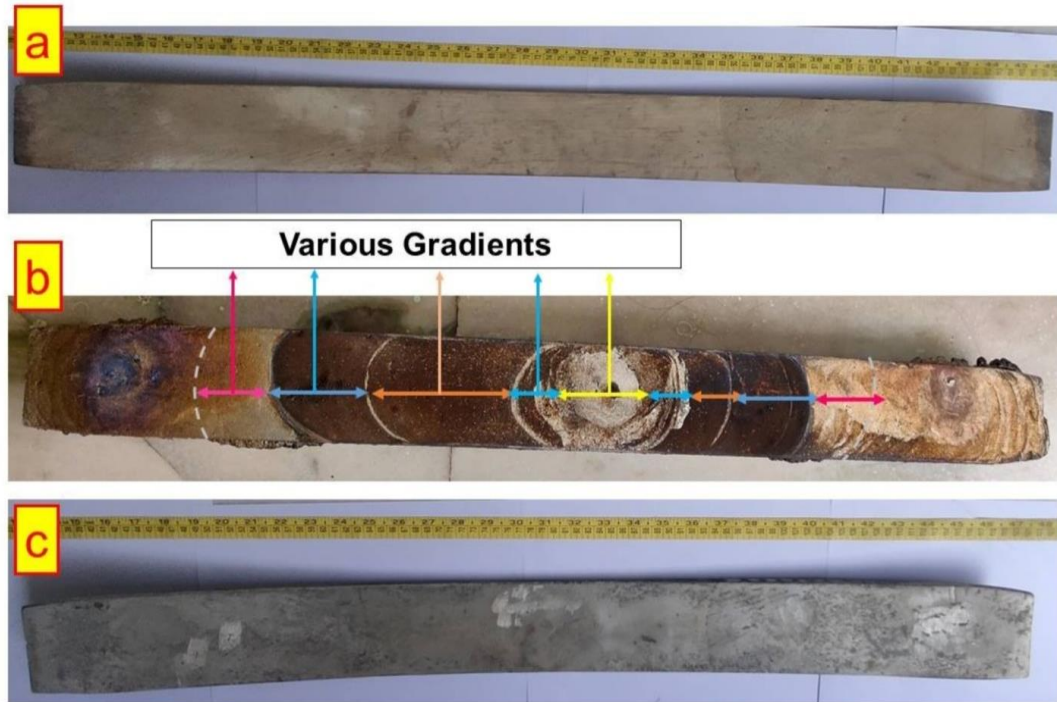
Figure 3.8: (a) Pattern of spring plate (b) Stir casted functionally graded materials leaf (c) Finished functionally graded materials leaf spring plate
