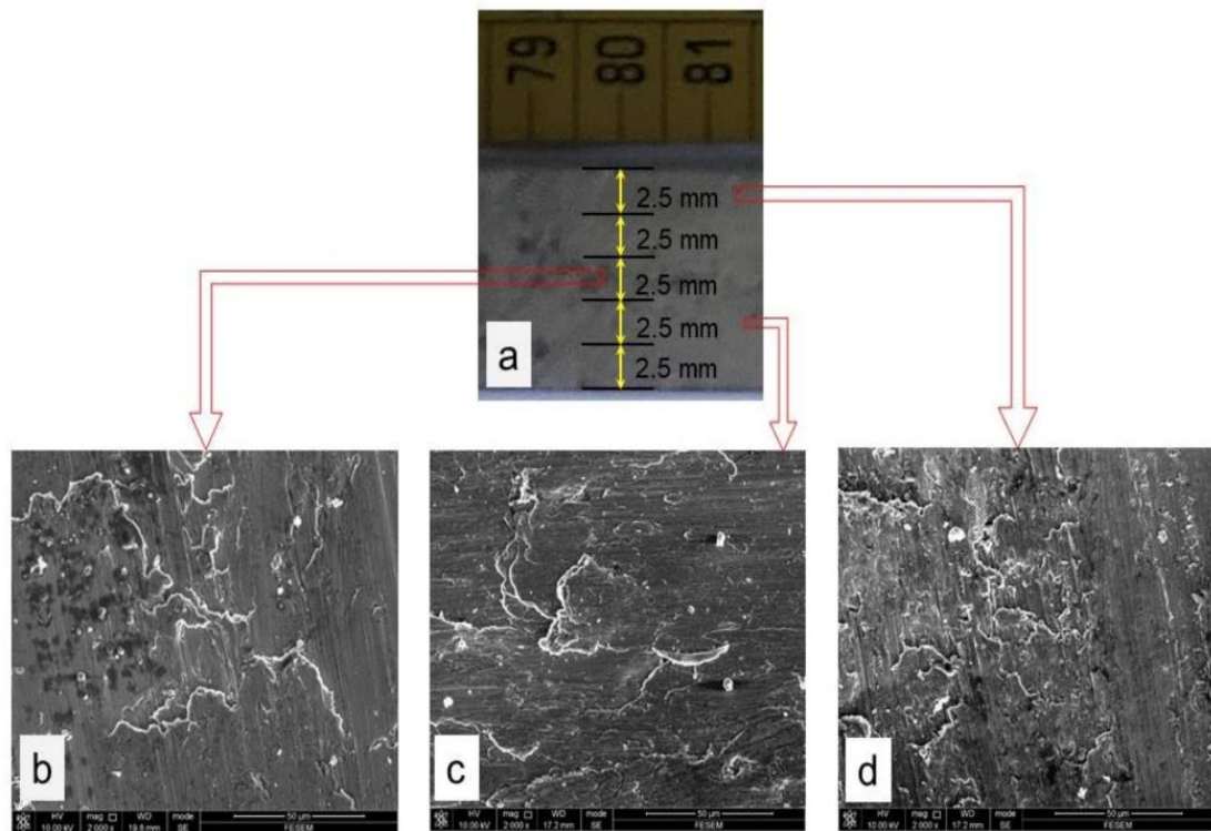
Figure 4.2: (a) sectioned FGM plate of 5 graded layers; (b) FESEM micrograph of 8 wt.% B 4 C, (c) and (d) FESEM micrographs of 12 and 16 wt.% B 4 C zones after T6 heat treatment.
