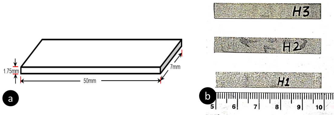
Figure 5.7: (a) Dimensions of specimens (b) DMA specimens of all three compositions
