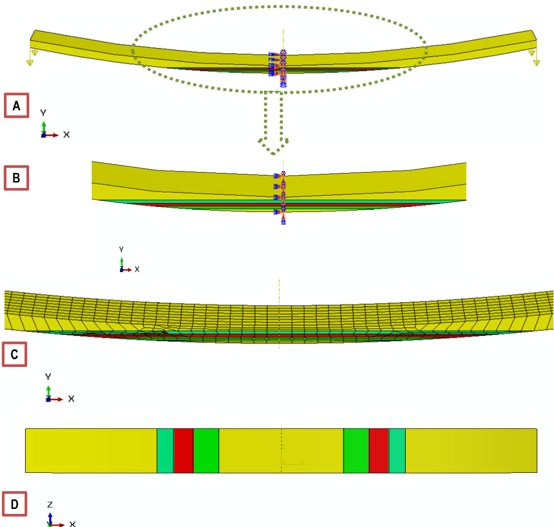
Figure 6.3: FGM plate FE model configuration. (A) Applied loading at free ends, (B) Fully fixed central region, (C) C3D8R meshing strategy, (D) Bottom view of 5-layer gradation.
