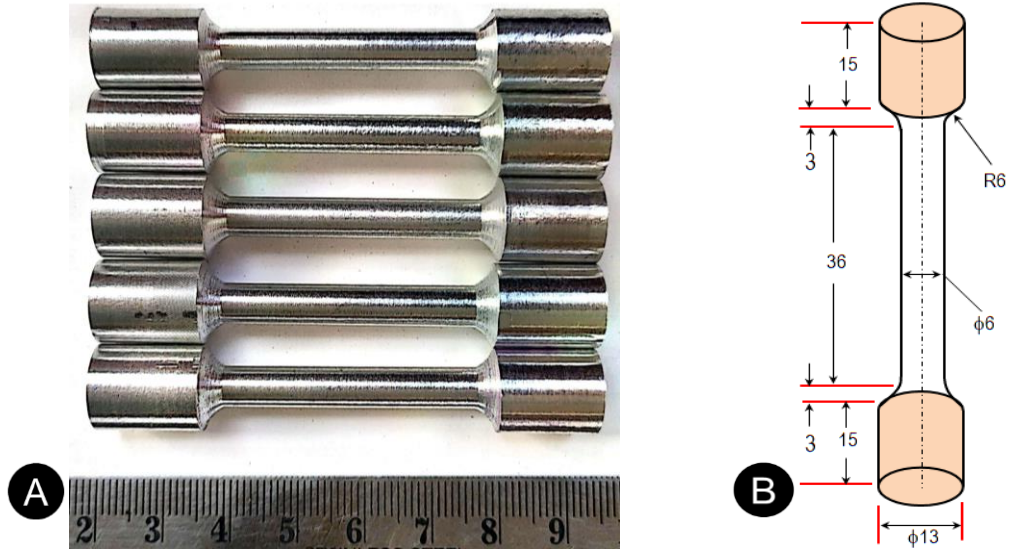
Figure 5.1: (A) Tensile test specimens (B) Dimensions of tensile test specimen (in mm)
