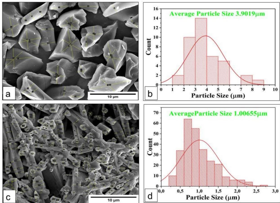
Figure 3.2: (a) FESEM of B 4 C particles (b) Crystallite size distribution of B 4 C particles (c) FESEM of K 2 TiF 6 particles (b) Crystallite size distribution of K 2 TiF 6 particles
