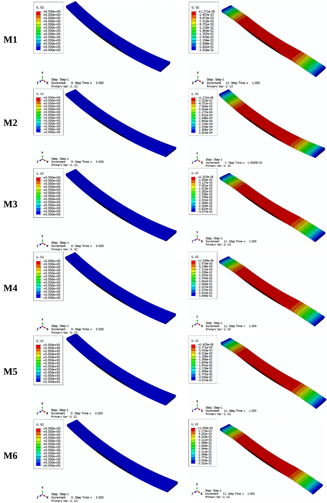
Figure 6.5: Vertical deformation for FGM models M1-M6.
