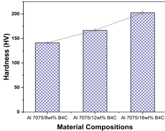
Figure 5.12: Variation of hardness of Al 7075–B 4 C composites with reinforcement percentage.
