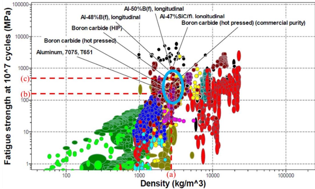
Figure 3.1: Fatigue strength vs Density chart generated using CES EduPack 2019 software
