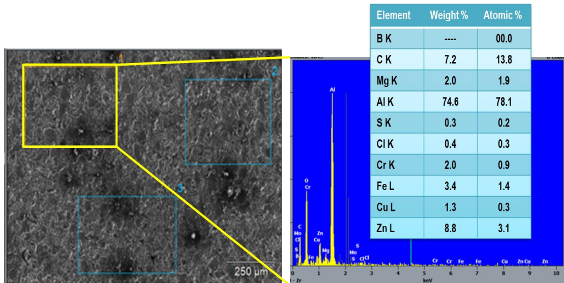
Figure 4.4: FESEM and EDS of Al7075/12 wt. % \text{B}_4\text{C} composite confirming successful reinforcement incorporation.
