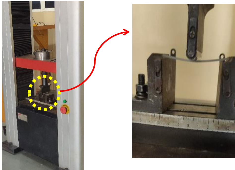
Figures 5.4: UTM setup and loading configuration
