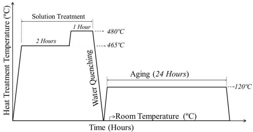
Figure 3.9: The detailed schematic of the T6 heat treatment cycle
