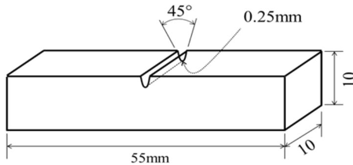
Figure 5.5: Schematic of the Charpy V-notch specimen
