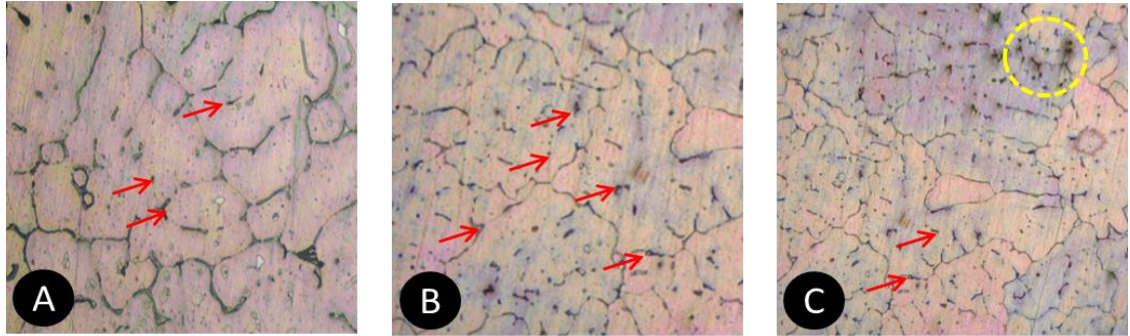
Figure 4.1: The microstructure of samples (A) Al7075-T6 /8wt. % B 4 C (B) Al7075-T6 /12 wt. % B 4 C (C) Al7075-T6 /16 wt. % B 4 C
