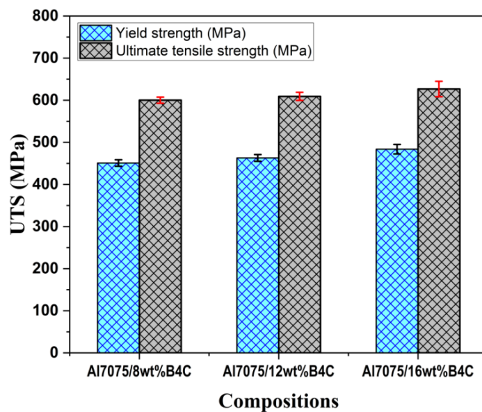
Figure 5.9: Yield and UTS values of all three composites
