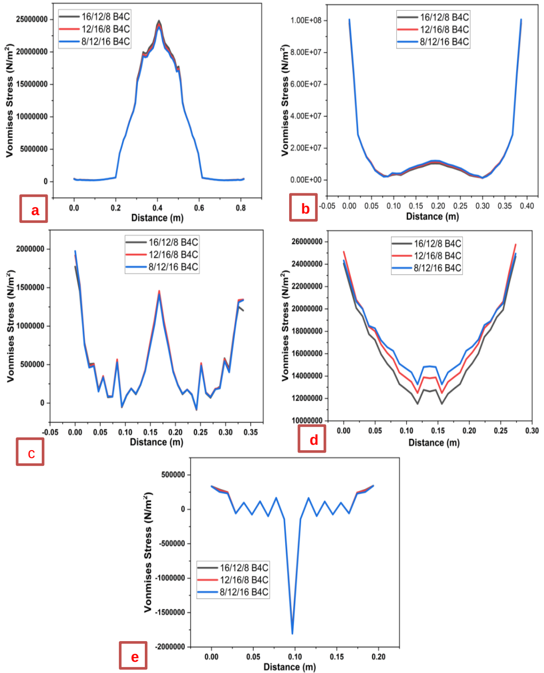
Figure 6.6: Layer-wise von Mises stress distribution (L1–L5) of the FGM leaf spring for 16/12/8, 12/16/8 and 8/12/16 wt.% B 4 C gradations under symmetric bending.
