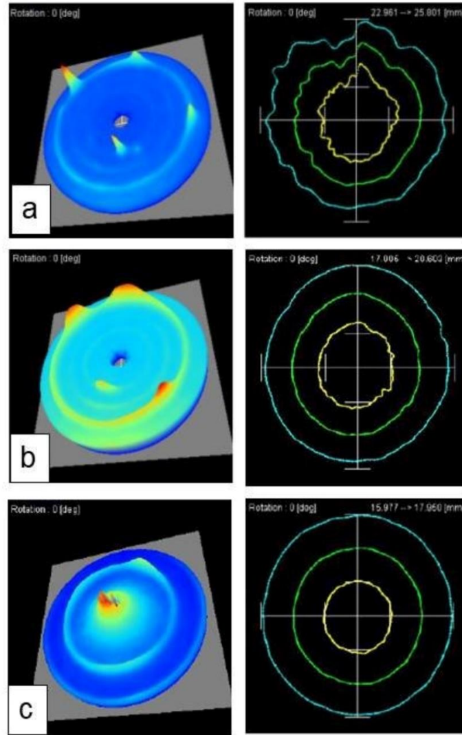
Figure 4.9: 3-D debye-scherrer ring and distortion for (a) Al 7075 8wt% B4C, (b) Al 7075 12wt% B4C, and (c) Al 7075 16wt% B4C
