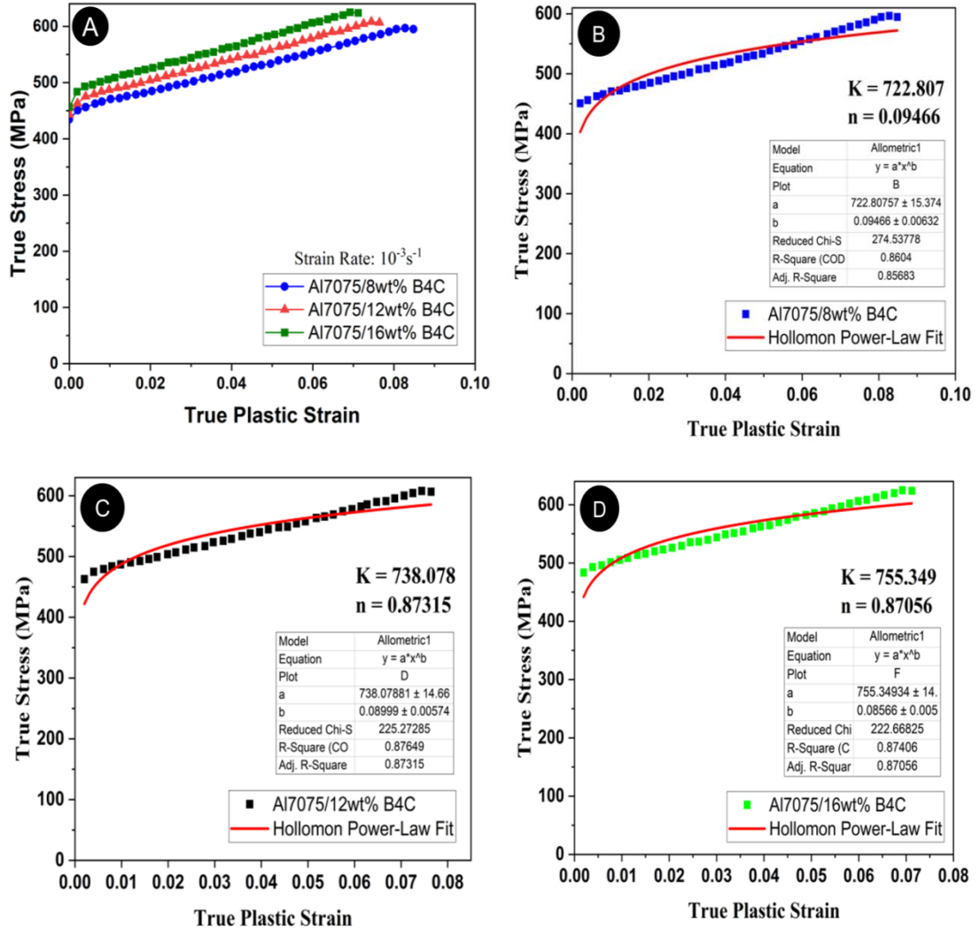
Figure 5.10: (A) True stress–true plastic strain curve; (B–D) Hollomon power law fitting for Al7075/8 wt.%, 12 wt.%, and 16 wt% B 4 C composites, respectively.
