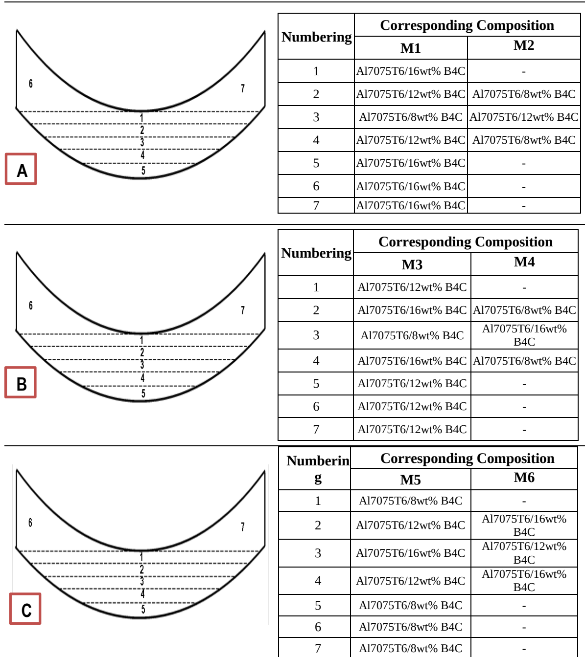
Figure 6.2: Central gradation schemes of the composite leaf spring.(A) 16-based arrangement; (B) 12-based arrangement; (C) 8-based arrangement.
