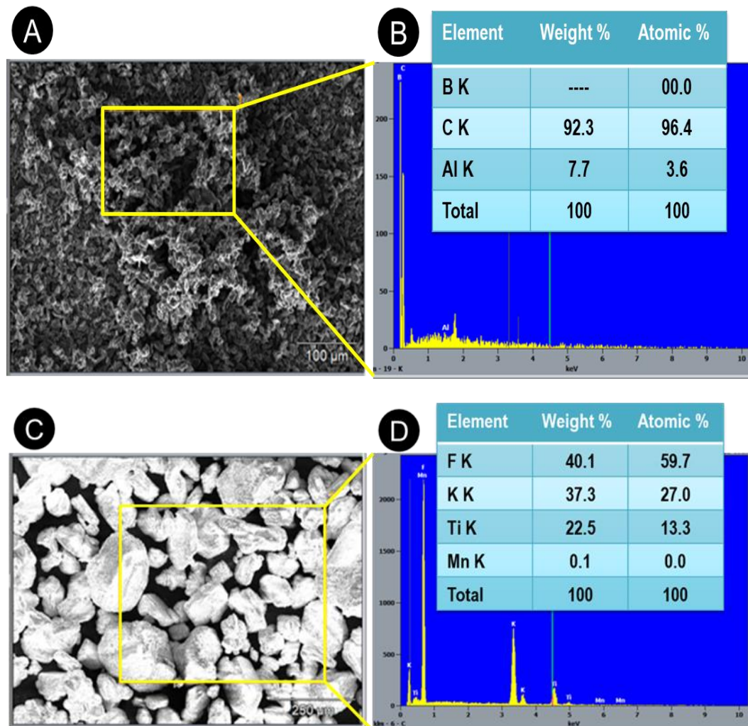
Figure 4.3: FESEM and EDS analysis of (a–b) B_4C powder, and (c–d) K_2TiF_6 powder.
