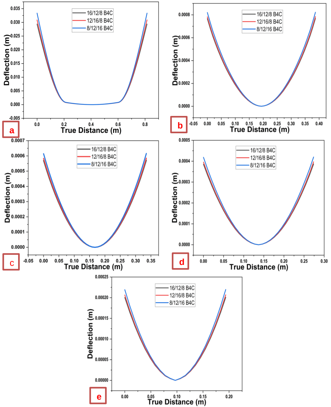
Figure 6.7: Layer-wise vertical deflection profiles (L1–L5) of the FGM leaf spring for 16/12/8, 12/16/8 and 8/12/16 wt.% B 4 C gradations under symmetric bending.
