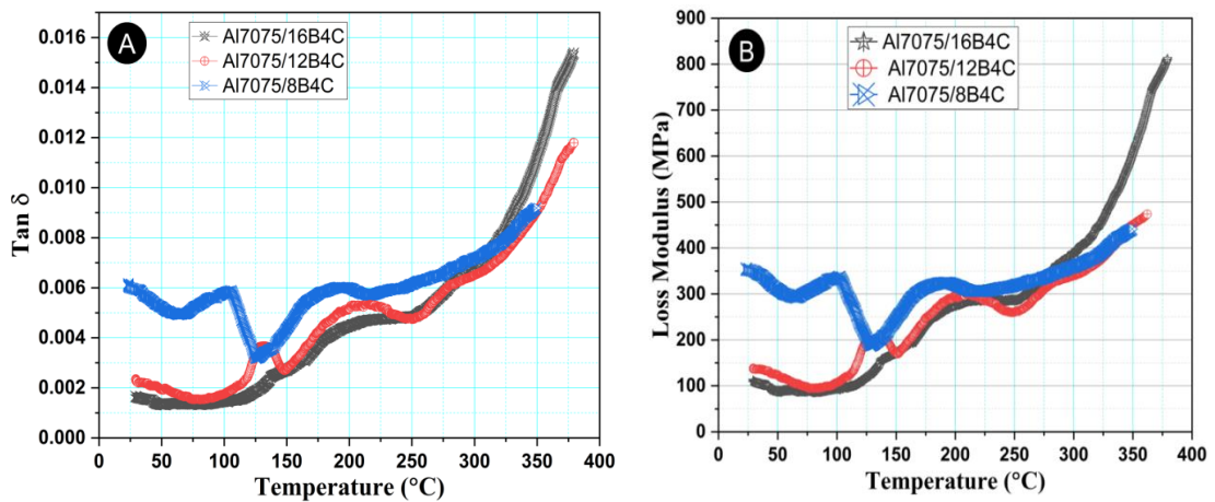
Figure 5.16: (A) Tan delta as function of temperature (B) Loss modulus as function of temperature
