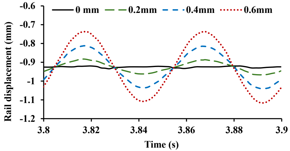
Figure 6.4 Rail displacement at contact point of first wheel when v = 160 km/h, \eta_x = 0 mm, 0.2mm, 0.4mm, 0.6 mm at \omega = 1.5
