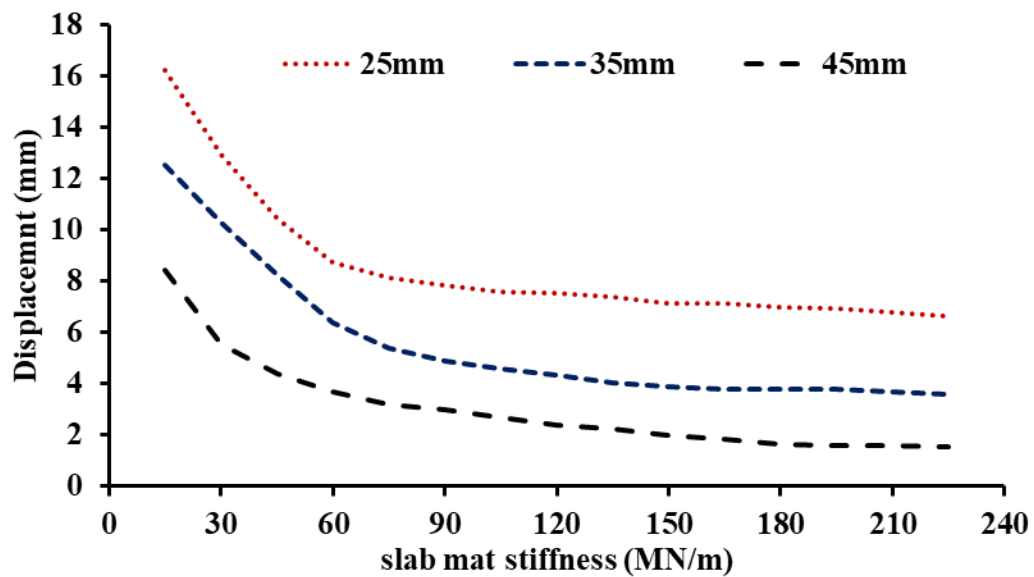
Figure 5.8 Effect of the slab mat thickness on rail displacement
