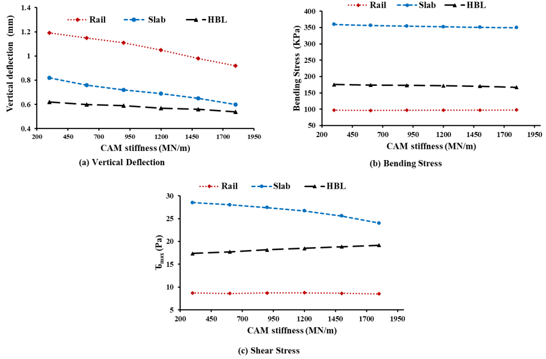
Figure 4.4 Effect of CAM stiffness on both vertical deflection and stress (a)vertical deflection (b)Bending stress (c) Shear stress
