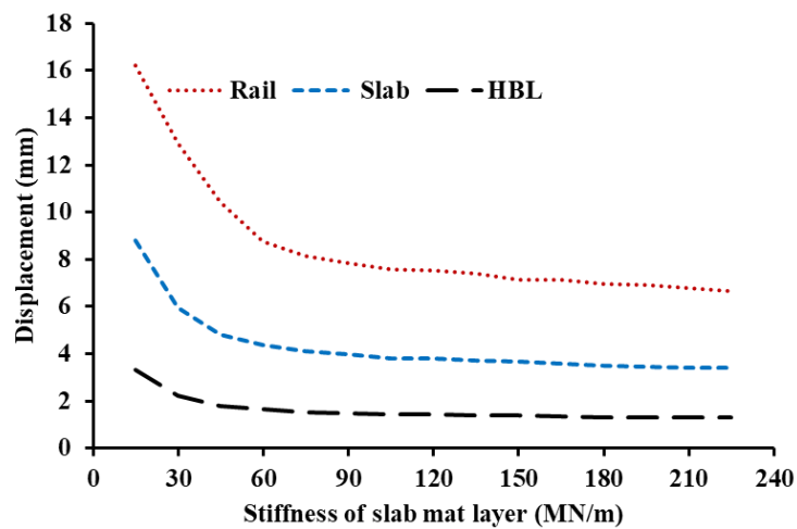
Figure 5.5 Effect of varying the slab mat stiffness on the displacement
