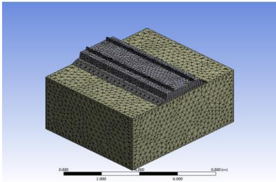
Figure 3.10 Tetrahedral medium meshing of the 3D model
