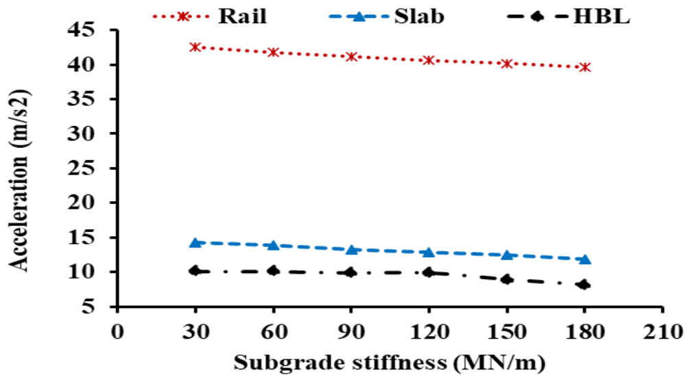
Figure 6.19 Influence of Subgrade stiffness on acceleration of track components
