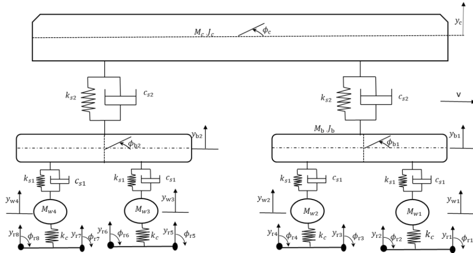
Figure.3.16 Symmetrical vehicle-track interaction
