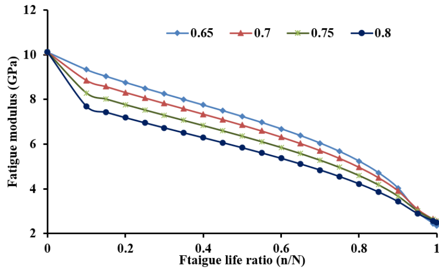
Figure 7.7 The fatigue modulus of CAM specimens is presented at various stress levels
