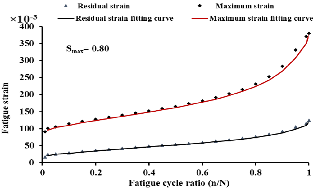
Figure 7.5 Fatigue strain in CAM under applied stress (0.80)
