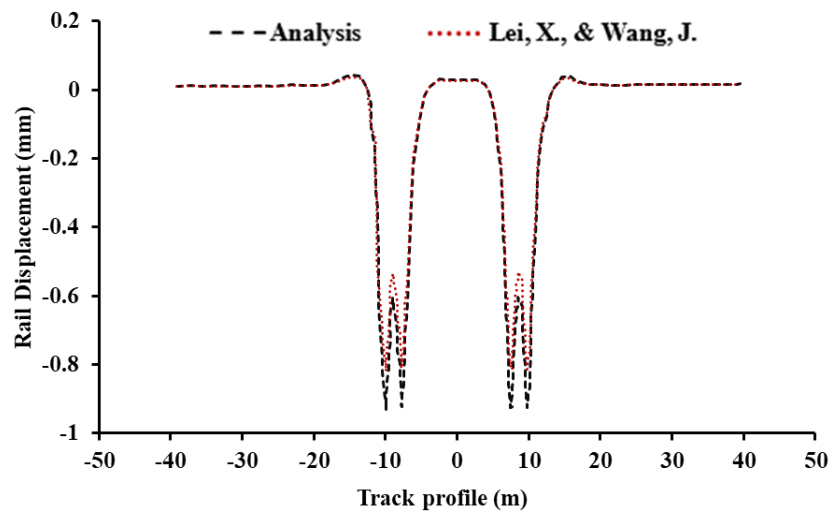
Figure 6.1 Rail displacement profile
