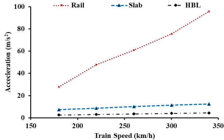
Figure 6.13 Acceleration of track components at varying train speed
