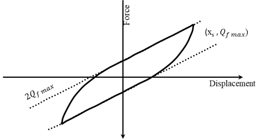
Figure. 3.15 Mechanical characteristics of nonlinear frictional rail pad model
