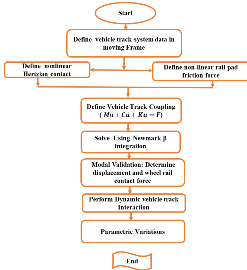
Figure 3.20 Flow chart of methodology for dynamic vehicle track interaction
