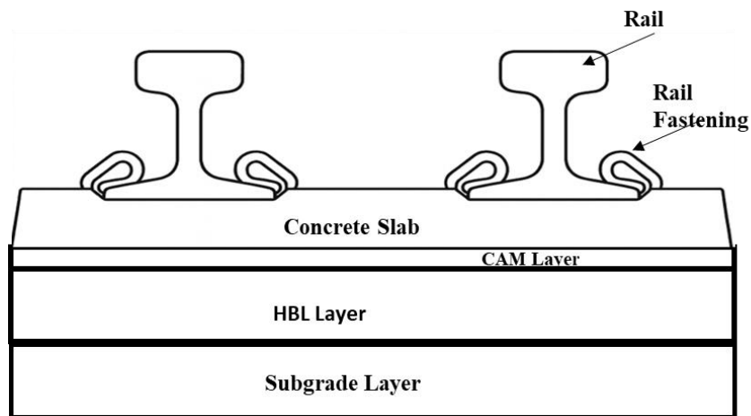
Figure 1.2 Slab track structure
