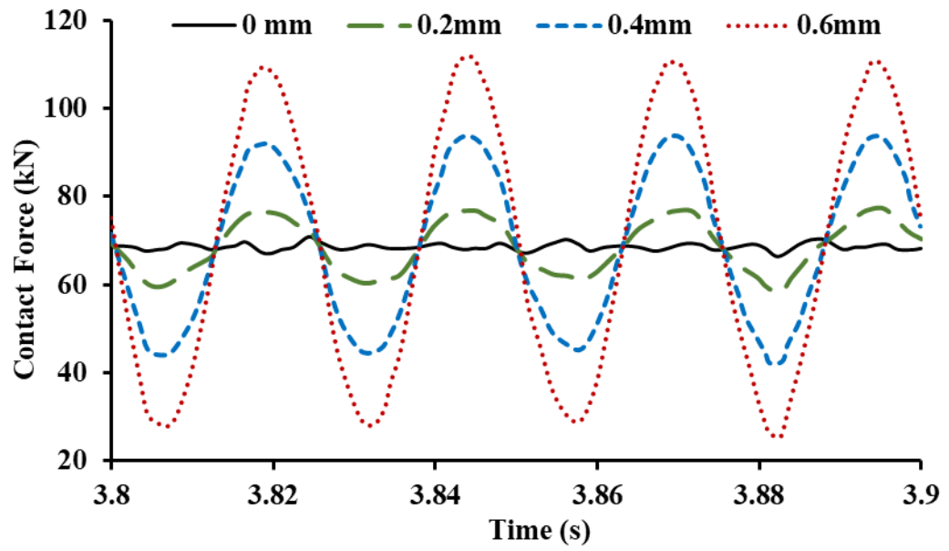
Figure 6.9 Wheel rail contact force at contact point of first wheel when v = 160 km/h, \eta_x = 0 mm, 0.2 mm, 0.4 mm, 0.6 mm at \omega = 1.0 m
