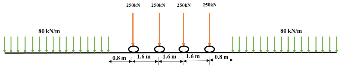
Figure 3.5 Static load condition UIC LM 71
