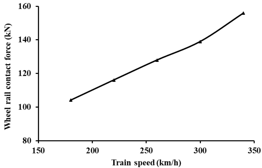
Figure 6.11 Wheel rail interaction force at varying train speed
