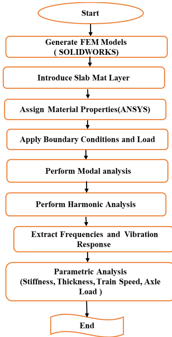
Figure 3.9 Flow chart for methodology of vibration response study
