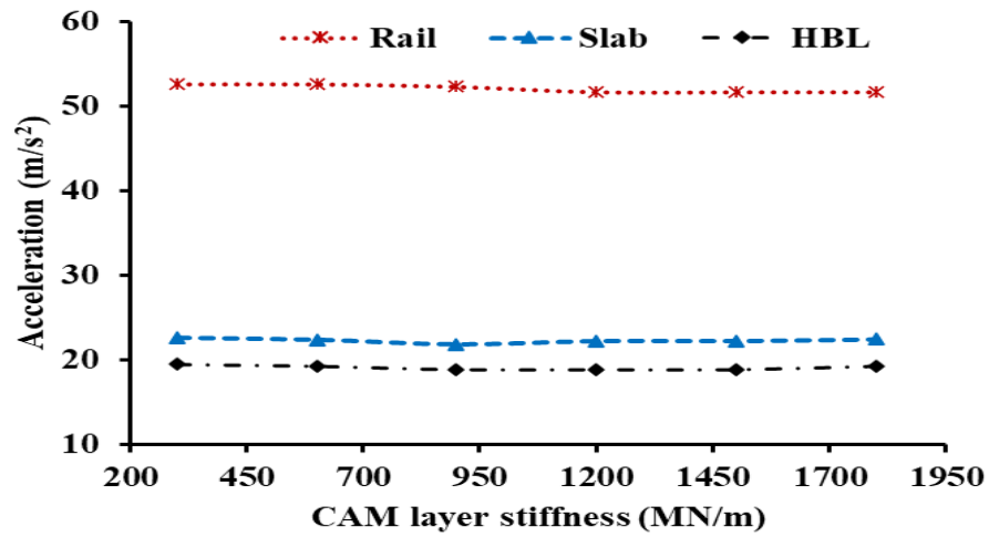
Figure 6.17 Influence of CAM layer stiffness on acceleration of track components
