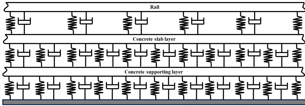
Figure 2.2 A layered schematic showing rail → rail pad (spring–damper) discrete → concrete slab layer→ concrete supporting layer- subgrade
