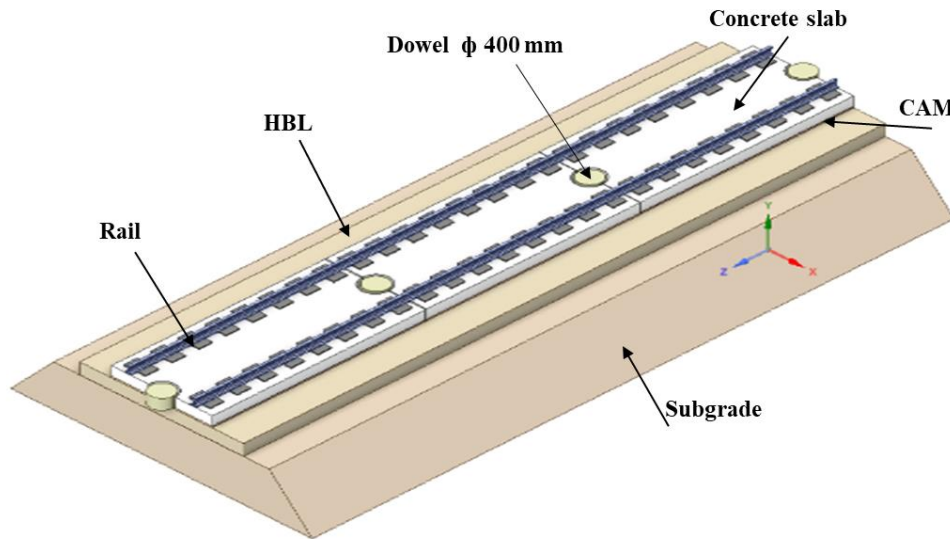
Figure 3.1 Three-dimensional schematic of the slab track FEM model
