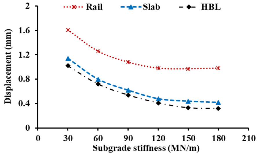
Figure 6.18 Influence of Subgrade stiffness on displacement of track components
