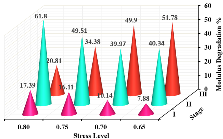
Figure 7.8 Modulus degradation of CAM specimens during flexural fatigue
