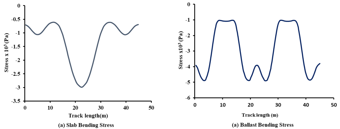
Figure 4.2 Bending stress distribution (a) Slab bending stress and (b) Ballast slab track
