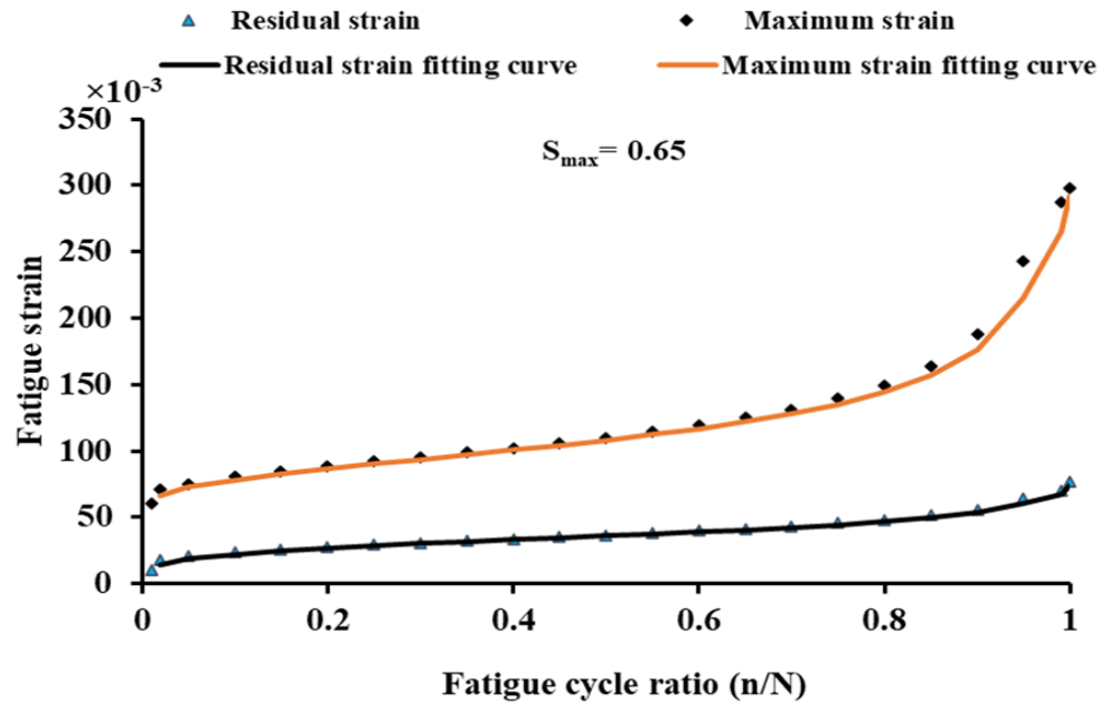
Figure 7.2 Fatigue strain in CAM under applied stress (0.65)
