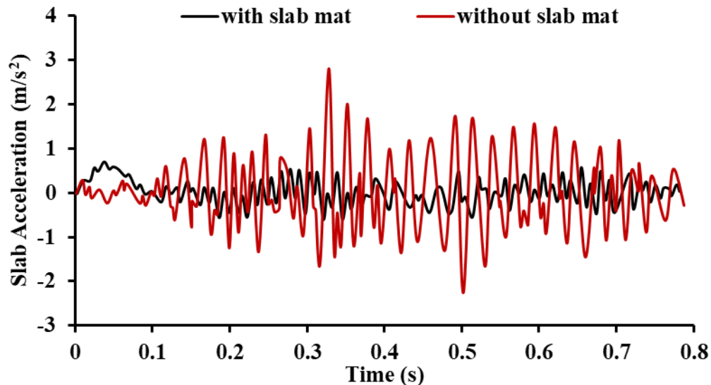
Figure 5.2 Vibration response of concrete slab layer of slab track
