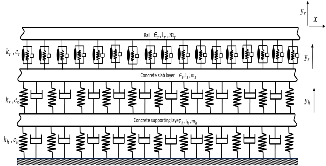
Figure 3.17 Simplified three-layer beam railway slab track model
