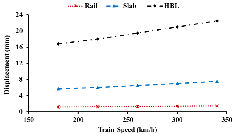
Figure 6.12 Displacement of track components
