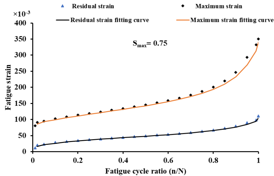
Figure 7.4 Fatigue strain in CAM under applied stress (0.75)
