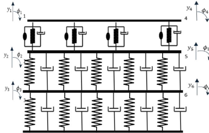
Figure 3.19 Moving three-layer slab track element model
