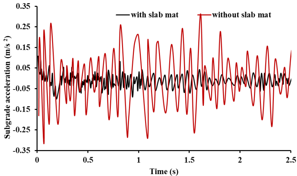
Figure 5.3 Vibration response of subgrade layer of slab track
