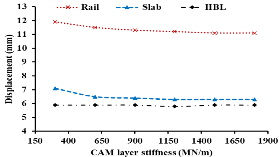
Figure 6.16 Influence of CAM stiffness on displacement of track components
