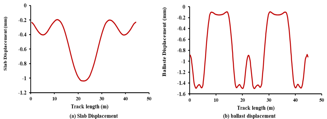
Figure 4.1 Vertical displacement of track under UIC LM71 load (a) Slab displacement (b) Ballast displacement
