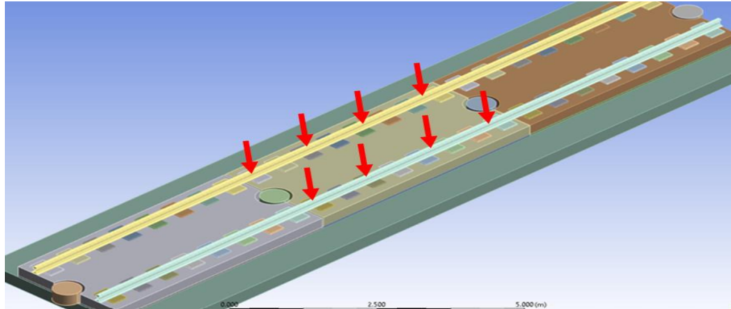
Figure 3.4 Application of loading on the slab track FEM model
