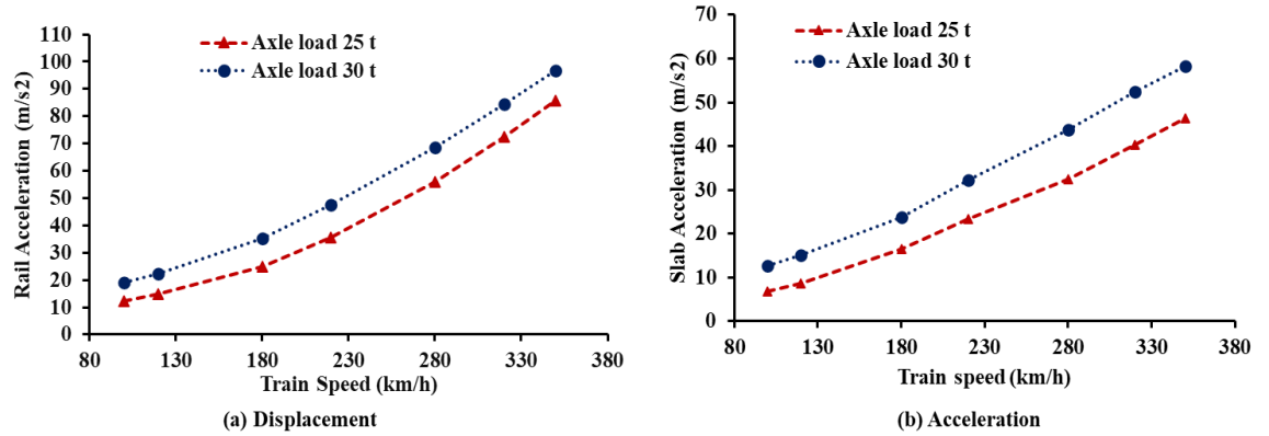
Figure 5.10 The effect of train speed on rail and concrete slab acceleration with varying axle load
