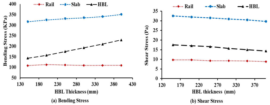
Figure 4.8 Effect of HBL thickness on stresses in Rail, slab and HBL (a) Bending stress (b) Shear Stress
