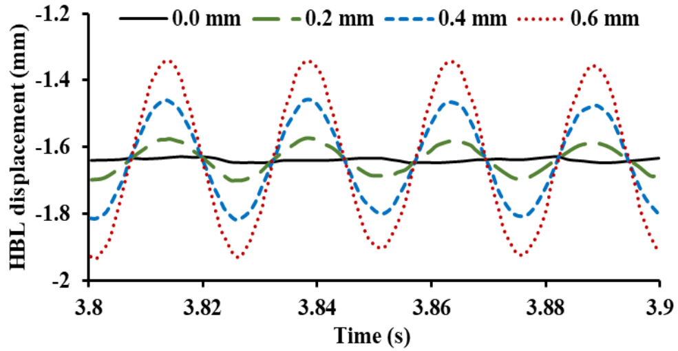
Figure 6.8 HBL displacement at contact point of first wheel when v = 160 km/h, \eta_x = 0 mm, 0.2mm, 0.4mm, 0.6 mm at \omega = 1.5 m
