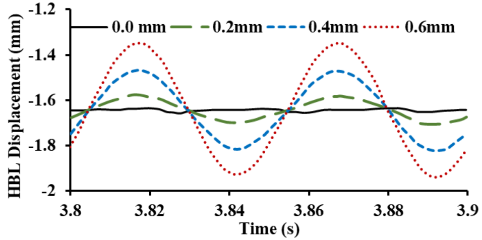
Figure 6.7 HBL displacement at contact point of first wheel when v = 160 km/h, \eta_x = 0 mm, 0.2mm, 0.4mm, 0.6 mm at \omega = 1.0 m
