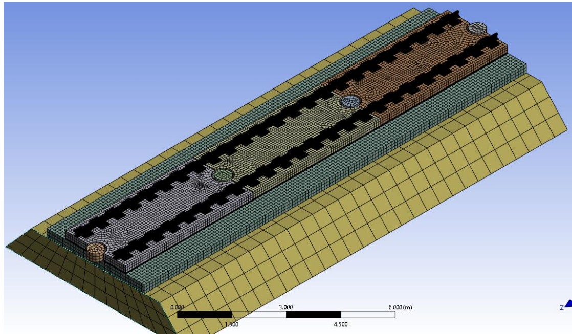
Figure 3.3 FEM mesh of slab track model
