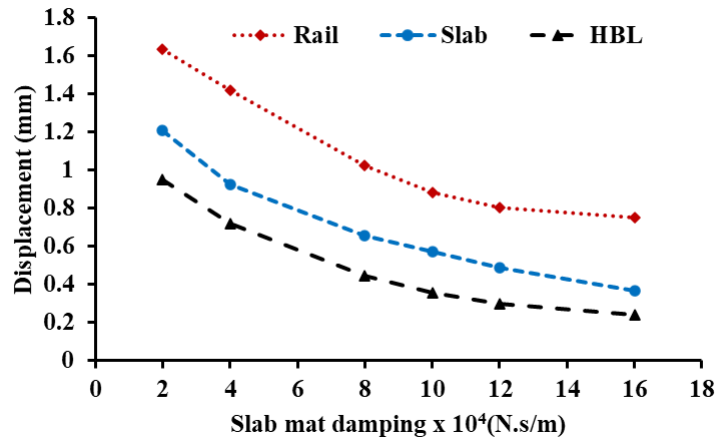
Figure 5.6 Effect of varying the slab mat damping on the vertical displacement
