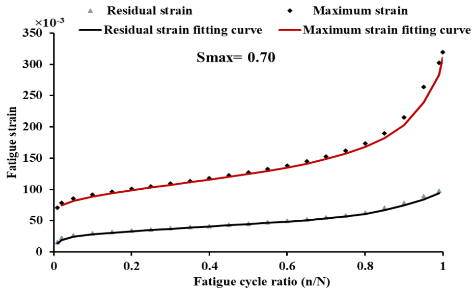
Figure 7.3 Fatigue strain in CAM under applied stress (0.70)
