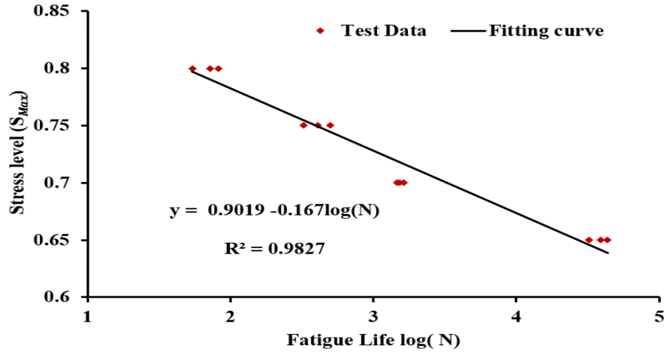
Figure 7.1 Fatigue life curve for the CAM
