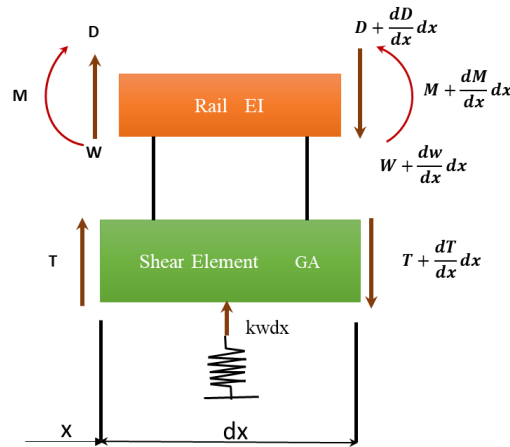
Figure 2.3 A rail beam on Winkler springs connected by a shear layer representing Pasternak's foundation
