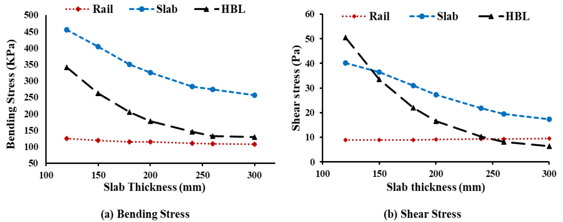
Figure 4.6 Effect of slab thickness (a) Bending stress (b) Shear stresses
