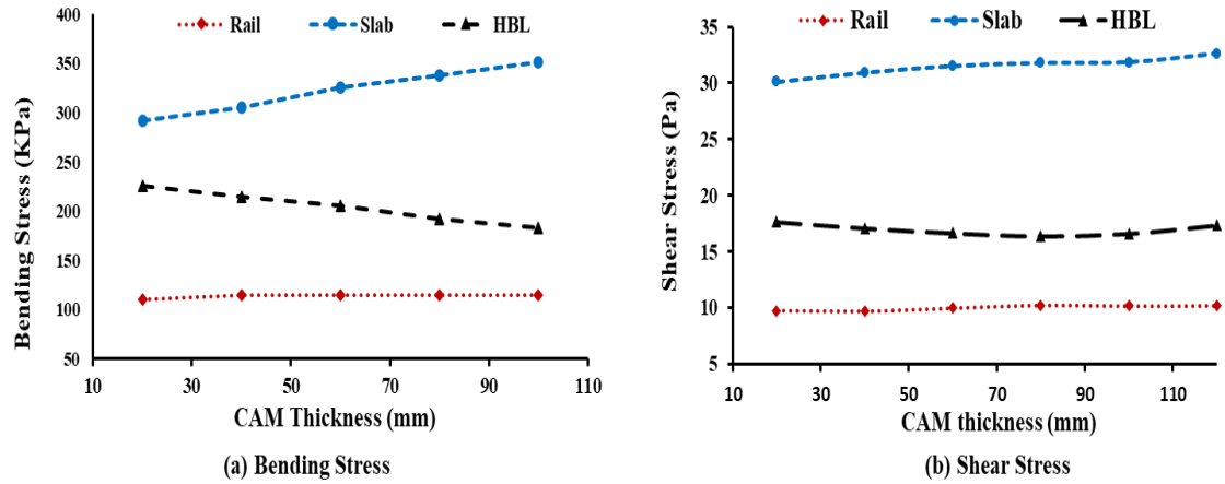
Figure 4.7 Effect of CAM thickness on stress redistribution between rail, slab and HBL (a) Bending stress (b) Shear Stress
