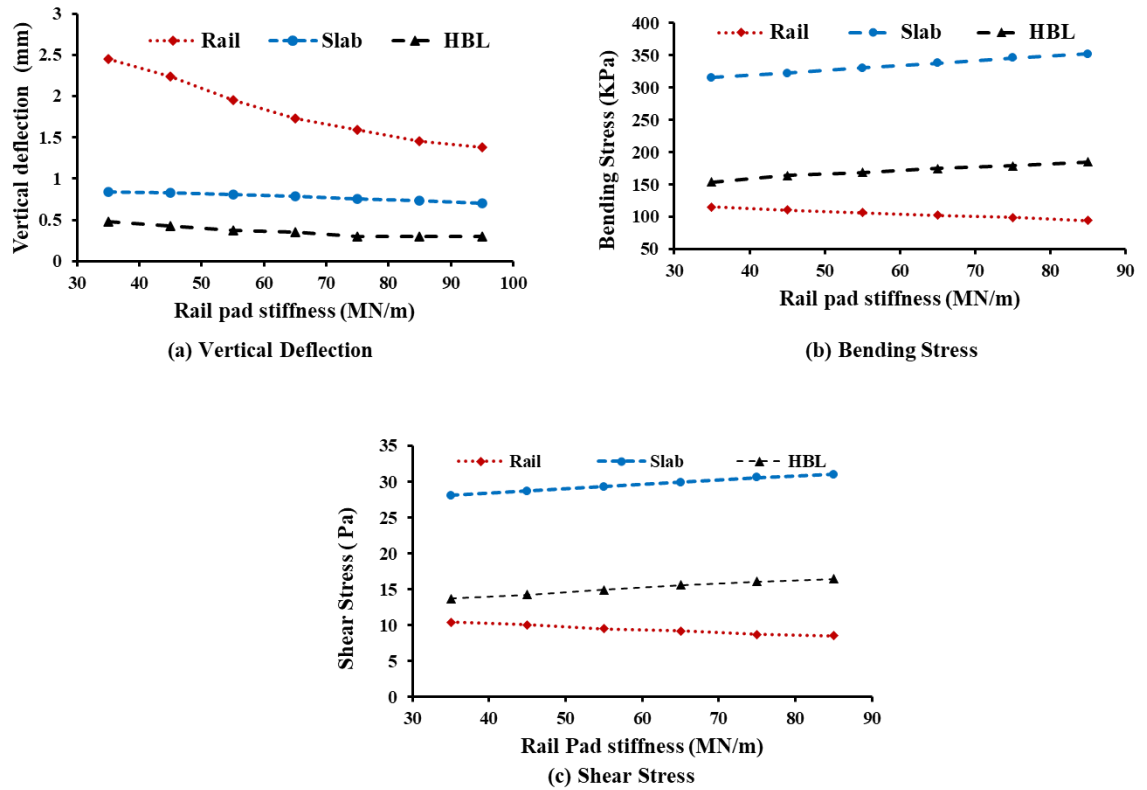
Figure 4.3 Impact of rail pad stiffness on both vertical deflection and stress (a) Vertical deflection (b) Bending stress (c) Shear stress
