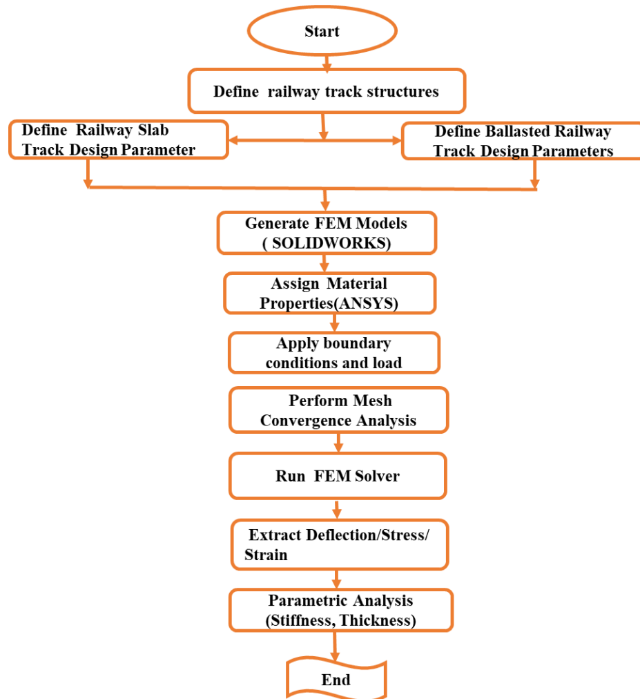
Figure 3.6 Flow chart for methodology of static response study
