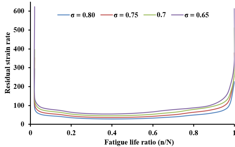
Figure 7.6 Variation of residual strain rate with number of fatigue cycles for CAM specimens
