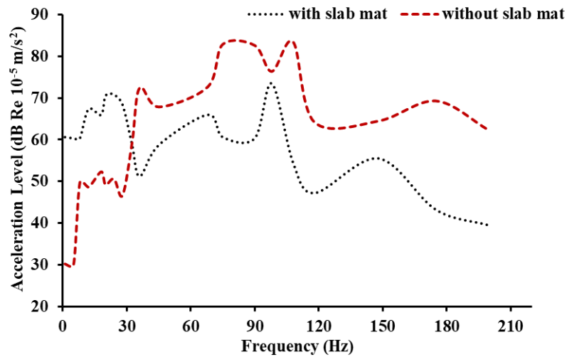
Figure 5.4 Vibration response of the subgrade layer of slab track in the frequency domain
