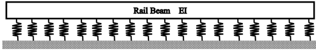
Figure 2.1 A schematic showing a continuous beam on Winkler springs
