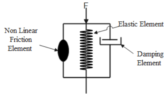
Figure 3.14 Rail pads nonlinear model
