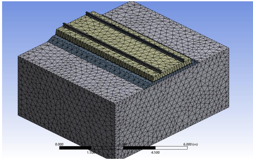
Figure 3.10 Tetrahedral medium meshing of the 3D model
