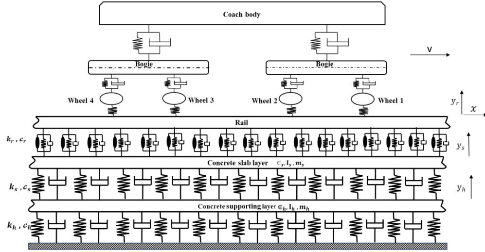
Figure 3.13 The model of system for vehicle-track coupling
