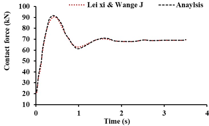
Figure 6.2 Wheel-rail contact force profile
