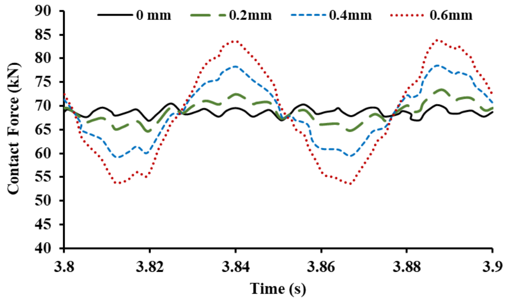
Figure 6.10 Wheel rail contact force at contact point of first wheel when v = 160 km/h, \eta_x = 0 mm, 0.2 mm, 0.4 mm, 0.6 mm at \omega = 1.5 m
