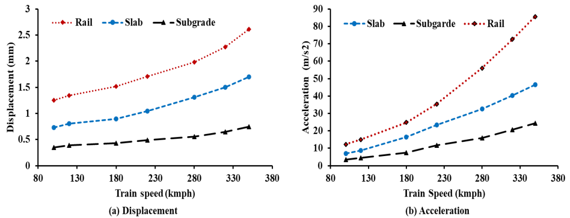
Figure 5.9 Effect of train speed on vibration response of track
