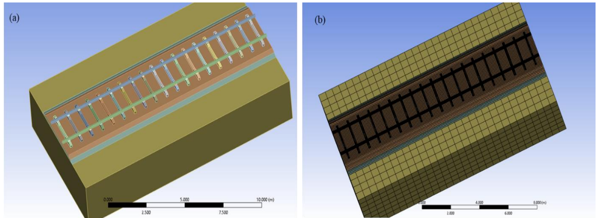
Figure 3.7 Isometric view of railway track structure and meshing model: a) FEM Ballast track model; b) Meshing ballast track model
