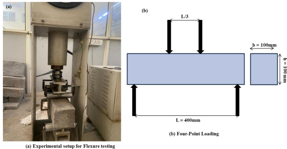
Figure 3.21 Experimental setup for the static four-point flexural strength test of CAM
