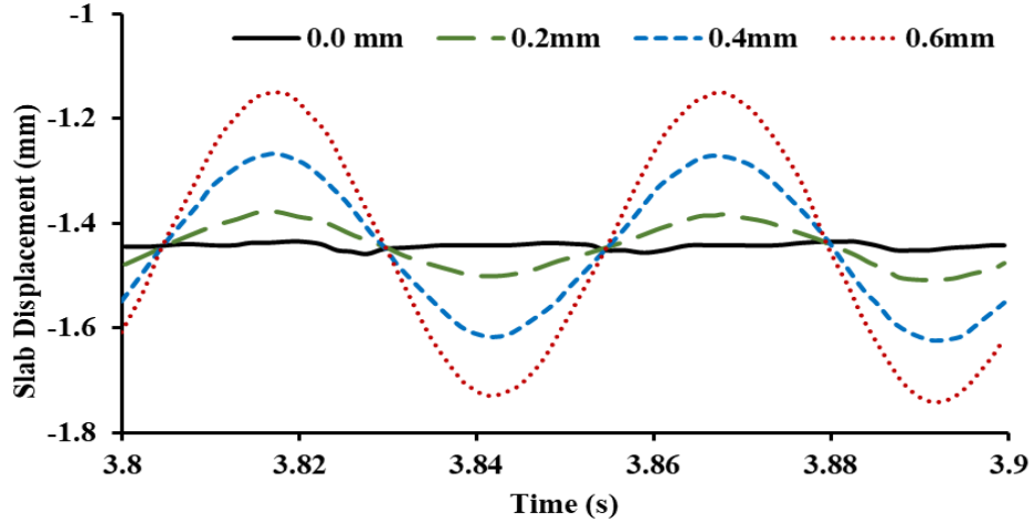
Figure 6.6 Slab displacement at contact point of first wheel when v = 160 km/h, \eta_x = 0 mm, 0.2mm, 0.4mm, 0.6 mm at \omega = 1.5 m
