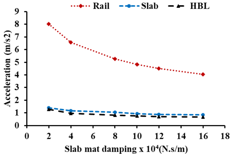
Figure 5.7 Effect of varying the slab mat damping on the vertical acceleration
