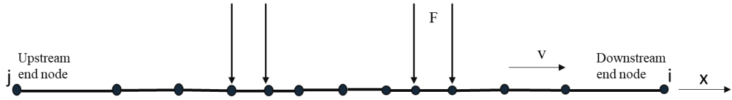
Figure 3.18 Discretization of rail beam of slab track into moving elements
