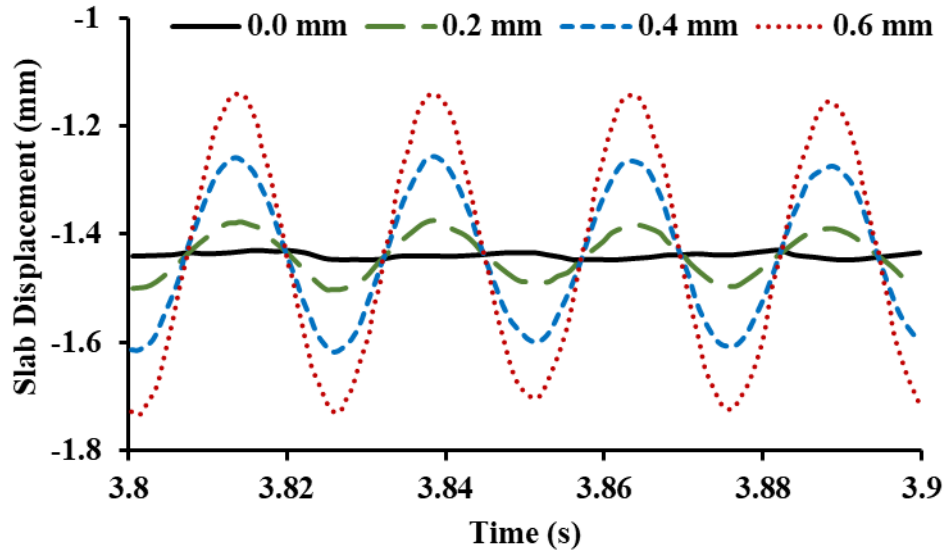
Figure 6.5 Slab displacement at contact point of first wheel when v = 160 km/h, \eta_x = 0 mm, 0.2mm, 0.4mm, 0.6 mm at \omega = 1.0 m
