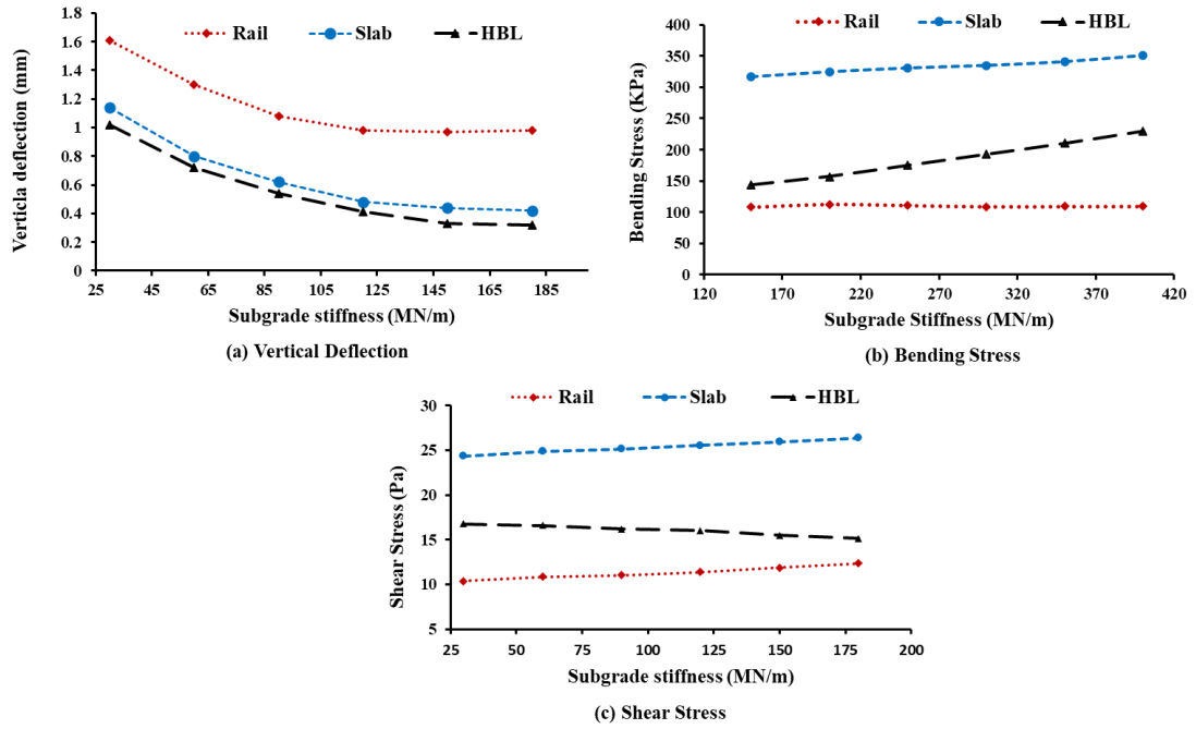
Figure 4.5 Influence of subgrade stiffness on both vertical deflection and stress (a)Vertical deflection (b)Bending stress (c) Shear stress
