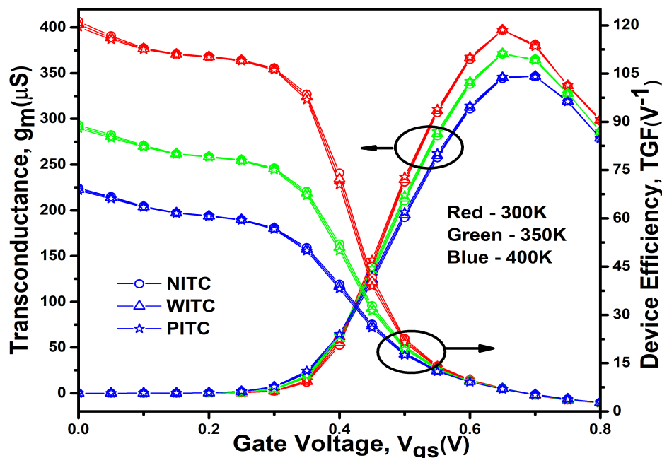
Figure 4.6: Impact of ITCs on transconductance and device efficiency of HD-VS-FeFinFET at different operating temperatures (VC25b).
