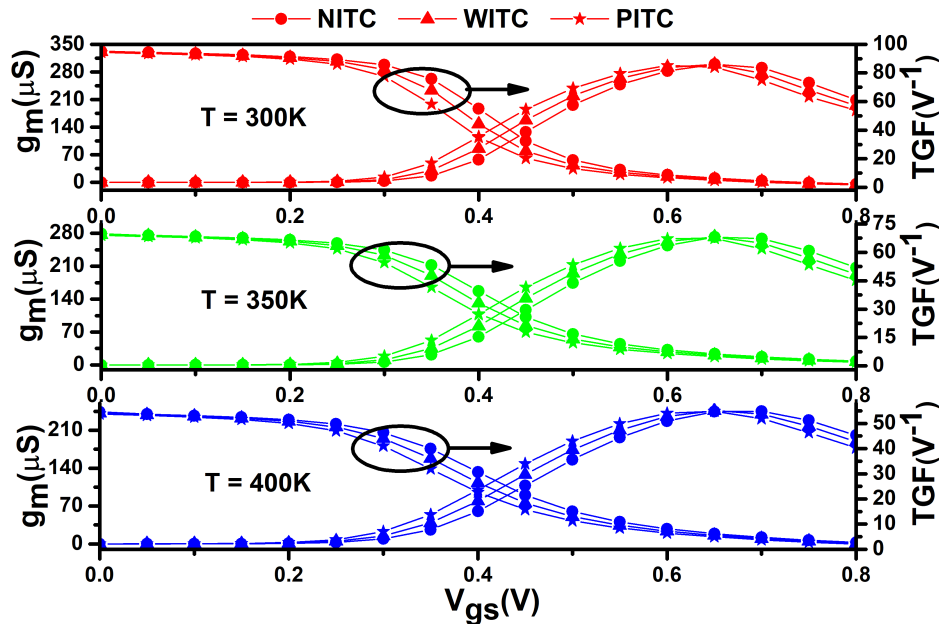
Figure 4.7: Influence of ITCs on transconductance and device efficiency of VS-FeFinFET at different operating temperatures (VC25b).
