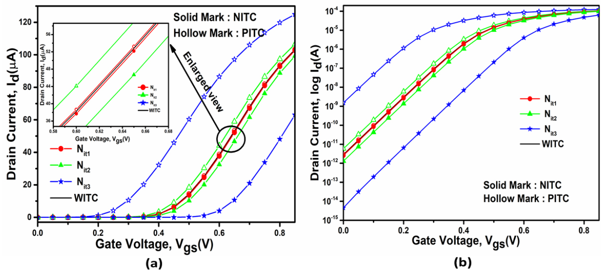
Figure 4.10: Impact of ITC's density and polarity on transfer characteristics of VS-FeFinFET in (a) linear and (b) log scale (VC25b).
