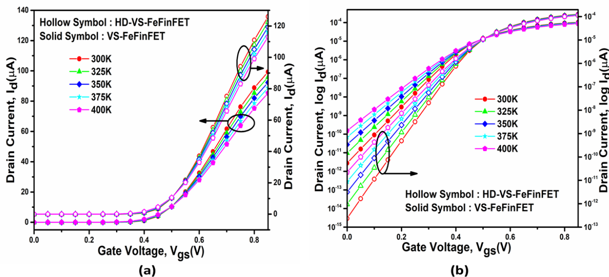
Figure 4.2: Impact of temperature on transfer characteristics of HD-VS-FeFinFET and VS-FeFinFET in (a) linear and (b) log scale (VC25b).
