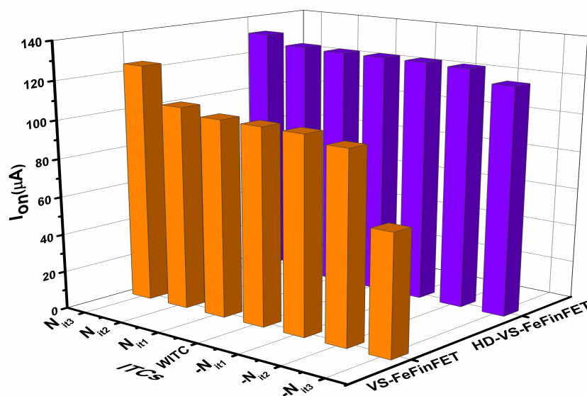
Figure 4.12: Effect of ITC's density and polarity on the ON current of HD-VS-FeFinFET and VS-FeFinFET (VC25b).
