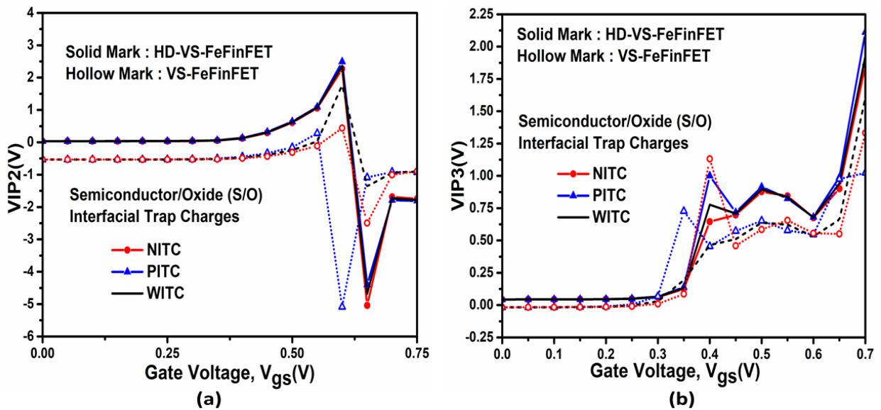
Figure 3.11: Effect of ITCs on voltage intercept point (a) VIP2 (b) VIP3 of HD-VS-FeFinFET and VS-FeFinFET at V_{ds}=0.4V (VC25c).
