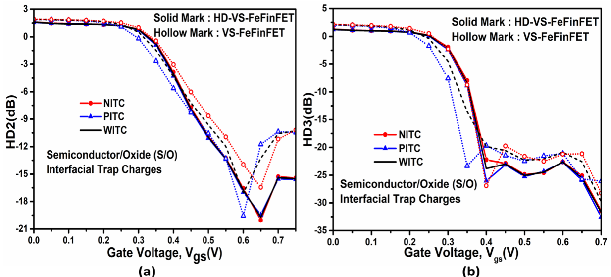
Figure 3.13: Effect of ITCs on harmonics distortion (a) HD2 and (b) HD3 for HD-VS-FeFinFET and VS-FeFinFET at V_{ds}=0.4V (VC25c).
