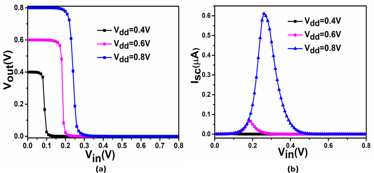
Figure 5.17: Impact of varying biasing voltage on (a) Voltage Transfer Characteristics and (b) Switching Current of HD-VS-FeFinFET based CMOS inverter (VC25a).
