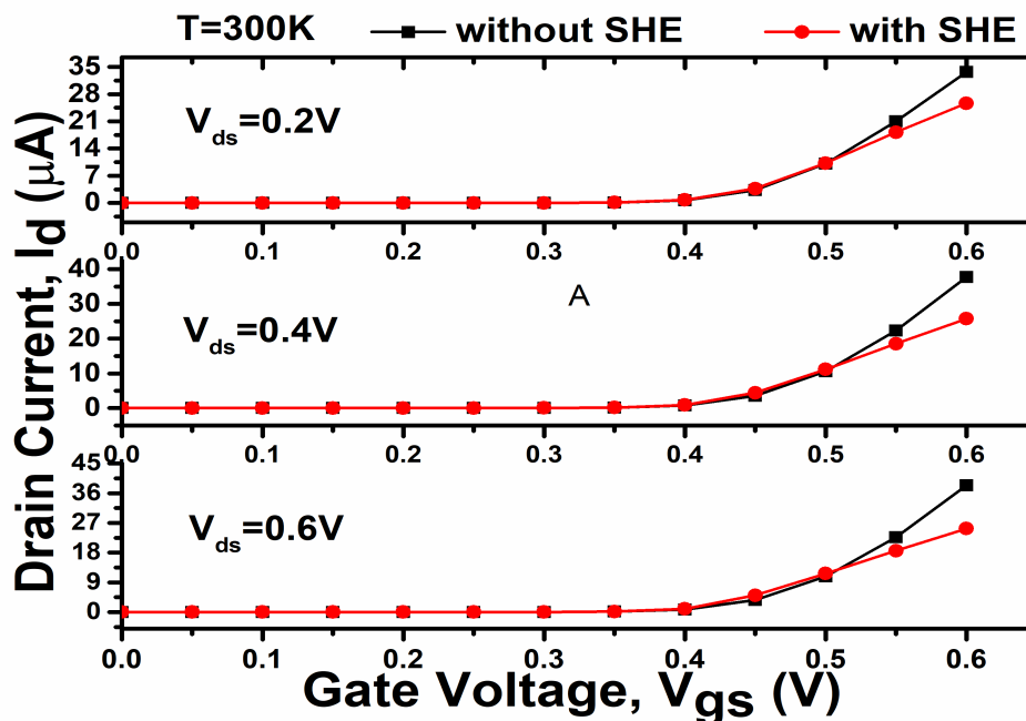
Figure 5.8: Influence of SHE on the transfer characteristics of HD-VS-FeFinFET at different biasing voltages (VC25a).
