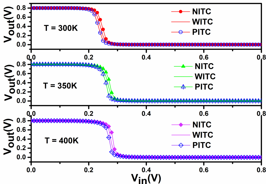
Figure 4.16: Impact of ITCs polarity on voltage transfer characteristics of HD-VS-FeFinFET based CMOS inverter at various operating temperatures (VC25b).
