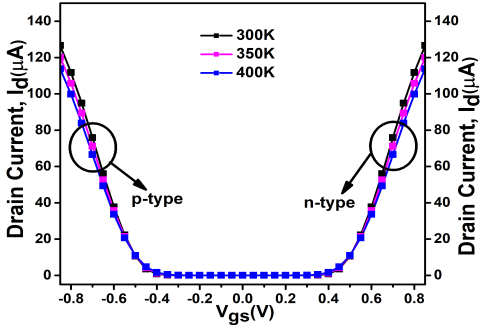
Figure 5.16: Influence of varying ambient temperature on threshold voltage matching curve for HD-VS-FeFinFET based CMOS inverter (VC25a).
