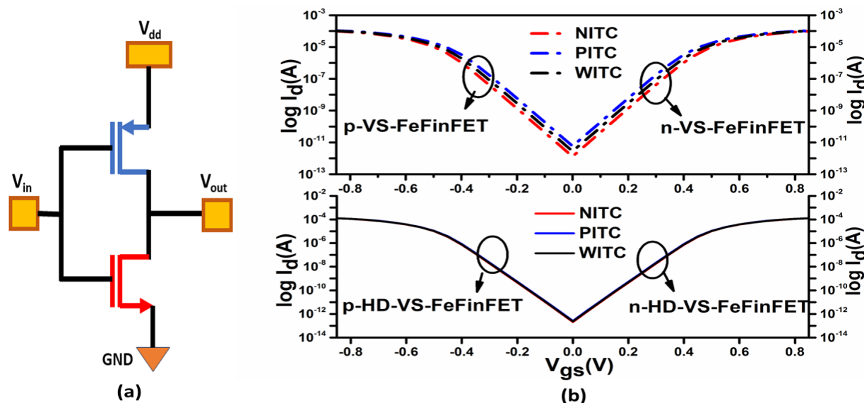
Figure 3.14: (a) Schematic diagram of CMOS Inverter (b) threshold voltage matching curve for HD-VS-FeFinFET and VS-FeFinFET under the influence of ITCs (VC25c).
