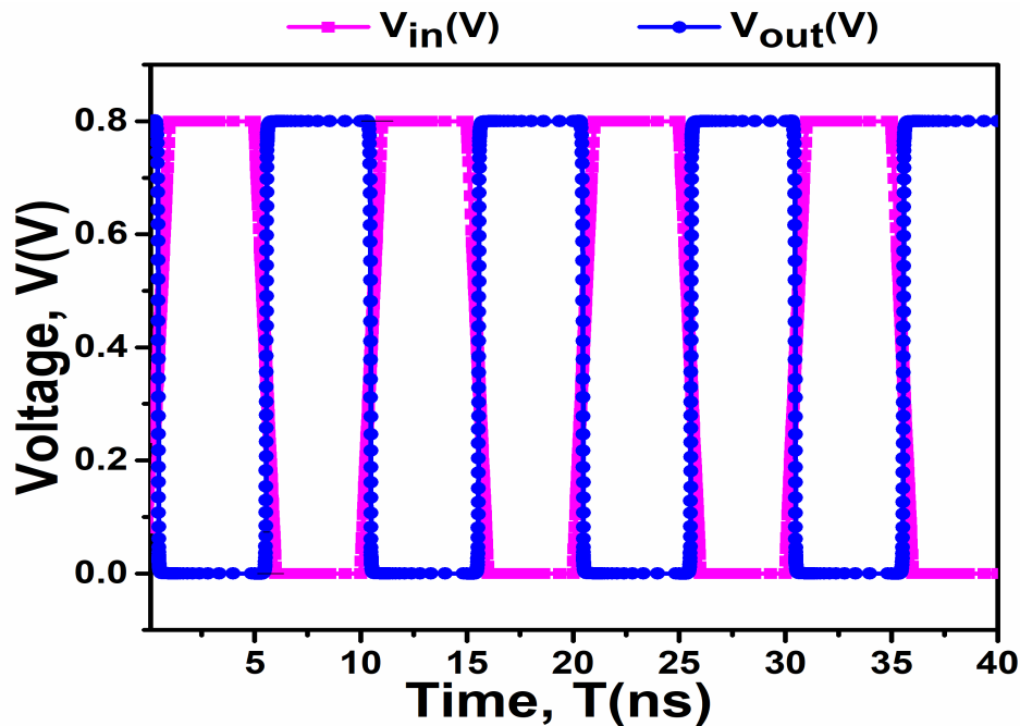
Figure 5.19: Output transition waveform of the HD-VS-FeFinFET based CMOS inverter (VC25a).
