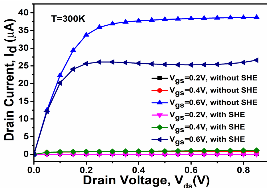
Figure 5.11: Influence of SHE on the output characteristics of HD-VS-FeFinFET at different biasing voltages (VC25a).
