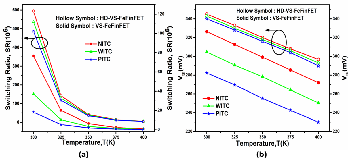
Figure 4.5: Variation in (a) switching ratio and (b) threshold voltage of both the devices under the influence of ITCs at different operating temperatures (VC25b).
