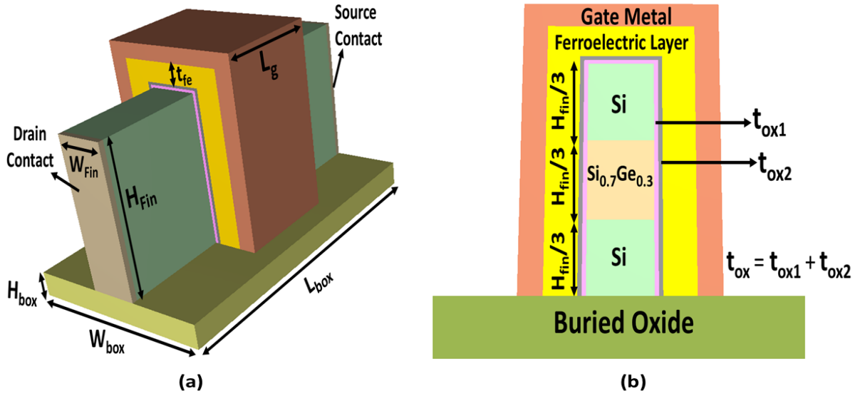
Figure 5.1: (a) 3D schematic view of HD-VS-FeFinFET (b) inset of vertical cross-sectional view of HD-VS-FeFinFET (VC25a).
