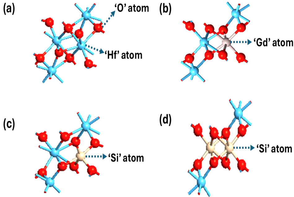
Figure 5.4: Atomic level structure considered for four different configurations (a) Undoped \text{HfO}_2 (b) gadolinium doped \text{HfO}_2 (c) singly Si-doped \text{HfO}_2 (d) doubly Si-doped \text{HfO}_2 (VC25a).
