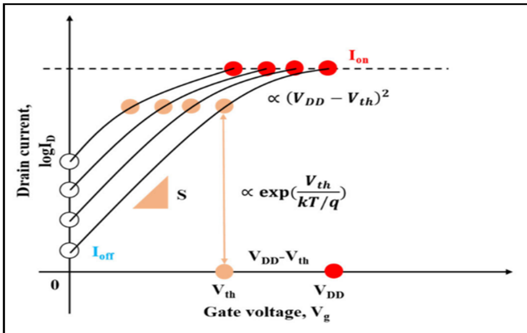
Figure 1.2: The I_d - V_g characteristics for conventional transistor with scaling of gate length (hpm).
