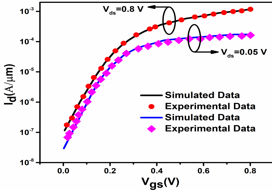
Figure 3.2: Experimental and simulated transfer characteristic for Silicon on Insulator (SOI) FinFET at V_{ds}=0.05V and V_{ds}=0.8V (VC25c).
