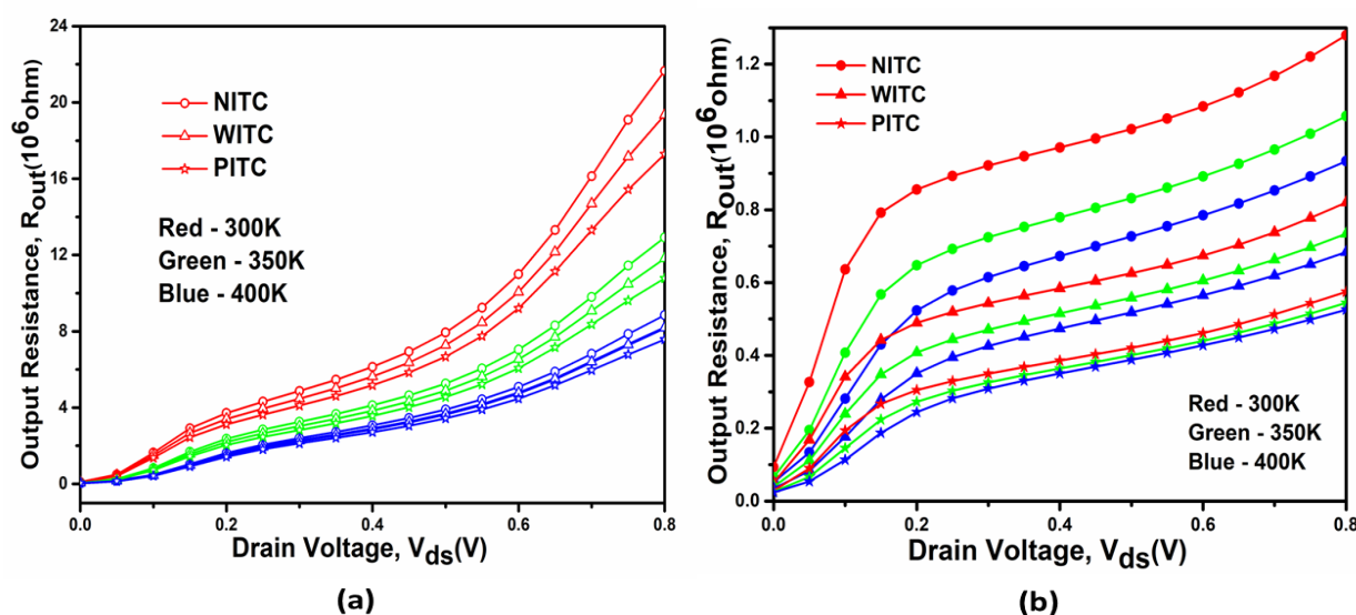
Figure 4.9: Variation in output resistance of (a) HD-VS-FeFinFET and (b) VS-FeFinFET under the influence of ITCs at different operating temperatures (VC25b).
