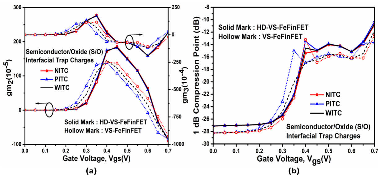
Figure 3.10: Impact of ITCs on (a) higher order transconductance coefficient ( g_{m2} and g_{m3} ) (b) 1-dB Compression Point of HD-VS-FeFinFET and VS-FeFinFET at V_{ds}=0.4V (VC25c).
