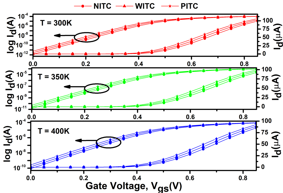
Figure 4.4: Impact of ITCs on transfer characteristics of VS-FeFinFET under different operating temperatures (VC25b).
