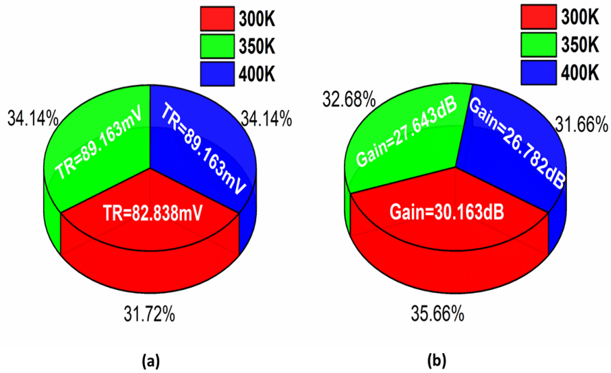
Figure 4.18: Comparison chart of (a) transition region (b) voltage gain of HD-VS-FeFinFET based CMOS inverter at various operating temperatures (VC25b).
