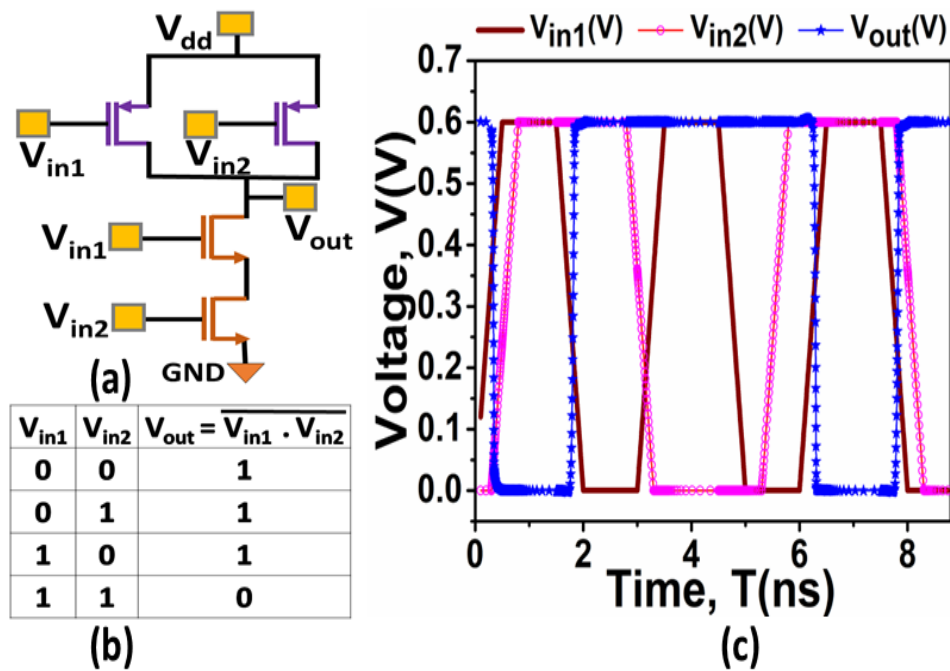
Figure 5.22: (a) Schematic of two-input NAND gate circuit (b) its truth table (c) transient response of NAND gate circuit (VC25a).
