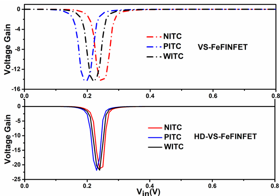
Figure 3.17: Impact of ITCs polarity on voltage gain of HD-VS-FeFinFET and VS-FeFinFET based inverter. (VC25c).
