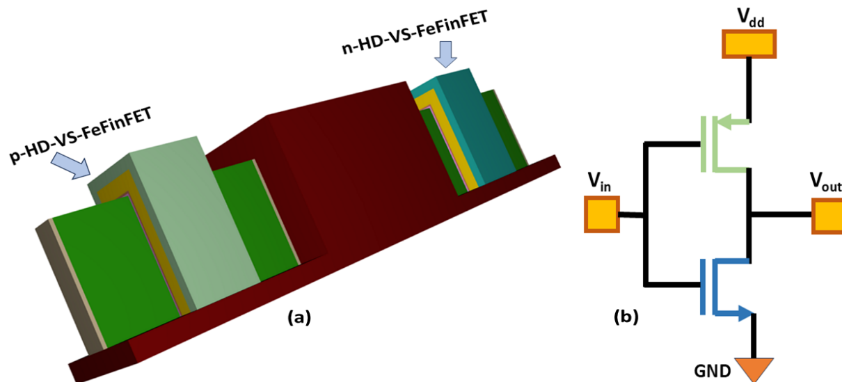
Figure 4.14: (a) 3D structure and (b) Schematic diagram of HD-VS-FeFinFET based CMOS inverter (VC25b).
