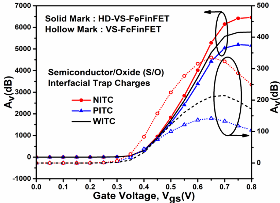
Figure 3.9: Variation of intrinsic gain ( A_v ) for HD-VS-FeFinFET and VS-FeFinFET in presence of different ITCs at V_{ds}=0.4V (VC25c).
