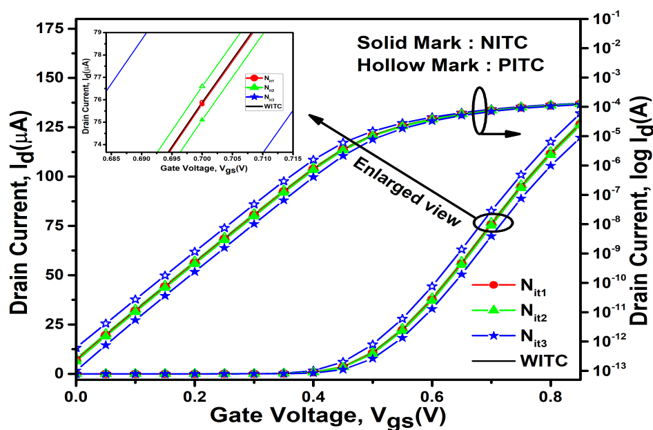
Figure 4.11: Effect of ITC's density and polarity on transfer characteristics of HD-VS-FeFinFET (VC25b).
