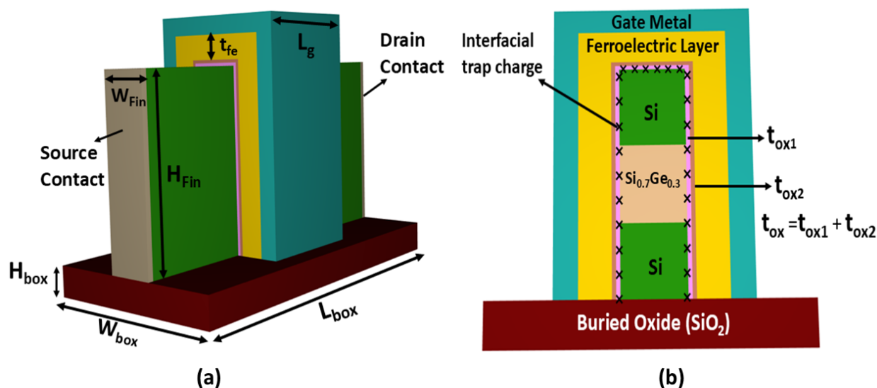
Figure 4.1: (a) 3D schematic view of HD-VS-FeFinFET (b) inset of vertical cross-sectional view of HD-VS-FeFinFET (VC25b).
