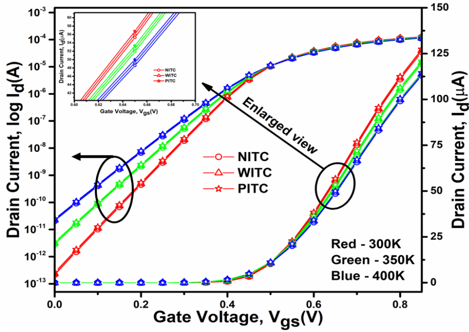
Figure 4.3: Impact of ITCs on transfer characteristics of HD-VS-FeFinFET under different operating temperatures (VC25b).
