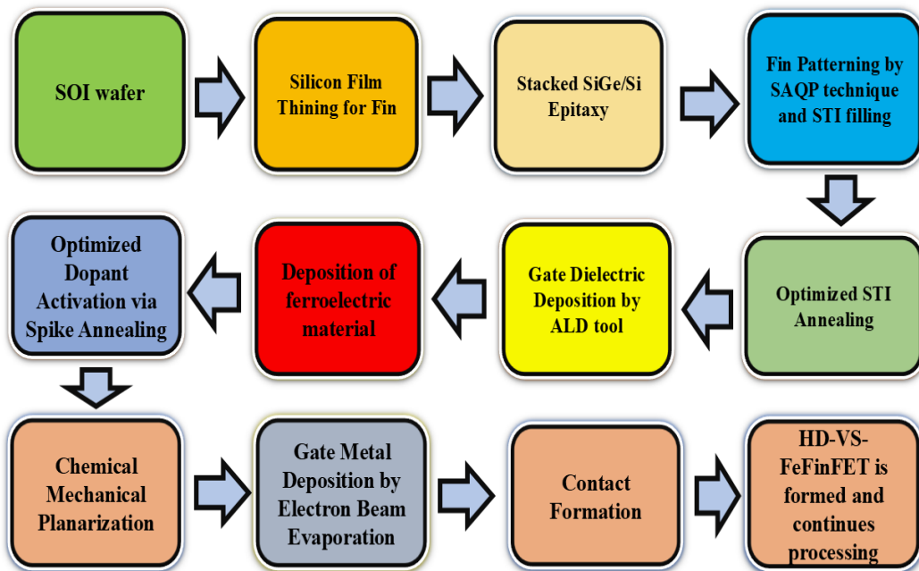
Figure 3.3: Fabrication process flow chart for HD-VS-FeFinFET (VC25c).
