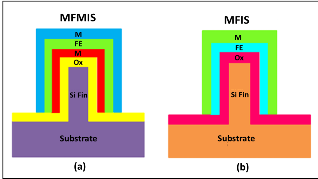
Figure 1.17: Structural view of FeFinFET in distinct configurations (a) MFMIS and (b) MFIS (WSZ + 24).
