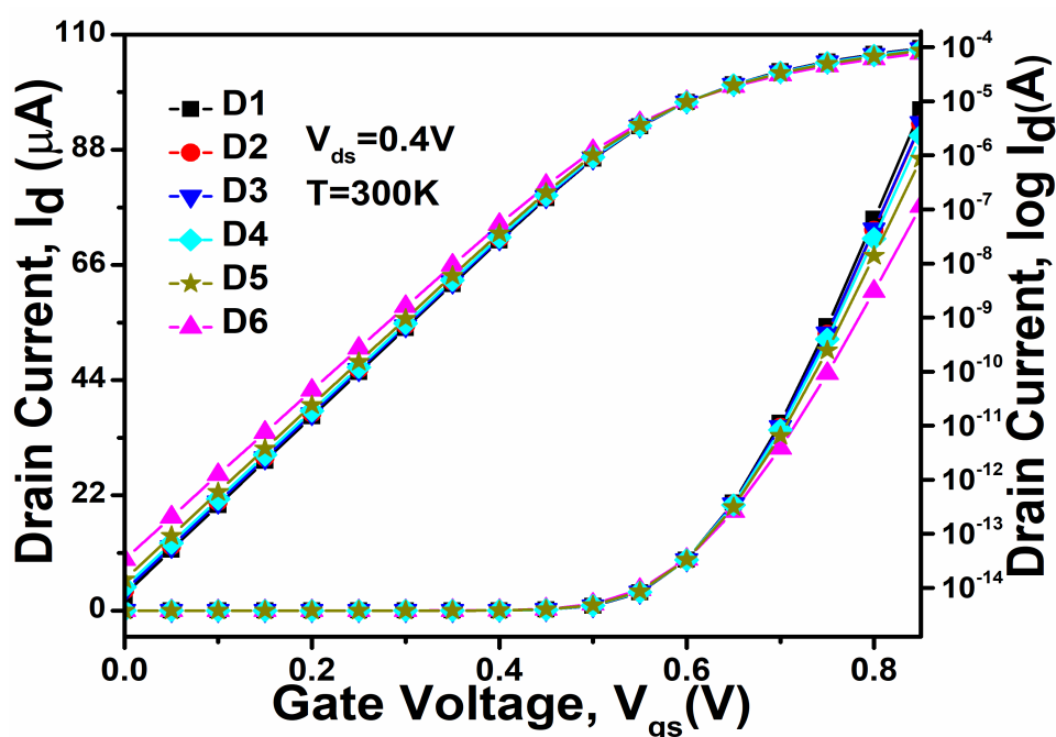
Figure 5.2: Impact of different dopant material on the transfer characteristics of HD-VS-FeFinFET linear and log scale (VC25a).
