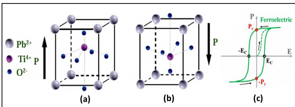
Figure 1.16: Atomic structure of \text{Pb}^{2+}\text{Ti}^{4+}\text{O}_3^{6-} for (a) ferroelectric with up polarisation and (b) ferroelectric with down polarisation (c) The plot of polarisation vs electric field for ferroelectric (Uch18).
