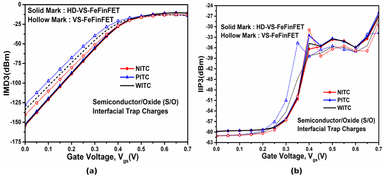
Figure 3.12: Impact of ITCs on (a) third order intermodulation distortion power (IMD3) (b) third order intercept input power (IIP3) of HD-VS-FeFinFET and VS-FeFinFET at V_{ds}=0.4V (VC25c).
