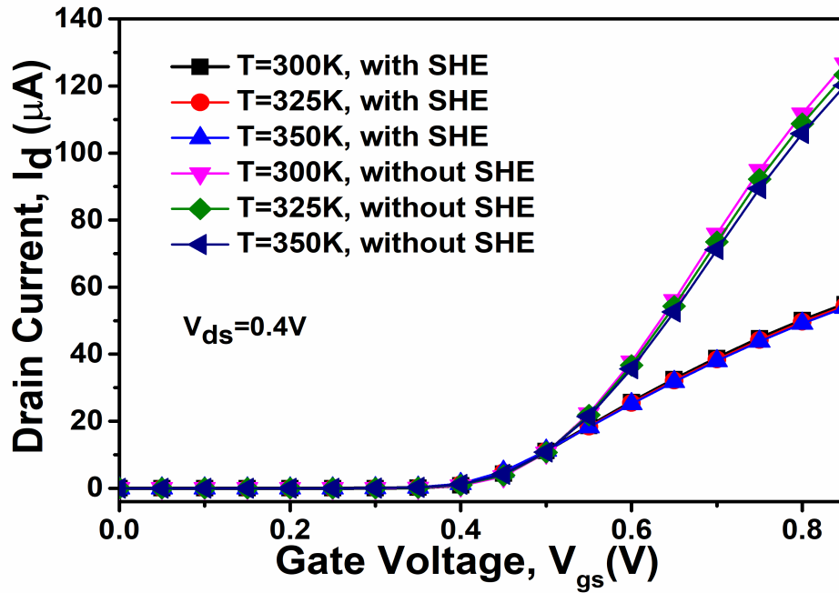
Figure 5.12: Influence of SHE on the transfer characteristics of HD-VS-FeFinFET at varying ambient temperatures (VC25a).
