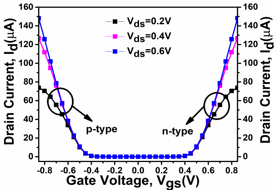
Figure 5.15: Influence of varying biasing voltage on threshold voltage matching curve for HD-VS-FeFinFET based CMOS inverter (VC25a).
