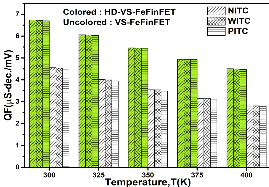
Figure 4.8: Variation in quality factor of HD-VS-FeFinFET and VS-FeFinFET under the influence of ITCs at different operating temperatures (VC25b).
