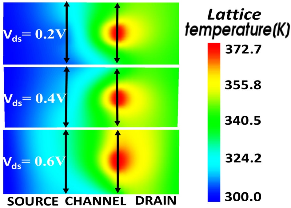
Figure 5.9: Contour profile of lattice temperature at different biasing voltages of HD-VS-FeFinFET under the influence of SHE (VC25a).
