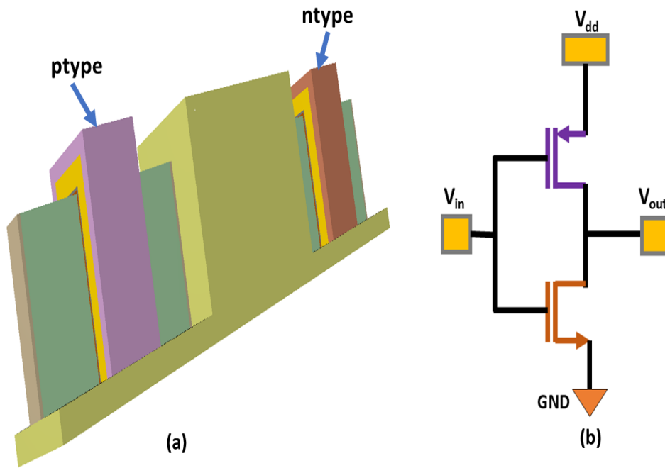
Figure 5.14: (a) 3D structure and (b) Schematic diagram of HD-VS-FeFinFET based CMOS inverter (VC25a).
