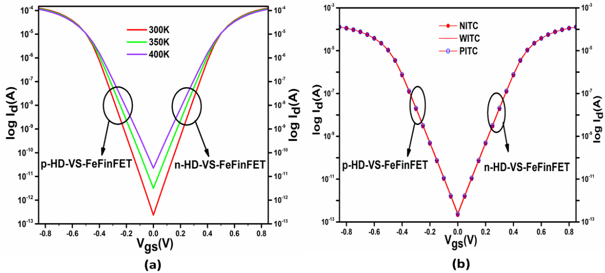
Figure 4.15: Influence of (a) temperature and (b) ITCs on threshold voltage matching curve for HD-VS-FeFinFET based CMOS inverter (VC25b).
