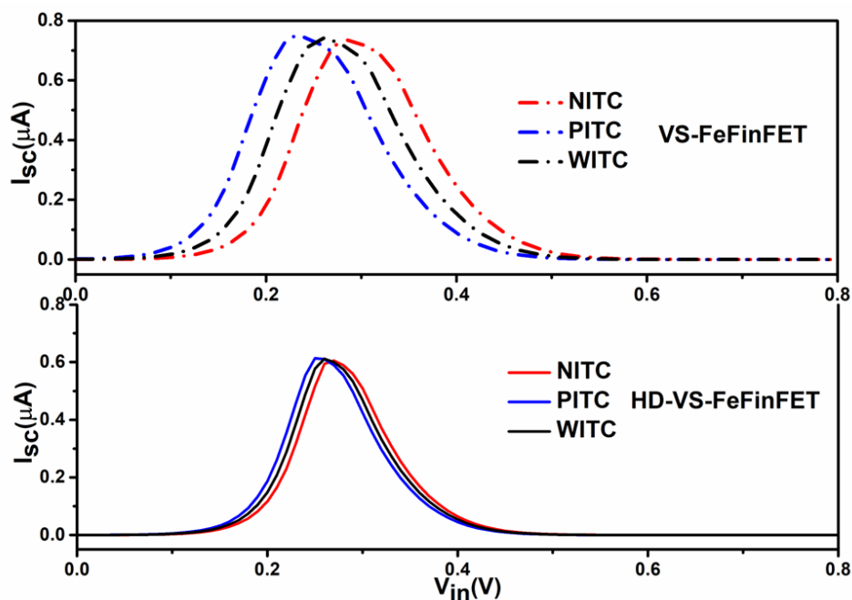
Figure 3.16: Effect of ITCs on switching current of HD-VS-FeFinFET and VS-FeFinFET based inverter (VC25c).
