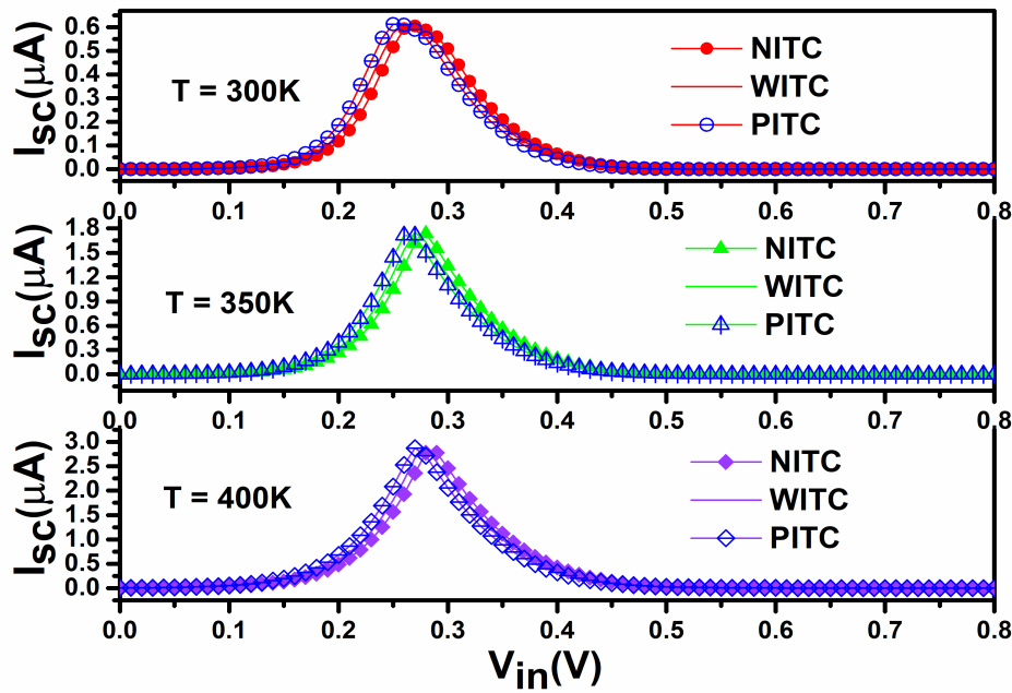
Figure 4.17: Impact of ITCs polarity on switching current of HD-VS-FeFinFET based CMOS inverter at various operating temperatures (VC25b).
