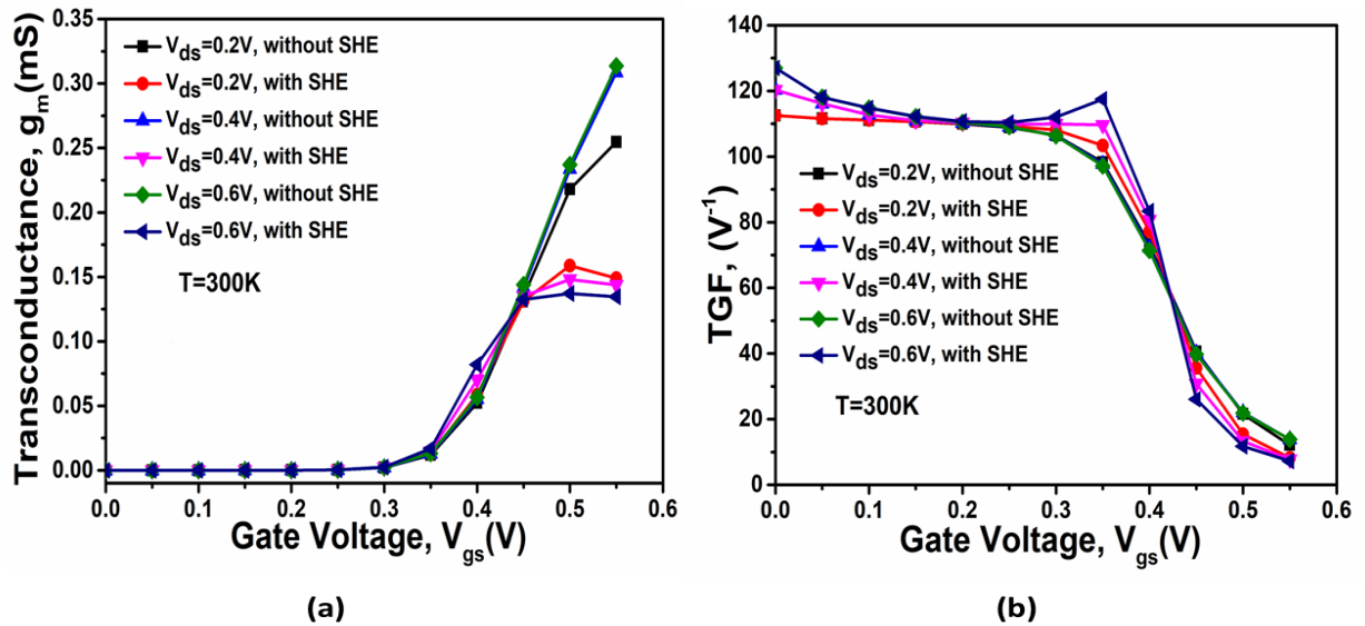
Figure 5.10: Influence of SHE on the (a) g_m (b) TGF for HD-VS-FeFinFET at different biasing voltages (VC25a).
