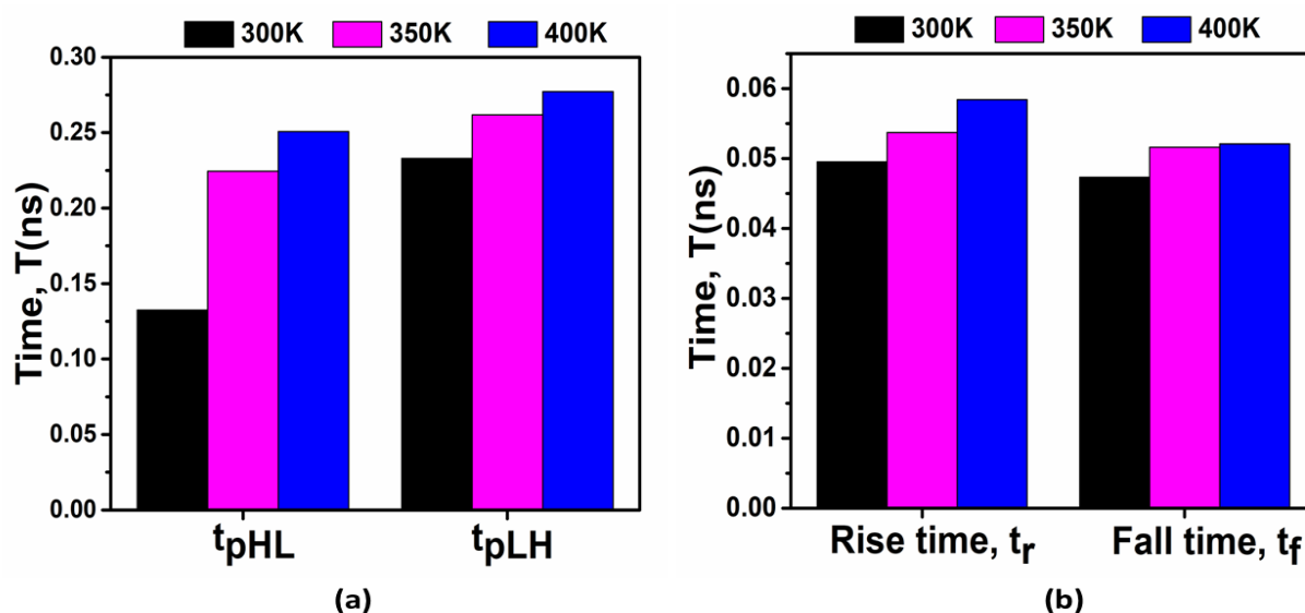
Figure 5.20: Influence of ambient temperature on (a) high to low propagation delay and low to high propagation delay (b) rise time and fall time of HD-VS-FeFinFET based CMOS inverter (VC25a).
