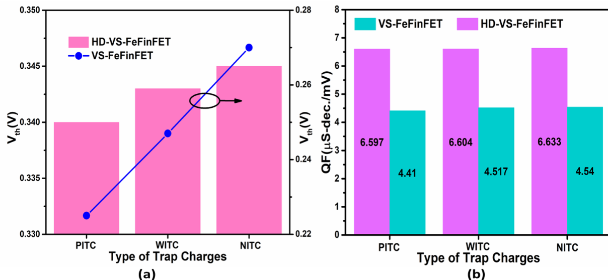
Figure 3.7: Effect of ITCs on (a) threshold voltage ( V_{th} ) (b) quality factor (QF) of HD-VS-FeFinFET and VS-FeFinFET at V_{ds}=0.4\text{V} (VC25c).
