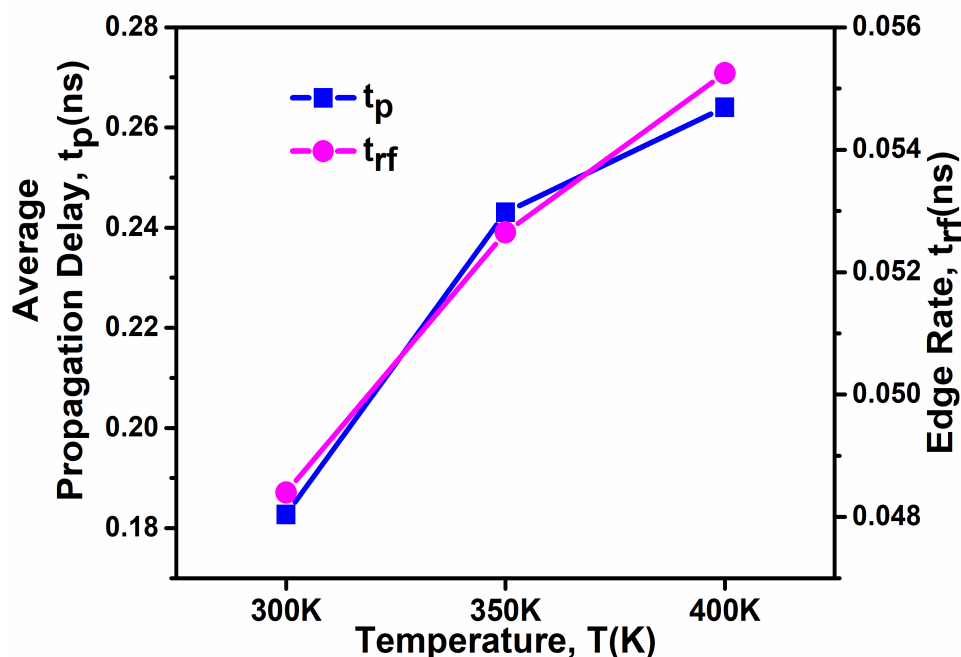
Figure 5.21: Impact of ambient temperature on Propagation delay and Edge Rate of HD-VS-FeFinFET based CMOS inverter (VC25a).
