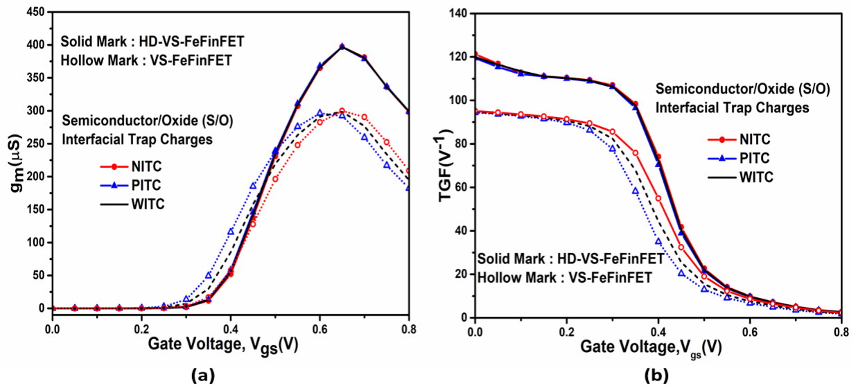
Figure 3.6: Variation in (a) transconductance ( g_m ) and (b) device efficiency (TGF) in presence of different ITCs at V_{ds}=0.4 V (VC25c).
