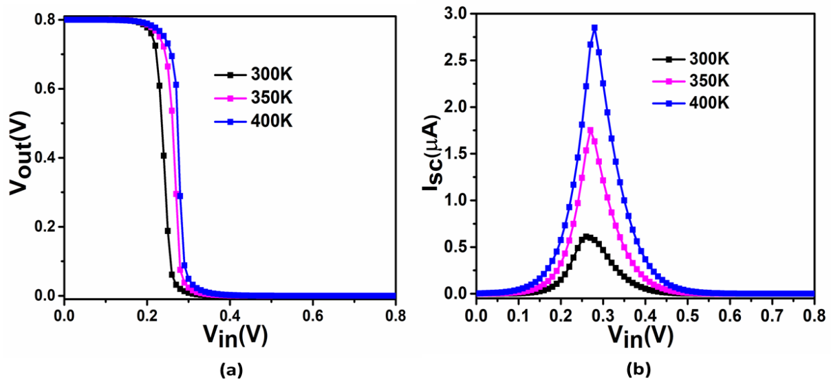
Figure 5.18: Impact of varying ambient temperature on (a) Voltage Transfer Characteristics and (b) Switching Current of HD-VS-FeFinFET based CMOS inverter (VC25a).
