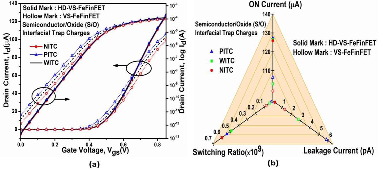
Figure 3.4: Transfer characteristics of HD-VS-FeFinFET and VS-FeFinFET in (a) linear and log scale at V_{ds}=0.4V (b) Comparison of different device characteristics such as ON current ( I_{on} ), leakage current ( I_{off} ) and switching ratio ( I_{on}/I_{off} ) in presence of different ITCs at V_{ds}=0.4V (VC25c).
