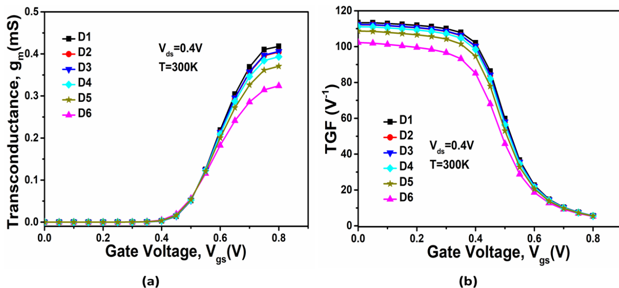
Figure 5.3: Impact of different dopant material on the transconductance and TGF of HD-VS-FeFinFET (VC25a).
