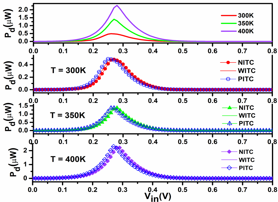
Figure 4.19: Impact of ITCs polarity on power dissipation of HD-VS-FeFinFET based CMOS inverter at various operating temperatures (VC25b).
