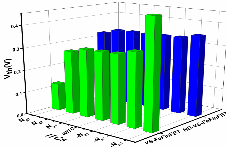
Figure 4.13: Effect of ITC's density and polarity on threshold voltage of HD-VS-FeFinFET and VS-FeFinFET (VC25b).
