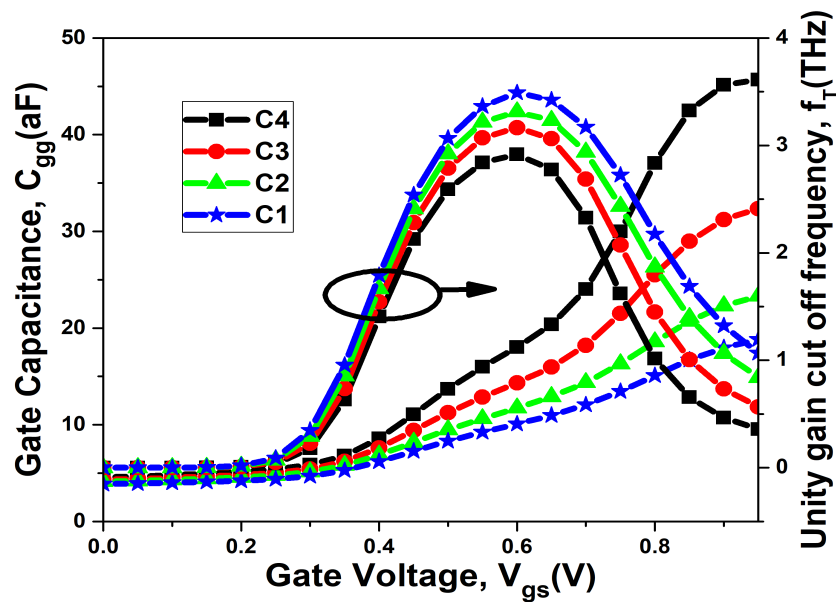
Figure 2.28: Variation in Gate Capacitance and Unity gain cut off frequency for different configurations (VC24a).
