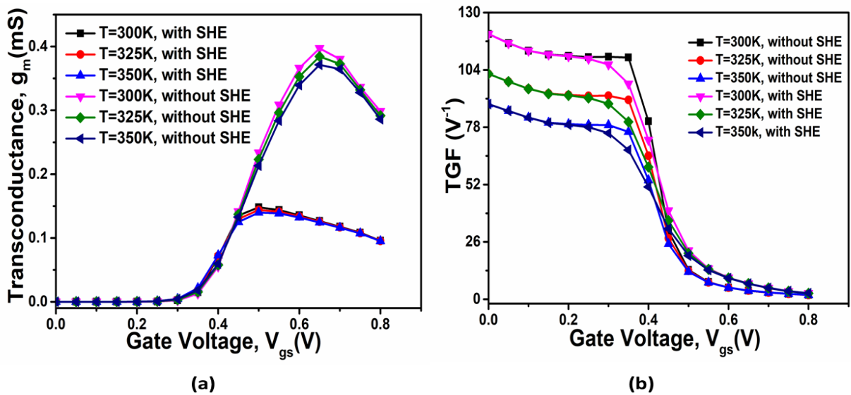
Figure 5.13: Influence of SHE on the (a) g_m (b) TGF for HD-VS-FeFinFET at varying ambient temperatures (VC25a).
