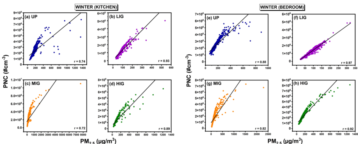
Figure 4.42 Correlation of PNC and PM_{2.5} in different households UP (a,e), LIG (b,f), MIG (c,g), and HIG (d,h) in kitchen and bedroom during winter season.
