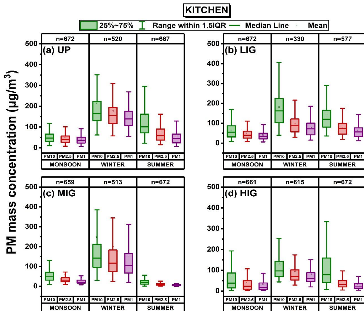
Figure 4.1 Box whisker analysis of \text{PM}_{10} , \text{PM}_{2.5} , and \text{PM}_1 during monsoon, summer, and winter in (a) UP, (b) LIG, (c) MIG, (d) HIG in kitchen. (The data represents 15-minute interval data for 7 days plotted using a box whisker plot in which '□' represents the mean concentration in each size bin. The center line of each box corresponds to the median value, and the box's boundaries correspond to the lower and upper quartile values. The '—' at the top and the bottom of each box denote the maximum and minimum values, respectively. The '+' symbols in red denote the outliers (data points scattered from the quartile values).
