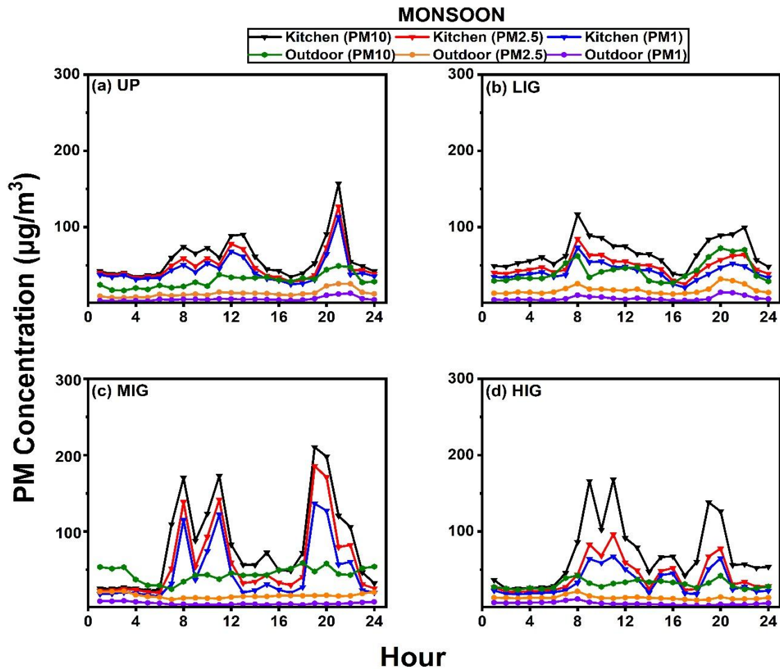
Figure 4.14 Diurnal variation analysis of PM 10 , PM 2.5 , and PM 1 in the kitchen & outdoors of selected households (a) UP (b) LIG (c) MIG (d) HIG during monsoon season.
