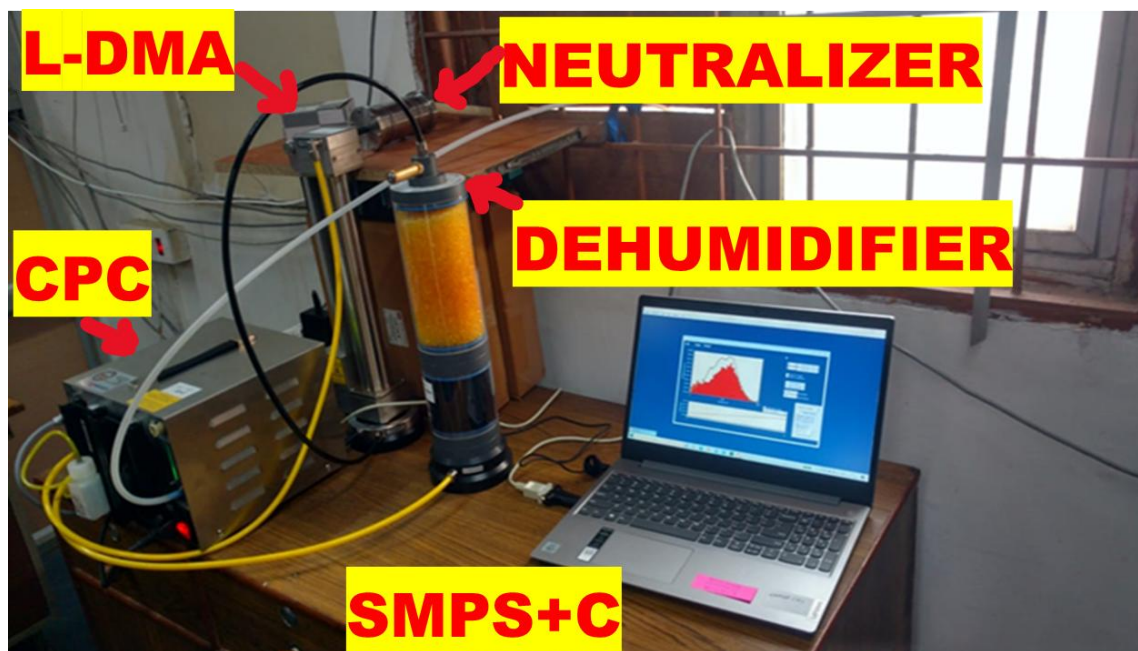
Figure 3.5 Pictorial view of the GRIMM SMPS instrument.
