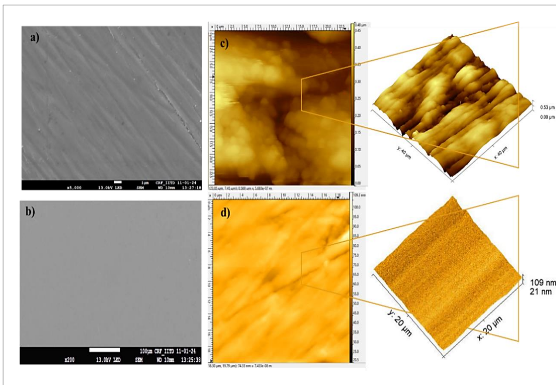
Fig. 5. 21 SEM images of Ti64 alloy before the CH-MR process (a), and after CH-MR with optimal parameters (b), AFM image for Ti64 alloy before the CH-MR process (c), and after CH-MR with optimal parameters (d)
