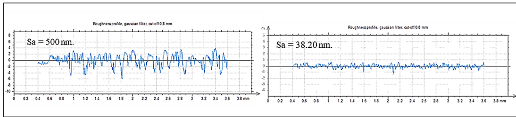
Fig. 5. 20 Roughness profile for Ti64 alloy before and after the CH-MR process
