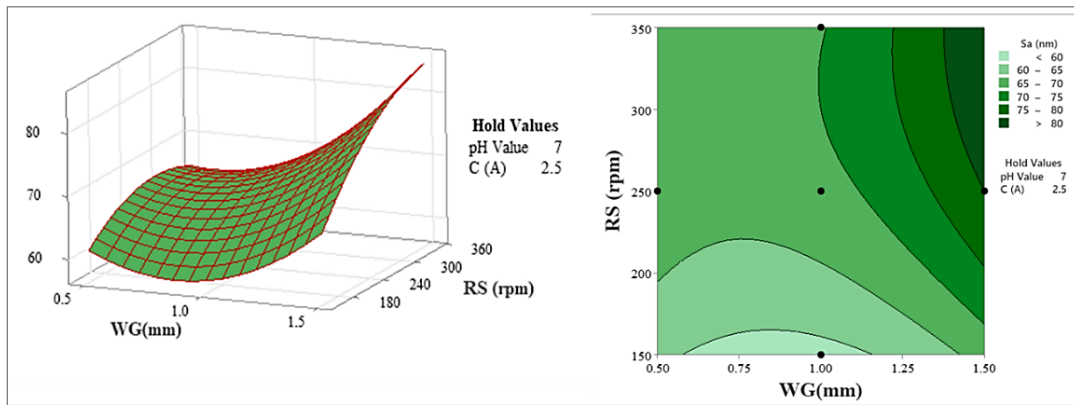
Fig. 5. 18 The interaction plot of Sa vs. C and WG with the contour plot
