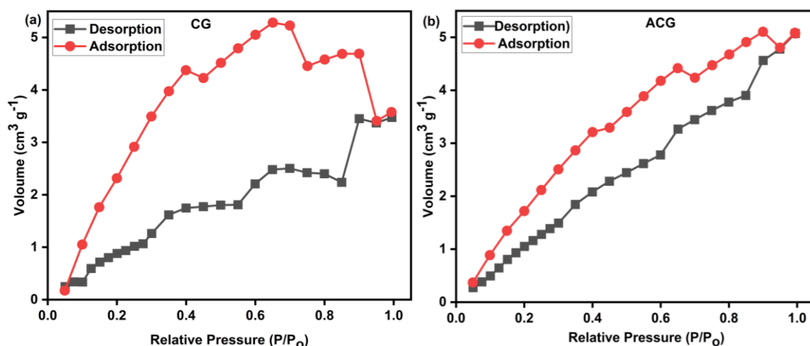
Figure 6. N 2 adsorption-desorption BET analysis of (a) CG and (b) ACG
