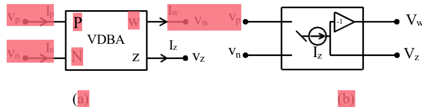
Fig. 4.1 (a) Symbolic Notation (b) Equivalent model of VDBA.
