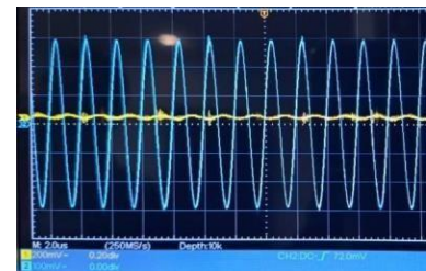
(c) LPF at 500.5k Hz
