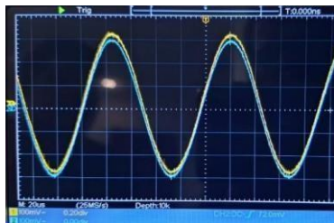
(a) LPF at 10.5k Hz
