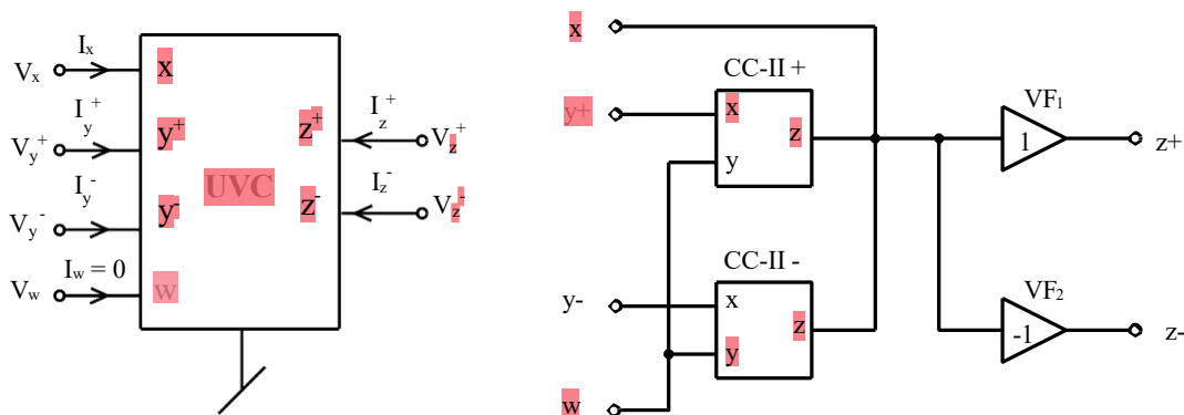
Fig. 2. 1. a) Symbolic Representation of UVC. b) Ideal Circuit Model Of UVC [1]
