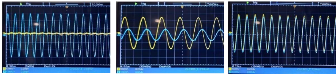
(a) HPF at 10.5k Hz
