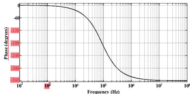
Fig. 5.4. Phase Response of All-Pass Filter
