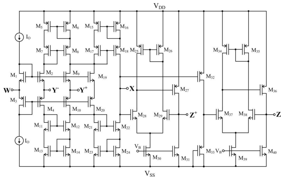
Fig. 2.4 CMOS Implementation Of UVC [2]
