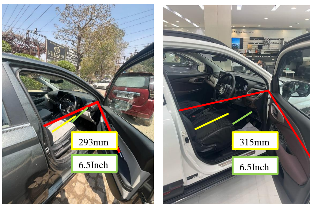
Figure 64: Door Opening Angle (Red), Thigh Support (Yellow), Seat adjustment range (Green) for Fronx and I20
