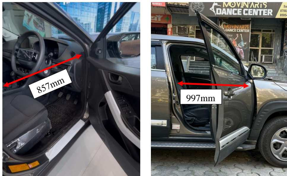
Figure 49: Door Opening for Brezza and Nexon
