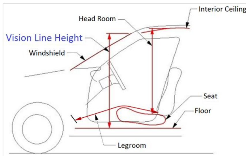
Figure 27: Vehicle clearance/room measurement
