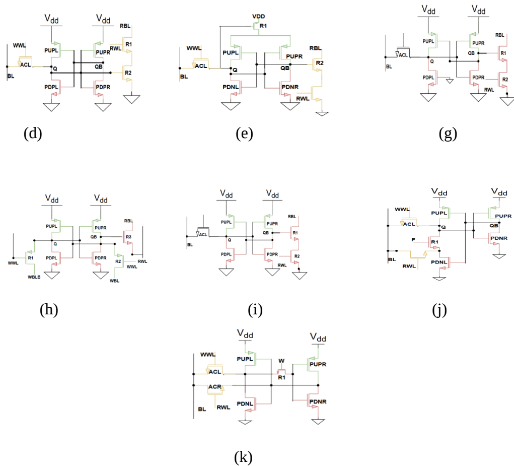
Fig. 3.1 Schematic Diagram For (a)7TDESPA, (b)7TDESPGi, (c)7TDEDP, (d)7TDESPC, (e)7TDESPD, (f)7TDESPGi, (g)7TDESPK, (h)7TDESPD, (i)7TDESPK, (j)7TDESPRt
