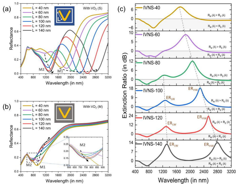
Fig. 6.2 Reflectance spectra obtained from an IVNS based plasmonic switch for different values of arm lengths of the VNSs placed on a gold coated \text{SiO}_2 substrate with \text{VO}_2 in its (a) semiconducting state and (b) metallic state. (c) Extinction ratio spectra for the IVNS based plasmonic switch for different values of arm lengths of the VNSs placed on a \text{VO}_2 coated gold \text{SiO}_2 substrate. The thickness of the \text{VO}_2 film ( t ), width of VNS ( W ), height of VNS ( H ), angle between two arms of VNS ( \theta ), and gap ( G ) between adjacent VNSs is taken to be 100 nm, 20 nm, 50 nm, 60^\circ , and 30 nm, respectively. The arm length of VNS ( L ) is varied from 40 nm to 140 nm.
