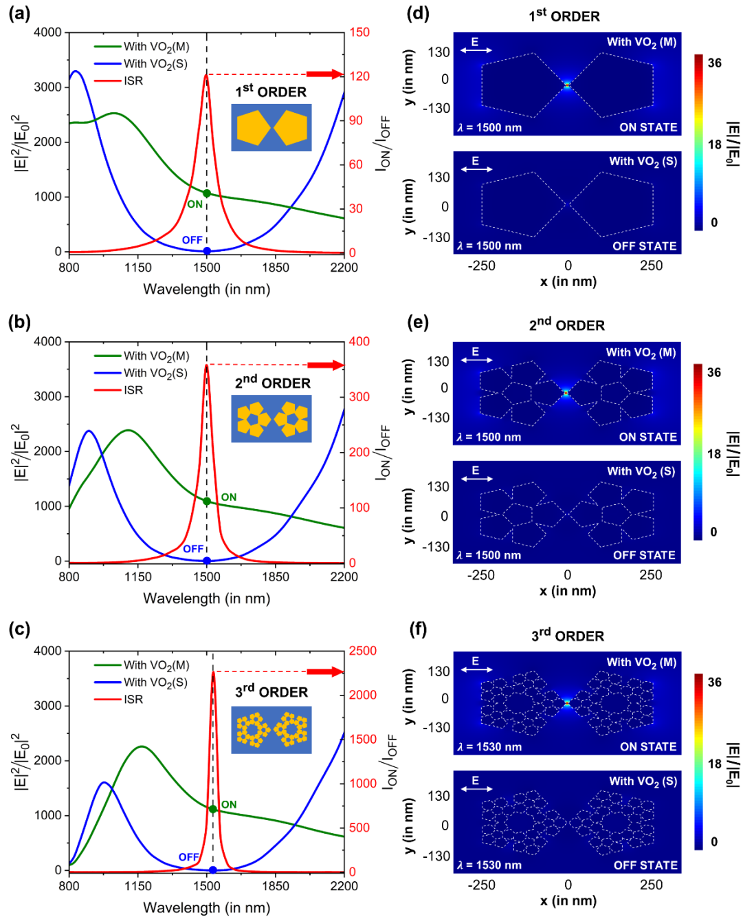
Fig. 7.2 Effect of fractalization of pentagon shaped plasmonic nanoantennas. Intensity enhancement spectra for VO 2 (M) and VO 2 (S), and ISR spectra of the plasmonic switches with pentagon shaped fractals for (a) 1 st order, (b) 2 nd order, and (c) 3 rd order. Electric-field profiles of the plasmonic switches with pentagon shaped fractals for (d) 1 st order, (e) 2 nd order, and (f) 3 rd order. The length of the pentagon segment ' L ', the height of the pentagon segment ' H ', the gap between the pentagon segments ' G ', and the thickness of VO 2 layer ' T ' are considered to be 250 nm, 150 nm, 5 nm, and 150 nm, respectively.
