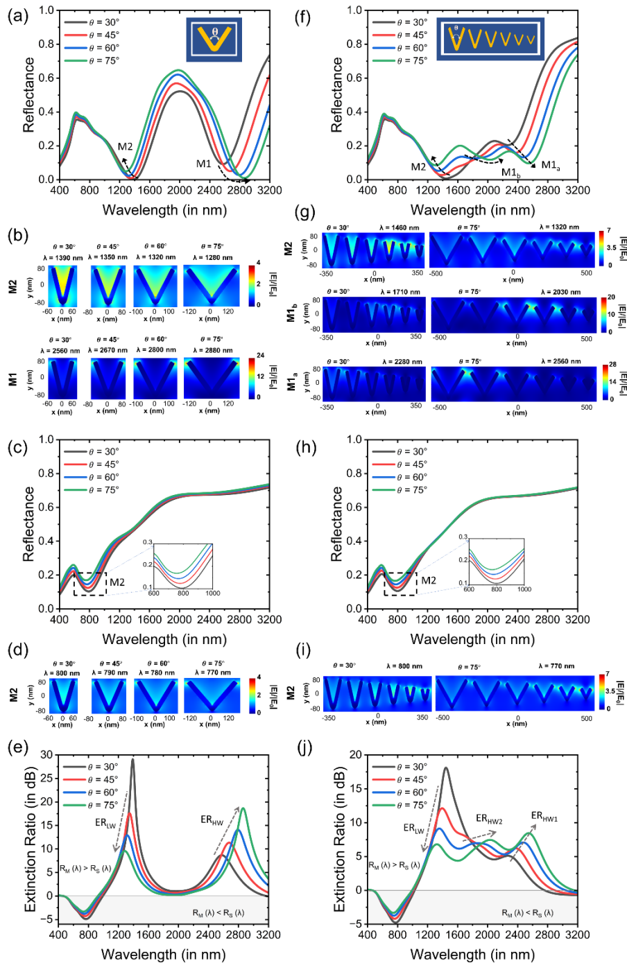
Fig. 6.7 Effect of varying the angle between two arms of VNS ( \theta ) of an IVNS-140 based switch on the (a) Reflectance spectra and (b) E-field profiles for Mode M1 and M2, with \text{VO}_2 in its semiconducting state; (c) Reflectance spectra and (d) E-field profiles for Mode M2, with \text{VO}_2 in its metallic state; and (e) Extinction ratio spectra. Effect of varying the angle between two arms of VNS ( \theta ) of a VVNS-140-120-100-80-60-40 based switch on the (f) Reflectance spectra and (g) E-field profiles for Mode M1 a , M1 b and M2, with \text{VO}_2 in its semiconducting state; (h) Reflectance spectra and (i) E-field profiles for Mode M2, with \text{VO}_2 in its metallic state; and (j) Extinction ratio spectra. The thickness of \text{VO}_2 film ( t ), width of VNSs ( W ), height of VNSs ( H ), and gap ( G ) between adjacent VNSs is taken to be 100 nm, 20 nm, 50 nm, and 30 nm, respectively.
