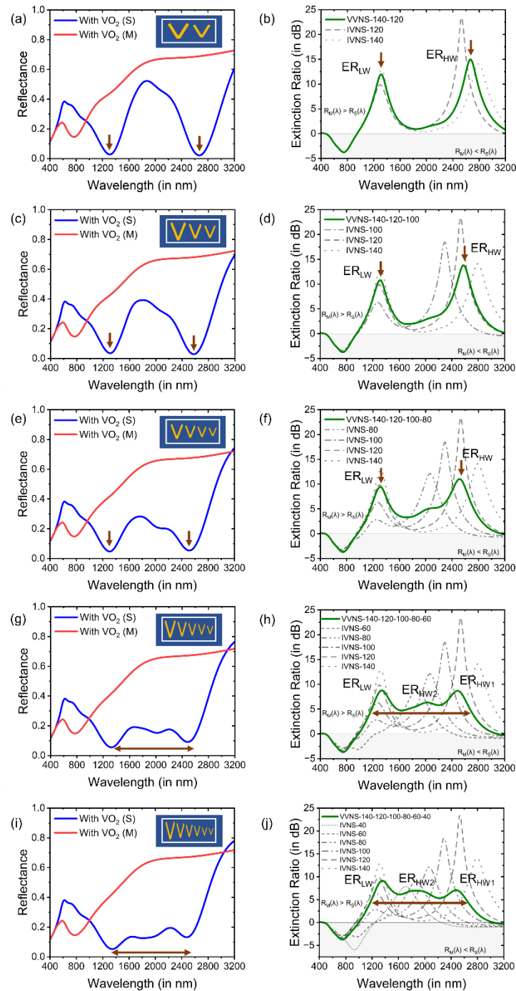
Fig. 6.3 (a) Reflection spectra with VO 2 (M) and VO 2 (S), and (b) Extinction ratio spectra for a VVNS-140-120 based plasmonic switch. (c) Reflection spectra with VO 2 (M) and VO 2 (S), and (d) Extinction ratio spectra for a VVNS-140-120-100 based plasmonic switch. (e) Reflection spectra with VO 2 (M) and VO 2 (S), and (f) Extinction ratio spectra for a VVNS-140-120-100-80 based plasmonic switch. (g) Reflection spectra with VO 2 (M) and VO 2 (S), and (h) Extinction ratio spectra for a VVNS-140-120-100-80-60 based plasmonic switch. (i) Reflection spectra with VO 2 (M) and VO 2 (S), and (j) Extinction ratio spectra for a VVNS-140-120-100-80-60-40 based plasmonic switch. The thickness of the VO 2 film ( t ), width of VNSs ( W ), height of VNSs ( H ), angle between two arms of VNSs ( \theta ), and gap ( G ) between adjacent VNSs is taken to be 100 nm, 20 nm, 50 nm, 60°, and 30 nm, respectively.
