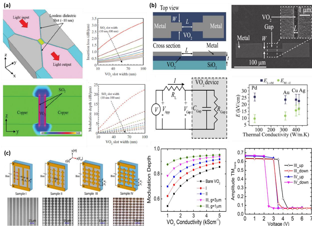
Fig. 2.16 Electrically activated VO 2 based plasmonic switches. (a) 3D view of a VO 2 based plasmonic dual-mode waveguide electroabsorption modulator, E-field mapping of surface plasmons in the Cu-SiO 2 -VO 2 -Cu slot during the ON state, and variations in insertion loss and modulation depth with respect to VO 2 and SiO 2 slot widths [130]. (b) Top and cross-section view of a VO 2 based lateral nano-junction, SEM image of the device, simplified circuit model of the device, and electric field distribution at the onset of phase transitions as a function of thermal conductivity of the contact metals [131]. (c) Design of the electrically driven hybrid bowtie antenna-VO 2 devices; modulation depth characterization at 1 THz for bare VO 2 , sample I, sample II and sample III; and electrical characterizations at 1 THz for sample III and sample IV [132].
