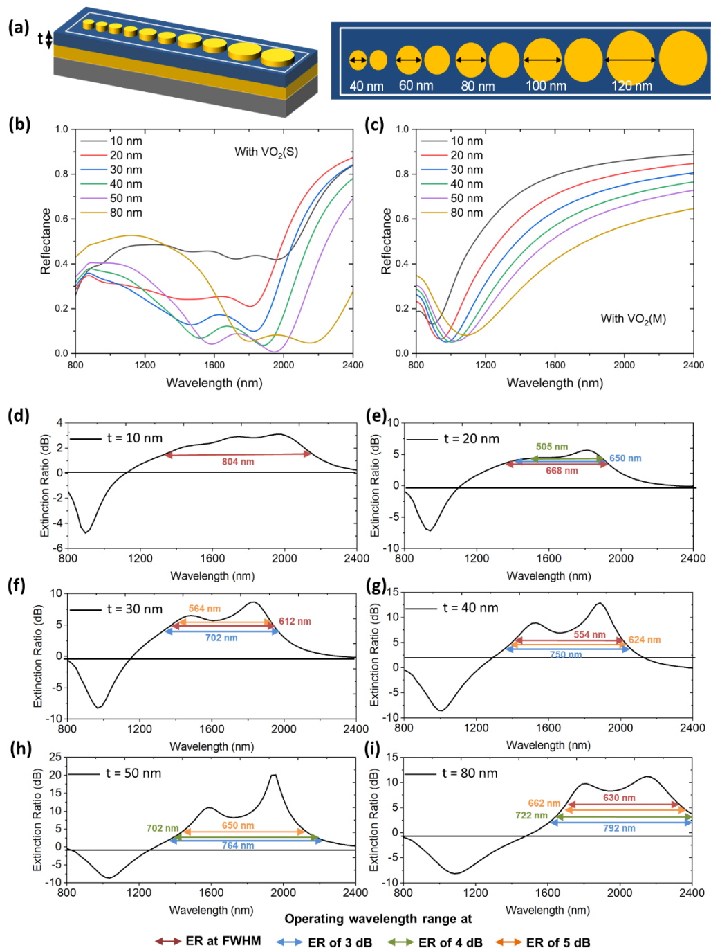
Fig. 4.11 (a) Schematic showing the periodic array of five sets of nanodisc-dimers on a VO 2 -coated plasmonic film with the diameters of the nanodisc-dimers being D 1 (40 nm), D 2 (60 nm), D 3 (80 nm), D 4 (100 nm) and D 5 (120 nm). Reflectance spectra of NDD-40-60-80-100-120 showing the effect of increasing the thickness of VO 2 , ' t ', from 10 nm to 80 nm when VO 2 is in its (b) semiconductor phase, and (c) metallic phase. Extinction ratio (ER) spectra showing the operating wavelength ranges for an ER of 3 dB, 4 dB, 5 dB and at the FWHM of the ER when the thickness of VO 2 , ' t ', is (d) 10 nm (e) 20 nm (f) 30 nm (g) 40 nm (h) 50 nm, and (i) 80 nm. The height of the nanodiscs, ' h ', and the gap between the nanodiscs, ' g ', were kept constant at 50 nm, and 5 nm, respectively, for all the above cases.
