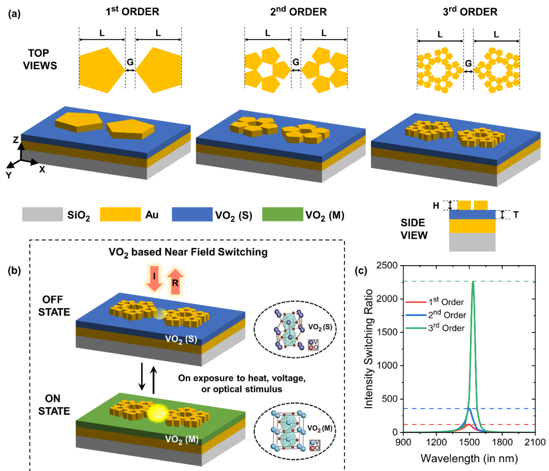
Fig. 7.1 (a) Schematics of 1 st order, 2 nd order, and 3 rd order fractalized pentagon shaped plasmonic nanoantennas on gold-coated \text{SiO}_2 substrate with \text{VO}_2 layer as a spacer between the nanoantennas and the underlying substrate. The geometrical parameters like the length of pentagon segment ' L ', the height of pentagon segment ' H ', the gap between the two pentagon segments ' G ', and the thickness of \text{VO}_2 layer ' T ' are also shown. (b) Illustration of near-field switching mechanism based on the phase transformation of \text{VO}_2 . (c) Intensity switching ratio spectra for all the three orders of the proposed plasmonic switches based on pentagon shaped fractal plasmonic nanoantennas.
