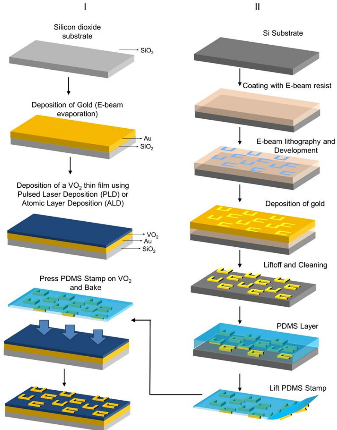
Fig. 5.12 Fabrication methodology to fabricate the proposed VO 2 based polarization-independent dual-wavelength U-C type plasmonic switch using a periodic combination of U and C shaped gold nanopillars on a gold coated SiO 2 substrate with a thin film of VO 2 as a spacer between the nanostructures and the underlying plasmonic substrate.
