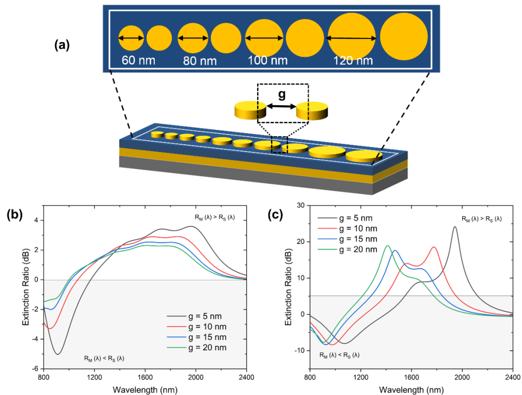
Fig. 4.12 (a) Schematic showing the periodic array of four sets of nanodisc-dimers on a VO 2 -coated plasmonic film with the diameters of the nanodisc-dimers being D 1 (60 nm), D 2 (80 nm), D 3 (100 nm) and D 4 (120 nm). Extinction ratio (ER) spectra for the proposed switch showing the effect of varying the gap, 'g', between the nanodiscs from 5 nm to 20 nm, when the thickness of VO 2 , 't', is (b) 10 nm, and (c) 50 nm. The height of the nanodiscs, 'h', is kept constant at 50 nm for both the cases.
