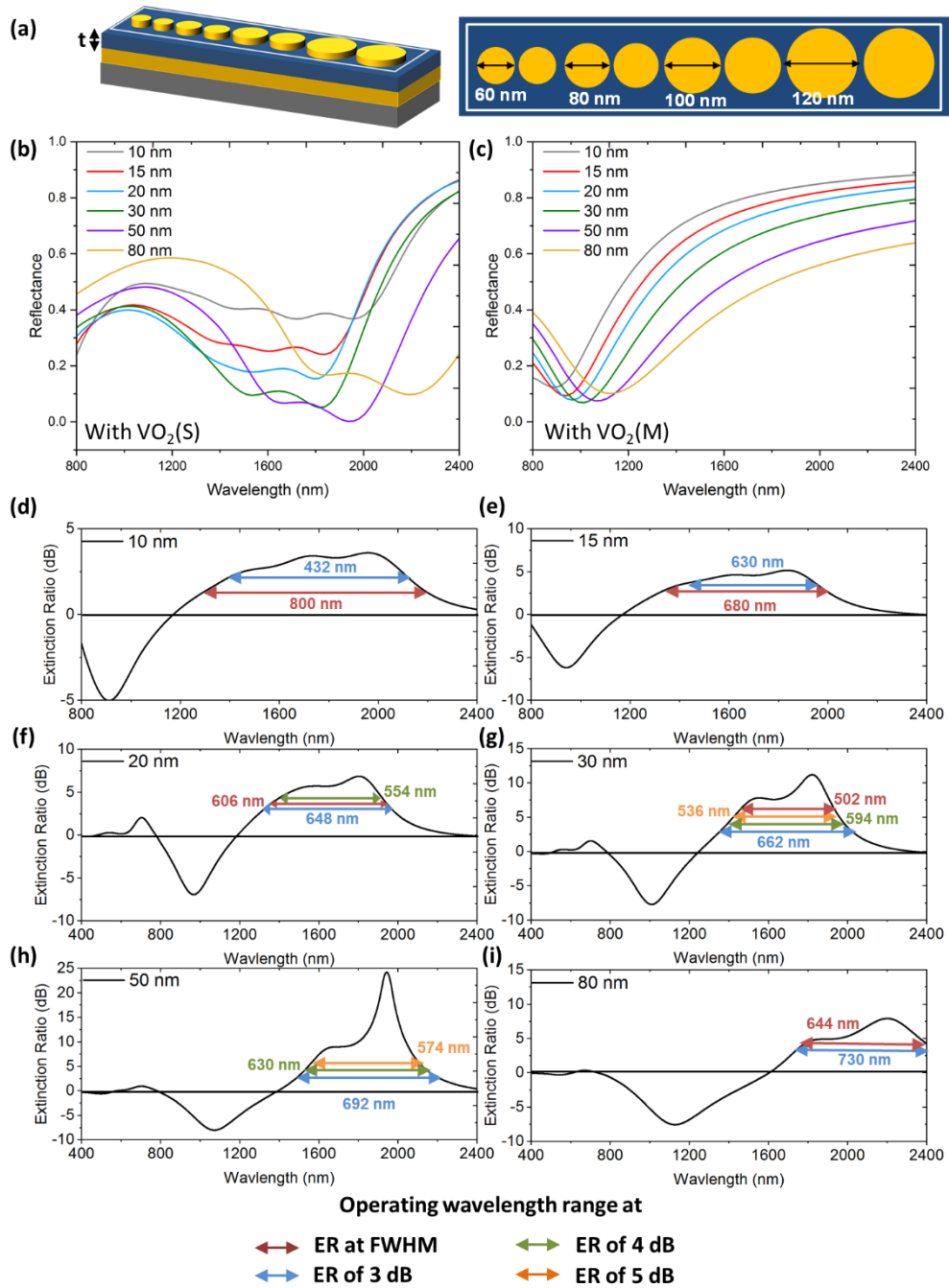
Fig. 4.6 (a) Schematic showing the periodic array of four sets of nanodisc-dimers on a \text{VO}_2 coated plasmonic film with the diameters of the nanodisc-dimers being D_1 (60 nm), D_2 (80 nm), D_3 (100 nm) and D_4 (120 nm). Reflectance spectra of the periodic array of four sets of nanodisc-dimers showing the effect of increasing the thickness of \text{VO}_2 , ' t ', from 10 nm to 80 nm when \text{VO}_2 is in its (b) semiconductor phase and (c) metallic phase. Extinction ratio (ER) spectra showing the operating wavelength range for an ER of 3 dB, 4 dB, 5 dB and for the FWHM of the maximum ER when the thickness of \text{VO}_2 , ' t ', is (d) 10 nm (e) 15 nm (f) 20 nm (g) 30 nm (h) 50 nm and (i) 80 nm. The height of the nanodiscs, ' h ', and the gap between the nanodiscs, ' g ', were kept constant at 50 nm, and 5 nm, respectively, for all the above cases.
