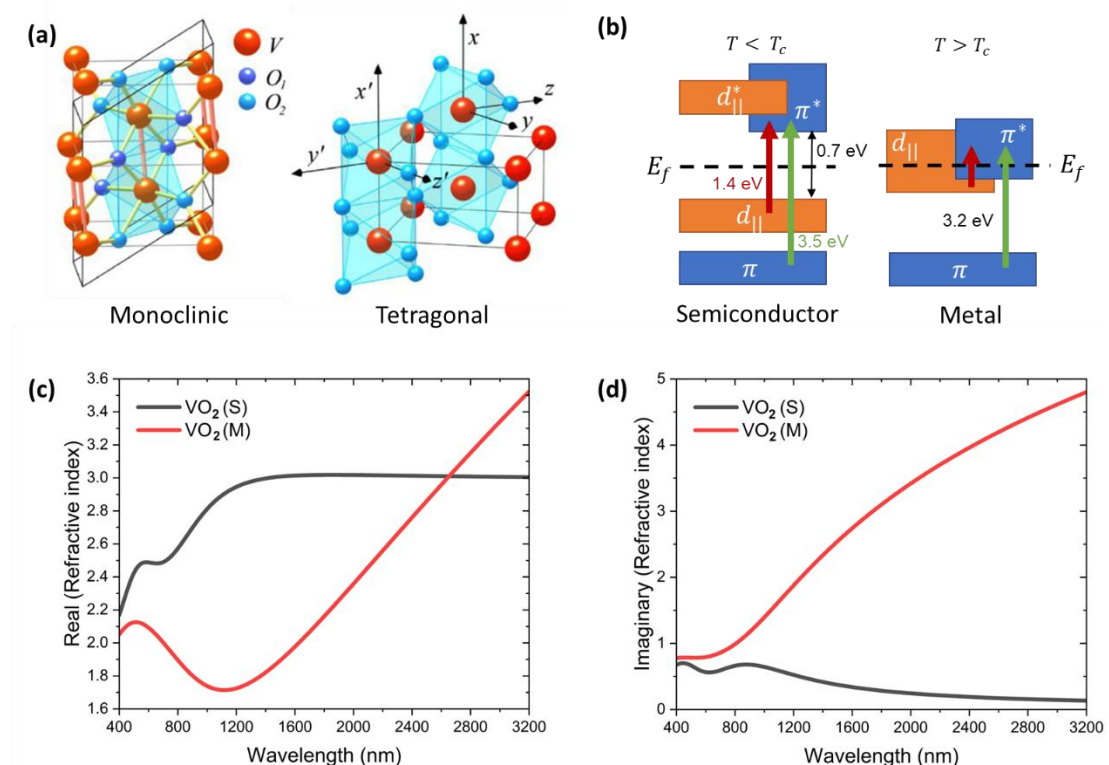
Fig. 2.4 (a) Crystal structures of VO_2 when it is in its monoclinic semiconducting phase and tetragonal metallic phase [68]. (b) Band structure for the monoclinic semiconducting phase and tetragonal metallic phase of VO_2 . (c, d) Real and imaginary parts of the complex refractive index of VO_2 in its monoclinic semiconducting phase ( VO_2(S) ) and tetragonal metallic phase ( VO_2(M) ), respectively.
