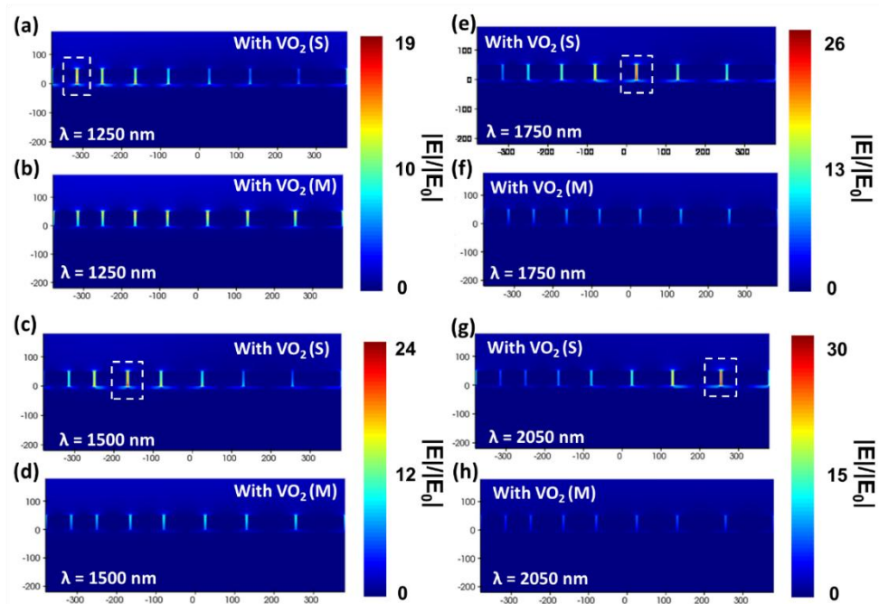
Fig. 4.7 E-field profile for the side view of the periodic array of a set of four nanodisc-dimers at a wavelength of (a, b) 1250 nm, (c, d) 1500 nm, (e, f) 1750 nm, and (g, h) 2050 nm with VO 2 in its semiconductor phase and metallic phase, respectively. The diameters of the set of four nanodisc-dimers are taken as D 1 (60 nm), D 2 (80 nm), D 3 (100 nm) and D 4 (120 nm), respectively. The thickness of VO 2 , 't', the height of the nanodiscs, 'h', and the gap between the nanodiscs, 'g', were kept constant at 10 nm, 50 nm, and 5 nm, respectively.
