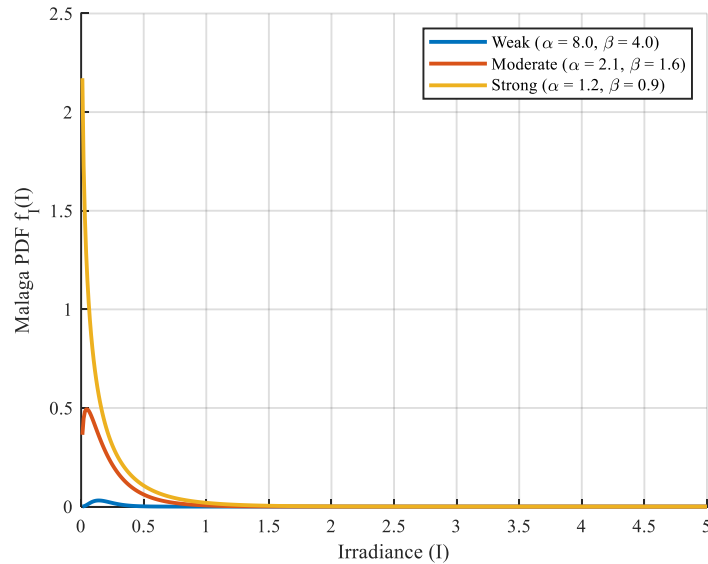
Figure 4.3 PDF of Málaga distribution under different turbulence conditions
