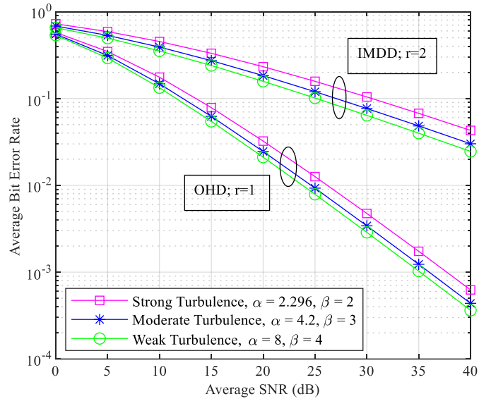
Figure 4.5 Average BER vs average SNR operated under both detection schemes for various turbulence conditions
