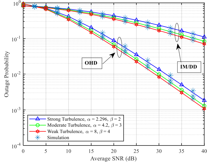
Figure 4.12 Outage probability vs average SNR for various turbulence conditions under fixed pointing condition operated under both detection schemes
