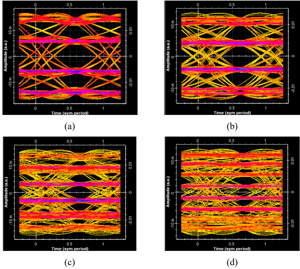
Figure I-2 Eye diagrams of received QAM symbols in a MIMO UOWC system under GG turbulence. (a) 8-QAM (b) 16-QAM (c) 32-QAM and (d) 64-QAM
