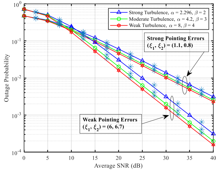
Figure 4.13 Outage probability vs average SNR for various turbulence conditions operated under variable pointing errors
