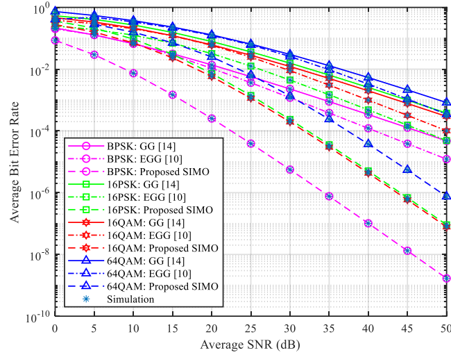
Figure 3.9 Average BER comparison of the proposed model with existing models for various modulation schemes
