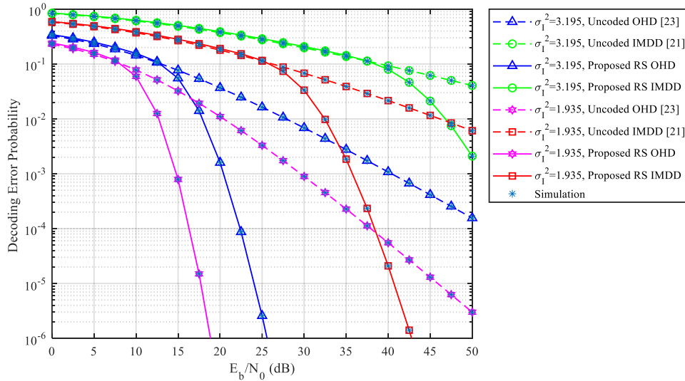
Figure 5.4 DEP using both types of detection techniques under strong and moderate turbulence conditions
