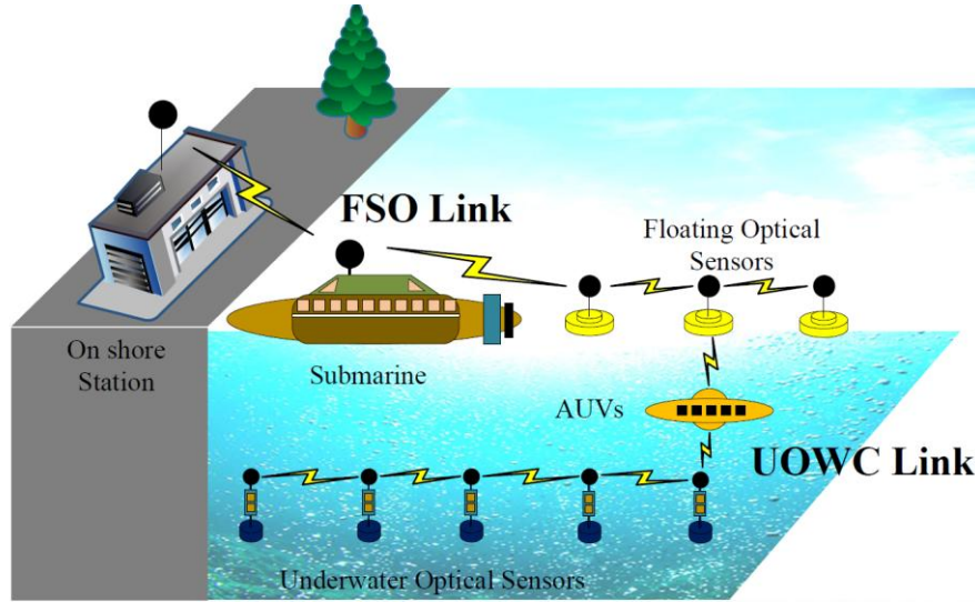
Figure 5.1 FSO and UOWC links in underwater communication
