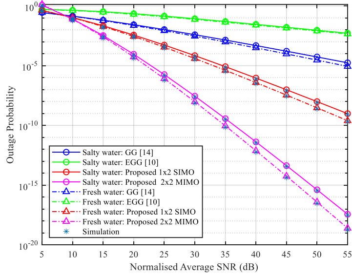
Figure 3.7 Outage probability comparison of proposed model with existing models operated under salty and fresh water for thermally uniform UOWC channel
