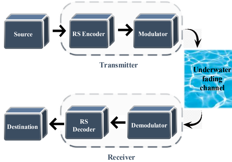
Figure 5.3 Block diagram of RS coded UOWC system
