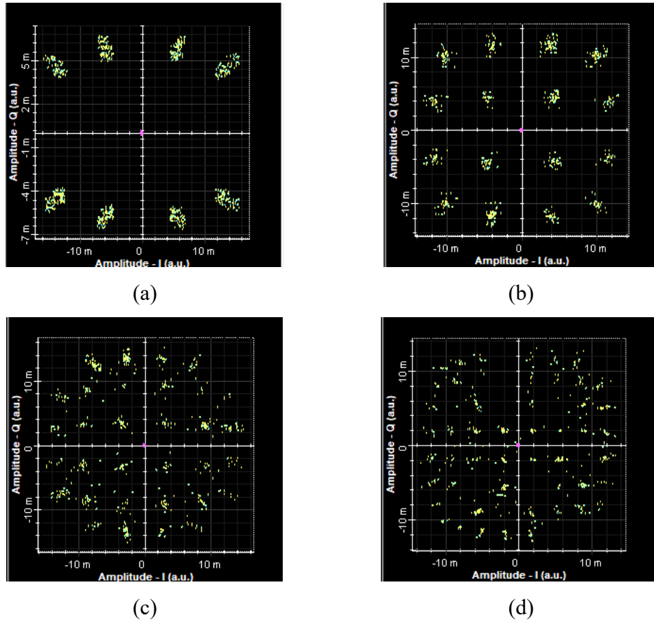
Figure I-1 Constellation diagrams of received QAM symbols in an UOWC system under GG turbulence. (a) 8 QAM (b) 16 QAM (c) 32 QAM and (d) 64 QAM
