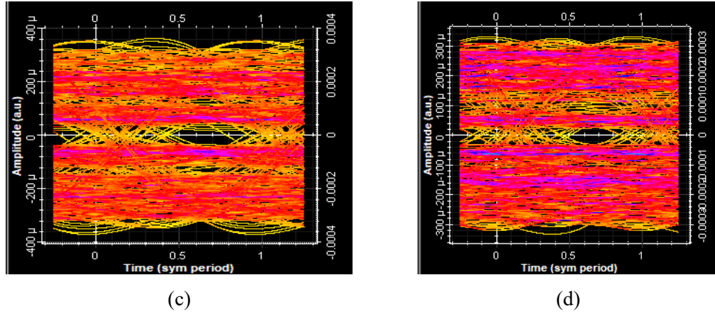
Figure I-4: Eye diagrams of received QAM symbols in an UOWC system under dual hop relaying scheme. (a) 8-QAM (b) 16-QAM (c) 32-QAM and (d) 64-QAM
