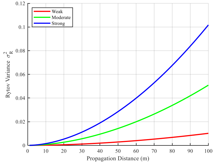
Figure 3.1 Variation of Rytov variance versus propagating distance
