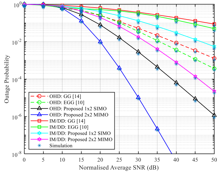
Figure 3.6 Outage probability versus normalized average SNR for strong turbulence condition operated under optical heterodyne detection
