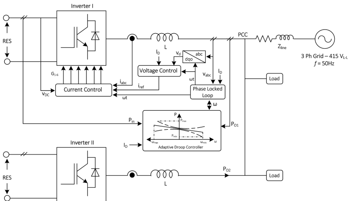
Fig. 6.1 System Configuration
