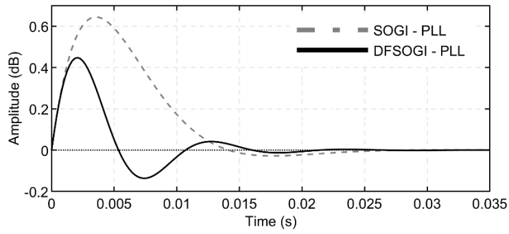
Fig. 5.7 Bode Plot of DFSOGI – PLL and SOGI – PLL
