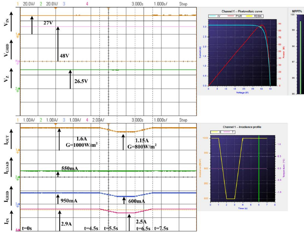
Fig 3.12 a) i) Input Voltage ( V_{IN} ) ii) Grid Voltage ( V_G ) iii) Capacitor Voltage ( V_Z ) b) i) Output Current ( I_{OUT} ) ii) Load Current iii) Grid Current iv) Input Current ( I_{IN} ) for irradiation change (Weak grid)
