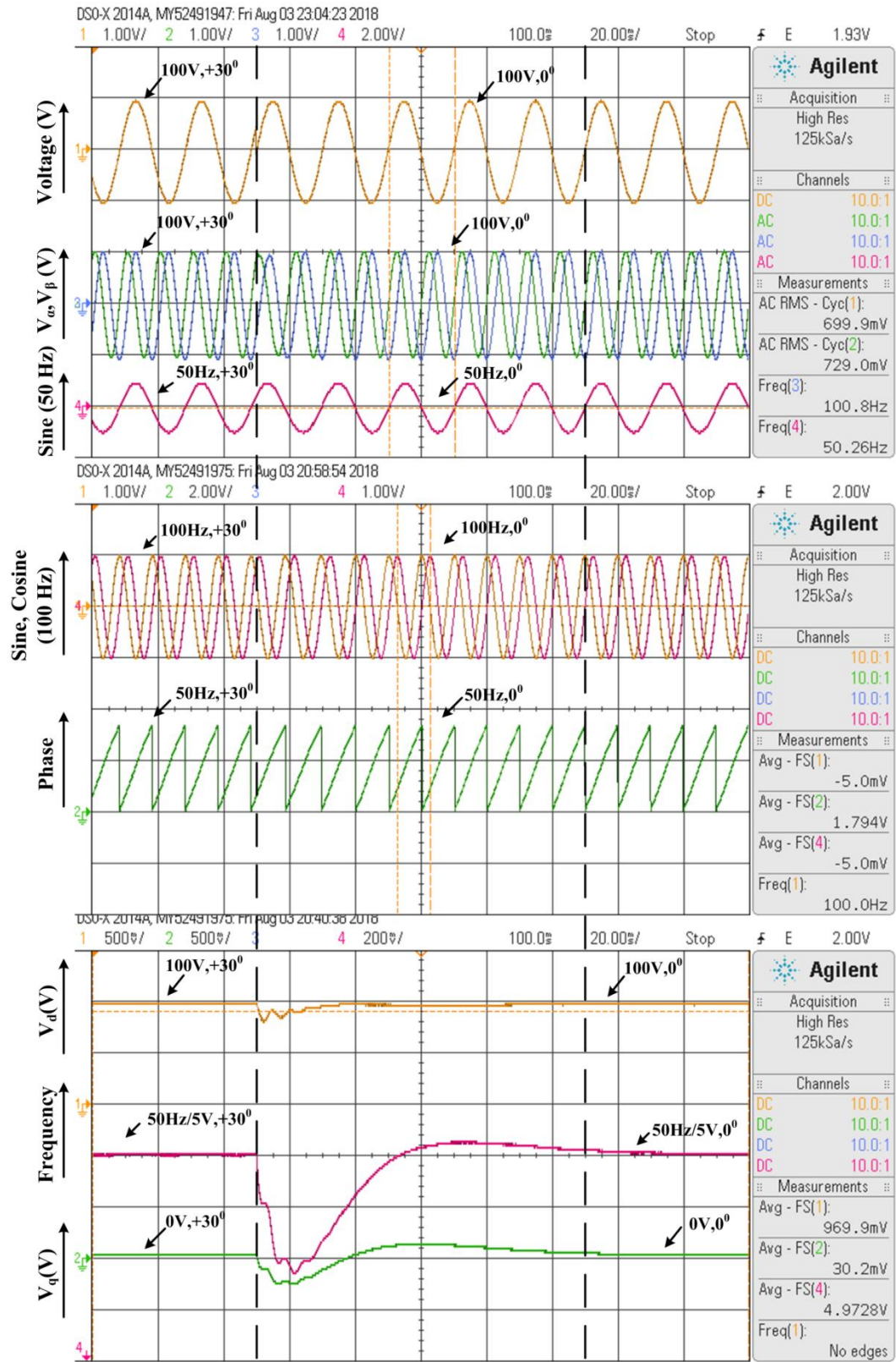
Fig. 5.13 Zoomed ( t = 1.5s ) – Response – Phase Change a) i) input voltage ( V_{IN} ) ii) v_a and v_b iii) sine reference (50 Hz) b) i) sine and cosine reference (100Hz) ii) phase c) i) frequency iv) v_d v) v_q
