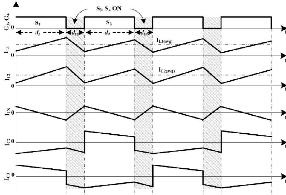
Fig 4.4.3 Charging Mode
