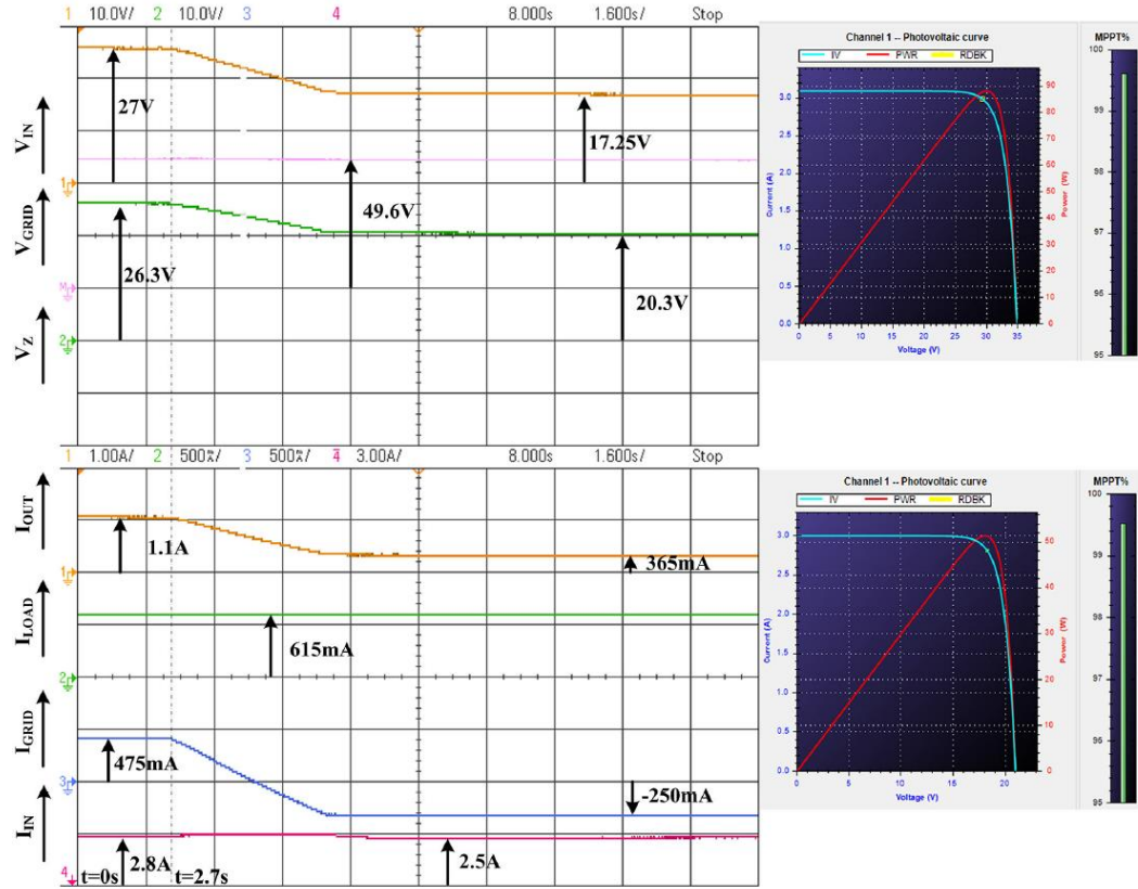
Fig 3.13. a) i) Input Voltage ( V_{IN} ) ii) Grid Voltage ( V_G ) iii) Capacitor Voltage ( V_Z ) b) i) Output Current ( I_{OUT} ) ii) Load Current iii) Grid Current iv) Input Current ( I_{IN} ) for partial shading (27V to 18V)
