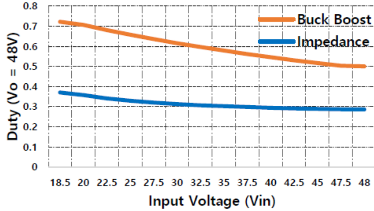
Fig. 4.18 Performance comparison conventional buck boost converter and impedance converter
