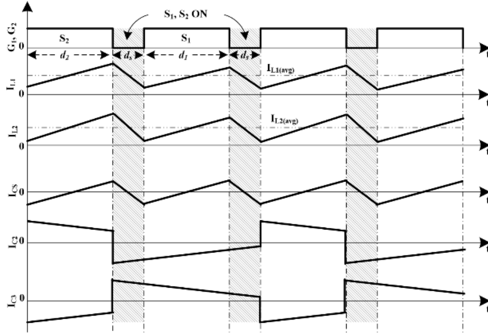
Fig 4.4.2 Discharging Mode with Operating Duty > 0.5
