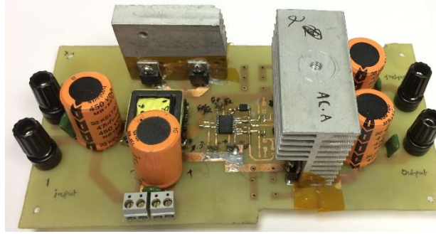
Fig 3.10 Hardware Prototype of Proposed Impedance Converter
