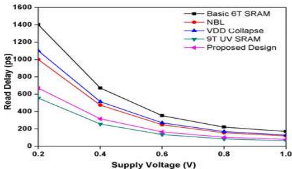
Figure 5.19. Variation of read delay vs supply voltage.
