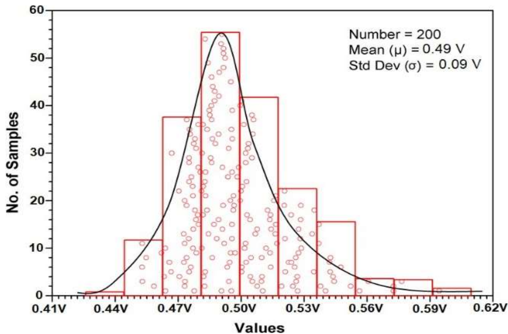
Figure 5.8. Monte Carlo of WSNM for proposed design.
