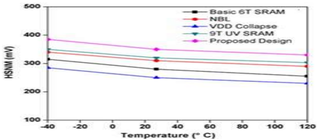
Figure 5.14. Variation of HSNM vs temperature.
