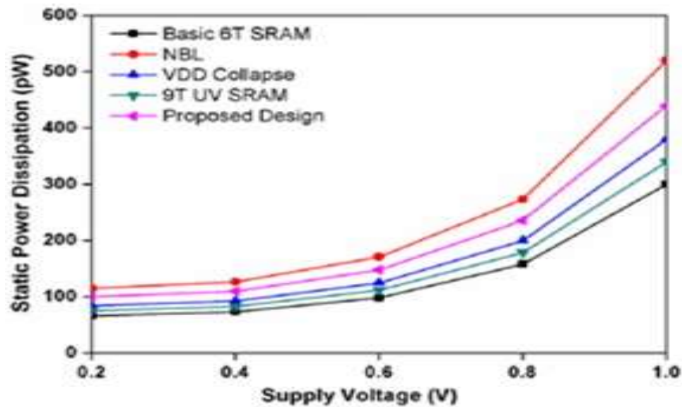
Figure 5.15. Static power dissipation at various VDD.
