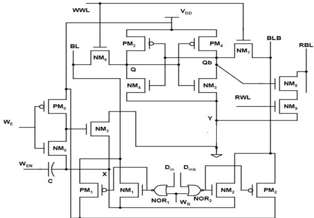
Figure 5.3. Proposed Design.
