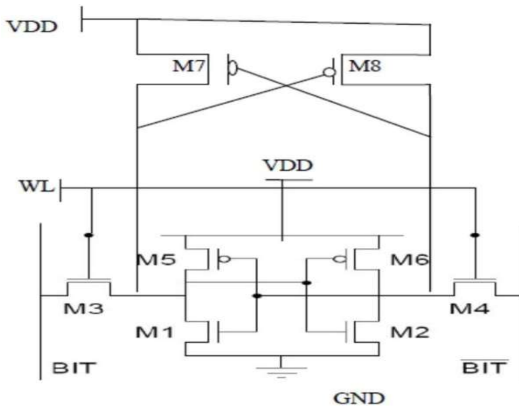
Figure 3.7. Proposed 8T SRAM cell with swing restoration inverter (W/L is in nanometers).
