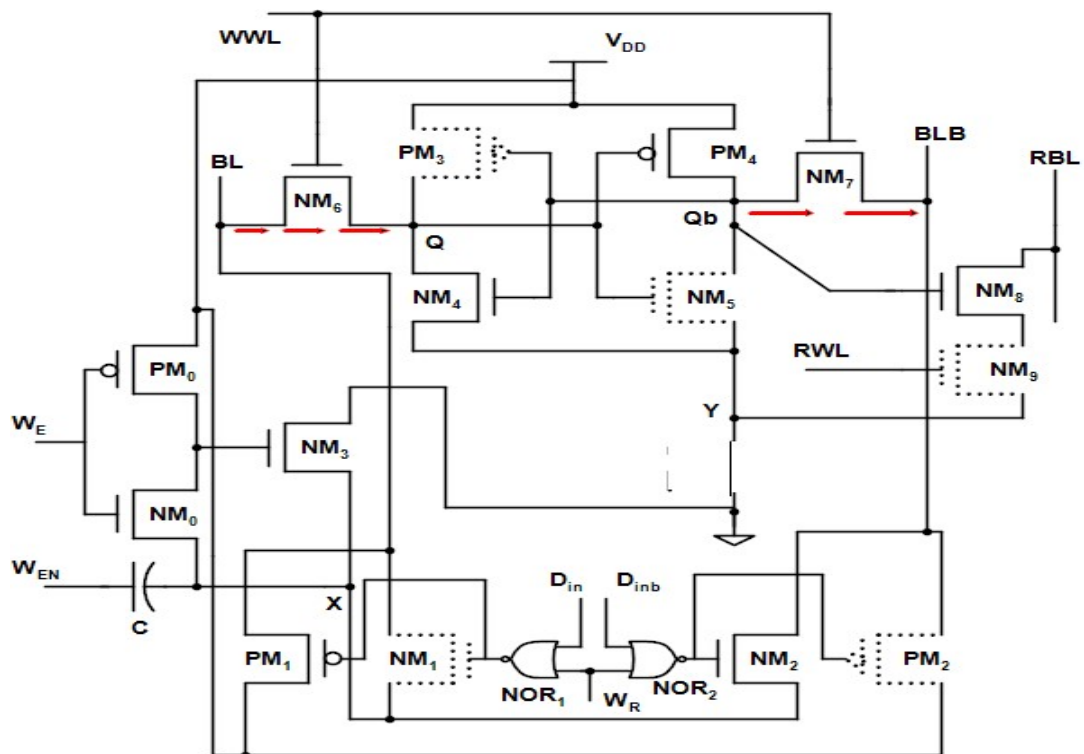
Figure 5.4(a). Proposed design during write operation.
