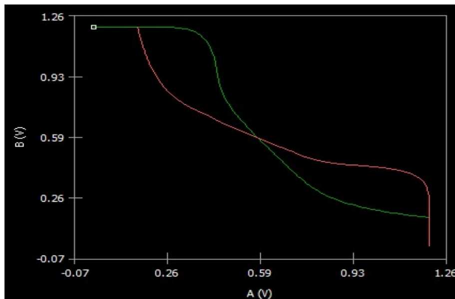
Figure 4.10. RSNM standard 8T SRAM cell.
