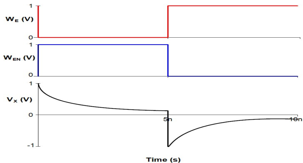
Figure 5.2(b). Output voltage at node X [127].
