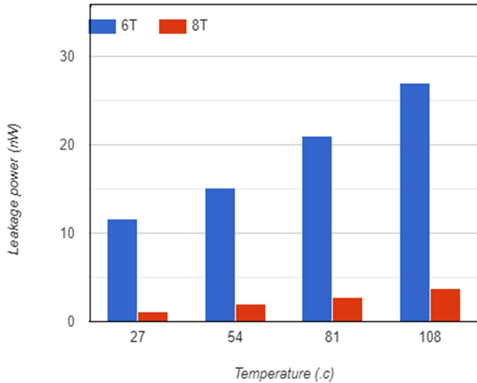
Figure 3.8. Temperature dependency of leakage power.
