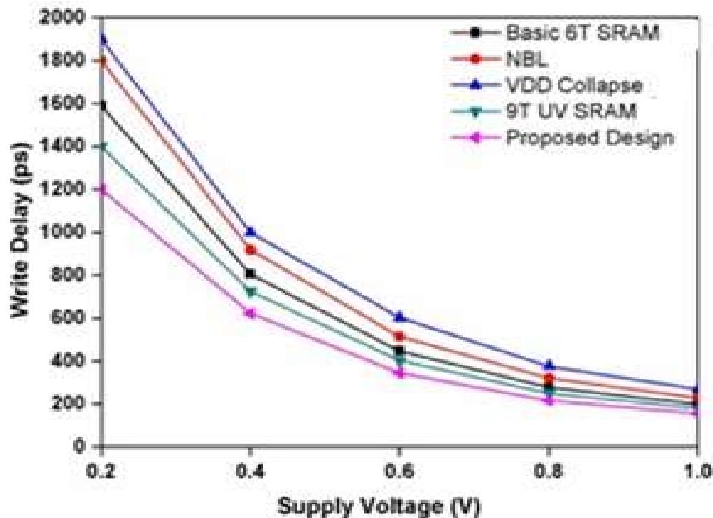
Figure 5.17. Variation of write delay vs supply voltage.
