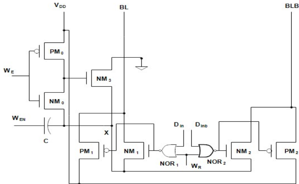
Figure 5.2(a). Circuit of negative bit line generator [127].
