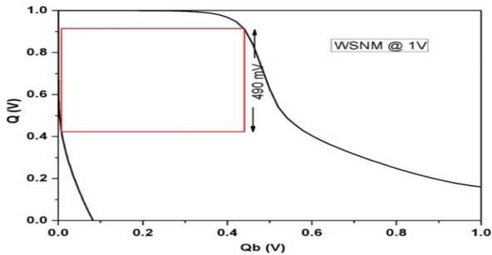
Figure 5.5. Butterfly curve for write stability.
