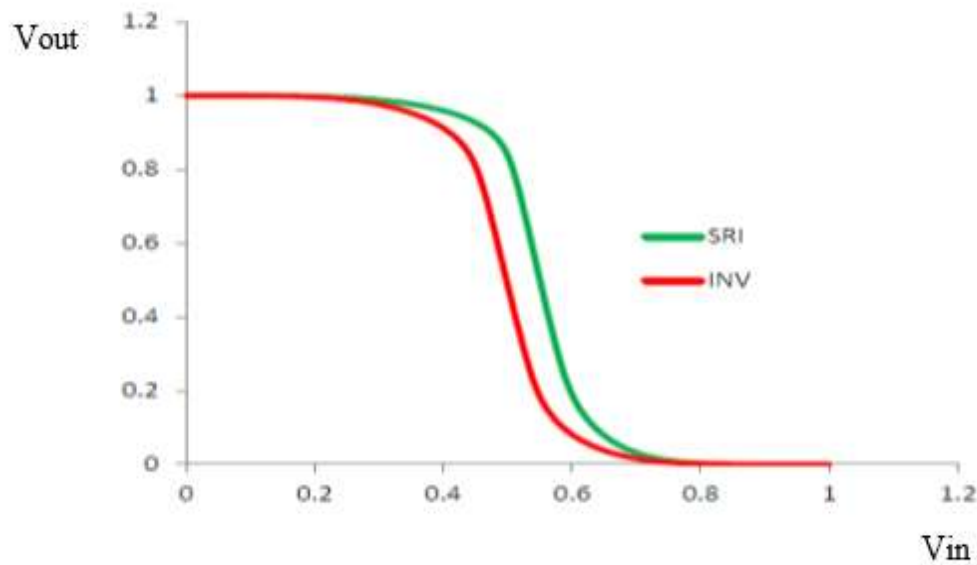
Figure 3.4. Inverter characteristics.
