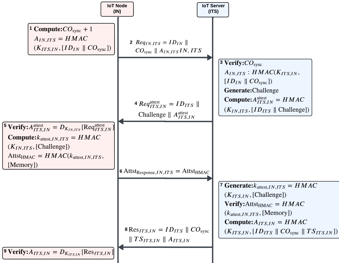
Figure 4.6: KFLIT: Attestation and time synchronization phase.
