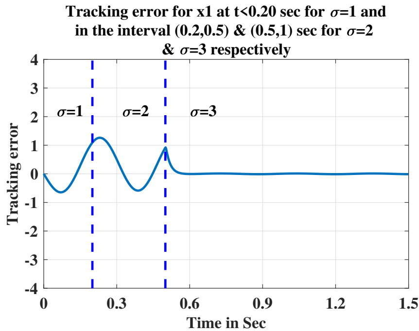
FIGURE 6.4: Tracking error for reference signal \sin(20t) .
