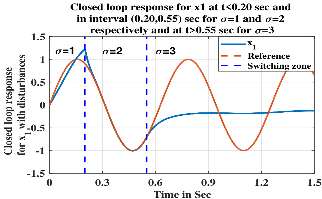
FIGURE 3.8: Closed loop response for Average dwell time not satisfying \tau_a > \frac{\ln \mu}{\beta^0} and doesn't track the reference signal \sin(10t)
