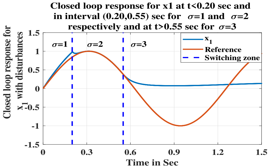
FIGURE 3.4: Closed loop response for Average dwell time not satisfying \tau_a > \frac{\ln \mu}{\beta_0} and doesn't track the reference signal \sin(5t)
