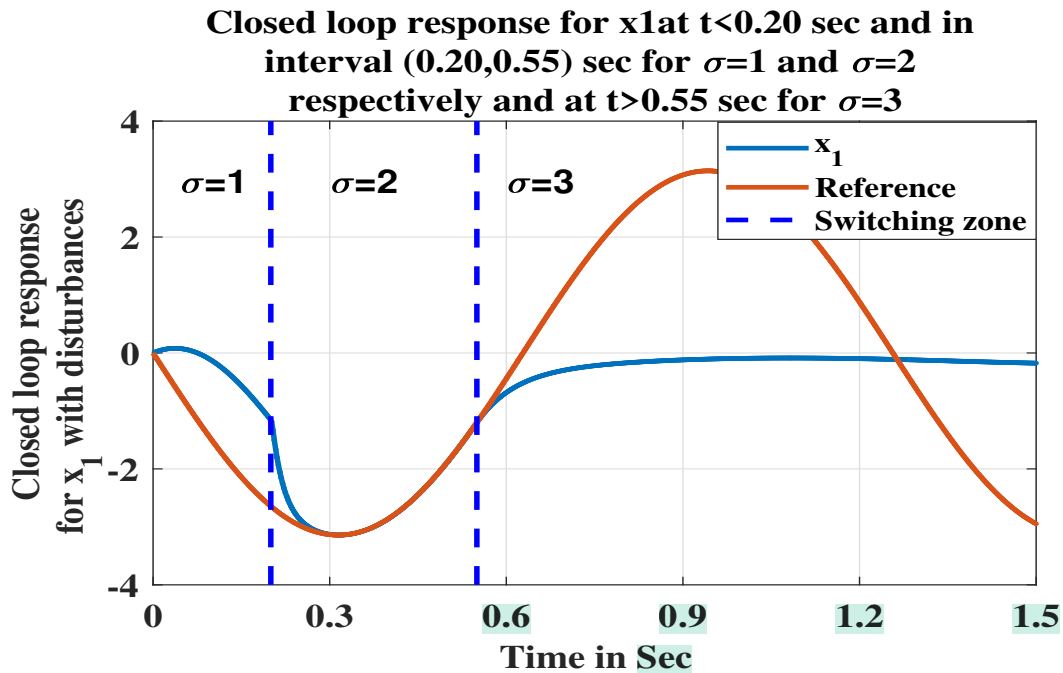
FIGURE 3.12: Closed loop response for Average dwell time not satisfying \tau_a > \frac{\ln l_\mu}{\beta^0} and doesn't track the reference signal \pi \sin(-5t)
