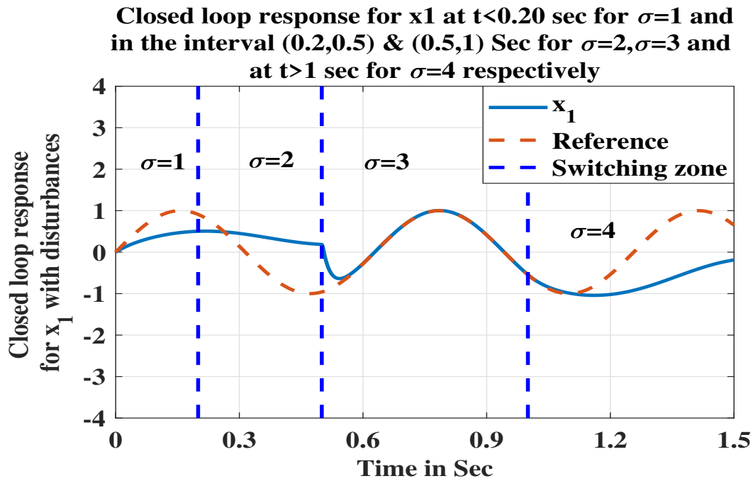
FIGURE 5.5: Closed loop response for \tau_a \neq \frac{\ln l_\mu}{\beta^o} and doesn't track the reference \sin(10t) .
