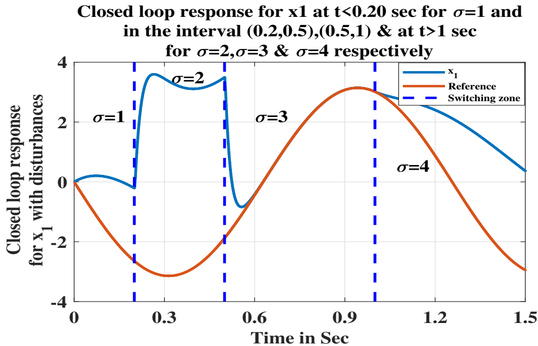
FIGURE 3.21: Closed loop response for Average dwell time not satisfying \tau_a > \frac{\ln l_u}{\beta^0} and doesn't track the reference signal \pi \sin(-5t) .
