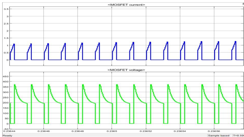
Fig.5. 7 Graph of voltage and current across switch
