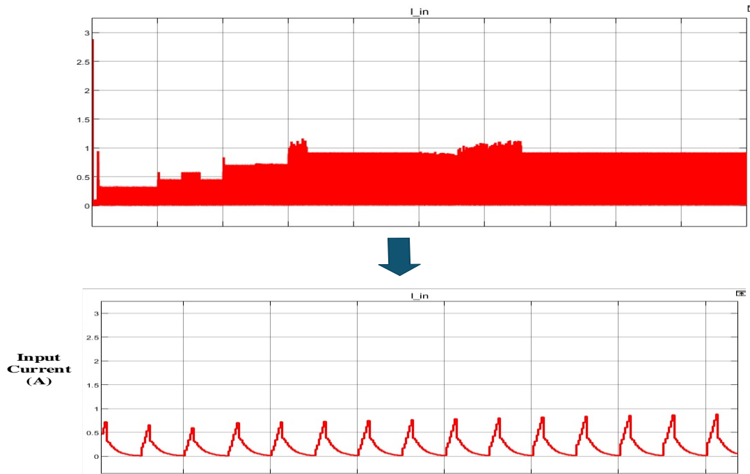
Fig.6. 2 Graph of Input Current
