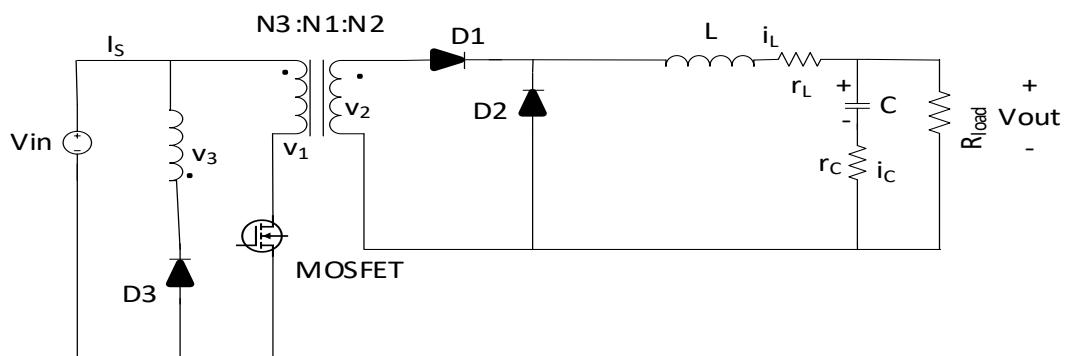
Fig.3. 2 schematic diagram of forward converter
