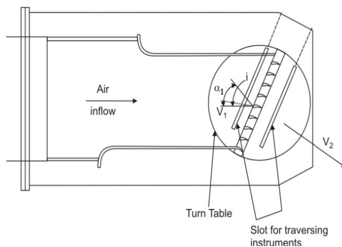
Figure 4.10: Wind tunnel for losses measurement for flow through turbomachine cascades
