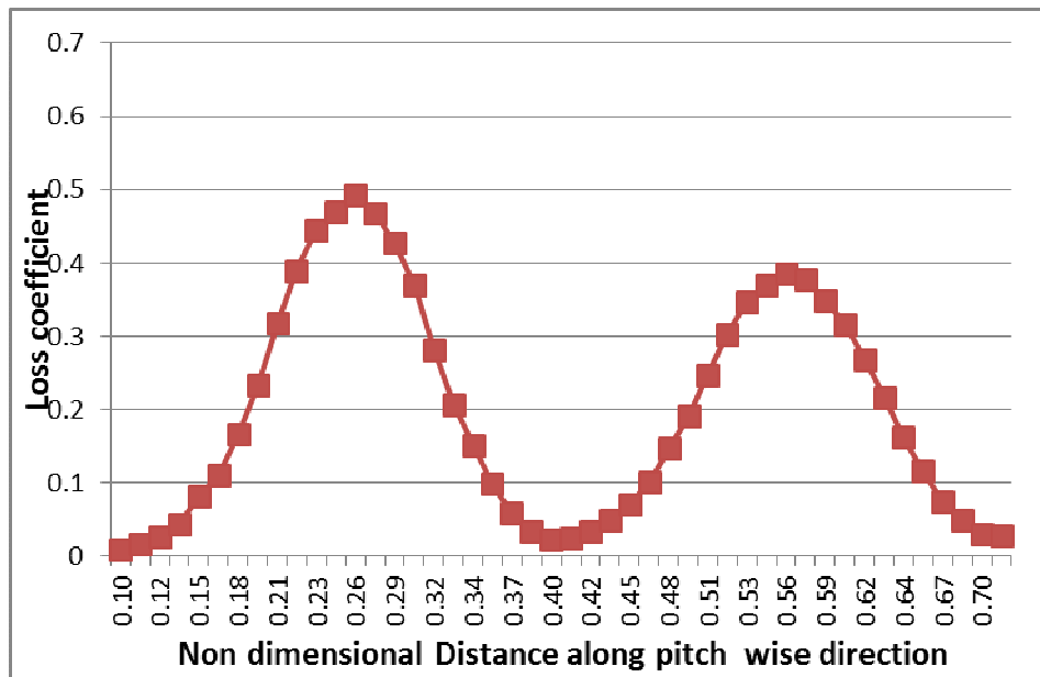
Figure 5.14: Variation of Local Loss Coefficients relative to the nondimensional distance in pitch wise direction, for the span position of 2mm from bottom wall
