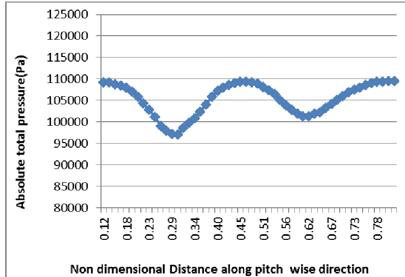
Figure 5.9: Variation of magnitude of absolute total pressure relative to the pitch wise direction, for the span position of 0 mm (at the lowest position of the blades i.e. at bottom wall)
