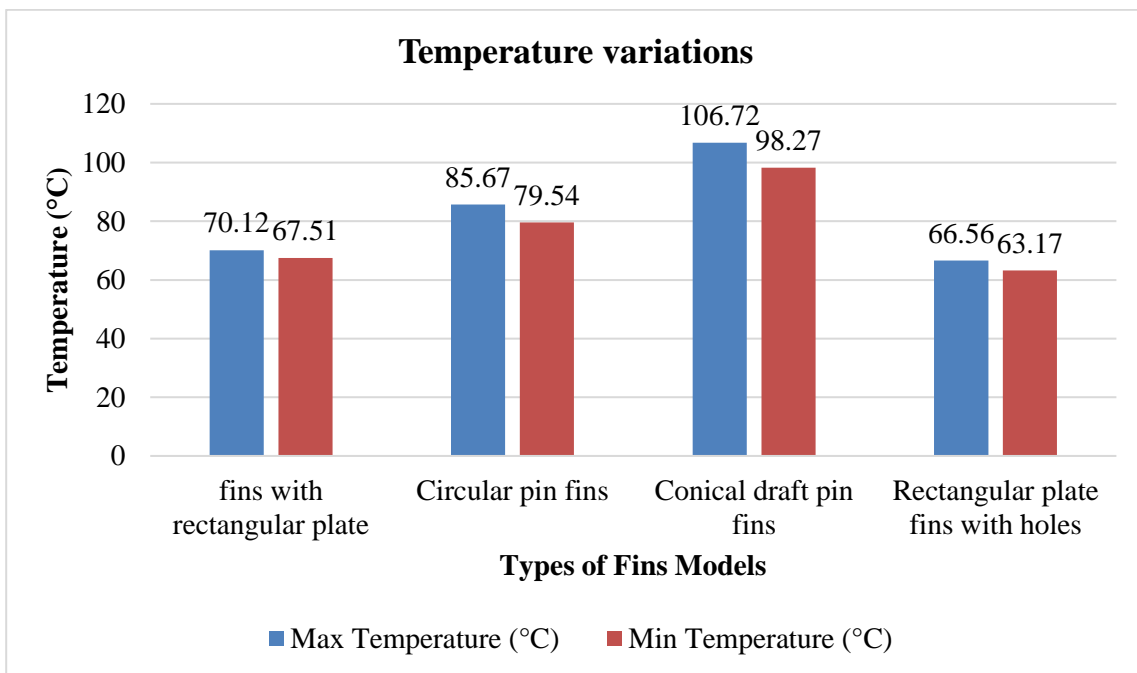
Figure 5.14: Maximum and Minimum Temperature found on Fin Models
