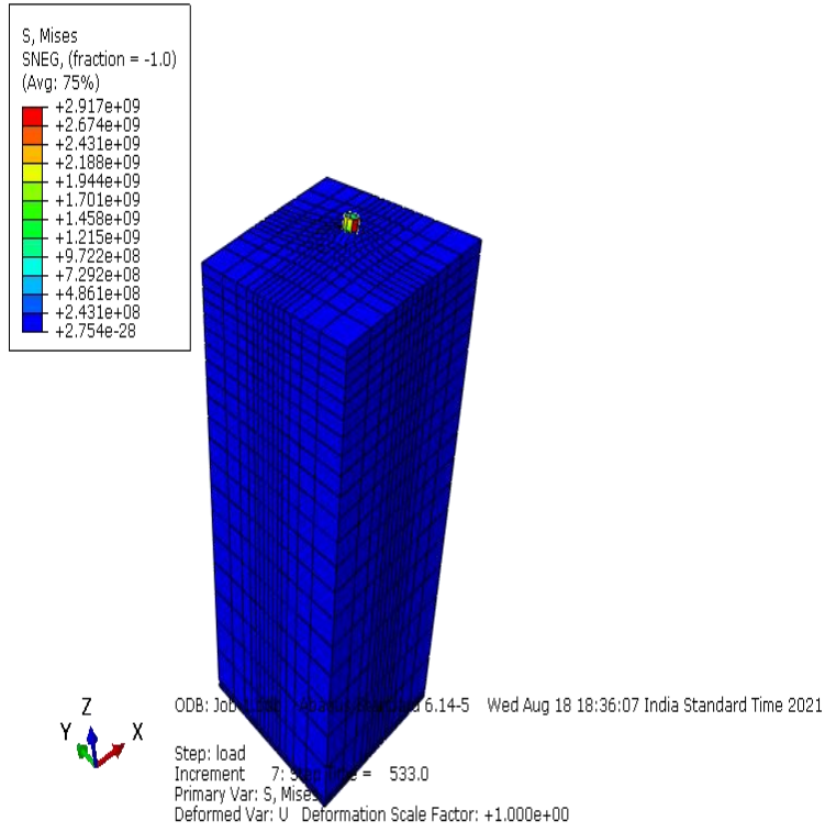
Figure 15- Stress variation in the pile of thickness 10mm
