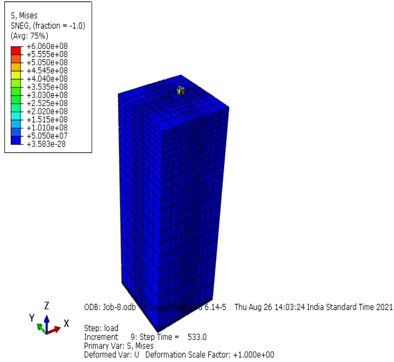
Figure 21- Stress variation in the pile of thickness 30mm
