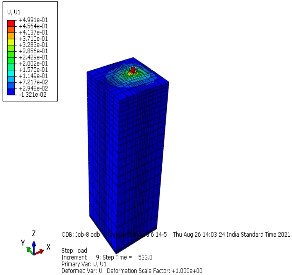
Figure 20- Displacement in the pile of thickness 30mm
