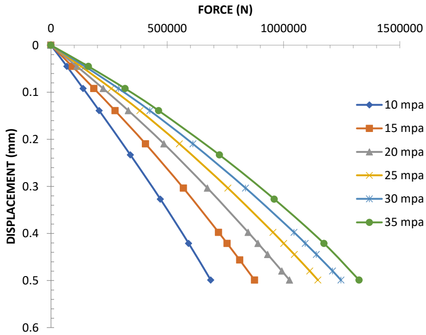
Figure 16- P-Y curve of pile 10mm thick for varying modulus of elasticity
