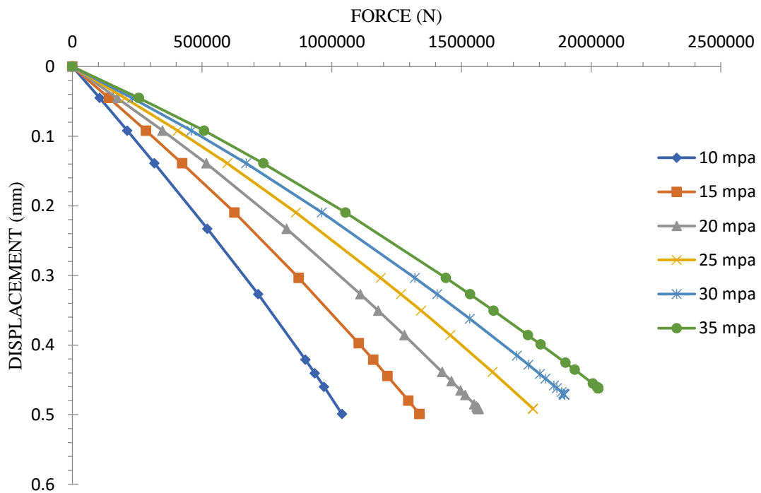
Figure 25- P-Y curve of pile 40mm thick for varying modulus of elasticity
