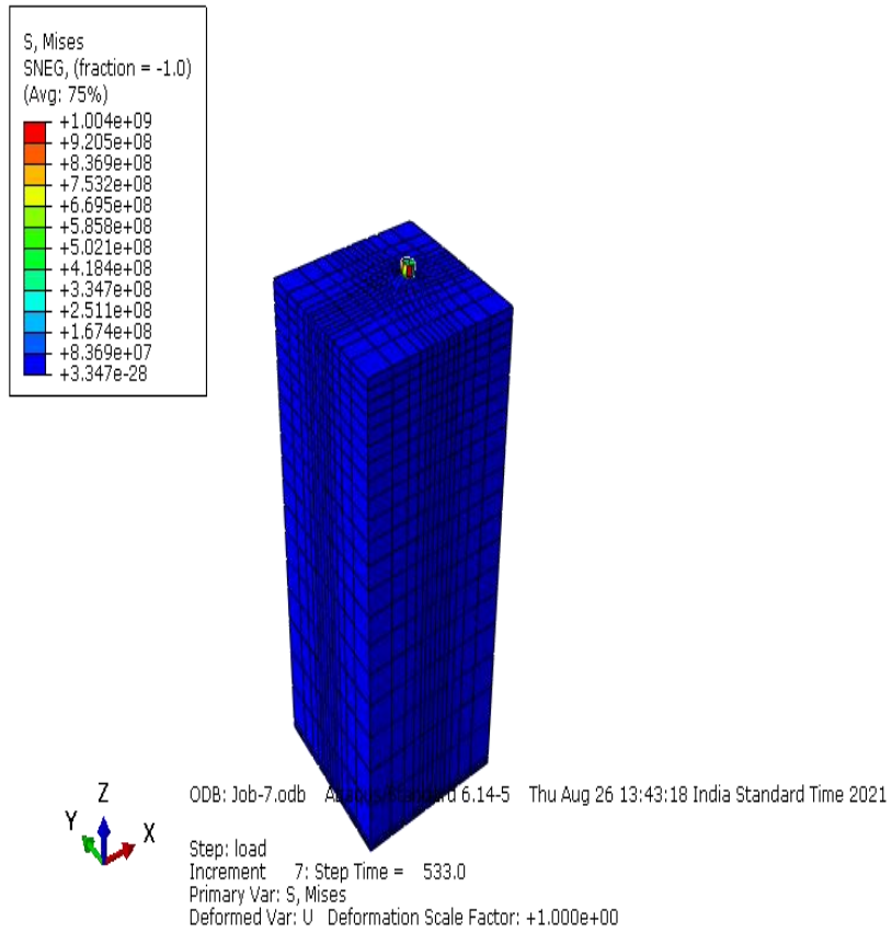
Figure 18- Stress variation in pile of thickness 20mm
