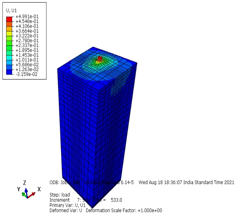
Figure 14- Displacement of the pile of thickness 10mm
