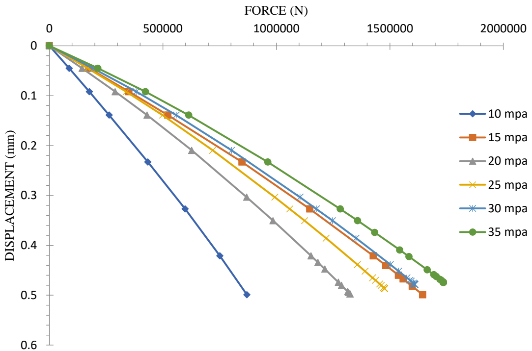
Figure 19- P-Y curve of pile 20mm thick for varying modulus of elasticity
