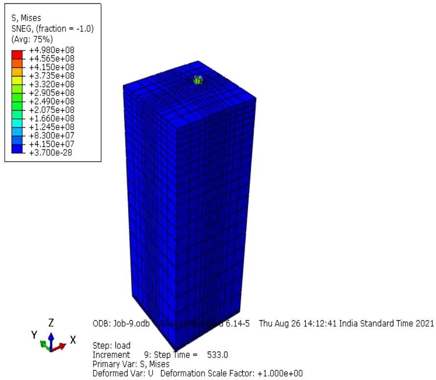
Figure 24- Stress variation in the pile of thickness 40mm
