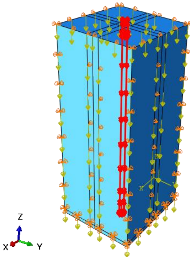
Figure 12- Body forces on the model
