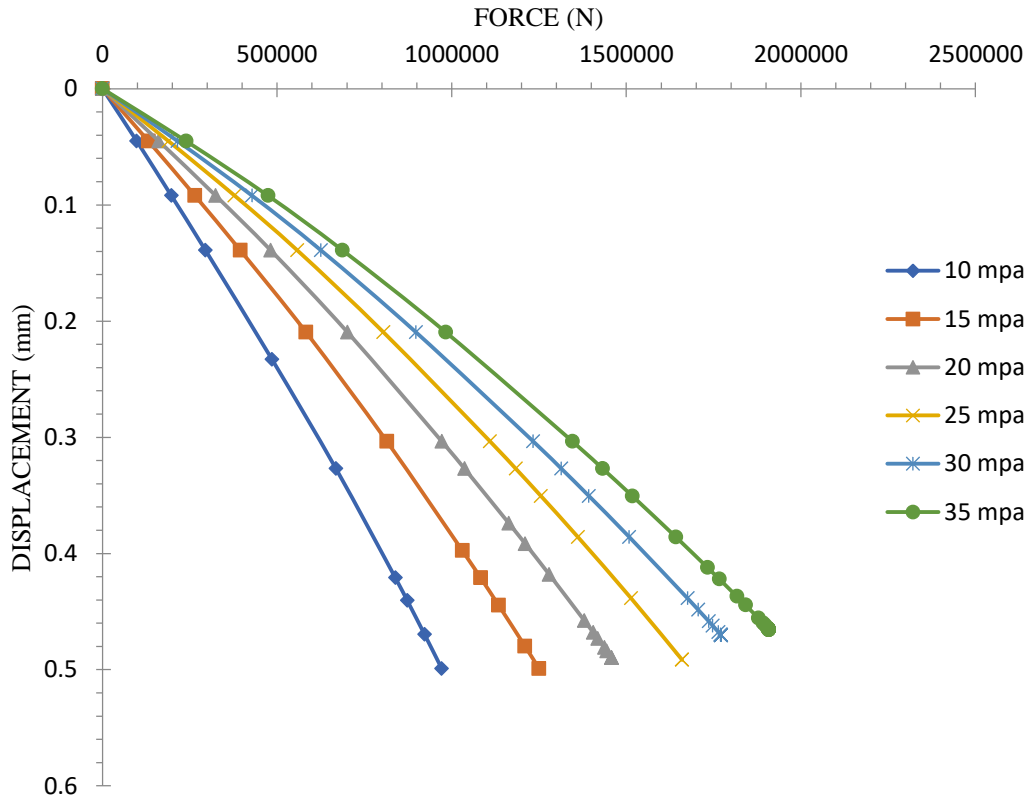
Figure 22-P-Y curve of pile 30mm thick for varying modulus of elasticity
