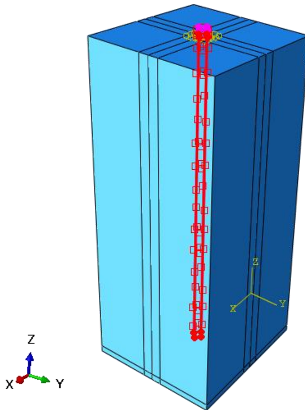
Figure 10- Interaction between soil and pile surface
