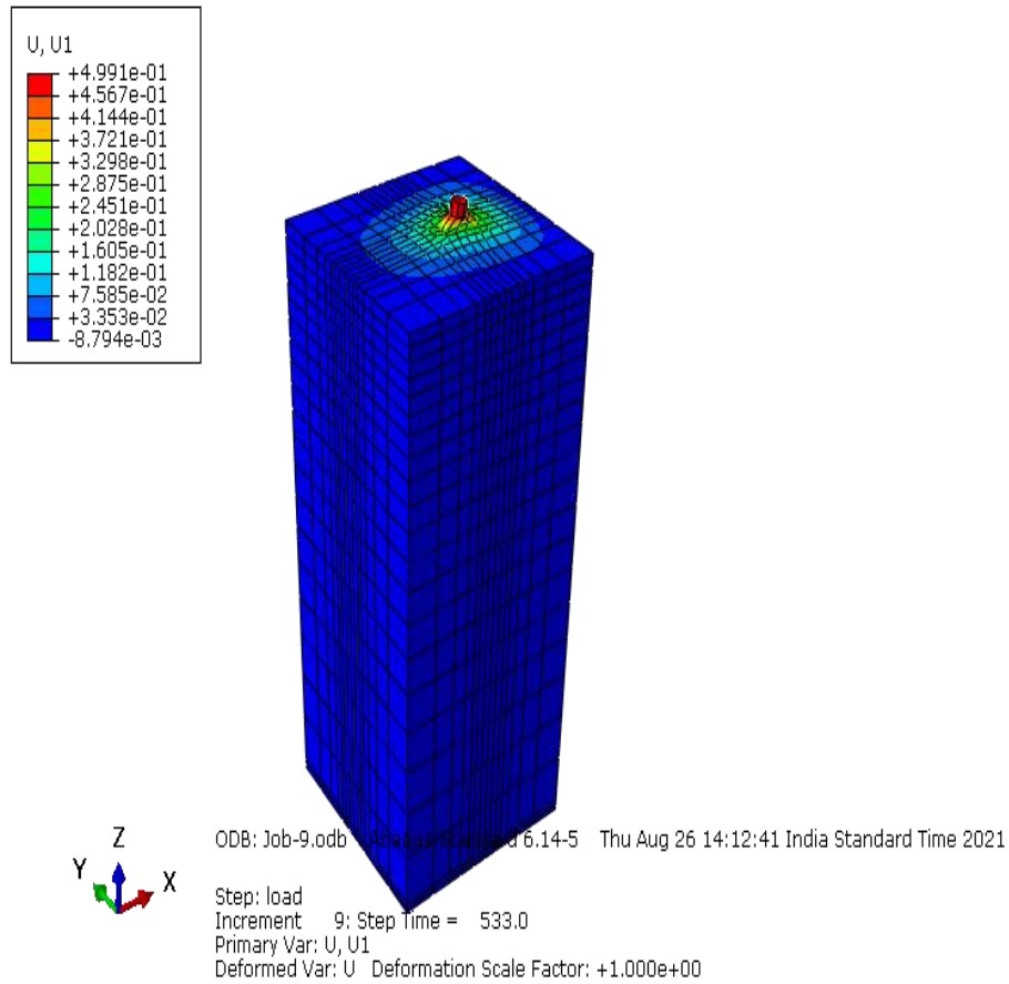
Figure 23- Displacement of the pile of thickness 40mm
