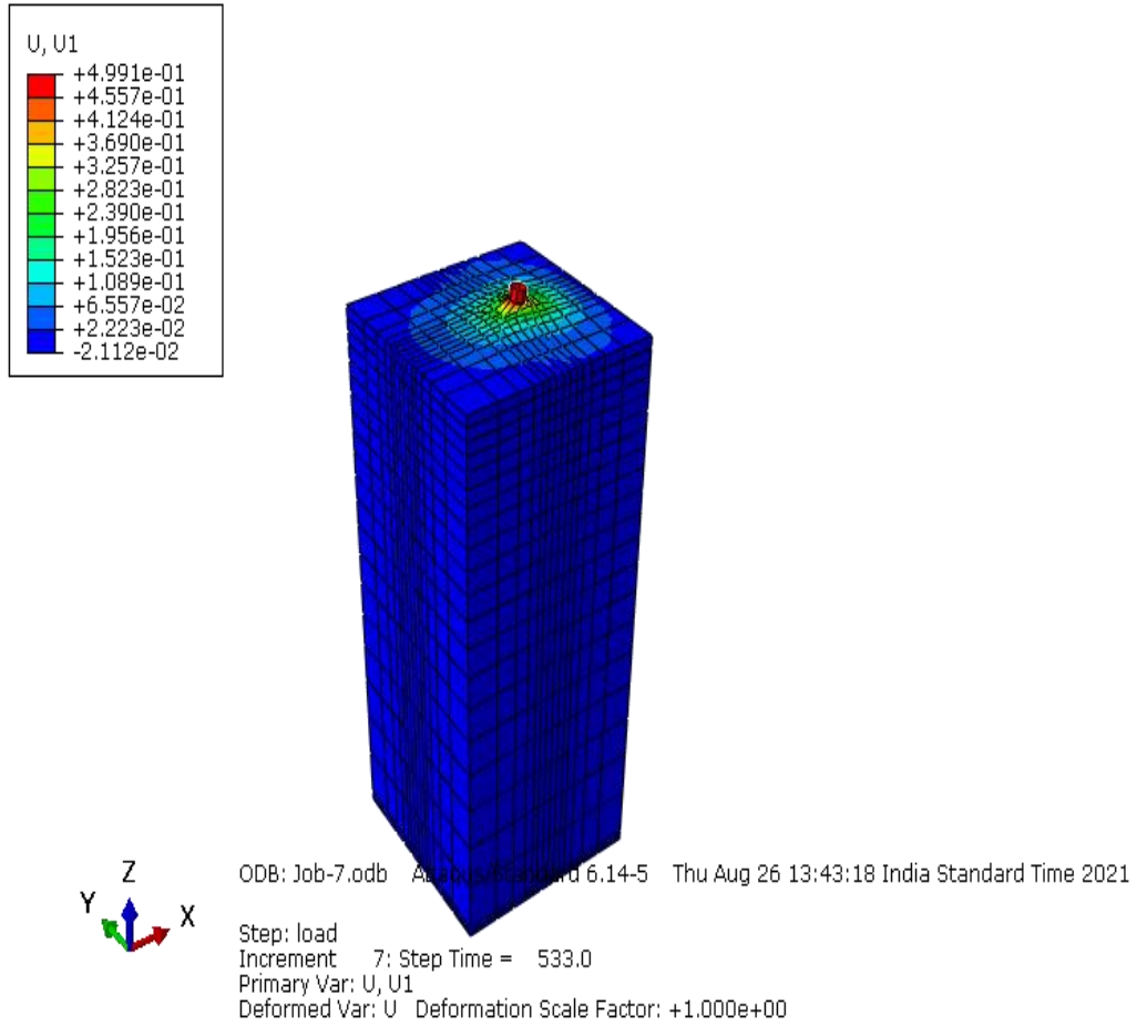
Figure 17- Displacement of pile of thickness 20mm
