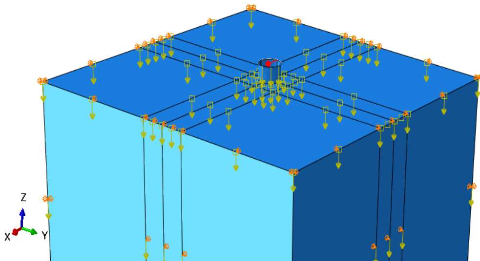
Figure 13- Lateral loading on the pile
