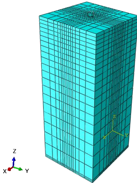
Figure 9- Whole model mesh
