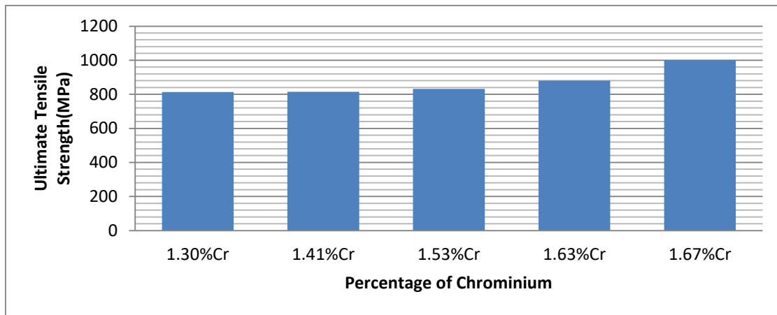
Fig. 5.3 Chromium vs Ultimate Tensile Strength
