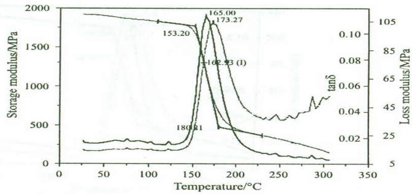
Fig. 2a DMA curve of PFM10 sample at 1 Hz frequency
