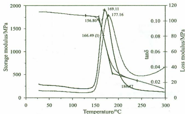
Fig. 3b DMA curve of PFBM10 sample at 10 Hz frequency
