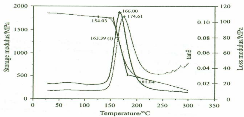
Fig. 3a DMA curve of PFBM10 sample at 1 Hz frequency
