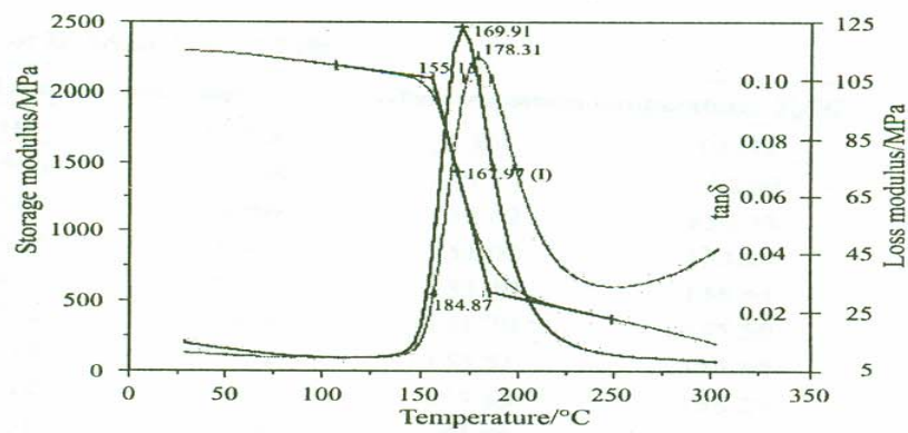
Fig. 2b DMA curve of PFM10 sample at 10 Hz frequency
