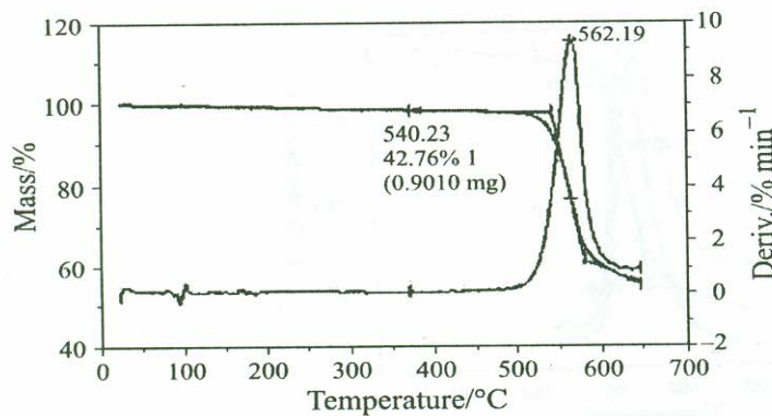
Fig. 1a Thermogravimetric trace of PFM10 samples
