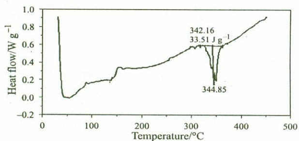
Fig. 4b DSC scan of PFBM10 sample
