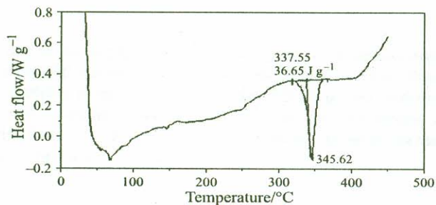
Fig. 4a DSC scan of PFM10 sample
