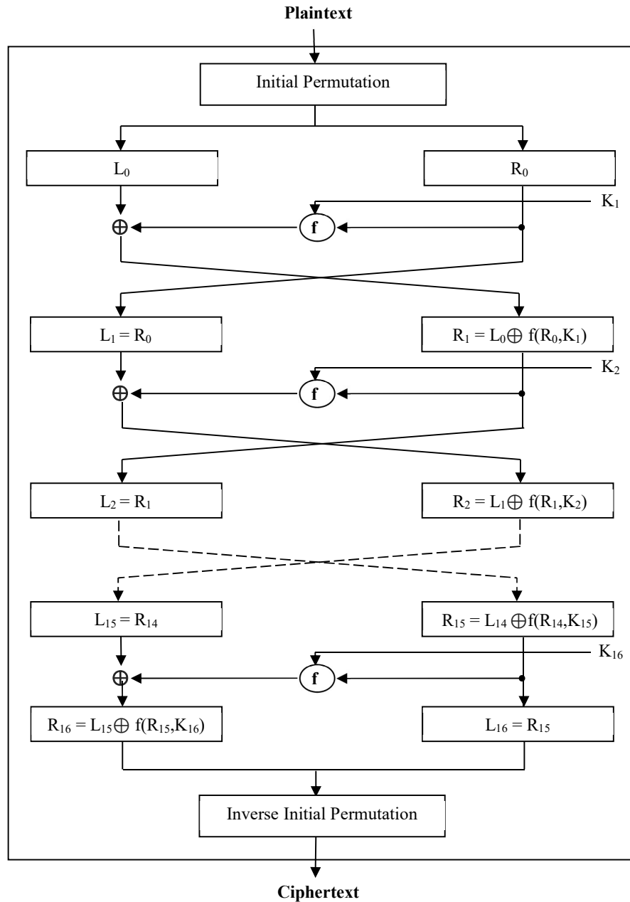
Fig. 1 Block Diagram for DES block cipher
