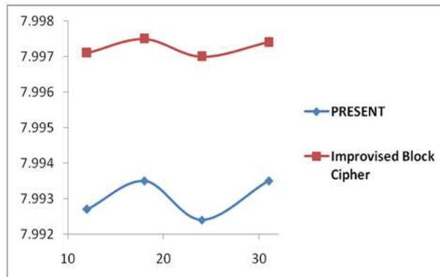
Fig. 20 Plot for comparison of Entropy Variation with change in number of Rounds for PRESENT vs Proposed Improved Block Cipher
