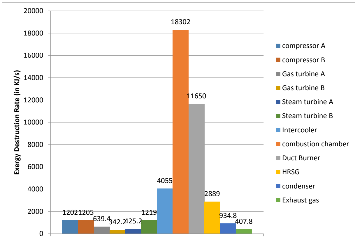
Fig 4.4 Exergy destruction rate in different components
