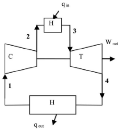
Fig.1.1 A closed cycle gas turbine [2]
