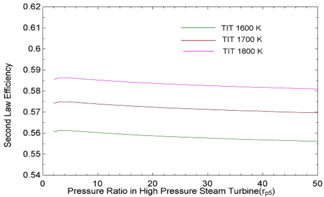
Fig 4.16 effect of pressure ratio of high pressure steam turbine on second law efficiency
