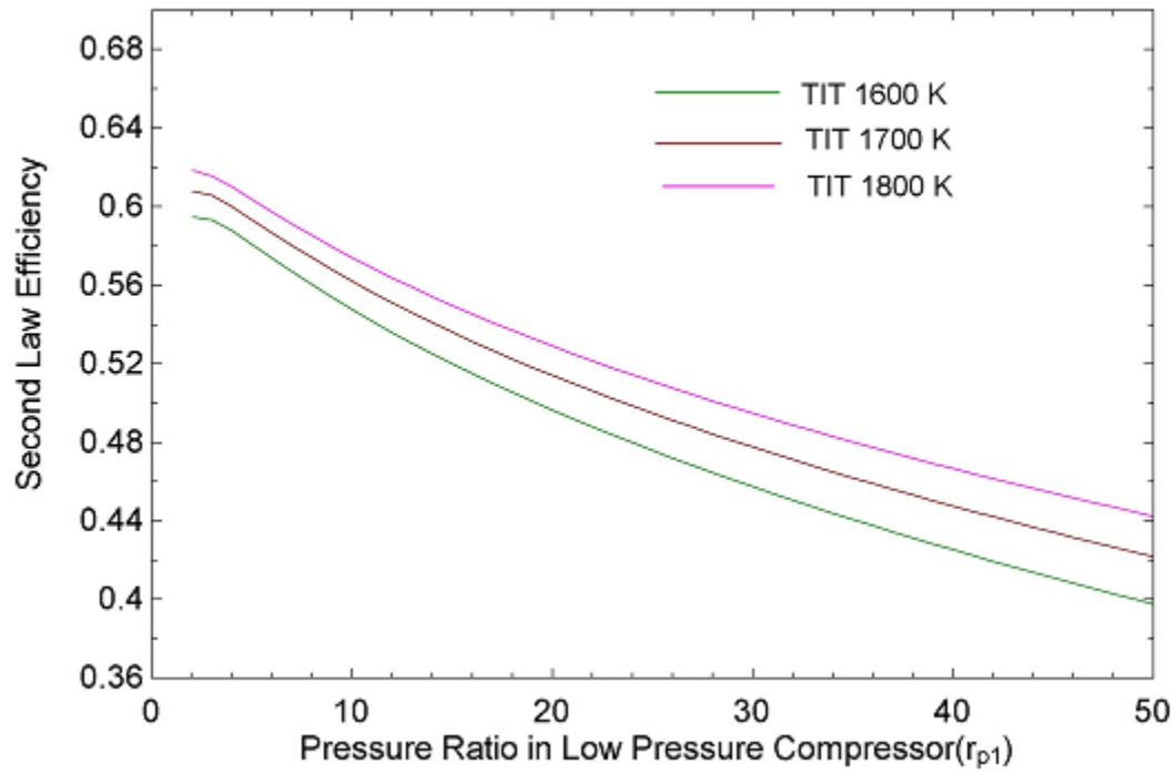
Fig 4.8 effect of pressure ratio in low pressure compressor on second law efficiency
