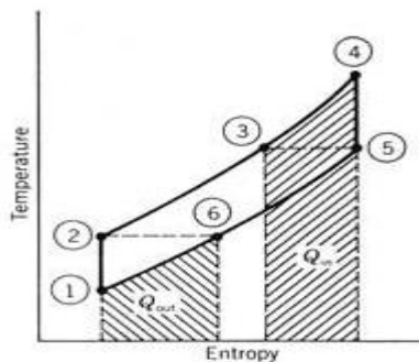
Fig. 1.4 T-s diagram of open regenerative Brayton cycle [2]
