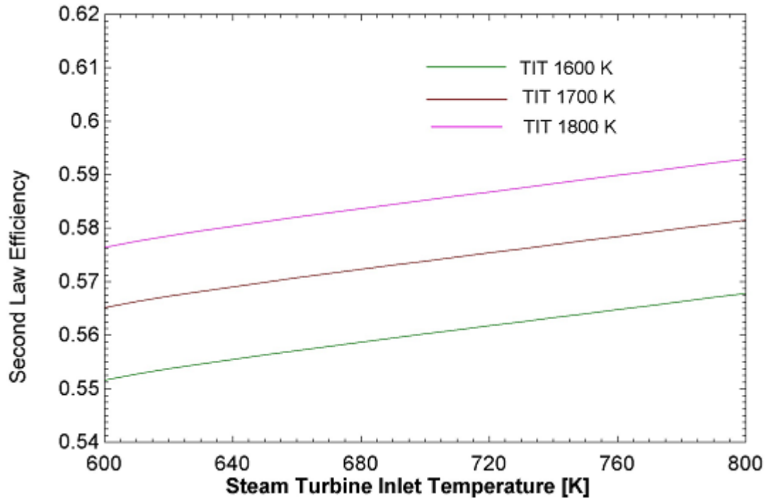
Fig 4.18 effect of steam turbine inlet temperature on second law efficiency
