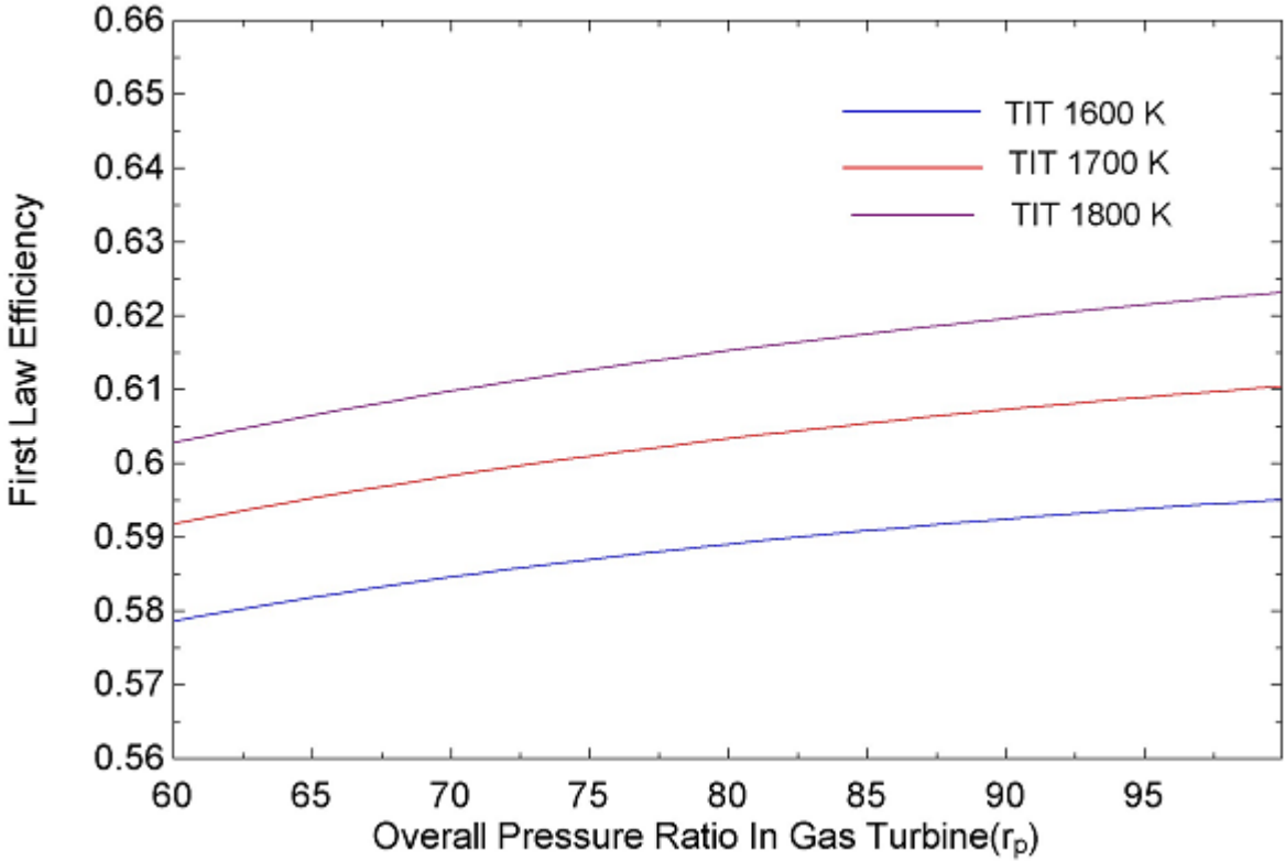
Fig 4.5 Variation of first law efficiency with overall pressure ratio in gas turbine
