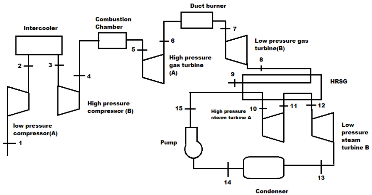
Fig.3.2 combined cycle gas turbine (in present analysis)
