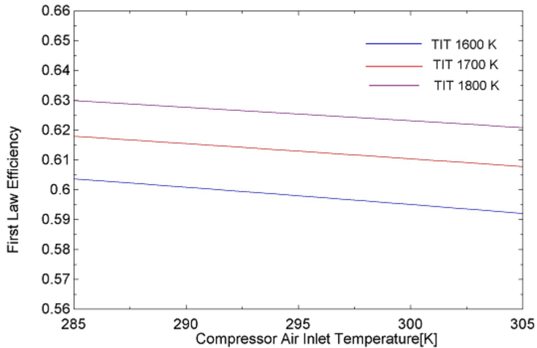
Fig 4.19 effect of compressor inlet air temperature on first law efficiency
