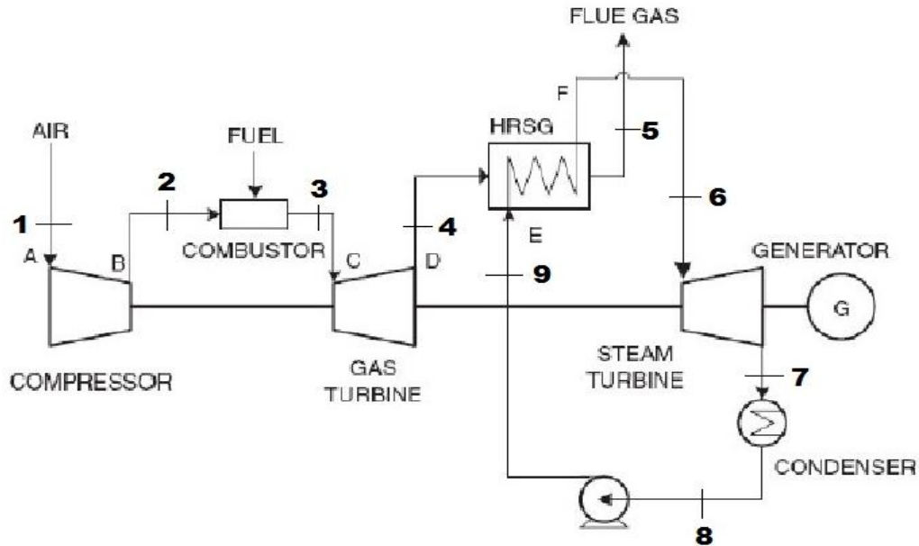
Fig. 4.1 Simple Combined Cycle Gas Turbine System
