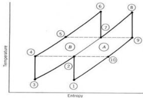
Fig.1.6 T-s diagram of open Brayton cycle with intercooling, reheat and regeneration [2]
