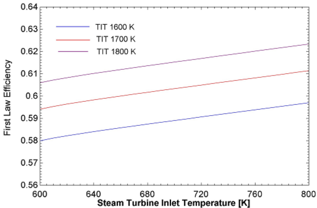
Fig 4.17 effect of steam turbine inlet temperature on first law efficiency
