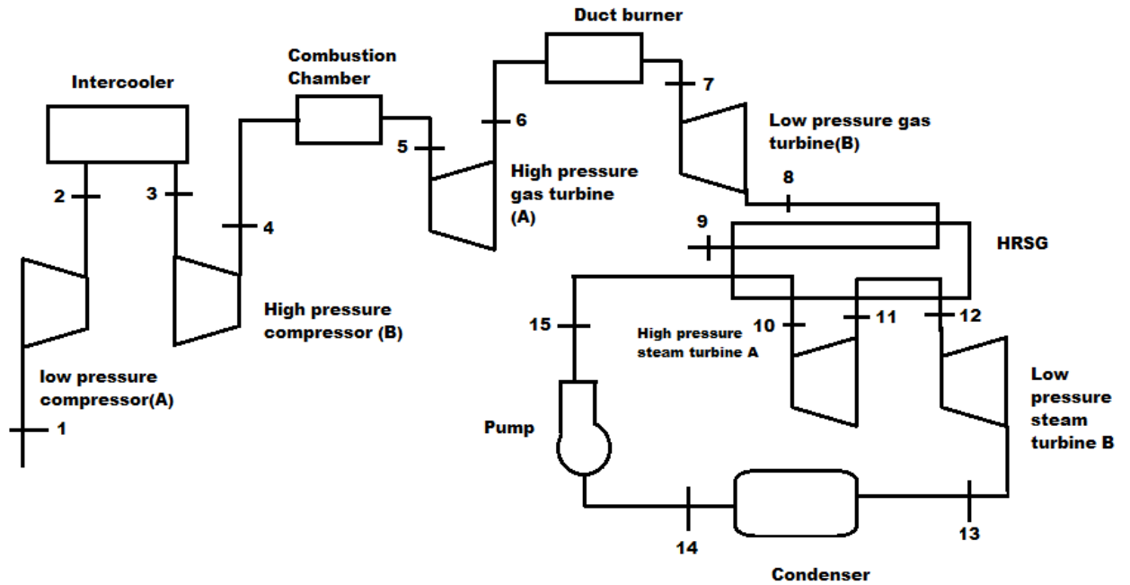
Fig. 4.2 modified combined cycle system
