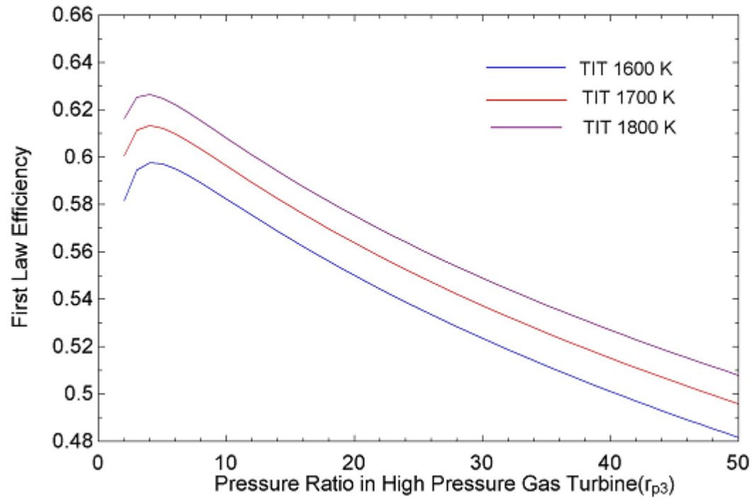
Fig 4.9 effect of pressure ratio in high pressure gas turbine on first law efficiency
