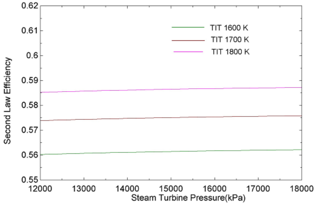
Fig 4.14 effect of steam turbine pressure on second law efficiency
