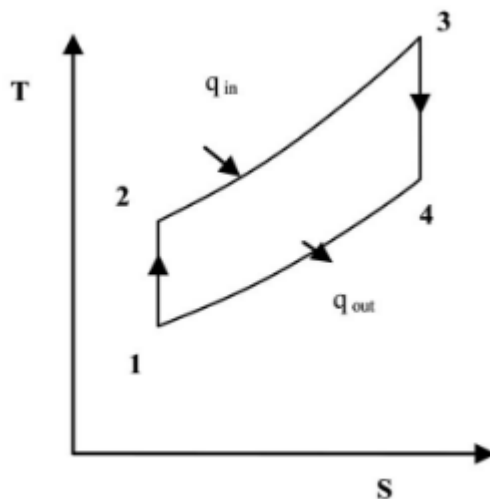
Fig.1.2 T-s diagram of Brayton cycle [2]
