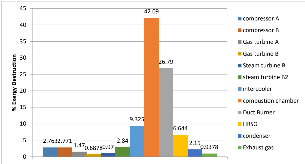
Fig. 4.3 % Exergy destruction of total Exergy destruction in different components
