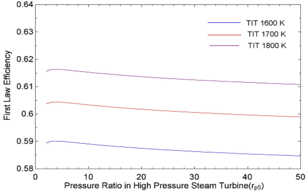
Fig 4.15 effect of pressure ratio of high pressure steam turbine on first law efficiency
