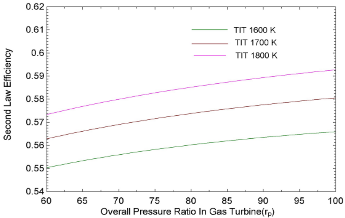
Fig 4.6 Variation of second law efficiency with overall pressure ratio in gas turbine
