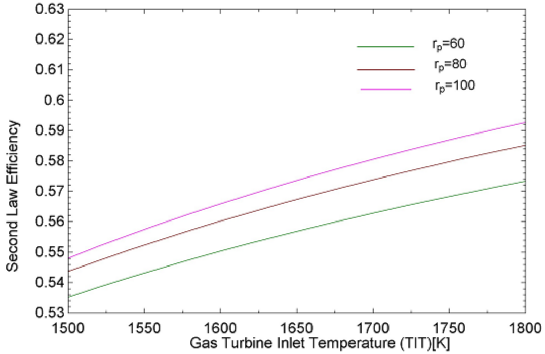
Fig 4.12 effect of gas turbine inlet temperature on second law efficiency
