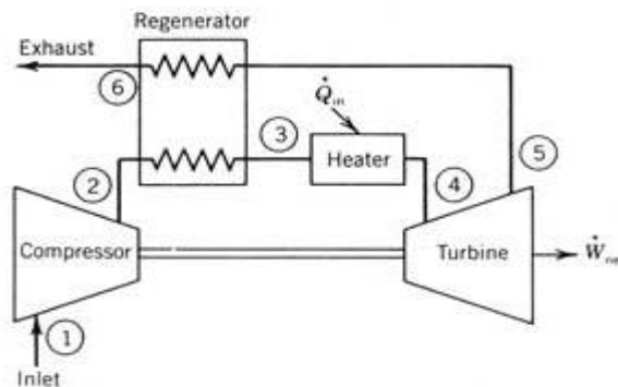
Fig.1.3 open regenerative Brayton cycle [2]
