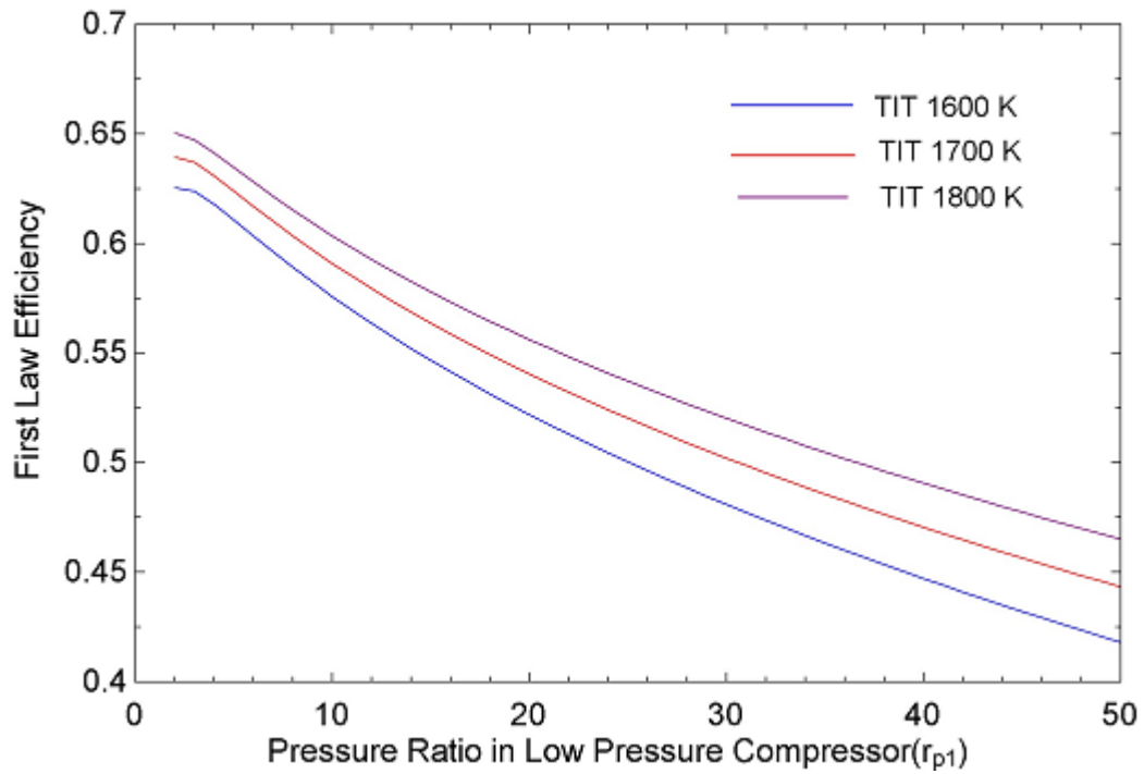
Fig 4.7 effect of pressure ratio in low pressure compressor on first law efficiency
