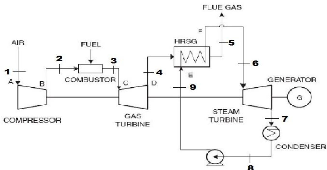
Fig.3.1 Simple combined cycle gas turbine
