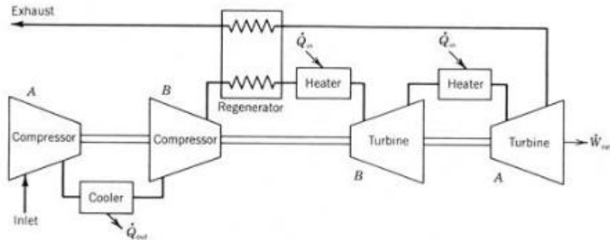
Fig. 1.5 open Brayton cycle with intercooling [2]
