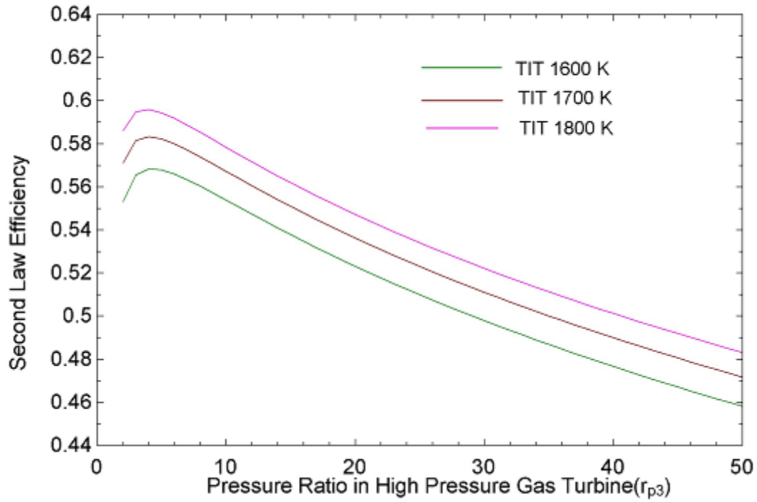
Fig 4.10 effect of pressure ratio in high pressure gas turbine on second law efficiency
