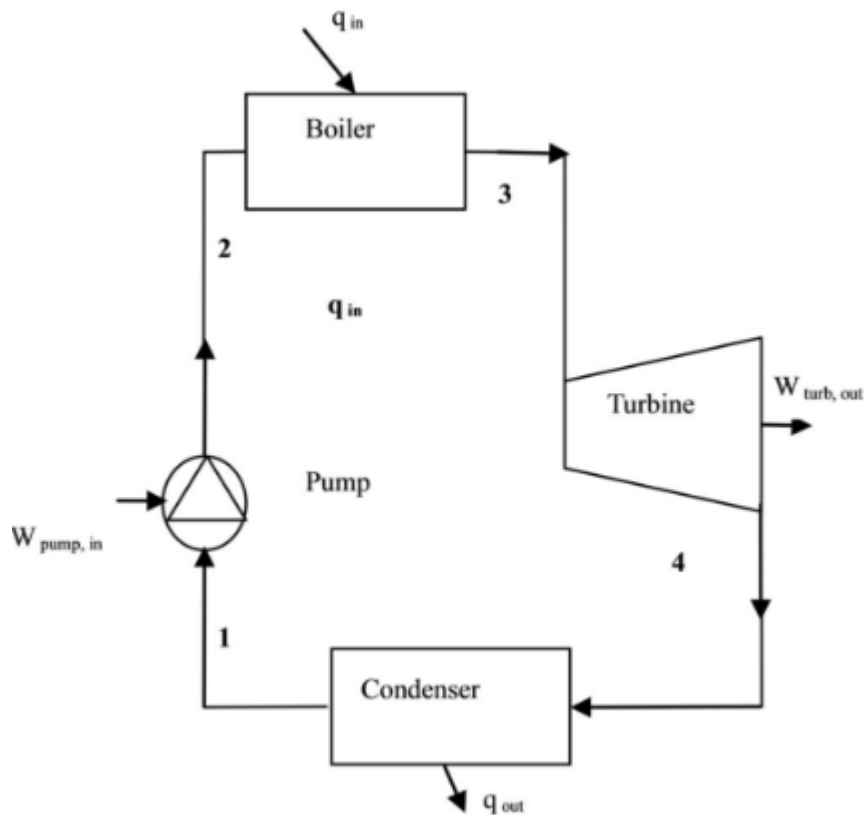
Fig. 1.7 simple Rankine cycle [2]
