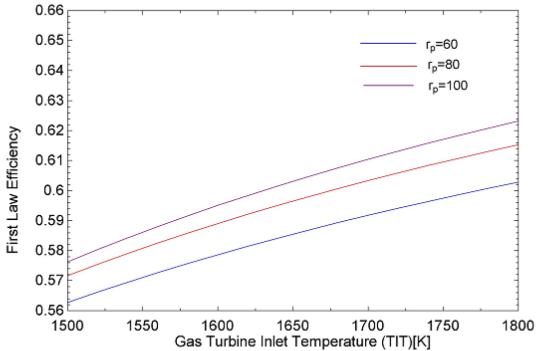
Fig 4.11 effect of gas turbine inlet temperature on first law efficiency
