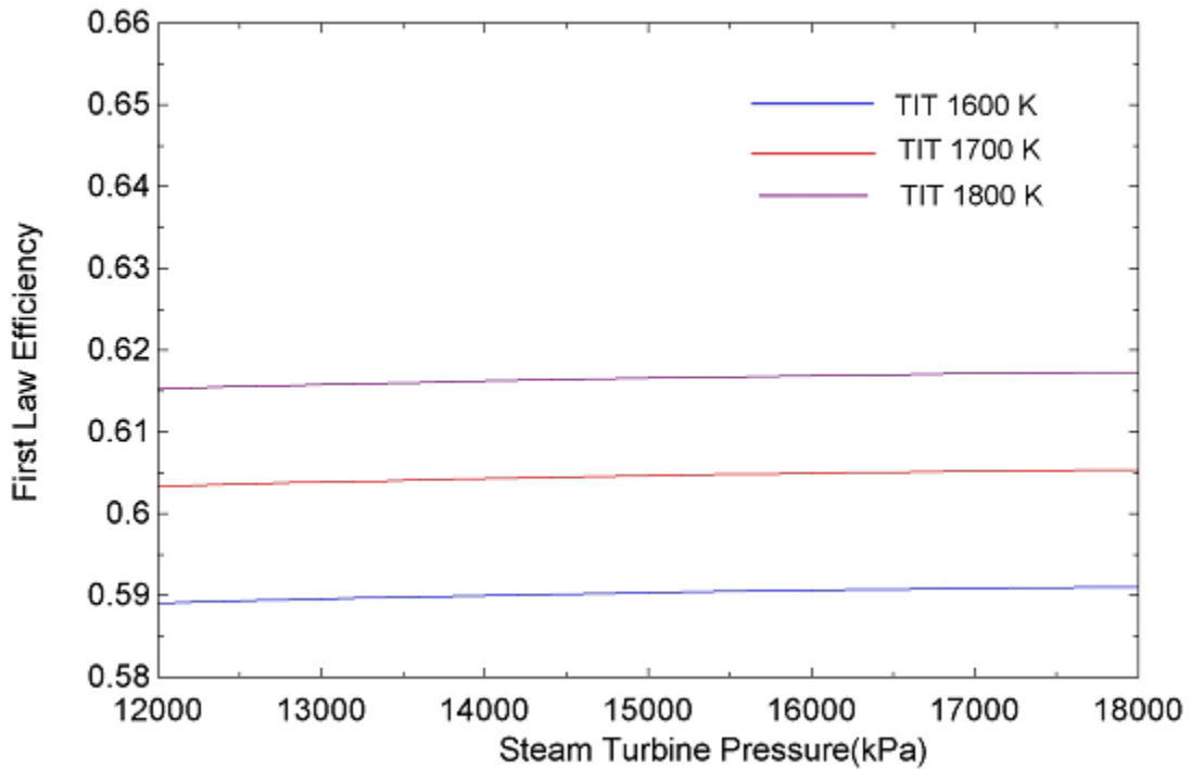
Fig 4.13 effect of steam turbine pressure on first law efficiency
